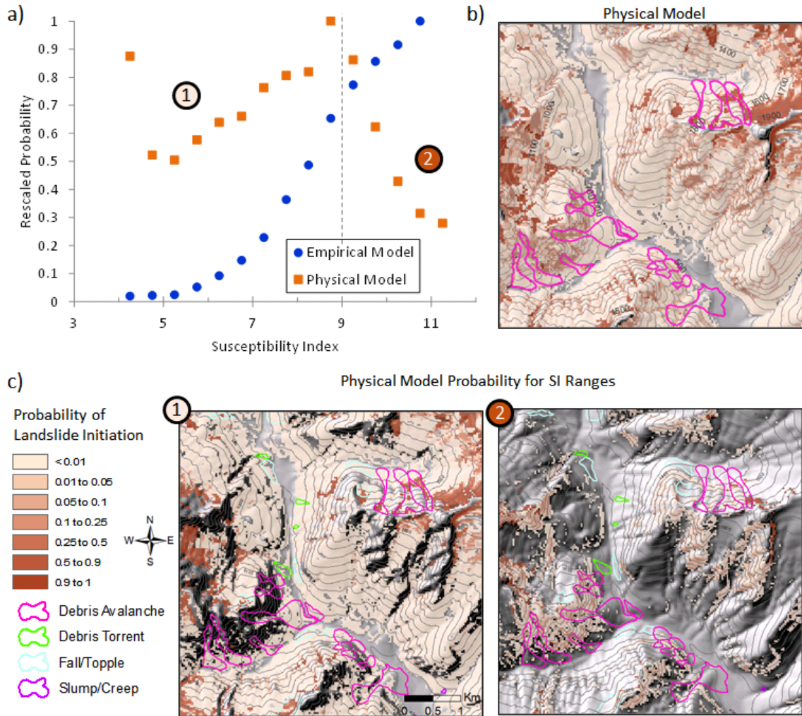
Figure 4.6 - a) Comparison of rescaled P(LS_r|SI_r) from empirical model for debris avalanche source areas with the mean probability of landslide initiation P(F) from the physical model within 0.5 size bins of SI (rescaled by dividing by maximum). Portion of NOCA showing: b) P(F) from physical model; and c) same area showing only P(F) corresponding to the two regions of SI (region 1: SI \leq 9 ; region 2: SI > 9 , depicted in (a)) overlain on hillshade. Location of the portion of NOCA shown as box in Fig. 4.7.
