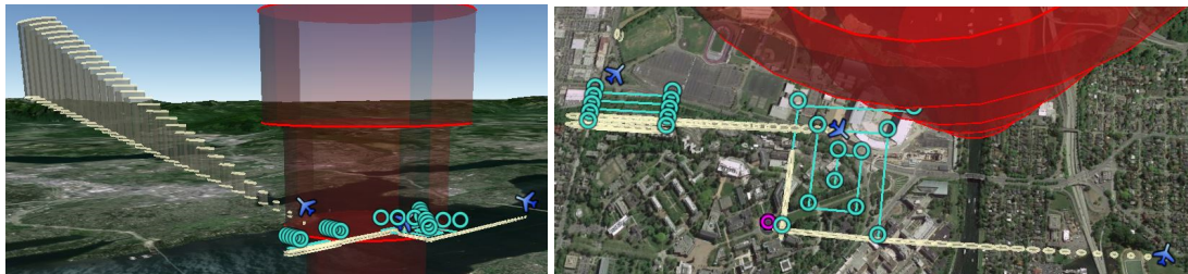
Figure 5.19: Simulation 1, FSE results at 45 secs side view (left) and top view (right)
