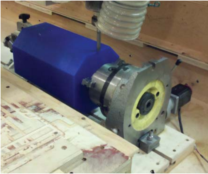
Figure 8: Stock material prior to CNC routing
