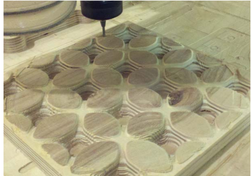
Figure 33: CNC routed plywood mold for second [m]form prototype membrane
