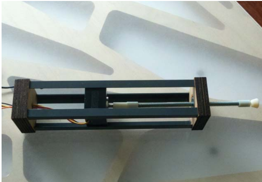
Figure 34: Forming rod unit with rails, stepper motor, & connectors
