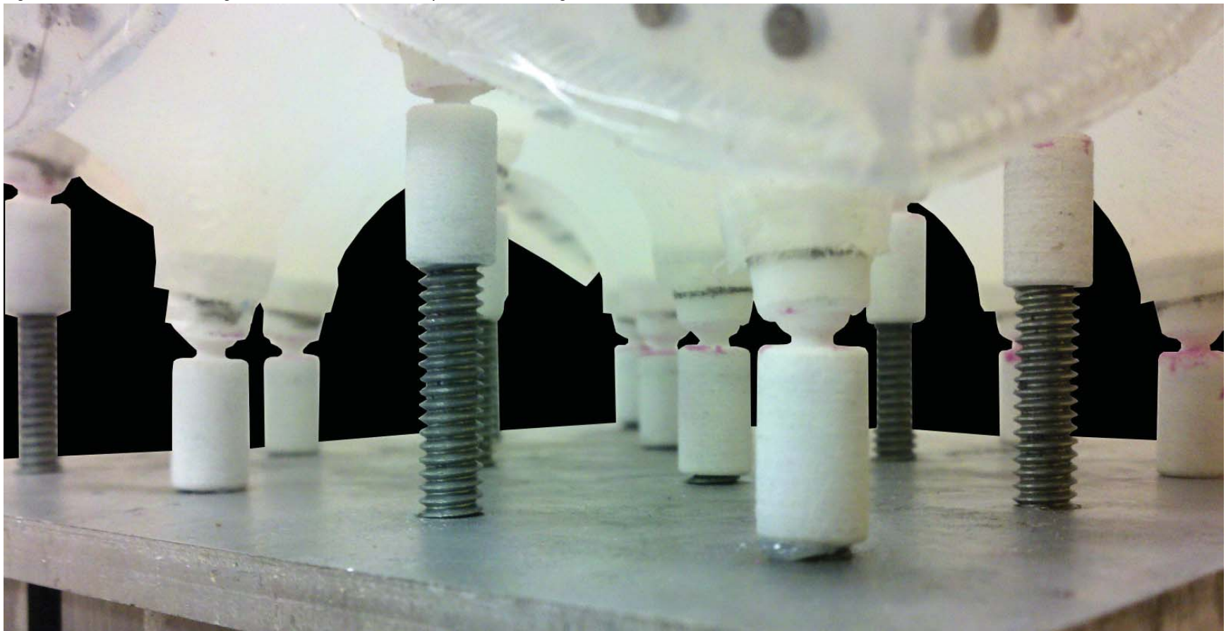
Figure 43: Backside of forming membrane showing 3-D printed nylon ball joints and 1/4"-20 threaded rods extending out of aluminum wall
