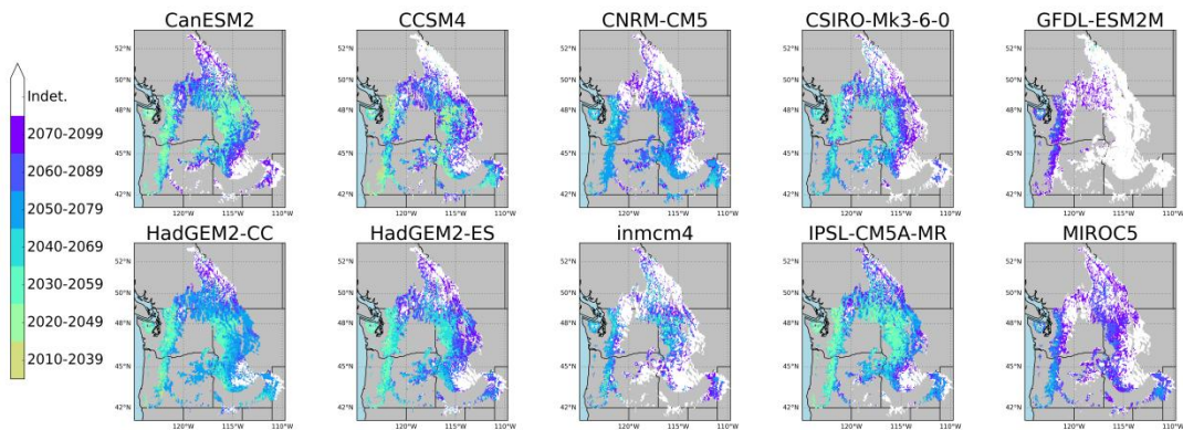
Annual maximum SWE: When will the 10th percentile of 1980-2009 become the 50th? As projected by 10 different GCMs and RCP 8.5
