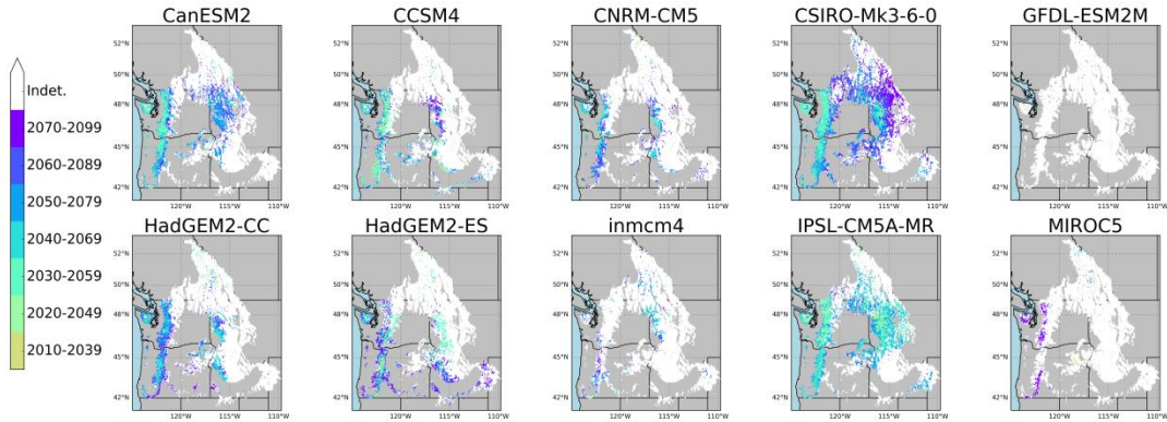
Annual maximum SWE: When will the 10th percentile of 1980-2009 become the 50th? As projected by 10 different GCMs and RCP 4.5
