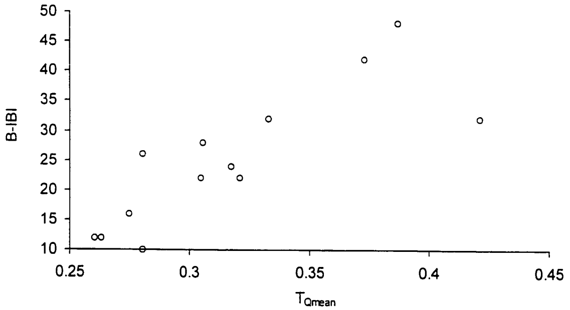
Figure 2:17: Benthic index of biological integrity (B-IBI) plotted against fraction of time that daily mean discharge rate exceeds annual mean discharge rate ( T_{Qmean} ) for 13 Puget Lowland streams.
