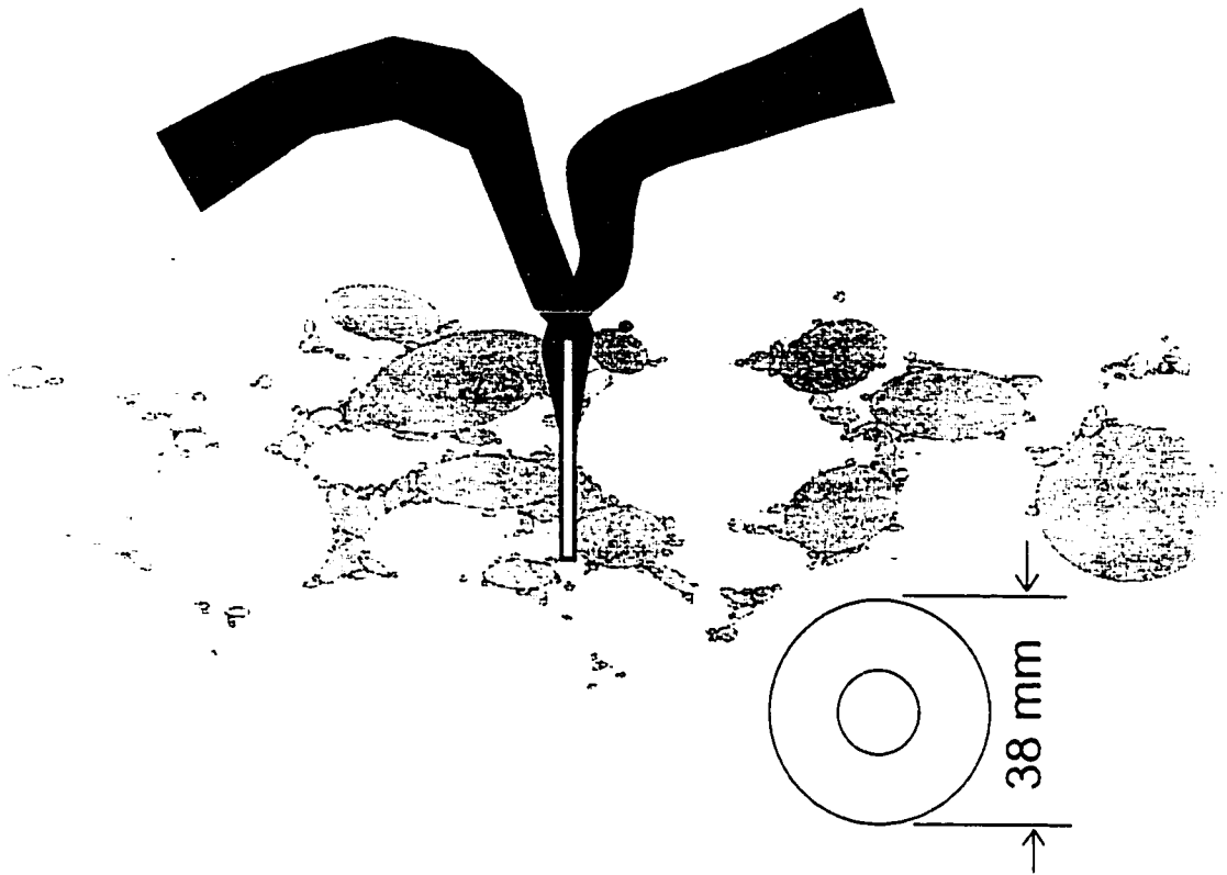
Figure 4.5: Cross-section of bed tag placement in a stream bed.
