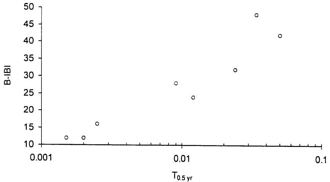
Figure 2.19: Benthic index of biological integrity (B-IBI) plotted against the fraction of the period of record that discharge exceeded the magnitude of a "1/2 yr" flood ( T_{0.5,yr} ) for 8 Puget Lowland streams.
