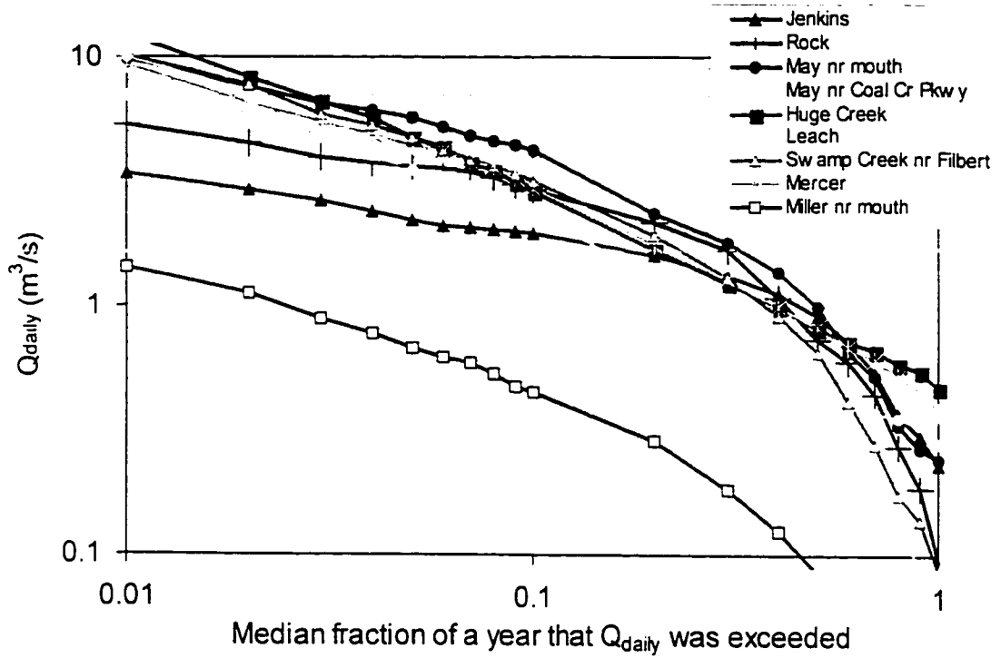
Figure 2.6: Median annual flow duration curves for Puget Lowland streams.
