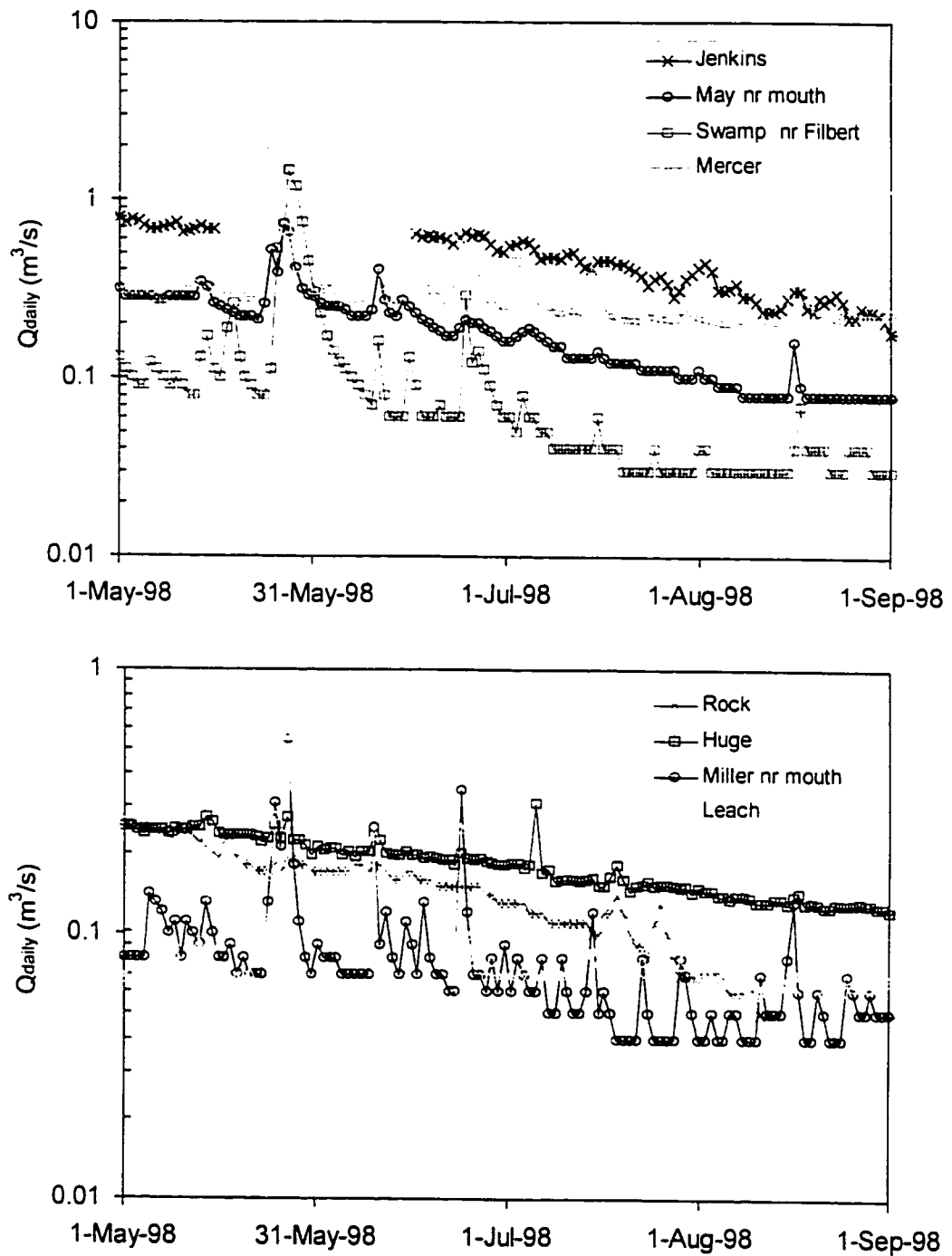
Figure 2.3: Daily mean discharge rate ( Q_{\text{daily}} ) for 8 Puget Lowland streams from 1 May to 1 September 1998.
