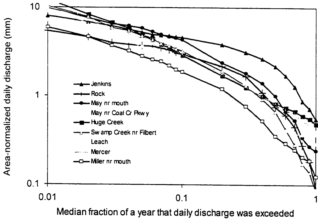
Figure 2.7: Area-normalized, median annual flow duration curves.
