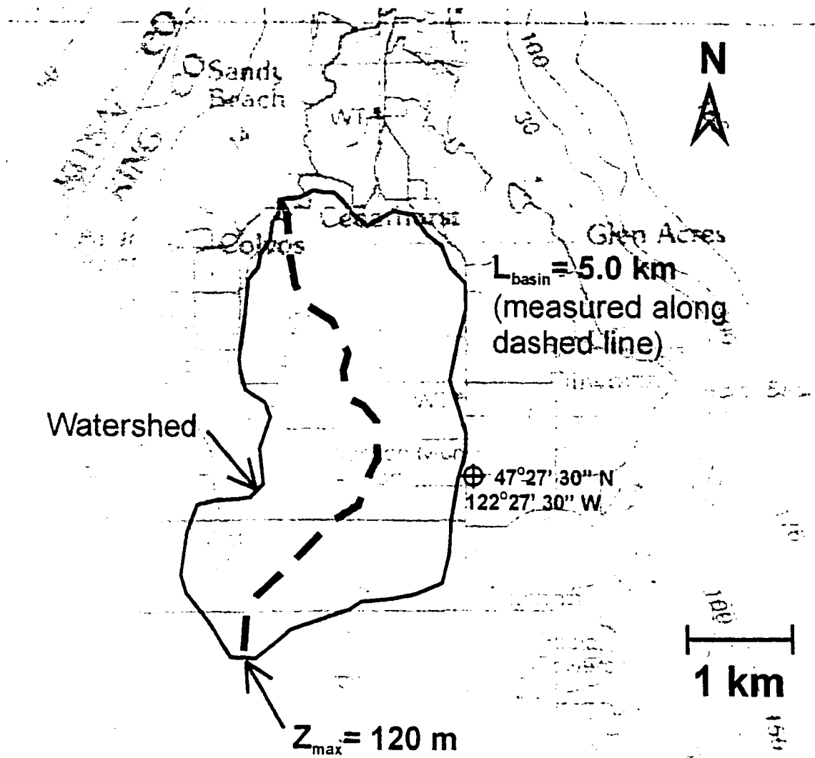
Figure 3.2: Shinglemill Creek basin showing the watershed, basin length ( L_{\text{basin}} ), and point of maximum valley elevation ( Z_{\text{max}} ). Source: USGS Vashon 7.5 minute quadrangle, 1: 24,000.
