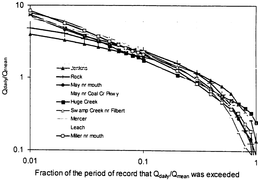
Figure 2.9a: Daily flow duration curves normalized by mean discharge rate.
