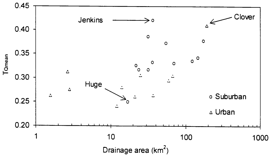
Figure 2.12: Fraction of year that daily mean discharge rate exceeded annual mean discharge rate ( T_{Qmean} ) as a function of drainage area for 18 streams during WY1989-1998.
