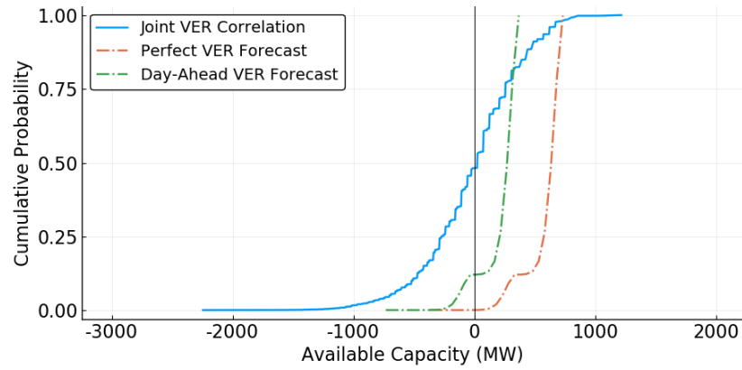
(b) Medium VER, Region 5
