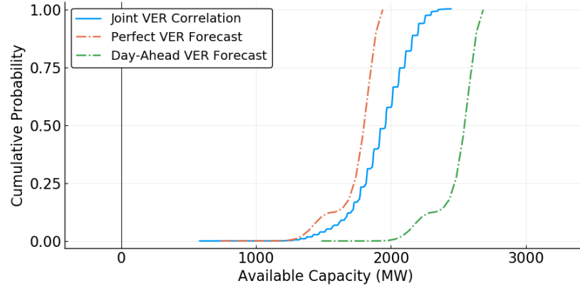
(a) Low VER, Region 3
