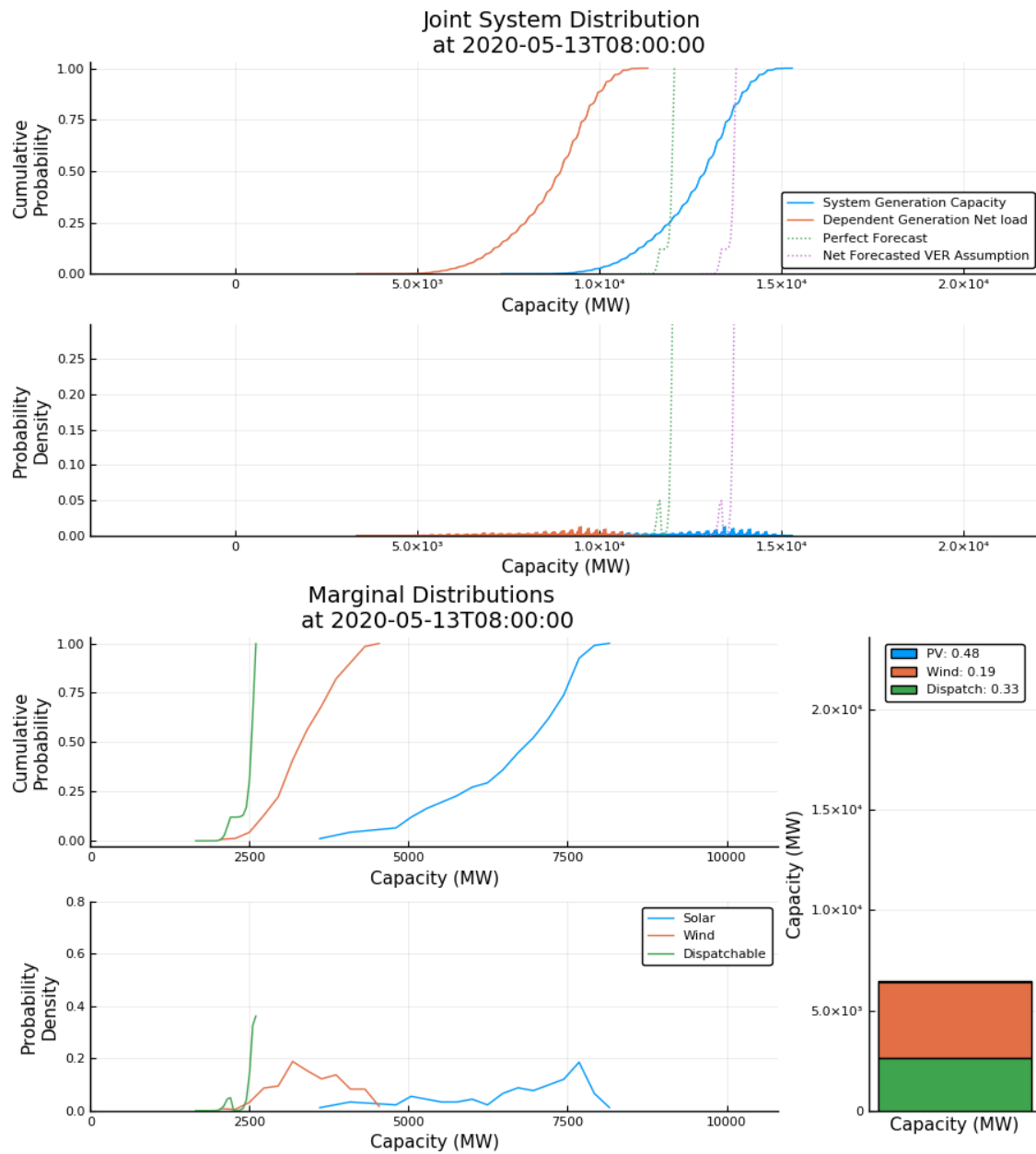
Figure A.3: Scenario summary from Region 5, high VER, spring morning
