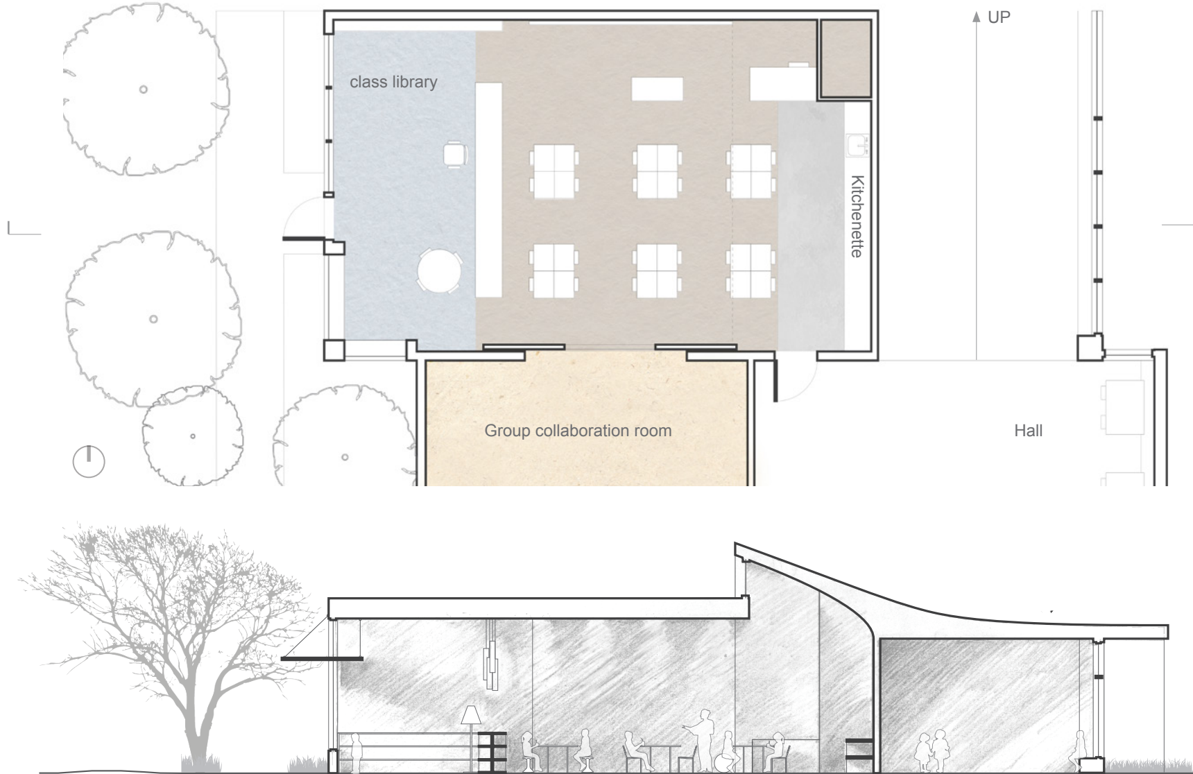
Figure 53.1 Representative Classroom Plan (Above)
