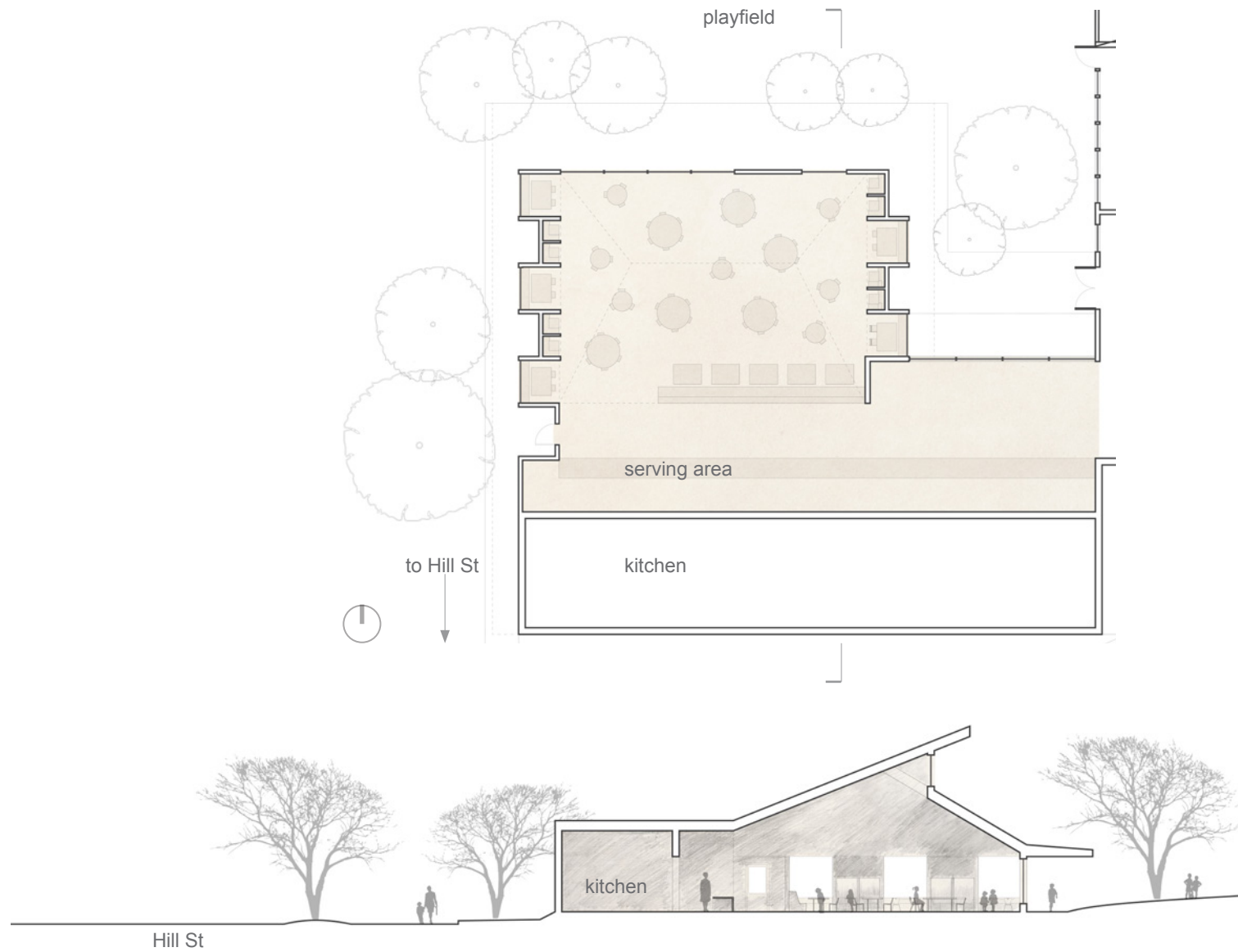
Figure 59.1 Dining Hall Plan
