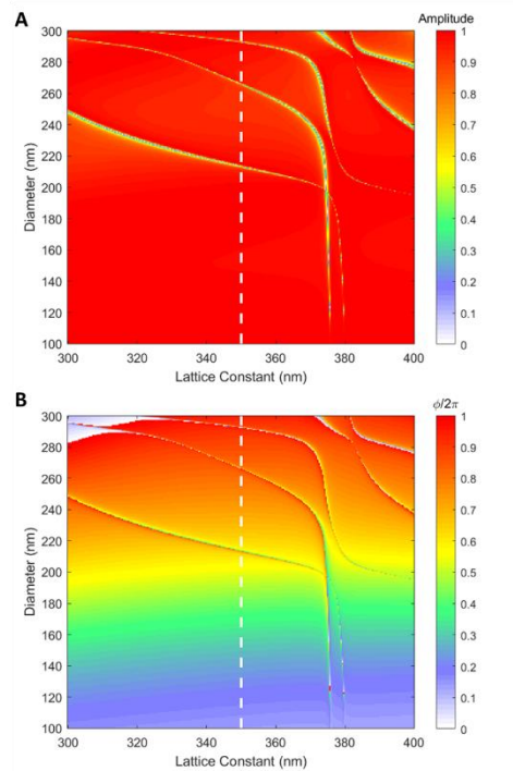
Figure 5.8. Transmission coefficient as a function of diameter and lattice constant. The transmission amplitude (A) and phase (B) are shown as a function of diameter and lattice constant at 530 nm wavelength. The white dashed line indicates the lattice constant value used for the nanopost design in the main text.
