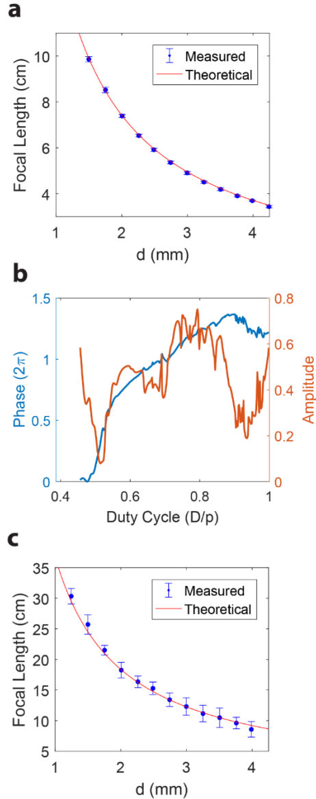
Figure 4.3. Experimental and theoretical focal lengths of the tunable lens designs. Focal length as a function of lateral displacement for the infrared (a) and visible (c) designs are shown. Errors bars represent a 95% confidence interval where the 1\sigma uncertainty is estimated during measurement by finding the range of distances over which the lens appears to be in focus. (b) Simulated transmission coefficient of the 1.5 \mu\text{m} thick silicon nitride nanoposts on a quartz substrate.
