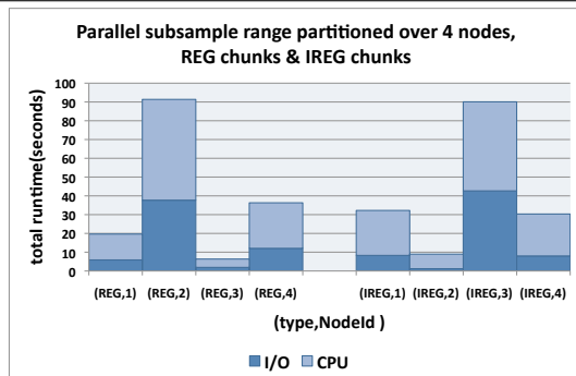
Figure 2.8 Parallel subsample with REG or IREG chunks distributed using range partitioning across 4 nodes. Subsample runs only on a few nodes causing skew, independent of the chunking scheme chosen.
