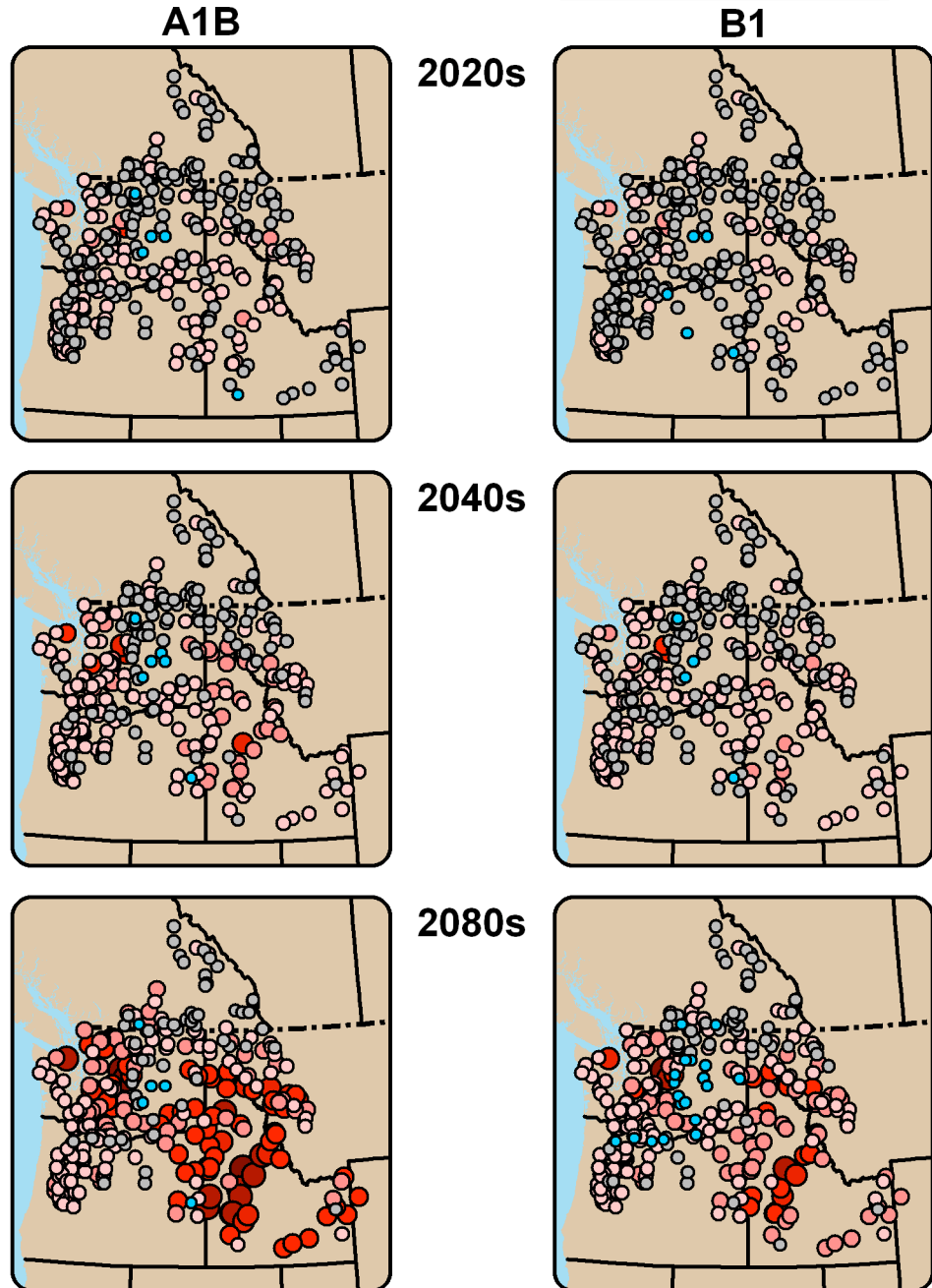
Figure 5: Maps of the ratio of the 100-year flood magnitude (future/ historical) for three future time intervals, under two scenarios. (Higher ratios indicate more intense flooding events projected for the future).
