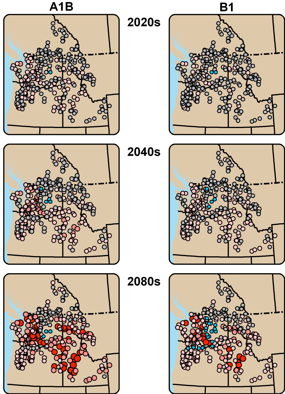
Figure 3: Maps of the ratio of the 20-year flood magnitude (future/ historical) for three future time intervals, under two scenarios. (Higher ratios indicate more intense flooding events projected for the future).
