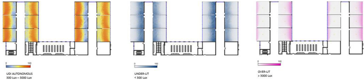
Image ccc: False color for First floor
