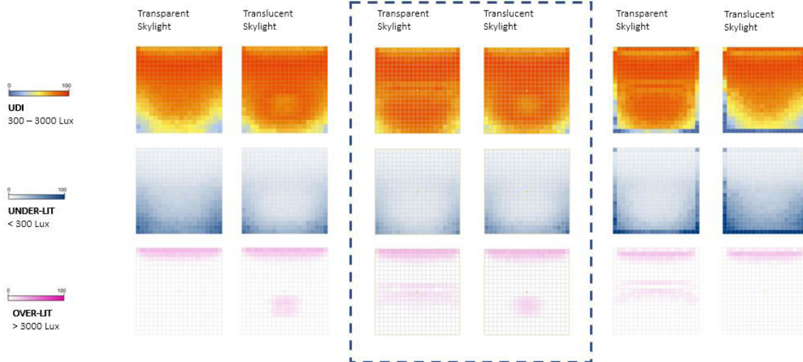
Image p : Daylight analysis for top-lighting for North facing Classrooms with 75% window to wall ratio
