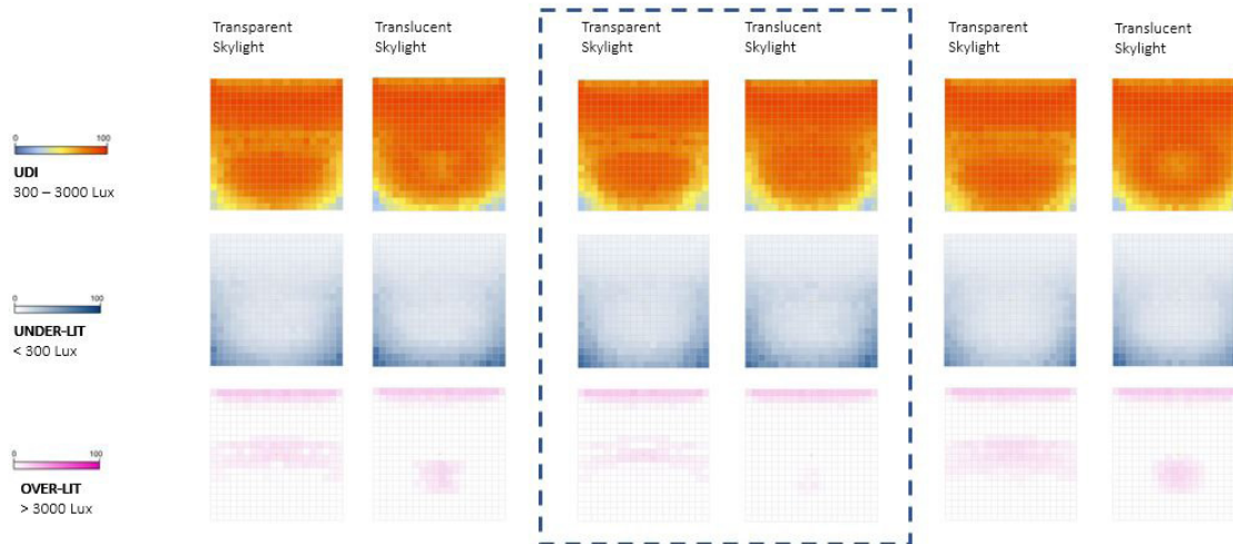
Image q : Daylight analysis for top-lighting for North facing Classrooms with 65% window to wall ratio
