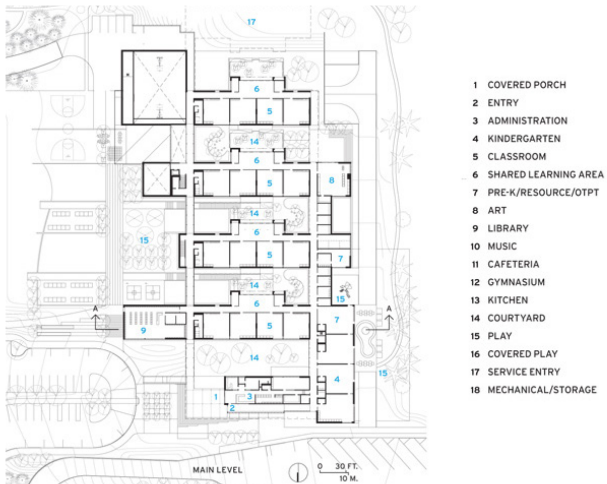
Image d: Site Plan for the Wilkes Elementary School
