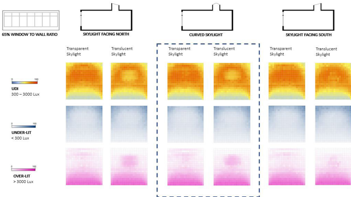
Image y : Daylight analysis for top-lighting for South facing Classrooms with 65% window to wall ratio
