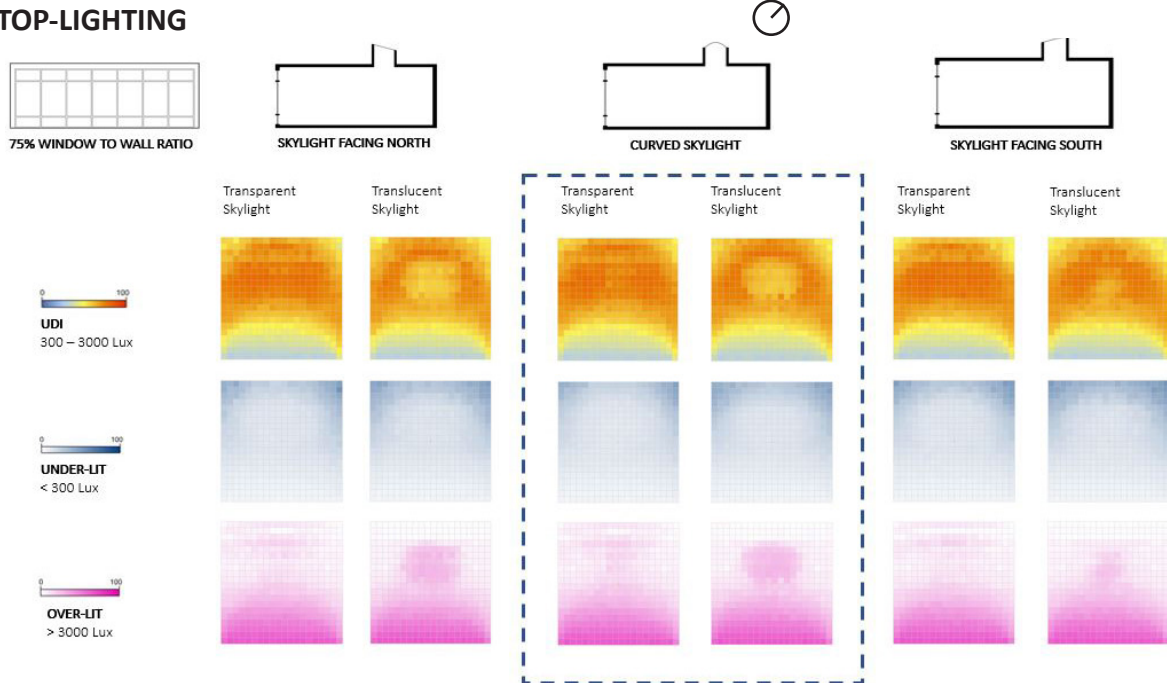
Image x : Daylight analysis for top-lighting for South facing Classrooms with 75% window to wall ratio
