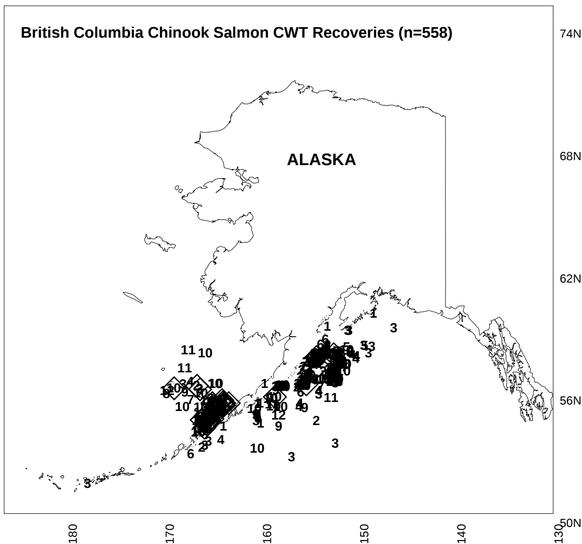
Fig. 12. Recovery locations of coded-wire tagged (CWT) British Columbia chinook salmon caught by U.S. and joint-venture groundfish (trawl) fishery vessels in the eastern Bering Sea and Gulf of Alaska (north of 50°N), 1982-2003 (adapted from Myers et al. 2001). The numbers at each location indicate the month of recovery. Twenty-three new recoveries reported by Myers et al. (2003) are indicated by open diamonds.
