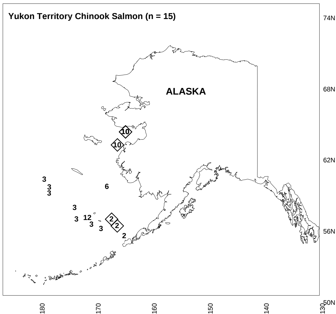
Fig. 9. Recovery locations of coded-wire tagged (CWT) Yukon River (Yukon Territory) hatchery chinook salmon caught by U.S. research and groundfish (trawl) fishery vessels in the eastern Bering Sea, 1992-2003. The numbers at each location indicate the month of recovery (adapted from Myers et al. 2001). Five new recoveries reported by Myers et al. (2003) are indicated by open diamonds (two overlap at the northernmost location). Three new recoveries of coded-wire tagged juvenile (ocean age-0) fish during a U.S. NMFS survey in October 2002 at 64°06'N, 164°31'W (2 recoveries) and at 63°00'N, 165°58'W are northern extensions of the known ocean range of Yukon River chinook salmon. Two new recoveries in February show the overwintering location of Yukon River salmon during their first winter at sea.
