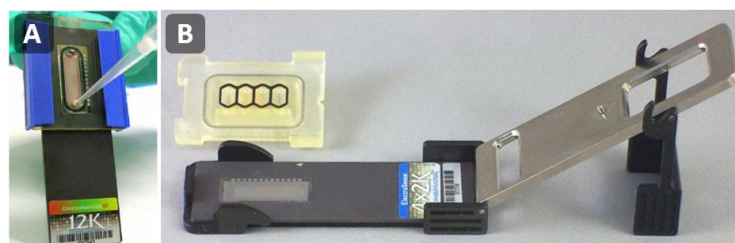
Figure 14. (A) The single chamber flow cell is clamped against the chip using plastic clips on either side. (B) The four-chamber flow cell requires a clamping structure to secure it in place.
