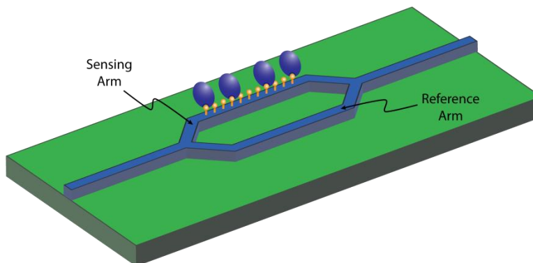
Figure 11. Schematic representation of a chip-based MZI biosensor. Changes in the RI surrounding the sensing arm induce a phase change, resulting in interference upon recombination with the reference arm.
