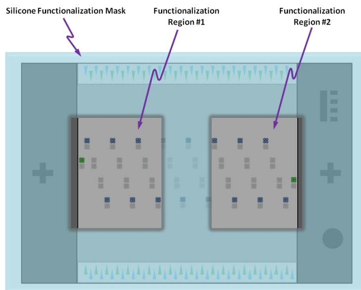
Figure 29. Schematic of the silicone functionalization mask overlaid on top of the sensor chips. Two openings are cut into the silicone that correspond to groups of rings (24 addressable rings, indicated in blue, in each opening). 16 rings are left covered, and the hydrophobic nature of the silicone prevents aqueous solutions from wicking underneath the mask.
