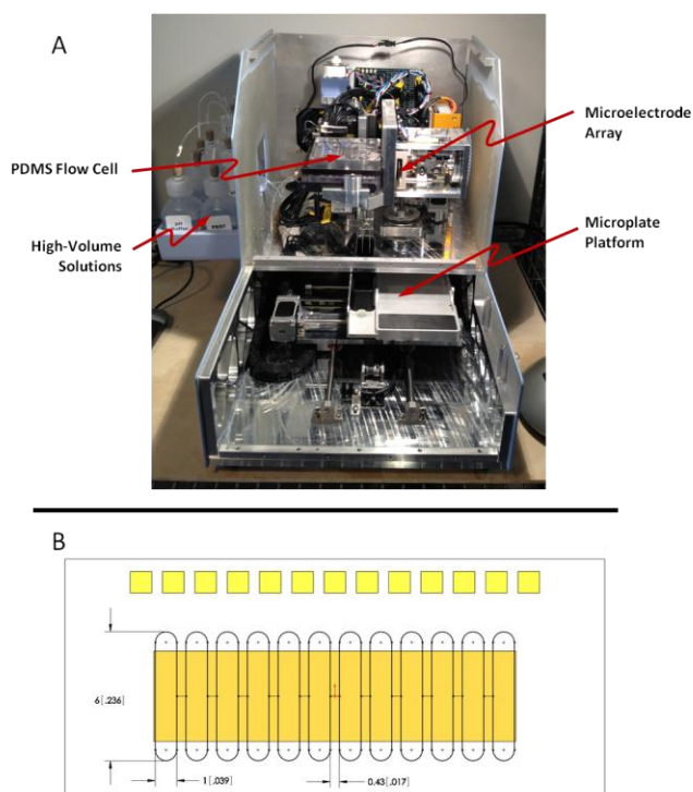
Figure 17. (A) Picture of the MX3120 with the cover removed to expose the internal components. Some of the primary components are highlighted. The PDMS flow cell (i.e. the CFM) is enclosed in a plexiglass casing. The “High-Volume Solutions” include buffers and cleaning reagents that are used in high volumes. The microelectrode array is inserted horizontally in a slot such that the CFM can be pressed onto the array surface. A 96-well plate is placed on the “Microplate Platform,” from which reagents are pulled by a fluidic pump (not shown). (B) Schematic representation of the flow cells as they are overlaid on the microelectrode array.
