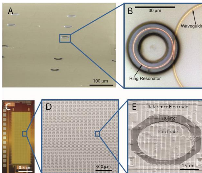
Figure 6. Two examples of multiplexed biosensor platforms, both of which are used in this research. (A) Each donut-shaped depression seen in the scanning electron micrograph represents an individual microring resonator (B) exposed through lithographic etching of a polymer coating. Microrings are interrogated with a bus waveguide that comes within 100nm of the resonator. C-E illustrate a commercial microelectrode array manufactured by CustomArray, Inc. (Mukilteo, WA). The array contains 12,544 individually-addressable microelectrodes. Each electrode is 44 \mu\text{m} across and is separated from the reference electrode by an insulating layer (E). Photo Credits: (A) Nanophotonics Laboratory, University of Washington; (B) Tate Owen; (C) CustomArray, Inc.; (D,E) Authors
