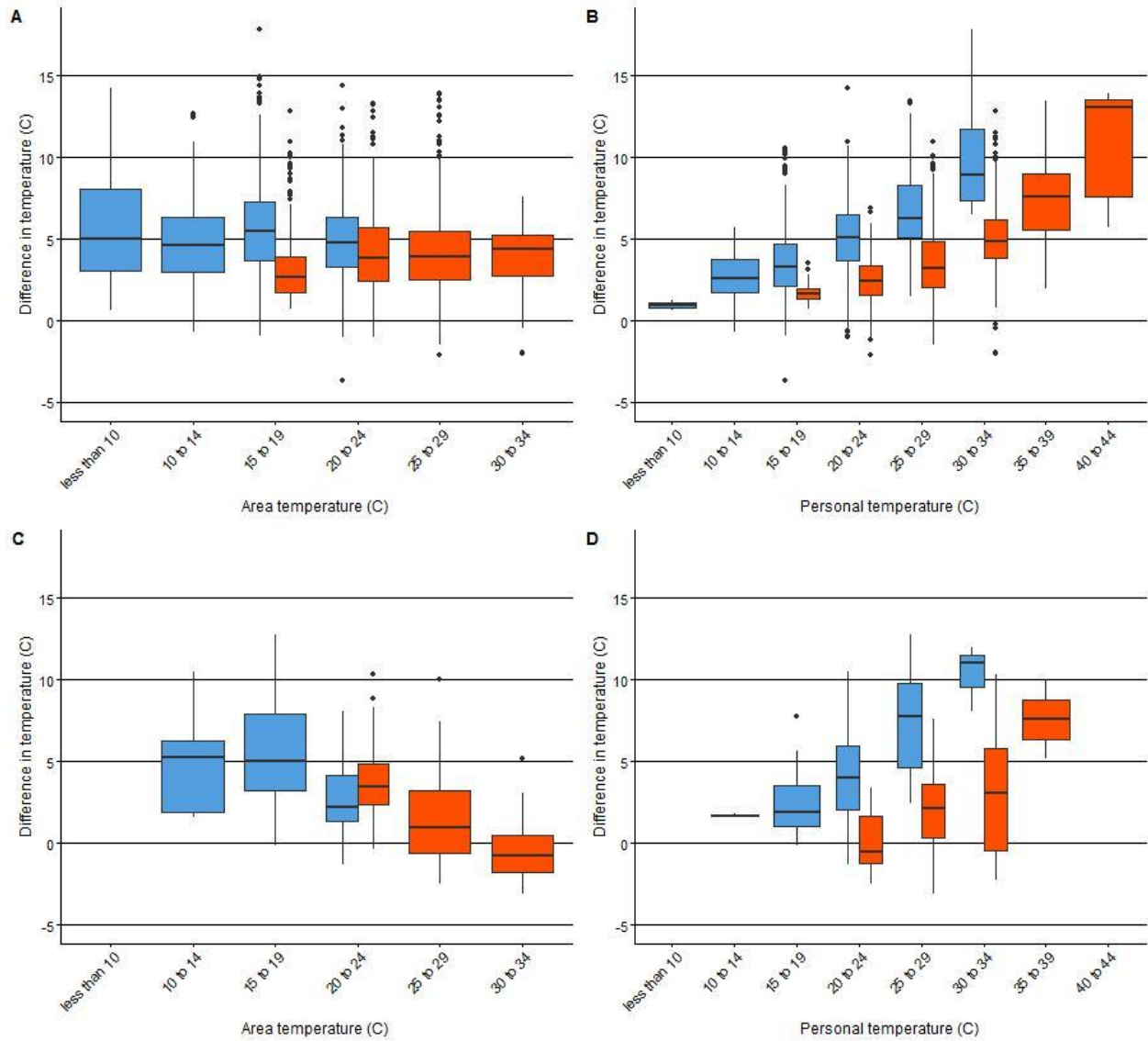
Figure 3.1: Difference in PL-AL T_a by exposure categories stratified by hot (red bars) and cool (blue bars) days. (A) Work periods by AL T_a . (B) Work periods by PL T_a . (C) Break periods by AL T_a . (D) Break periods by PL T_a .
