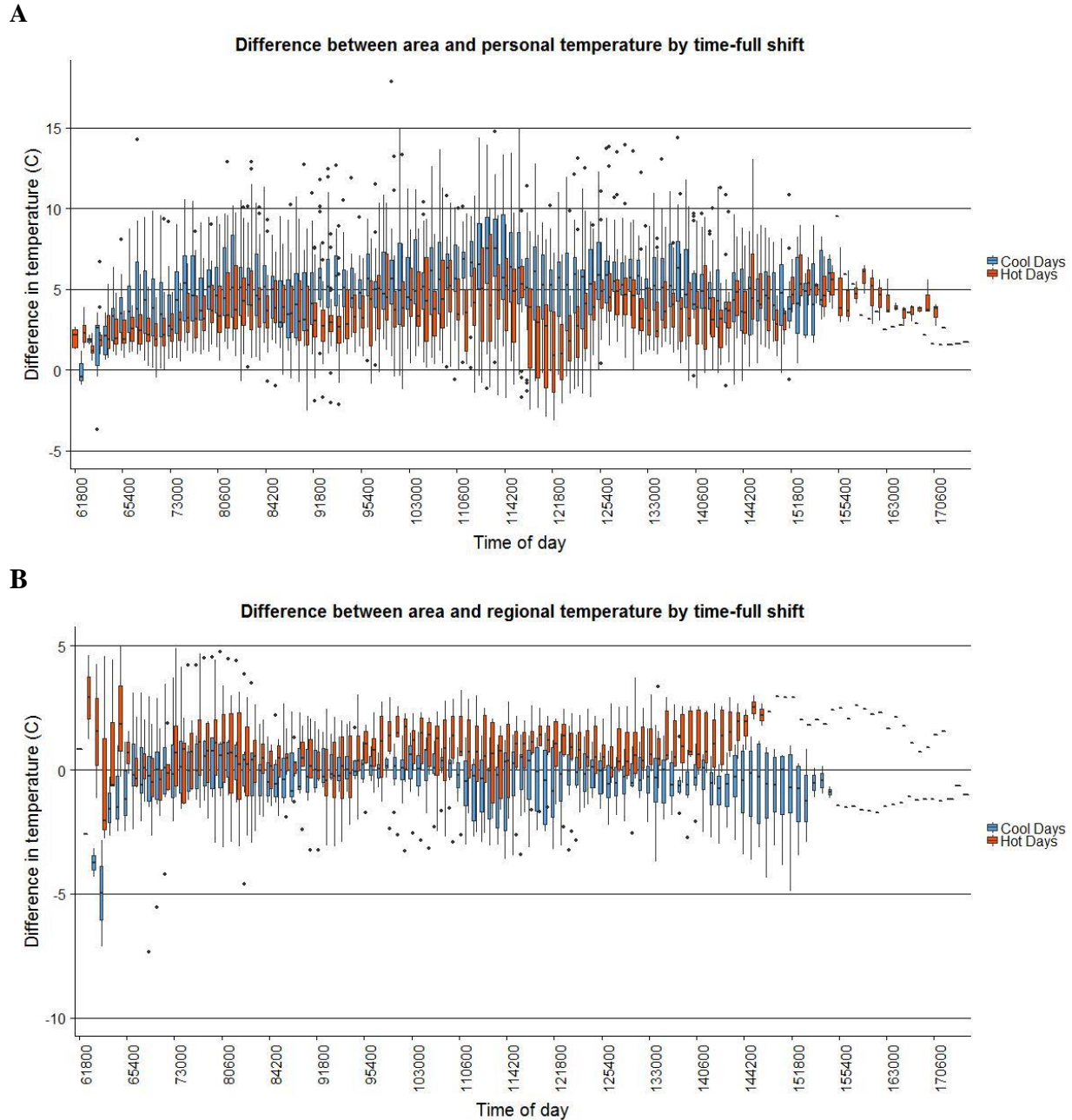
Figure 3.3: Difference in PL-AL and RL-AL T_a by time stratified by hot (red bars) and cool (blue bars) days. ( Top ) PL-AL by time of day. ( Bottom ) RL-AL by time of day. Median lunch break start and end times were 11:55 and 12:30.
