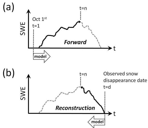
Figure 2.1 Conceptual schematic of SWE simulations from (a) forward and (b) reconstruction configurations of the same snow accumulation and melt model. SWE in (a) is simulated forwards in time from October 1 st , while SWE in (b) is simulated backwards in time from the observed snow disappearance date. In this example, peak SWE occurs at t=n .
