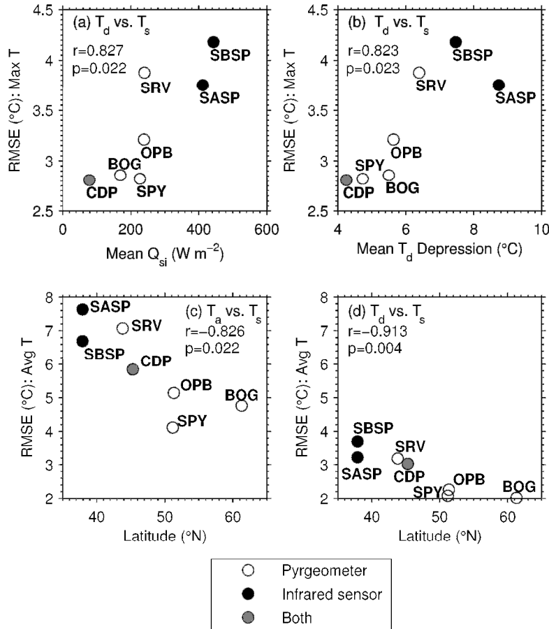
Figure 4.5 RMSE in simulating daily statistics of T_s vs. site characteristics. Shown are RMSE values when simulating maximum daily T_s with maximum daily T_d vs. (a) mean incoming shortwave radiation and (b) mean dew point depression (i.e., T_a - T_d ). Also shown are RMSE values plotted against latitude when simulating average daily T_s with (c) average daily T_a and (d) average daily T_d . Symbols represent the type of sensor used to measure T_s . Only periods with snow depth exceeding 10 cm are included in these statistics.
