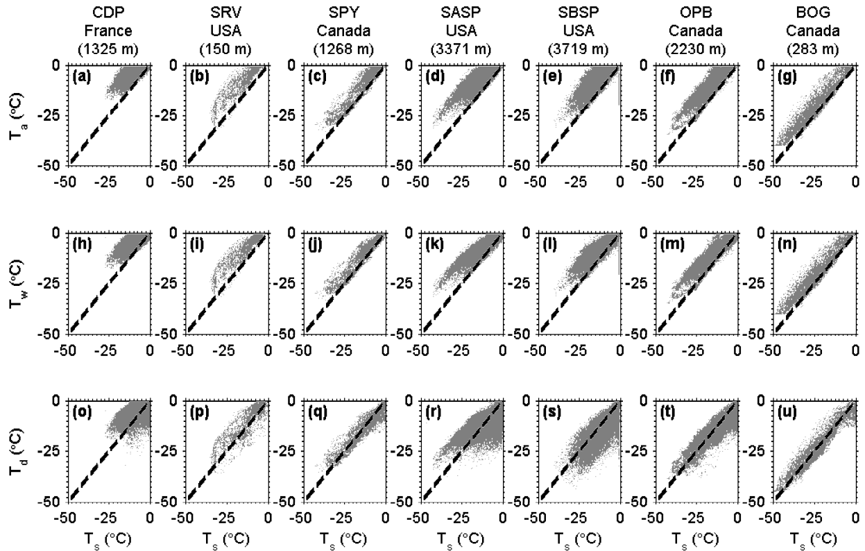
Figure 4.2 Comparisons between observed sub-daily snow surface temperature ( T_s ) and standard height (a-g) air temperature, (h-n) wet-bulb temperature, and (o-u) dew point temperature at the seven study sites. The sites are organized from warmest (left) mean DJF temperatures to coldest (right). Comparisons are only shown during periods when snow depth exceeded 10 cm.
