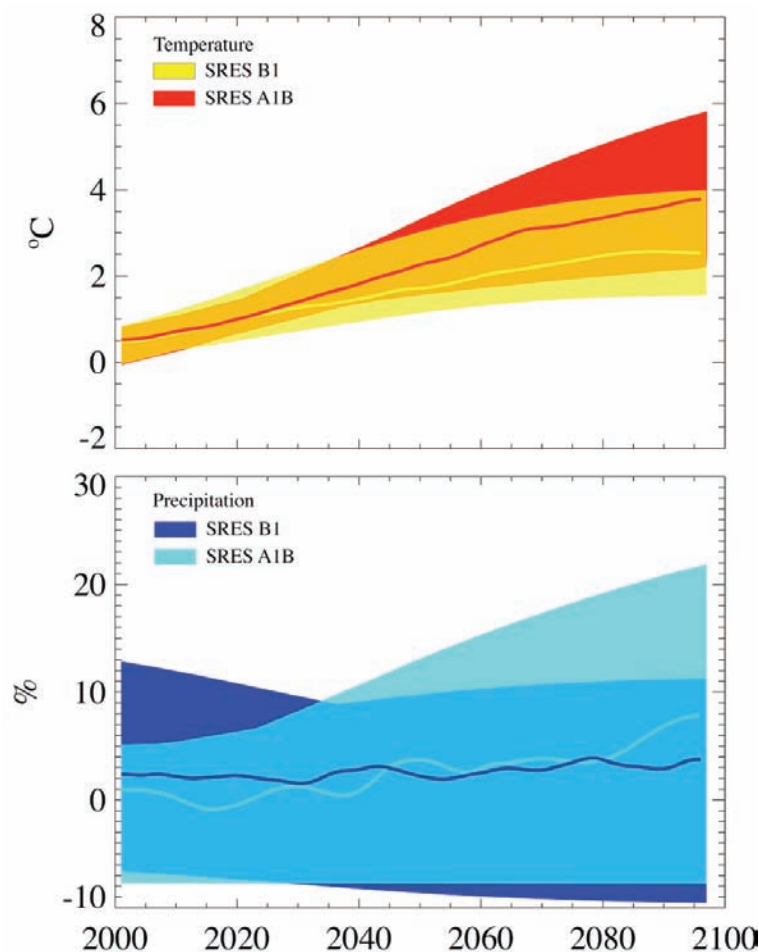
Figure 5.2. Changes in Pacific Northwest annual temperature (top) and precipitation (bottom) for IPCC global emissions scenarios B1 and A1B.
