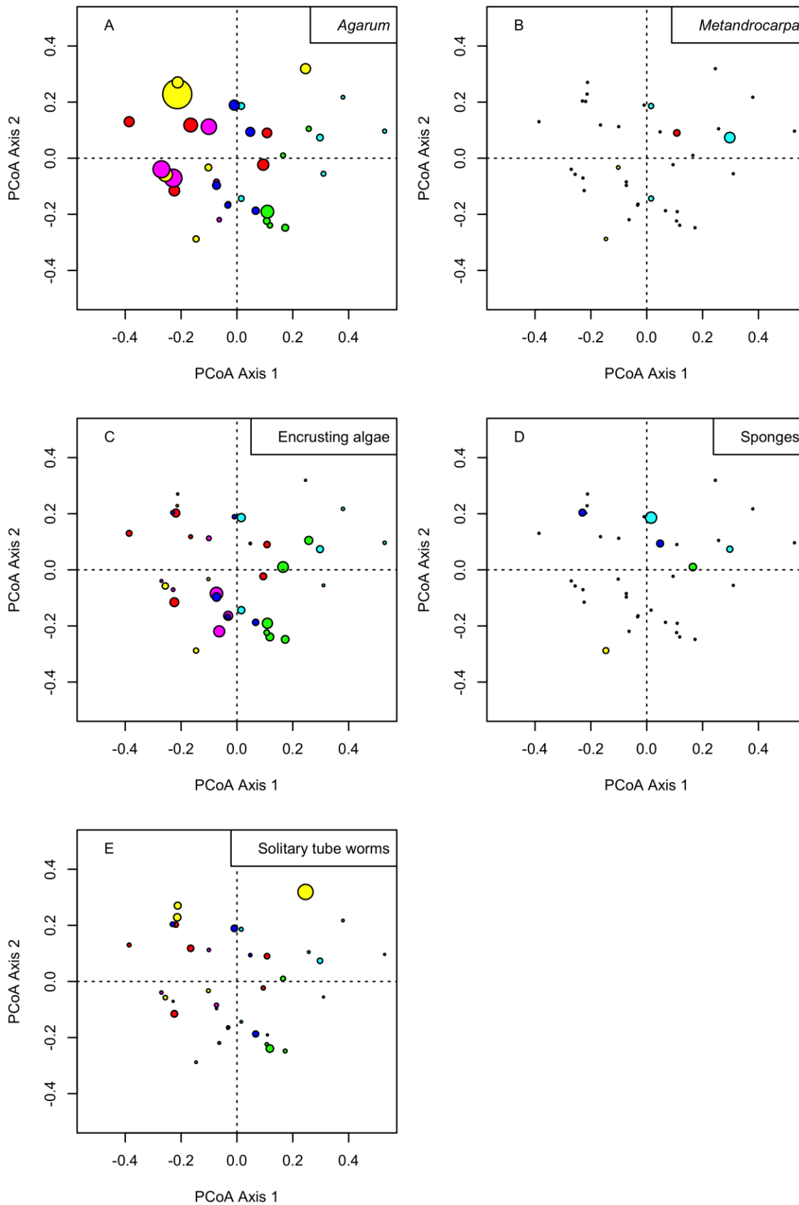
Figure 10. PCoA of the shallow mobile invertebrate assemblage, with overlays of sessile epibenthos cover. BIO-BIO analysis indicates that Agarum fimbriatum (A), Metandrocarpa taylori (B), non-coraline encrusting algae (C), sponges (D), and solitary tube worms (E), of the sessile epibenthos, together best predict the shallow mobile invertebrate assemblage. Point diameter is proportional to sessile epibenthic species cover. Point colors as in Fig. 2.
