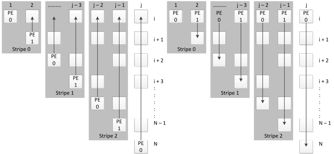
Figure 3.18 Striping for Normal (left) and Bifurcation (right) states
