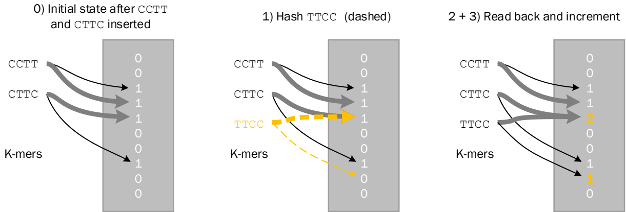
Figure 4.2 Counting Bloom filter insert operation for a 2-hash filter, where the thin line represents the first hash and the thick line the second
