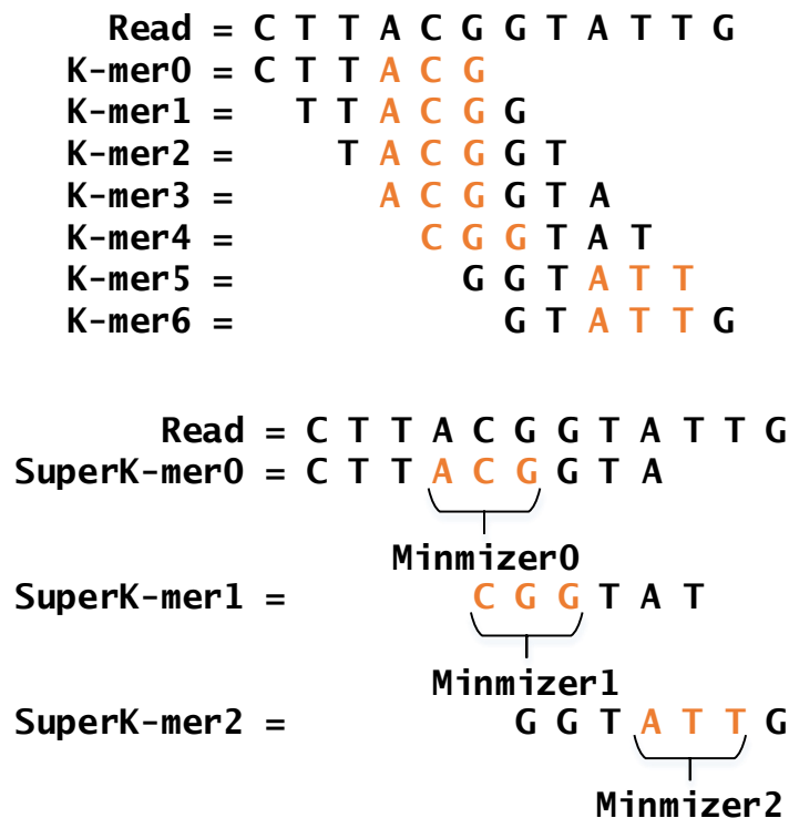
Figure 4.1 K-mers for a 12 bp read (top) and Super K-mers for the read (bottom), with minimizers shown in orange
