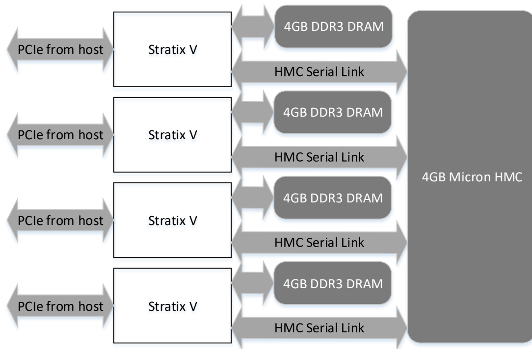
Figure 1.3 Micron SB-801 block diagram
