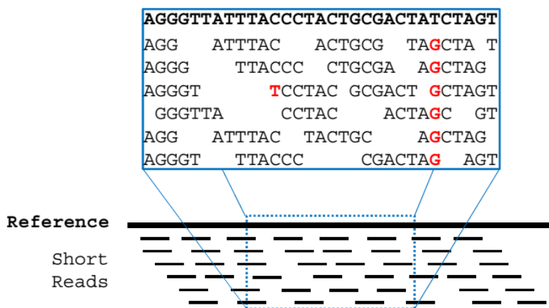
Figure 1.5 Short reads aligned to a reference genome
