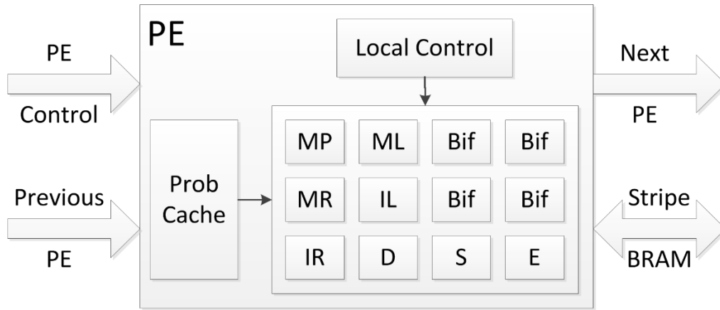
Figure 3.19 CM CYK PE block diagram
