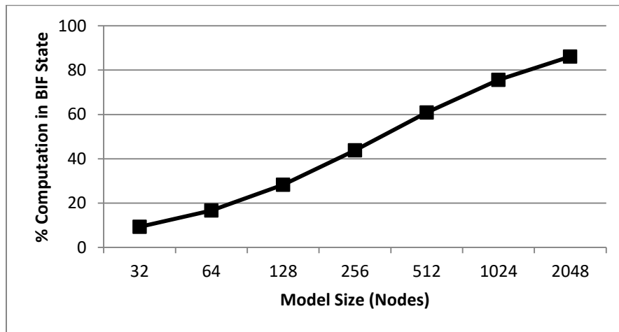
Figure 3.12 Computation in BIF state assuming 0.9% BIFs
