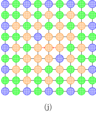
Figure 5.6: A controlled operation on a 9 \times 9 grid (continued).
