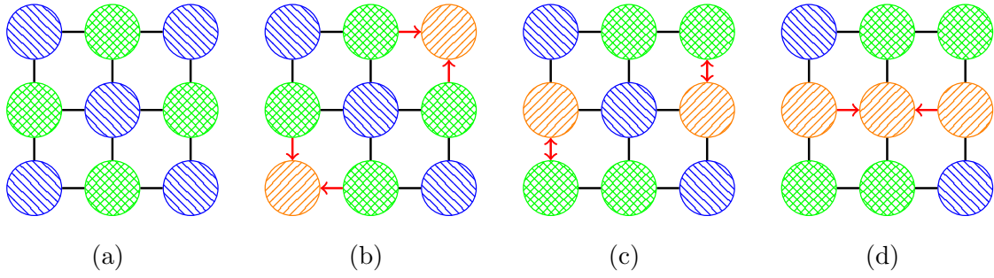
Figure 5.3: A controlled operation on a 3 \times 3 grid. The qubits crosshatched green are the data qubits, the qubits shaded with diagonal upward orange lines are ancilla qubits which store intermediate data and the qubits shaded with diagonal downward blue lines are ancilla qubits which are currently unused.
