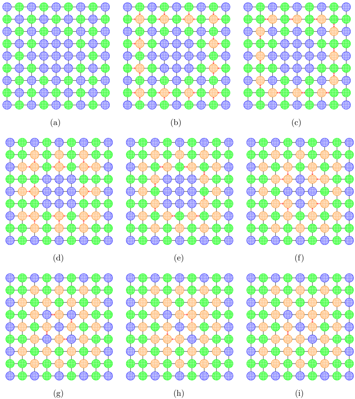
Figure 5.6: A controlled operation on a 9 \times 9 grid. See Figure 5.3 for the meaning of the colors and shadings used.
