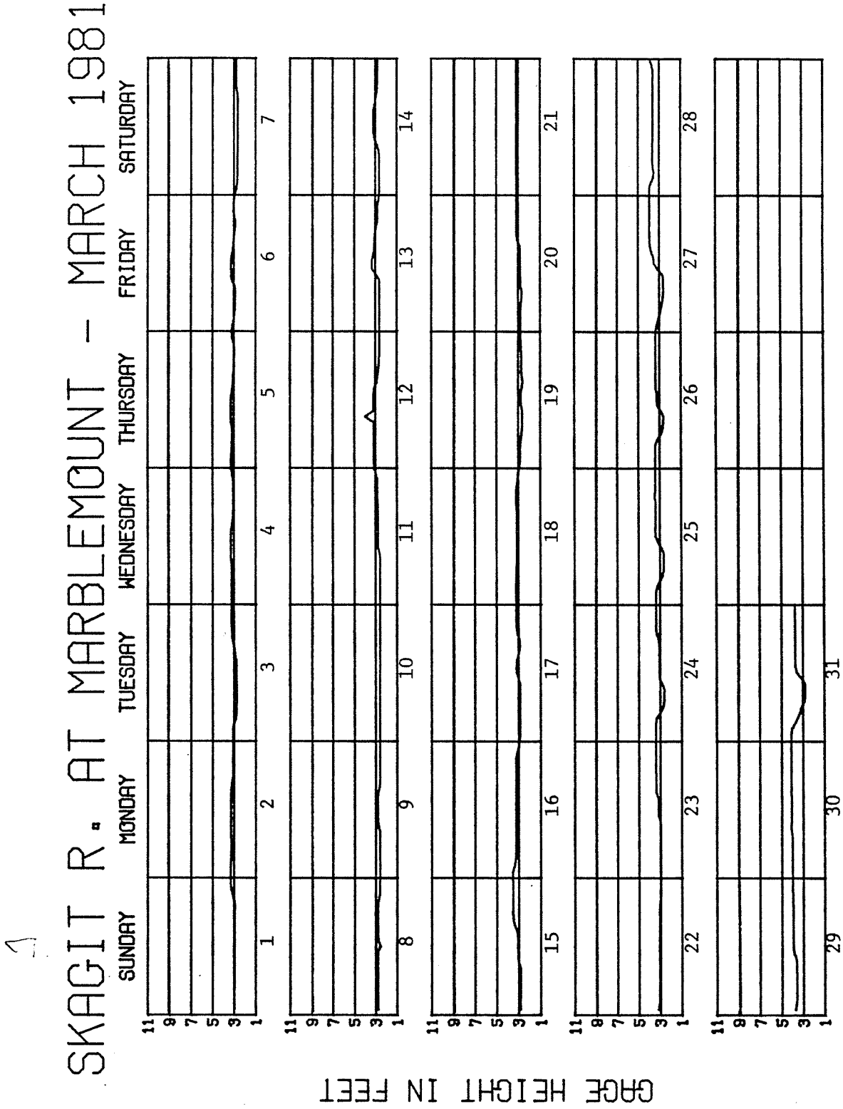
Appendix I, Figure 4. Hourly gage height data for Skagit River at Marblemount (USGS) January - December 1981. (Continued).
