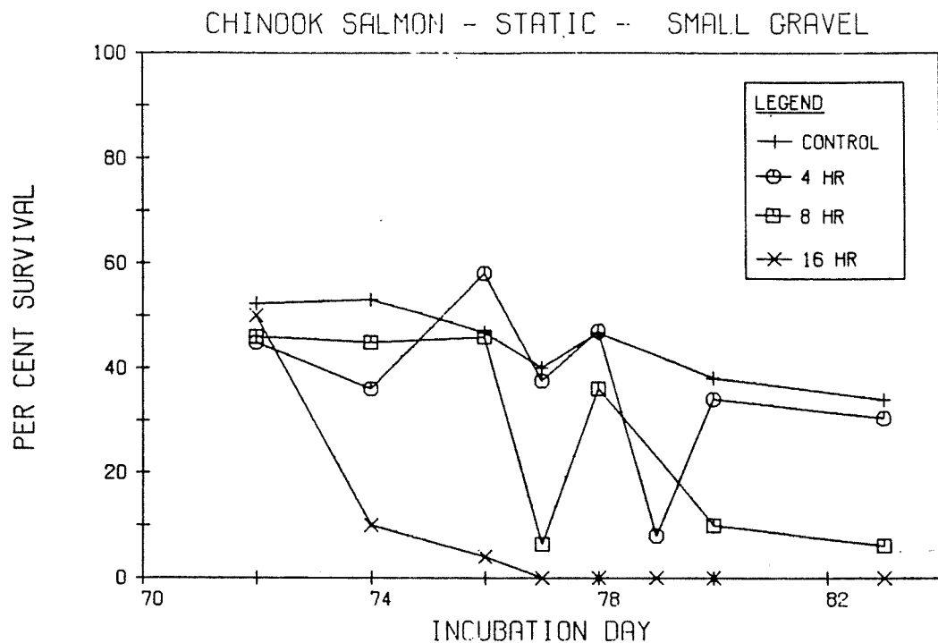
Fig. 29. Percent survival of chinook salmon embryos in static water for 4, 8 and 16 hrs/day in small gravel from eyed through hatching.
