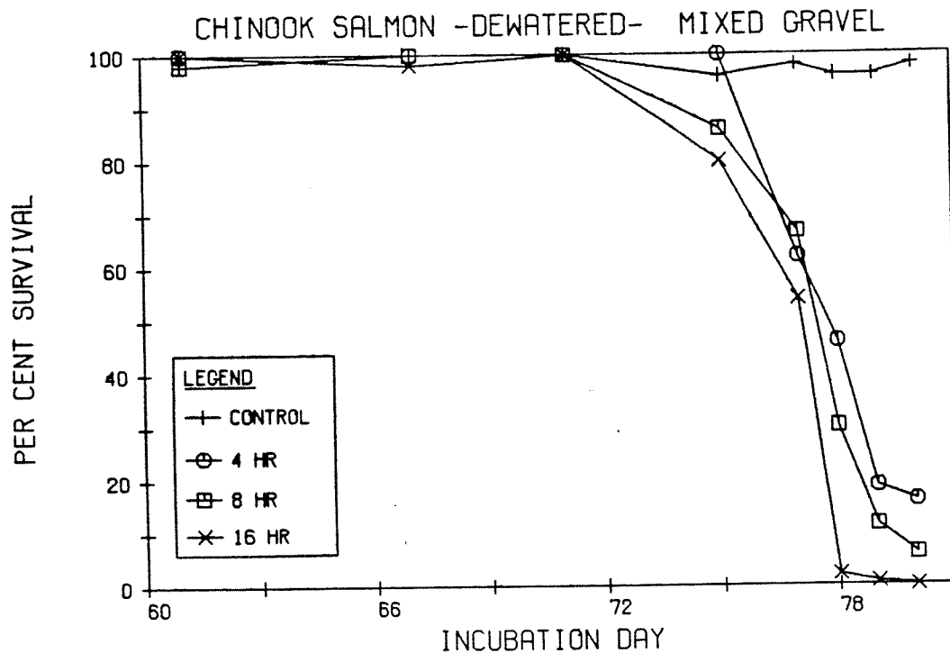
Fig. 19. Percent survival of chinook salmon embryos dewatered for 4, 8 and 16 hrs/day in mixed gravel from eyed through hatching.
