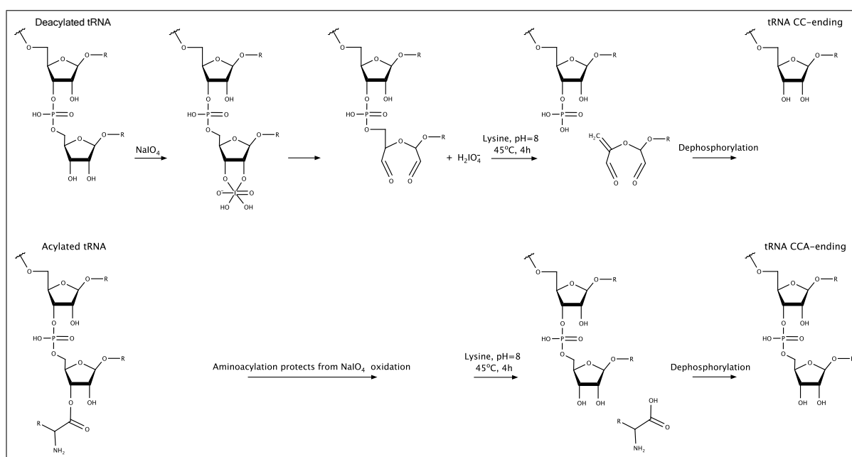
Figure D.1: Schematic of the Whitfeld reaction with acylated and deacylated tRNA leading to generation of CCA and CC-ending tRNAs. For deacylated tRNA, 3' adenosine is oxidized by periodate and then cleaved off by lysine induced \beta -elimination [122, 151]. Acylated tRNA is protected from periodate oxidation but will be deacylated in the subsequent incubation with lysine.
