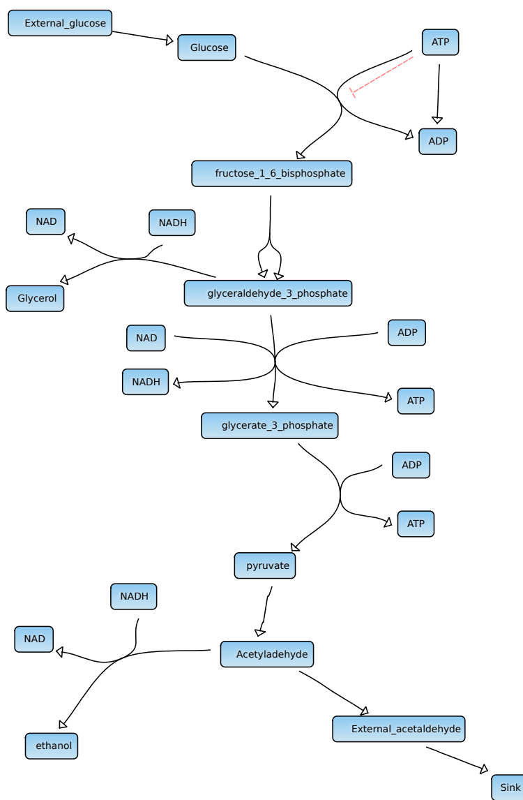
Figure 1.1: A canonical example of a metabolic pathway in the form of a condensed version of glycolysis (the conversion of fructose 1,6-bisphosphate to pyruvate is a 6-enzyme process — not all steps are shown). Glycolysis consumes six-carbon sugars and produces energy in the form of ATP and the reducing agent NADH. The diagram shown here depicts negative regulation (in red) of the fructose 1,6-bisphosphate committal step via ATP. Thus, an excess of ATP will tend to reduce glycolytic flux. Glycolysis is also negatively regulated by the downstream metabolite phosphoenolpyruvate (not shown) and possibly positively regulated by citrate. This diagram was generated from an SBML model [136], which also considers fermentation (hence the presence of reactions downstream from pyruvate in the diagram).
