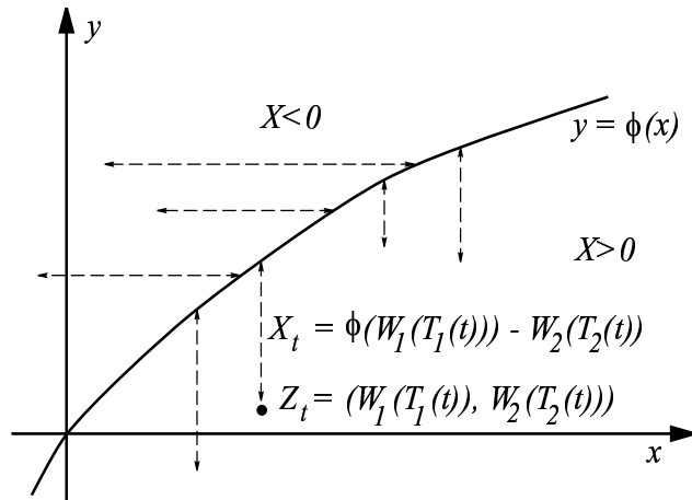
Figure 1: The process Z moves horizontally(vertically) above(below) the curve y = \phi(x) .
