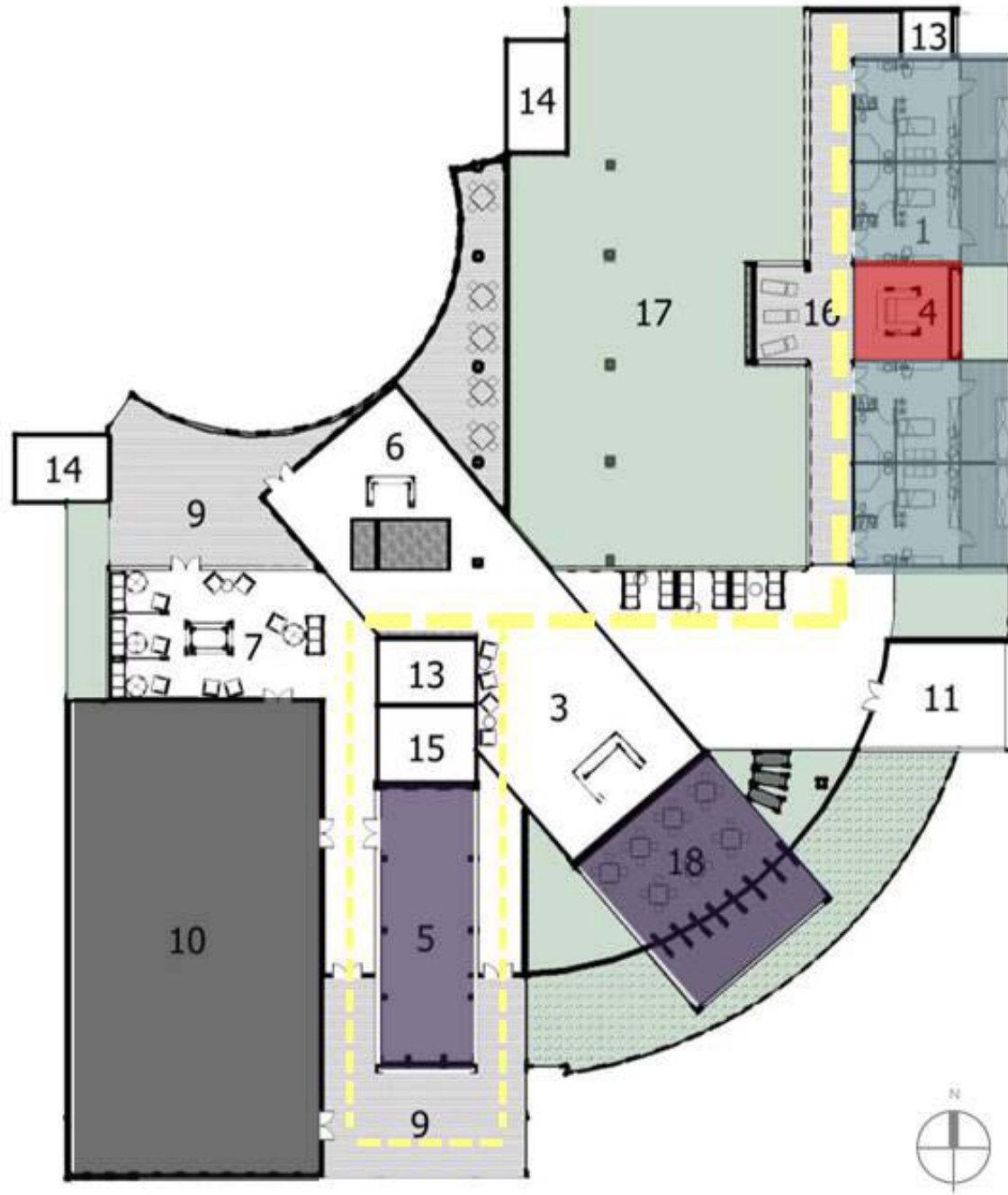
Figure 52: 7 Floor Plan
