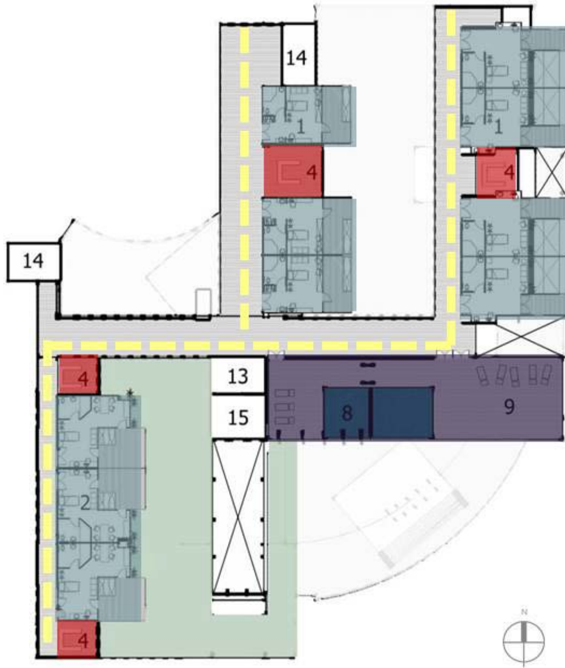
Figure 53: 8 Floor Plan
