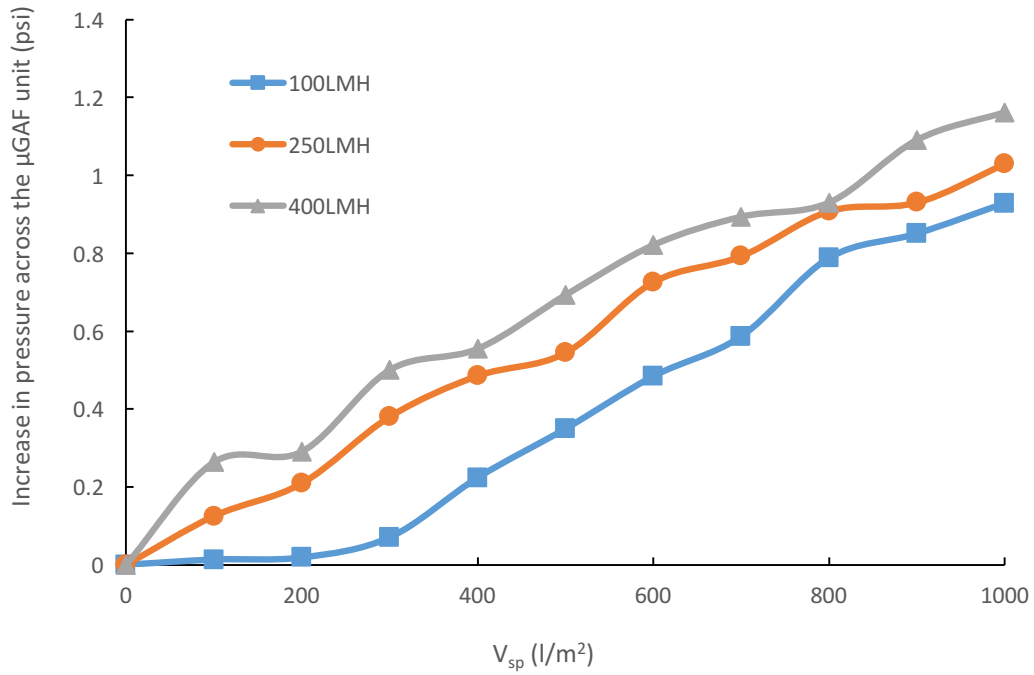
Figure 4-42 Pressure increase profiles of SA SUPER-μGAF units at different fluxes.
