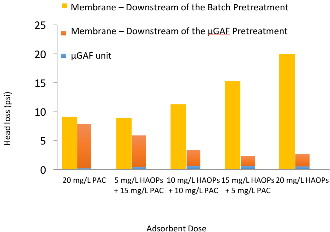
Figure 4-15 Final head loss at the end of the filtration V_{sp} of 2000 l/m 2 for batch pretreatment-membrane filtration tests and their corresponding \mu GAF pretreatment-membrane filtration experiments.
