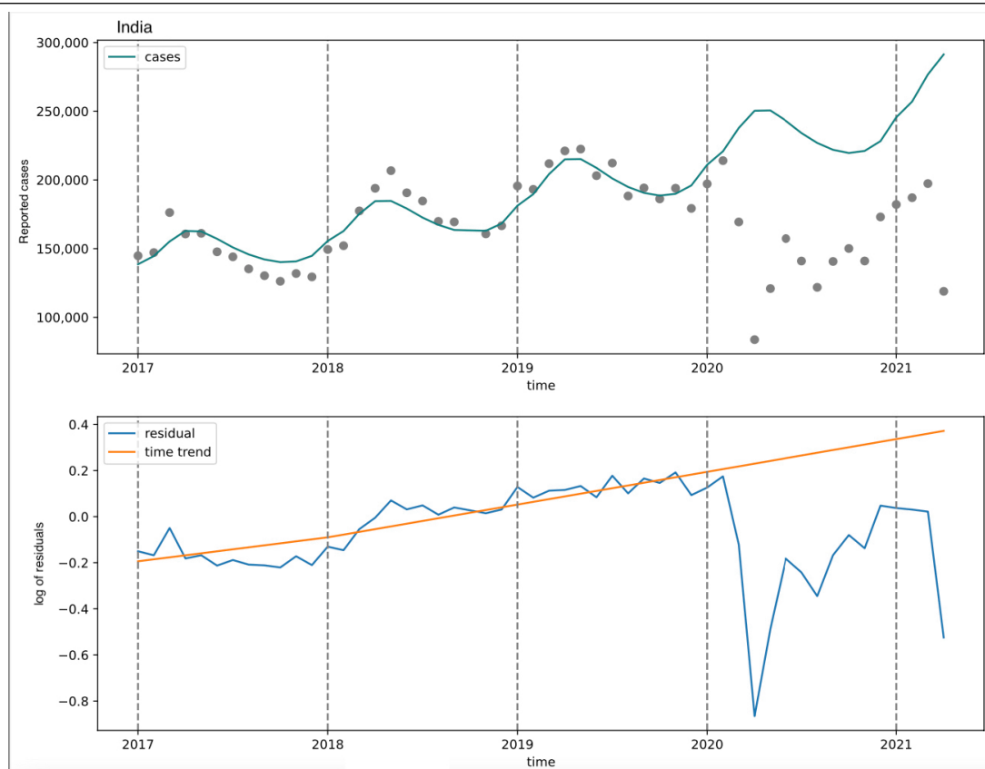
Figure 1: Top panel - Case notification in India from January 2017 to April 2021. Grey points represent case notification by month. The teal line represents a model fit to case notification seasonal and year trends from January 2017 to February 2020, prior to pandemic lockdown measures in March of 2020. This trends was then extended from March 2020 to April 2021 as the counterfactual expected cases in the absence of the pandemic (March 2020 to April 2021). Bottom panel - time trend of expected cases (orange line) fit to residuals (blue line) in India, January 2017 to April 2021.
