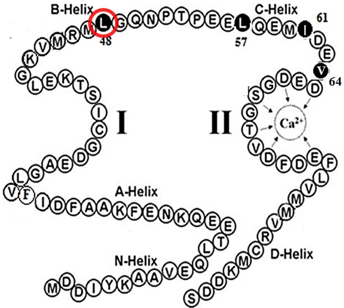
Figure 1.2: Amino acid sequence in the regulatory domain of cTnC including \text{Ca}^{2+} binding site I (defunct) and site II. The circled residue shows the location of the point mutation of leucine (L) to glutamine (Q) at position 48 in L48Q cTnC. Modified from [44].
