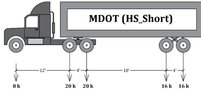
Figure 3.7 Kentucky (Type 4) (GVW = 80,000 lb.)
