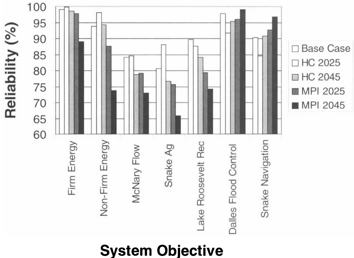
Figure 7. Effects to the Reliability of Columbia River Water Resources Objectives Simulated by the ColSim Model for the Climate Change Simulations Compared to the Base Case.
