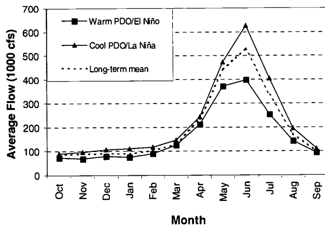
Figure 3. ENSO and PDO Composite Hydrographs for the Columbia River Basin. Composite hydrographs for 1900-1998 Columbia River naturalized streamflows at The Dalles, Oregon, during alternative phases of (a) ENSO, (b) the PDO, and (c) during warm PDO/El Niño and cool PDO/La Niña years. Dashed lines represent the long-term mean. ENSO years and PDO epochs are as defined in the text. Naturalized flow represents “virgin” streamflow, in which estimated human impacts on the river have been removed (see text).
