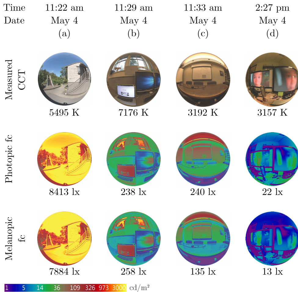
Figure 5.2. Variation of photopic and melanopic illuminance depending on architectural context HDR photos taken on May 4 th .
