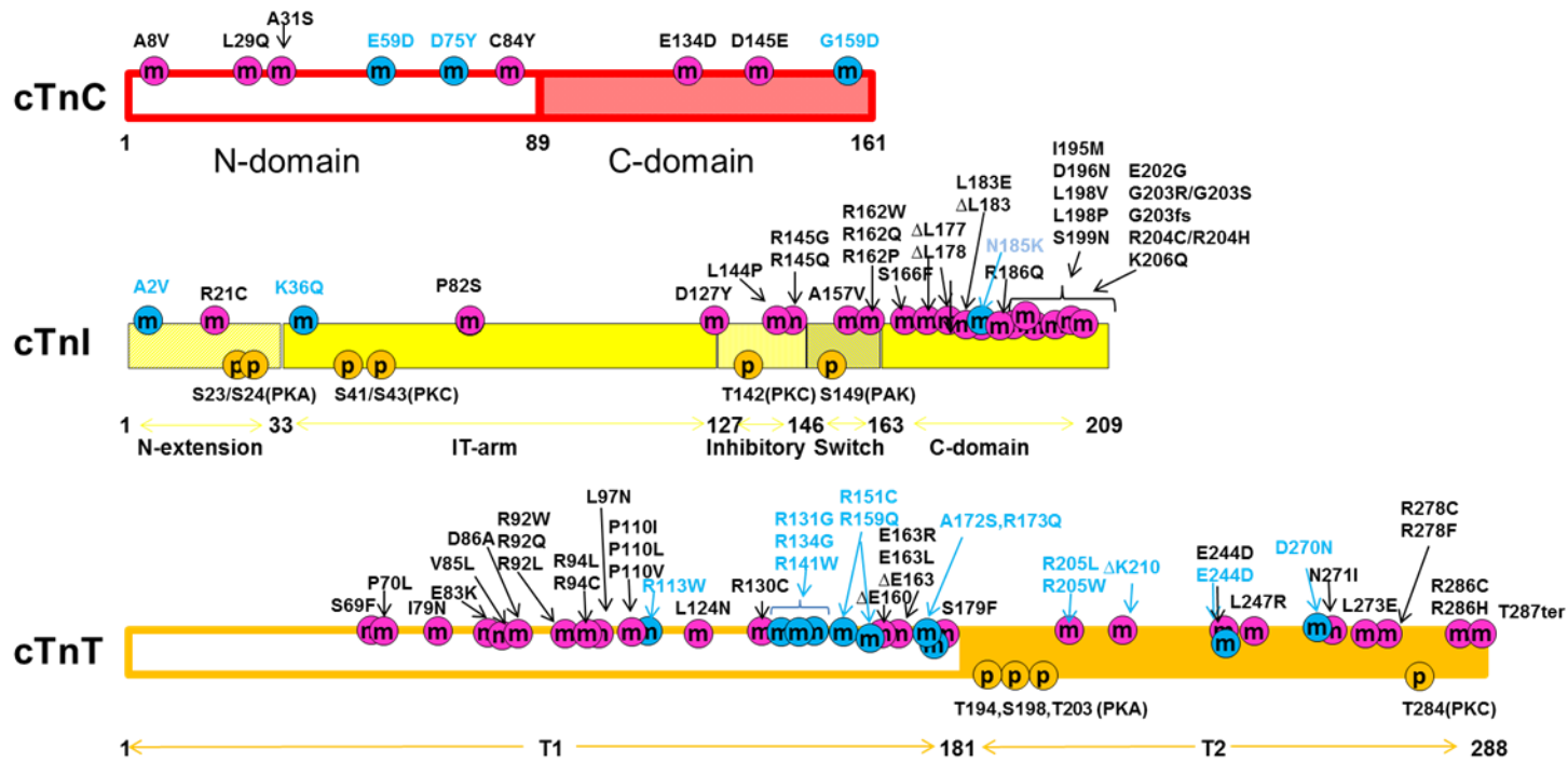
Figure 1.5. HCM and DCM related mutations and phosphorylation sites as identified on the primary sequences of human cTnC, cTnI, and cTnT: HCM associated mutations shown in pink, DCM shown in blue, phosphorylation sites labeled in gold.
