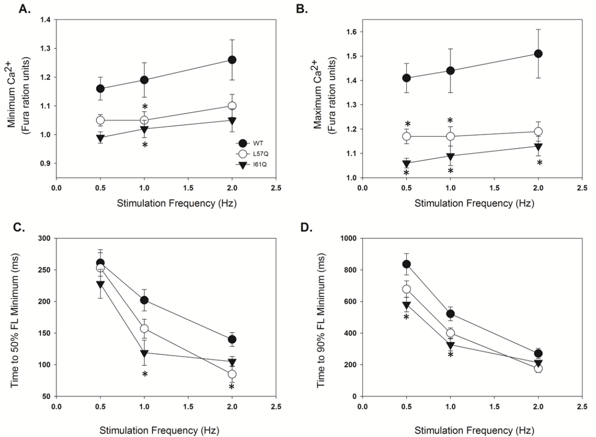
Figure 6.4. Effect of stimulation frequency on Ca^{2+} handling properties. L57Q transduced myocytes (open circles) and I61Q transduced myocytes (closed triangles) respond similarly to stimulation frequency as WT transduced myocytes (closed circles) in minimal (A) and maximal (B) fura fluorescence, while WT transduced myocytes showed higher level of fura fluorescence than I61Q and L57Q transduced myocytes at all frequencies (0.5, 1, 2 Hz). As with cardiomyocytes relaxation, Ca^{2+} transient decay time (DT) to 50% (C) and 90% (D) is shortened with increased stimulation frequency for all groups. * = p < 0.05 as compared to WT transduced.
