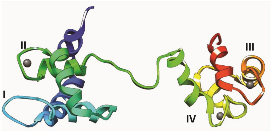
Figure 1.3. NMR structure of Ca 2+ saturated cTnC ( PDB:1LA0(10)): Ca 2+ shown as gray spheres, figure generated by Chimera(96).
