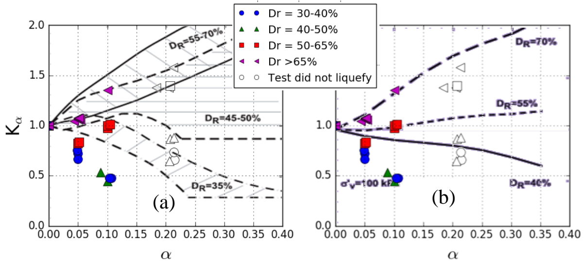
Figure 54: CSS tests of \sigma'_{v0} = 100 kPa from Figure 49 are then overlaid with (a) K_\alpha form of Seed and Harder 1990, and (b) Boulanger 2003. The point of liquefaction triggering is taken as r_u = 1.0 (for cases which did not fail in liquefaction, failure considered to point at which r_u reaches peak threshold)
