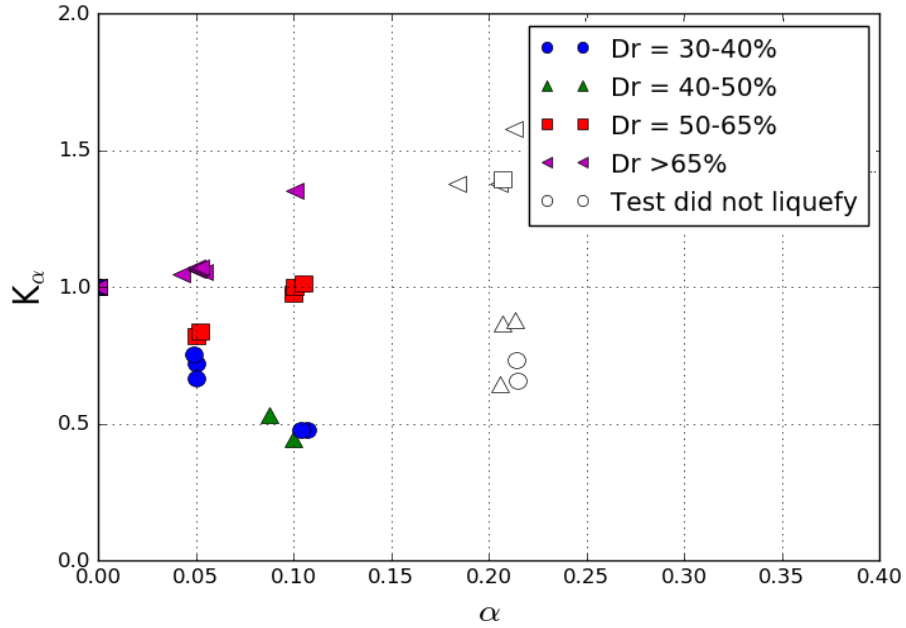
Figure 53: K_\alpha on Siri sands in \sigma_{v0} = 100 kPa. The point of liquefaction triggering is taken as r_u = 1.0 (for cases which did not fail in liquefaction, failure considered to point at which r_u reaches peak threshold)
