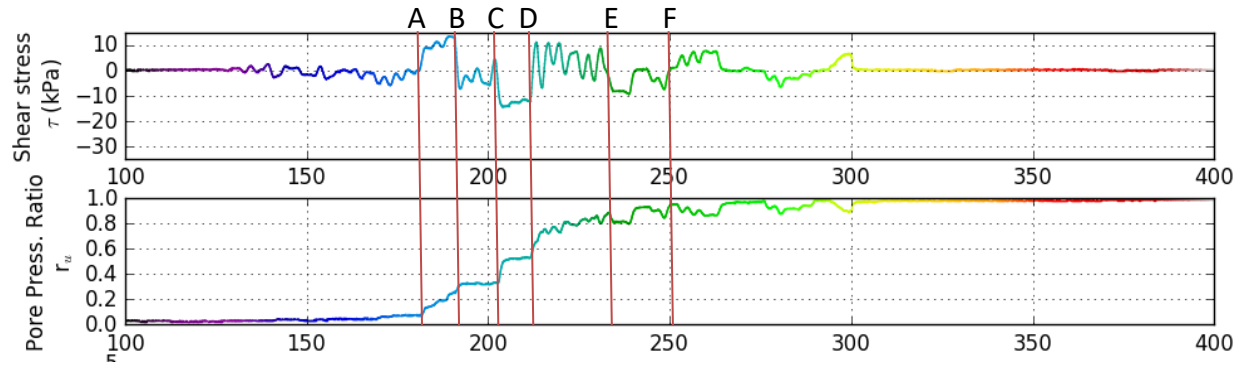
Figure 49: Typical pore pressure response in a test without initial shear stresses. Test N0407, Palm Spring motion on Nevada sand, D_r = 65\% , CSR = 0.15 , \alpha = 0 , \sigma_{vo} = 100 kPa.
