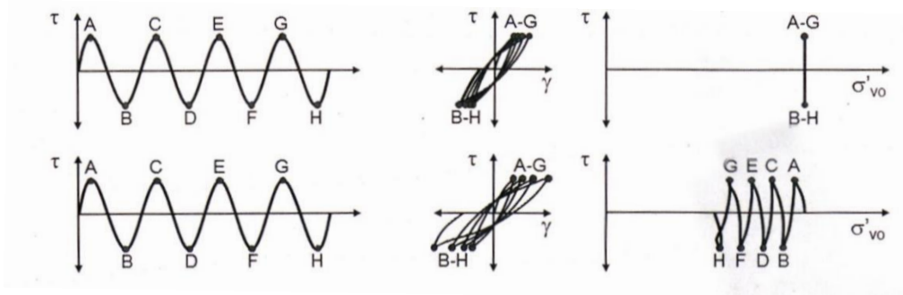
Figure 6: Cyclic degradation of a (top) unsaturated, and (bottom) saturated sand sample. Accumulation of strain \gamma with each successive cycle as stiffness incrementally decreases. In saturated samples, pore pressure increases and effective stress incrementally decreases, causing stiffness to degenerate at a higher rate and strains to accumulate faster (figure from Kramer 1996)
