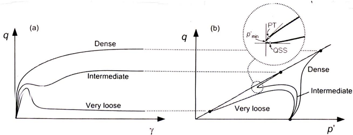
Figure 5: Illustration of effect of state on shear strength and volumetric change behavior in an unsaturated sample as shown on a stress vs. strain graph (or q - \gamma ) (left) and a shear stress vs. normal effective stress graph (or q - p' ) (right). Typical behavior of loose, intermediate, and dense soils are loaded until failure is reached. Intermediate soils often display a phase transformation (PT) which marks the change from contractive to dilative behavior (from correspondence with S. Kramer).
