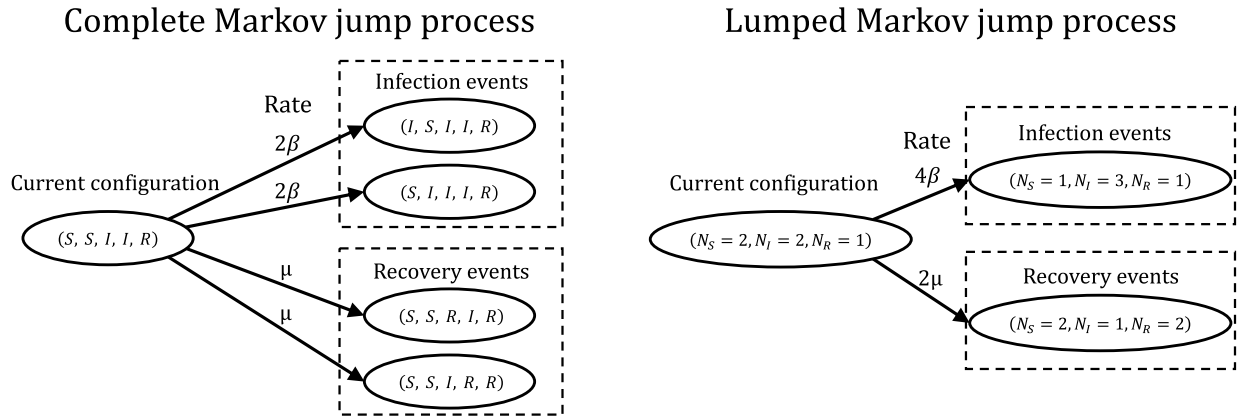
Figure 2.3: Complete and lumped representations of SIR dynamics in a population of five individuals. The per-contact infectivity rate, \beta , and the recovery rate, \mu , parameterize exponential waiting time distributions between transition events. The complete Markov jump process evolves on the state space of subject state labels, \mathcal{S} = \{S, I, R\}^N , with dynamics determined by the subject-level transition rates. Each susceptible may contact two infected individuals, while each infected individual recovers independently. The lumped process evolves on the state space of compartment counts, \bar{\mathcal{S}} = \{N_S, N_I, N_R : N_S + N_I + N_R = N\} , with dynamics determined by lumped transition rates. The waiting time distributions between transitions are derived by noting that if \tau_1 \sim \exp(\lambda_1) and \tau_2 \sim \exp(\lambda_2) , then \tau_{\min} = \min(\tau_1, \tau_2) \sim \exp(\lambda_1 + \lambda_2) .
