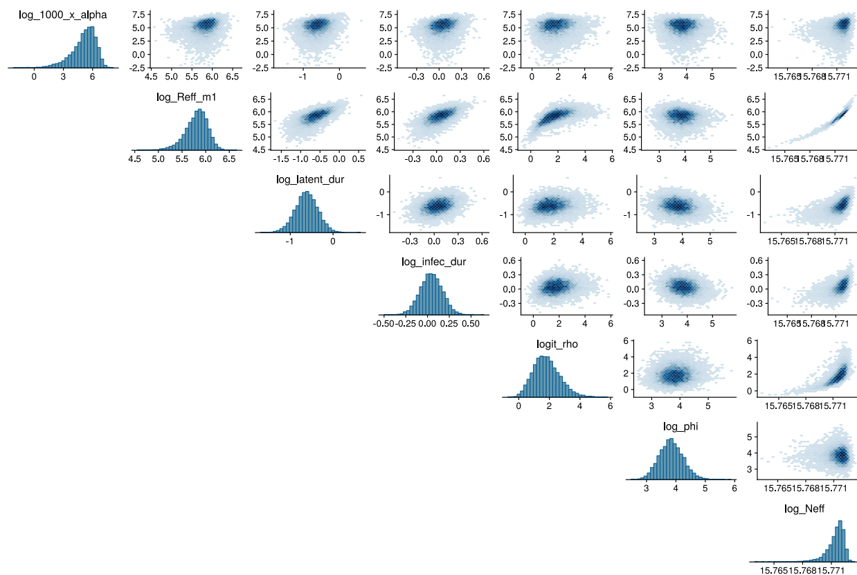
Figure B.3: Marginal histograms and pairwise scatterplots of posterior samples for parameters for the SEIR model fit to the Sierra Leone Ebola dataset using the estimation scale in Table B.3. The parameters on the estimation scales in this figure and their interpretations are provided in Table B.2.
