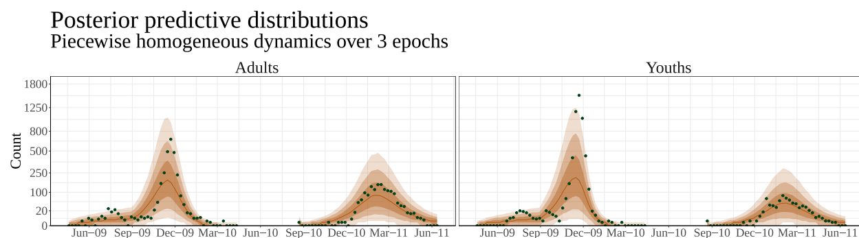
Figure 5.9: Posterior predictive distributions of a stratified SIRS ODE model with piecewise homogeneous dynamics over three epochs for A(H1N1)pdm09 in Finland.
