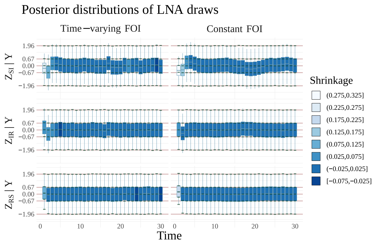
Figure C.5: Posterior distributions of the LNA draws for infection, recovery, and loss of immunity in SIRS models with time-varying and constant force of infection (blue boxplots). The lower and upper whisker tips correspond to the 2.5 th and 97.5 th posterior quantiles, the lower and upper hinges to the 25 th and 75 th quantiles, and the middle hash mark to the posterior median. The solid red lines are the theoretical quantiles of the posterior predictive distribution (or equivalently, the prior distribution) of the LNA draws, drawn at the quantiles of a standard normal distribution corresponding to the boxplot quantiles. The green ticks are the estimated quantiles of the posterior predictive distributions of the LNA draws, accounting for boundary conditions on the state space of the latent process and obtained by simulating LNA paths from the posterior predictive distribution. The posterior distributions of LNA draws are shaded according to the level of posterior shrinkage, computed as one minus the ratio of standard deviations of LNA draws in the posterior and prior.
