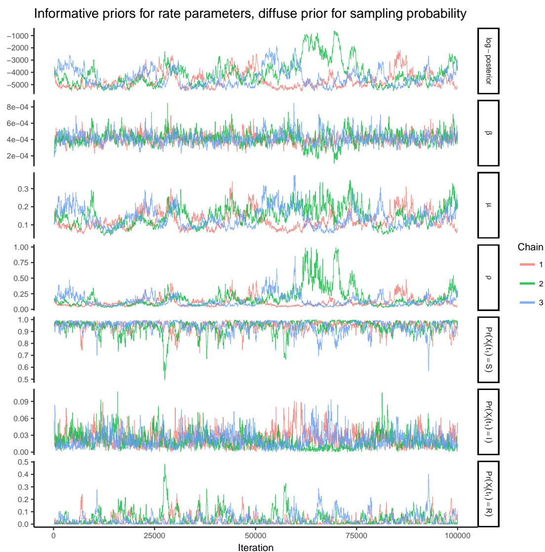
Figure A.18: Traceplots of the log-posterior and model parameters for the SIR model fit under informative priors for the rate parameters and a diffuse prior for the binomial sampling probability. \beta denotes the per-contact infectivity rate, \mu is the recovery rate, \rho is the binomial sampling probability. Traceplots are thinned to display every 50 th iteration.
