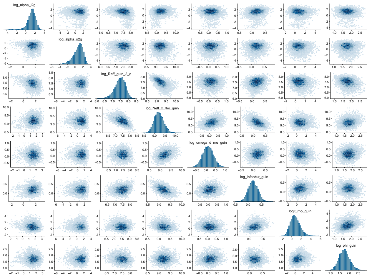
Figure B.28: Scatterplots of Guinea-specific parameters in a stratified SEIR LNA model fit to data from the West Africa Ebola outbreak.
