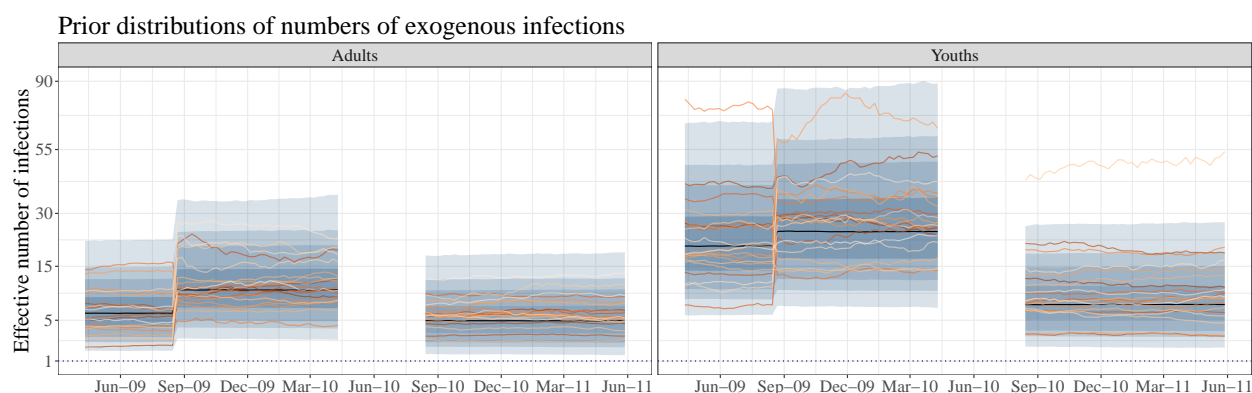
Figure C.7: Induced prior distribution of for the effective number of exogenous infections among youths and adults. Shaded bands correspond to the central 50%, 80%, and 95% prior probability intervals.
