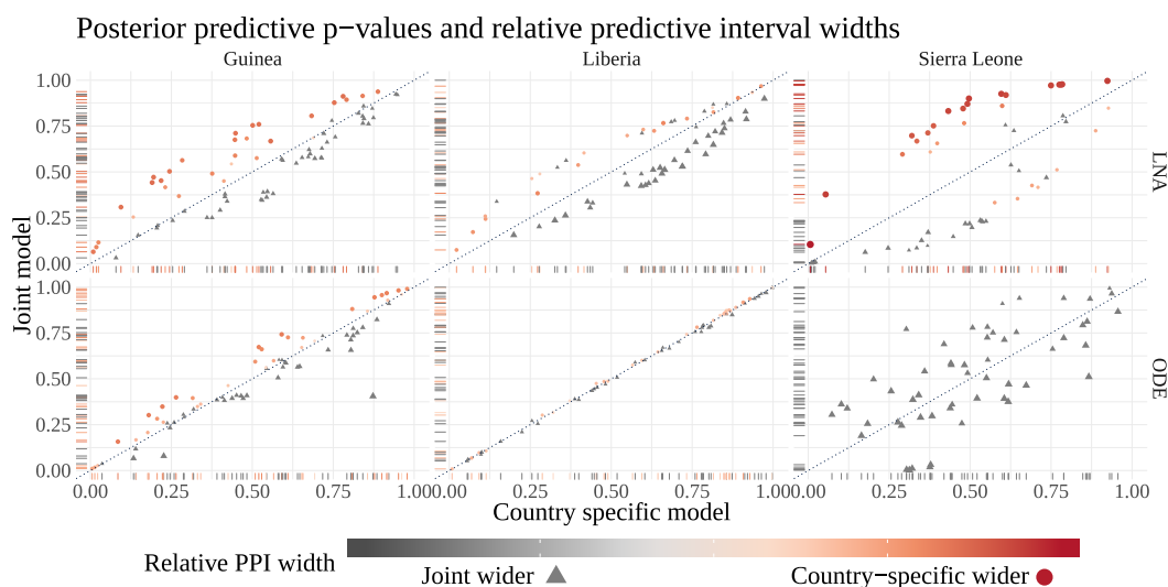
Figure 4.20: Comparison of country-specific and joint SEIR models for Ebola using posterior predictive p-values (PPPs) and relative posterior predictive interval (PPI) widths. The top row compares country-specific and joint models fit via the LNA, while the bottom row compares deterministic country-specific and joint models fit using ODE. Each point corresponds to the observed incidence in a given week. The X–Y coordinates give the PPPs of the data under the country-specific and joint models, respectively. The size and color of each point corresponds to the relative PPI width, computed as (\hat{\sigma}_{post,\ell}^{country-specific} - \hat{\sigma}_{post,\ell}^{joint}) / \hat{\sigma}_{post,\ell}^{joint} , and the sign of the relative width is further emphasized by the shape of the point. Dots indicate that PPIs for country-specific models are wider, while triangles corresponds to observations for which the PPI produced by the joint model was wider.
