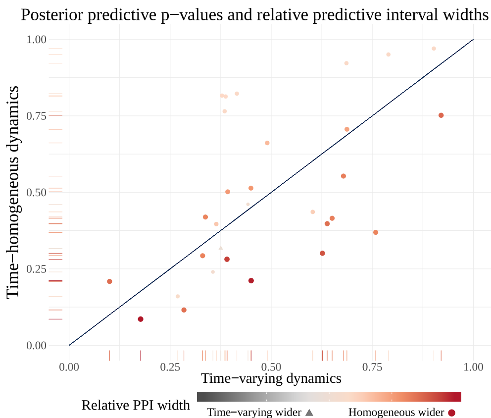
Figure 5.3: Comparison of models with time-varying and constant force of infection using posterior predictive p-values (PPPs) and relative posterior predictive interval (PPI) widths. Each point corresponds to the observed incidence in a given week. The X–Y coordinates give the PPPs under time-varying dynamics and time homogeneous dynamics, respectively. The size and color of each point corresponds to the relative PPI width, computed as (\hat{\sigma}_{post,\ell}^{constant} - \hat{\sigma}_{post,\ell}^{GMRF})/\hat{\sigma}_{post,\ell}^{GMRF} , and the sign of the relative width is further emphasized by the shape of the point. Dots indicate that PPIs with constant FOI are wider, the lone triangle corresponds to the one data point where the PPI for the model with time-varying FOI was wider.
