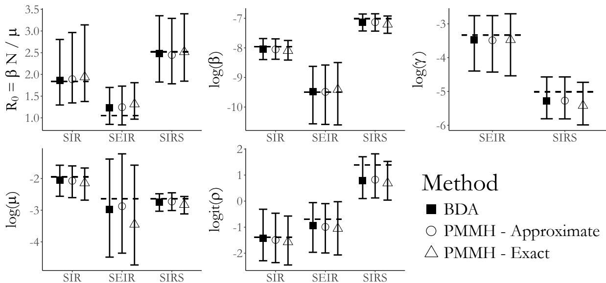
Figure 3.4: Posterior medians and 95% credible intervals of parameters in the SIR, SEIR, and SIRS models fit with Bayesian data augmentation (BDA) and particle marginal Metropolis–Hastings (PMMH) with particle paths simulated approximately (using \tau -leaping) and exactly (using Gillespie’s direct algorithm). Displayed are estimates of the basic reproductive number, R_0 , the rate parameters, and the binomial sampling probability. In all models, \beta is the per–contact infectivity rate, \mu is the recovery rate, and \rho is the binomial sampling probability. In the SEIR model, \gamma denotes the rate at which an exposed individual becomes infectious, while in the SIRS model \gamma denotes the rate at which immunity is lost.
