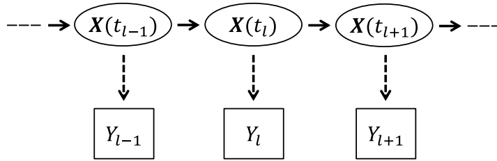
Figure 2.1: Diagram of a Hidden Markov model. The data, \mathbf{Y} , are conditionally independent given the latent epidemic process, \mathbf{X} .
