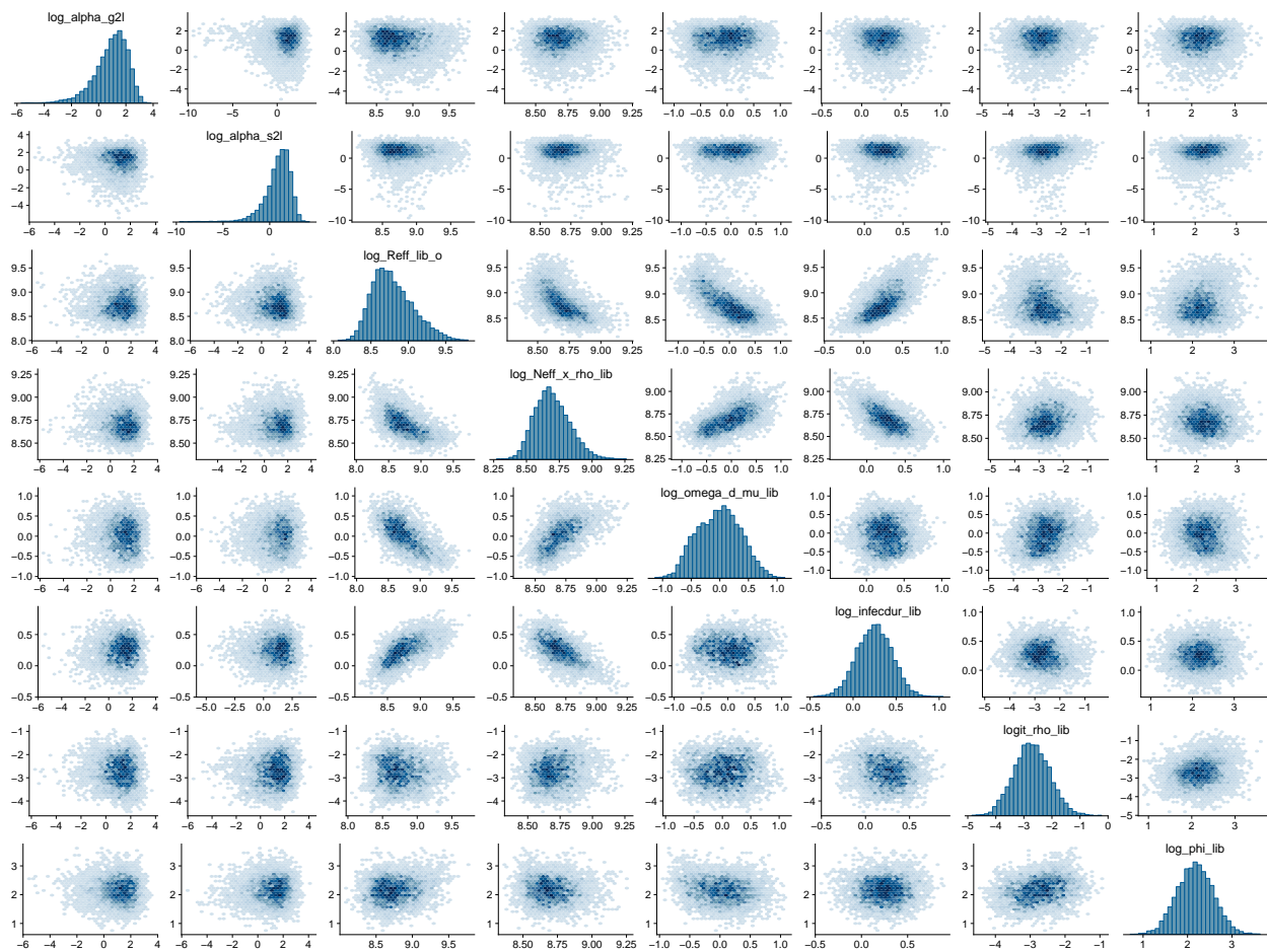
Figure B.29: Scatterplots of Liberia-specific parameters in a stratified SEIR LNA model fit to data from the West Africa Ebola outbreak.
