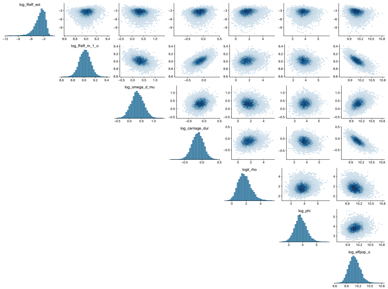
Figure B.16: Scatterplots of parameters for the SEIR LNA model fit to data from the Ebola outbreak in Sierra Leone.
