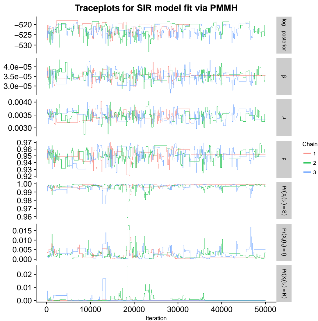
Figure A.13: Traceplots of the log-posterior and model parameters for the SIR model fit using PMMH with 2,500 particles, following a tuning run of 5,000 iterations used to estimate the covariance matrix for the RWMH. \beta denotes the per-contact infectivity rate, \mu is the recovery rate, \rho is the binomial sampling probability. Traceplots are thinned to display every 50 th iteration.
