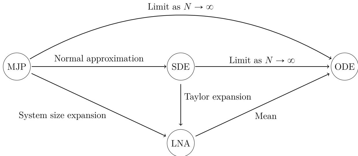
Figure 2.4: Relationship between various compartmental model representations. The Markov jump process (MJP) is typically the model of interest, and in large populations can be approximated by a system of stochastic differential equations (SDE). The linear noise approximation (LNA) is a tractable approximation obtained by Taylor expansion of the SDE about its deterministic limit, given by a system of ordinary differential equations (ODE), or by a system size expansion of the backward Kolmogorov equation of the MJP.
