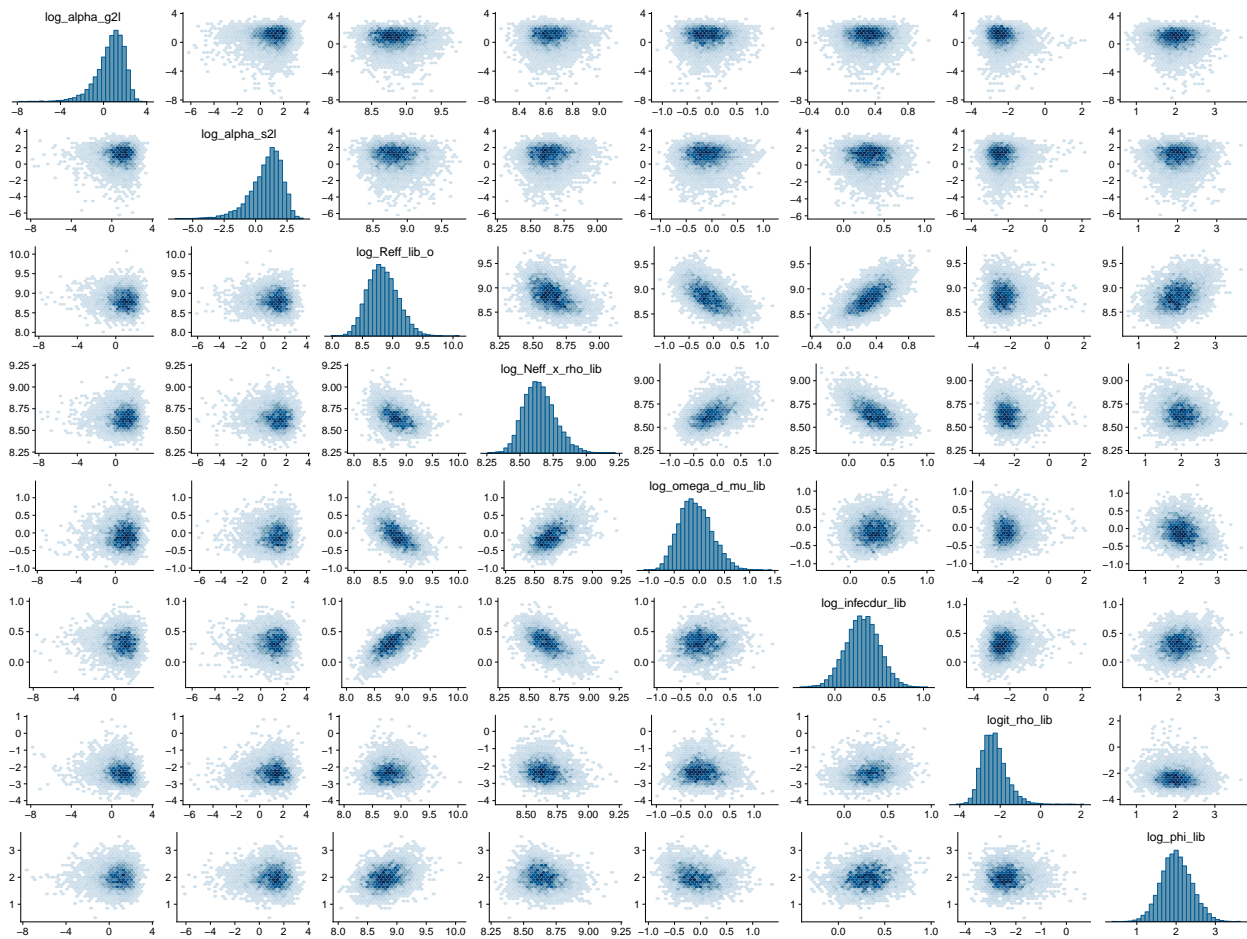
Figure B.35: Scatterplots of Liberia-specific parameters in a stratified SEIR ODE model fit to data from the West Africa Ebola outbreak.
