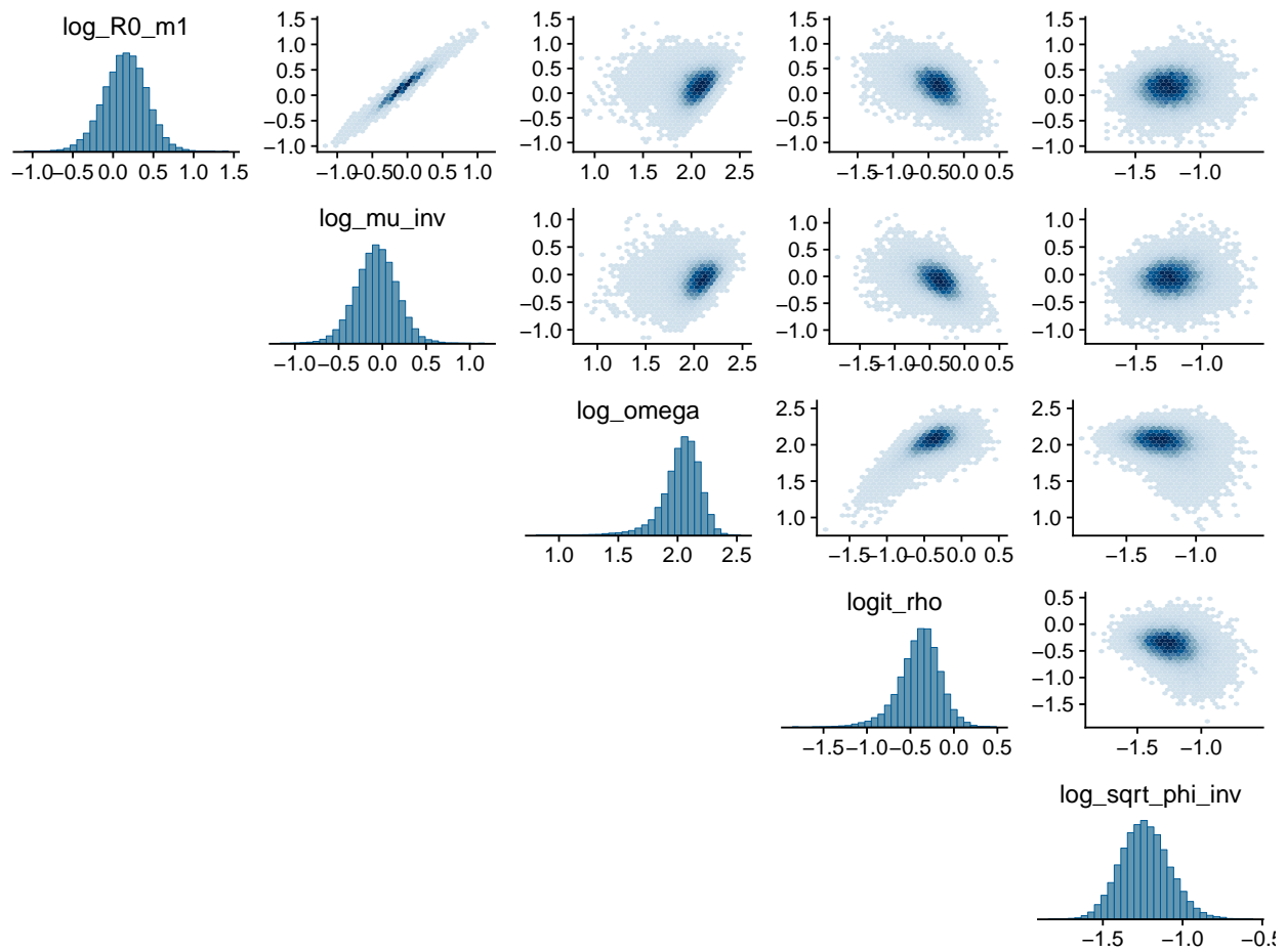
Figure C.4: Posterior histograms and pairwise hexplots for SIRS model parameters with time-homogeneous force of infection.
