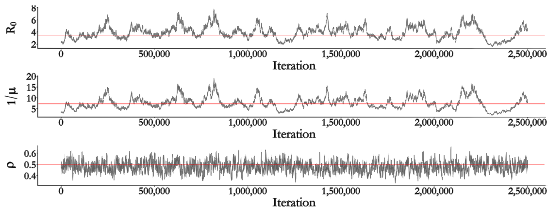
Figure 4.1: Posterior traceplots for parameters of interest for a single MCMC chain of an SIR model fit to negative binomial distributed incidence data. MCMC targeted the centered parameterization of the posterior (4.18), alternately updating the non-restarting LNA for \tilde{\mathbf{N}}|\theta, \mathbf{Y} via elliptical slice sampling, and \theta|\tilde{\mathbf{N}}, \mathbf{Y} via a multivariate random walk Metropolis algorithm. R_0 = \beta N/\mu is the basic reproductive number, 1/\mu is the mean infectious period duration, and \rho is the mean case detection rate. The true values (red lines) of R_0 , 1/\mu , and \rho were 3.5, 7, and 0.5, respectively.
