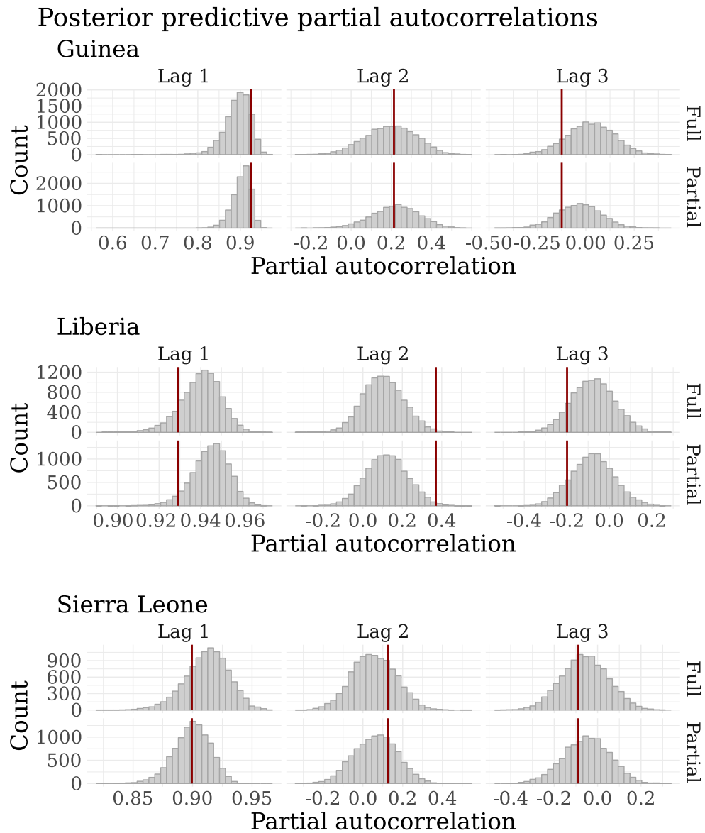
Figure 4.12: Distributions of partial autocorrelations at lags 1, 2, and 3 for datasets generated under the full and partial posterior predictive distributions. Vertical red lines are the partial autocorrelations for the observed incidence data at the respective lags.
