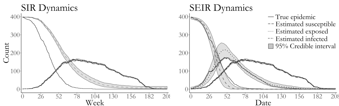
Figure 3.6: True epidemic path (solid lines), pointwise posterior median estimate of the numbers of susceptibles (dashed line), exposed (dotted line), and infected individuals (dash-dotted line) and pointwise 95% credible intervals (shaded regions) under SIR and SEIR dynamics.
