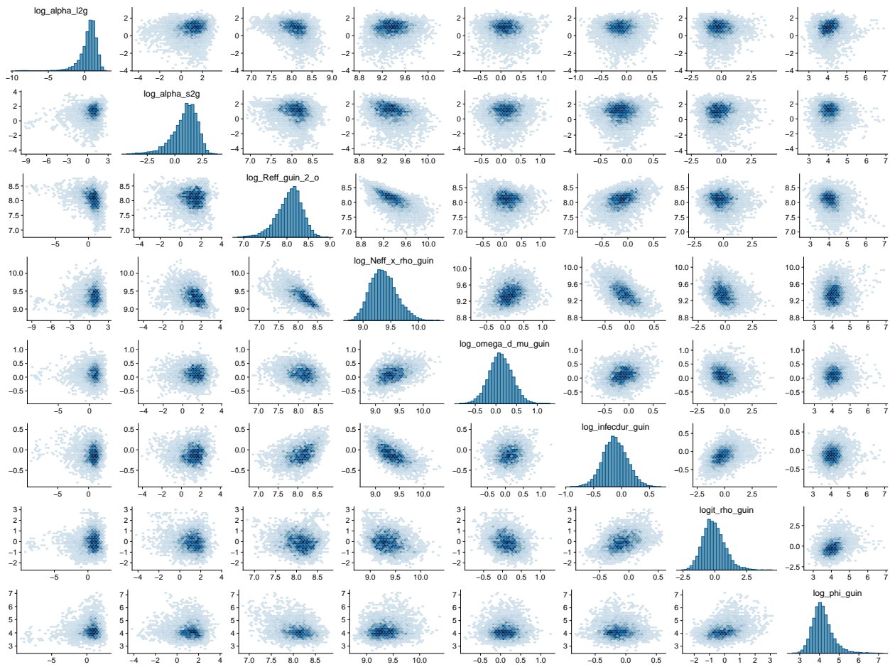
Figure B.7: Scatterplots of Guinea-specific parameters in a stratified SEIR model for a simulated Ebola outbreak.
