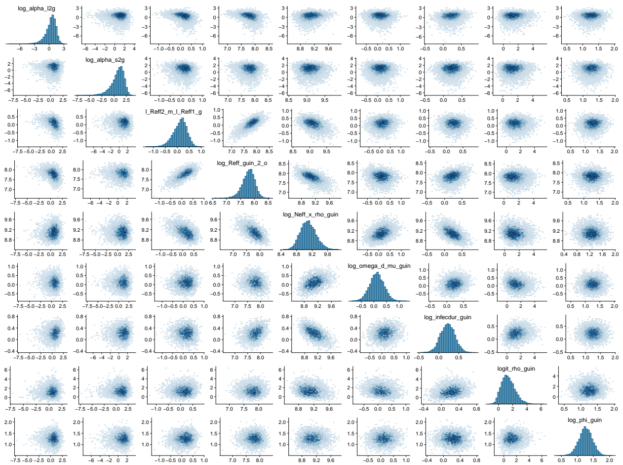
Figure B.34: Scatterplots of Guinea-specific parameters in a stratified SEIR ODE model fit to data from the West Africa Ebola outbreak.
