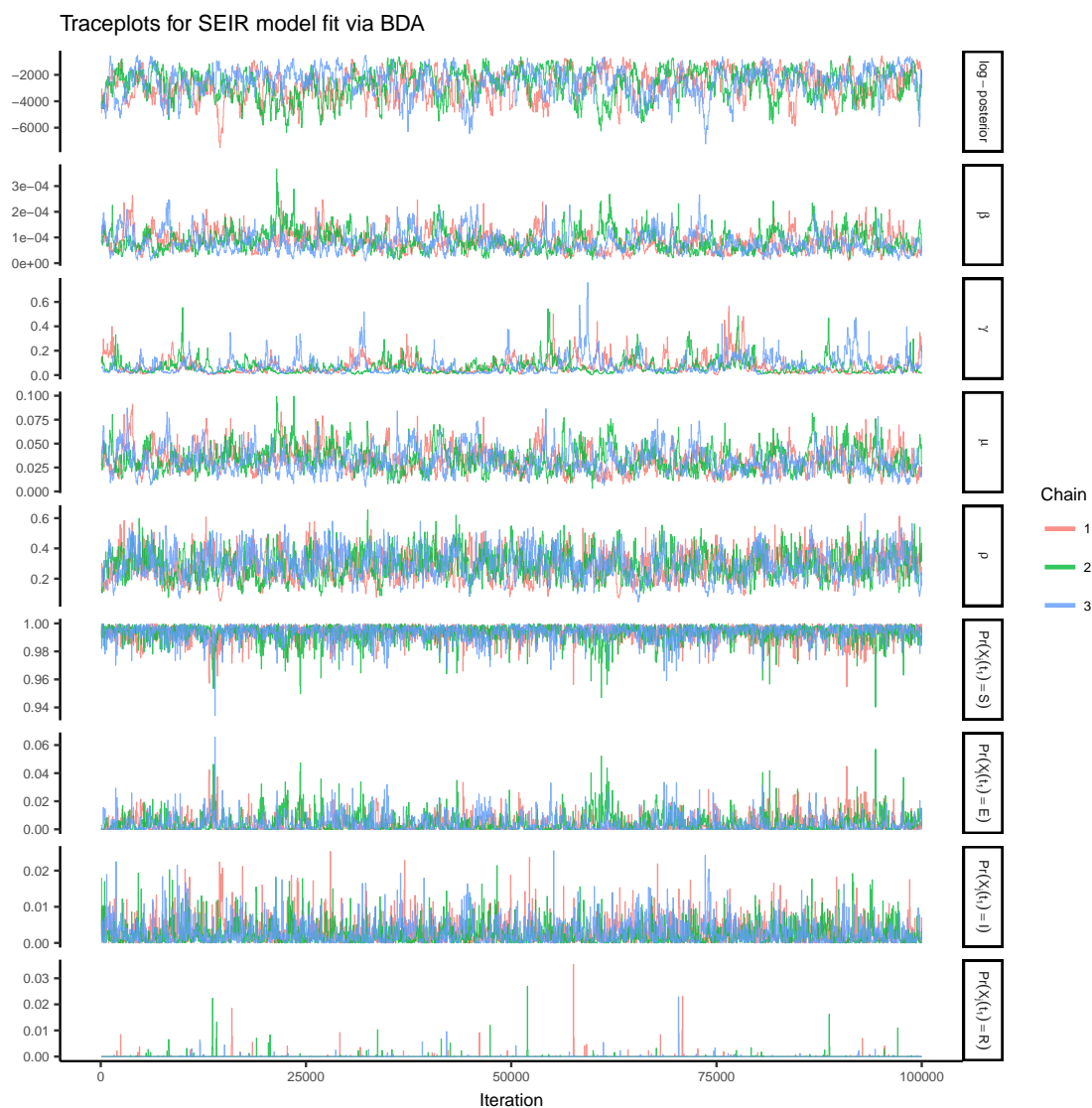
Figure A.4: Traceplots of the log-posterior and model parameters for the SEIR model fit using Bayesian data augmentation following an initial burn-in of 10 iterations. \beta denotes the per-contact infectivity rate, \gamma is the rate at which exposed individuals become infectious, \mu is the recovery rate, \rho is the binomial sampling probability. Traceplots are thinned to display every 50 th iteration.
