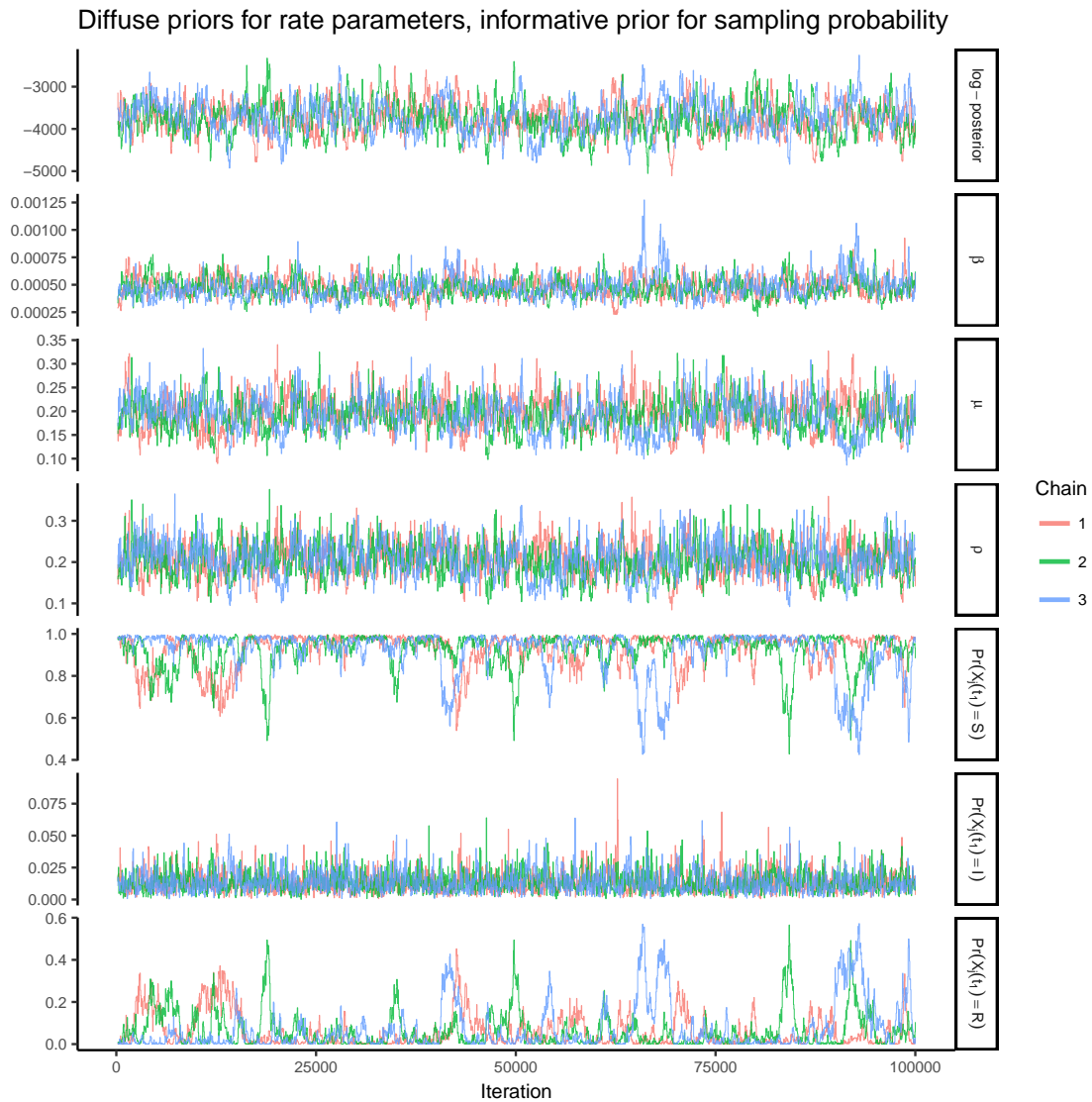
Figure A.17: Traceplots of the log-posterior and model parameters for the SIR model fit under diffuse priors for the rate parameters and an informative prior for the binomial sampling probability. \beta denotes the per-contact infectivity rate, \mu is the recovery rate, \rho is the binomial sampling probability. Traceplots are thinned to display every 50 th iteration.
