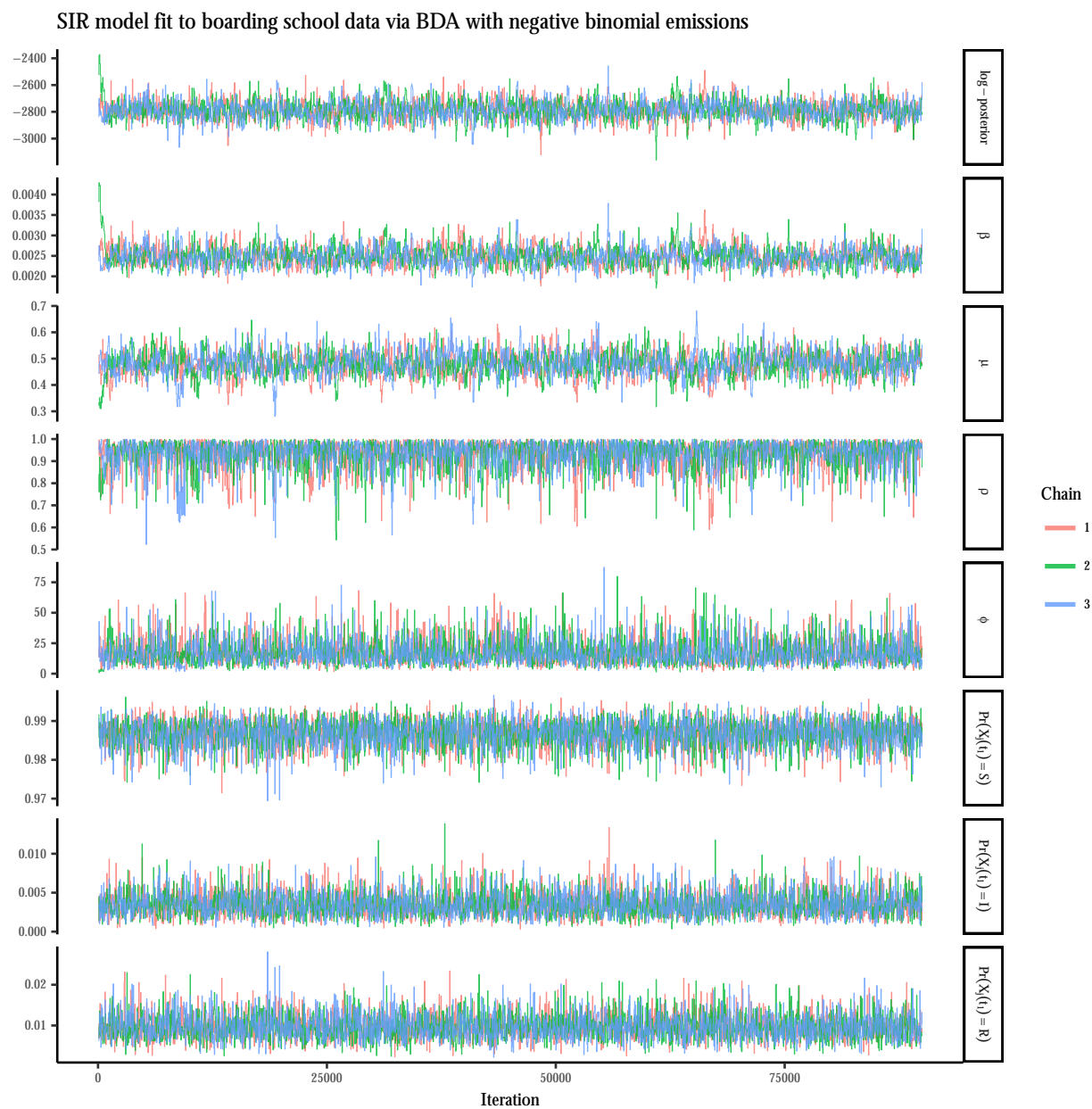
Figure A.27: Traceplots of the log-posterior and model parameters for the SIR model fit under negative binomial emissions using BDA following an initial burn-in of 100 iterations. \beta denotes the per-contact infectivity rate, \mu is the recovery rate, and \rho is the binomial sampling probability. Traceplots are thinned to display every 50 th iteration.
