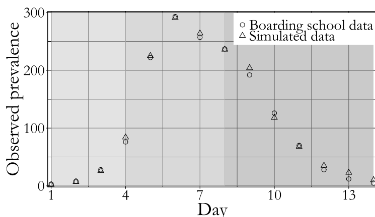
Figure A.24: British boardings school data and data simulated under SEIR dynamics with time-varying dynamics over three epochs (indicated by different shaded regions). The simulated dataset was generated using the following parameters: in the first epoch (days 1-4), \beta = 0.0035 , \gamma = 1.25 , \mu = 0.3 . In the second epoch (days 4-8), \beta = 0.065 , \gamma = 0.51 , \mu = 0.41 . In the third epoch (days 8-14), \beta = 0.06 , \gamma = 2.5 , \mu = 0.54 . The data were a binomial sample of the true prevalence with detection probability \rho = 0.98 . There were three exposed individuals and two infected individuals at the beginning of day 1.
