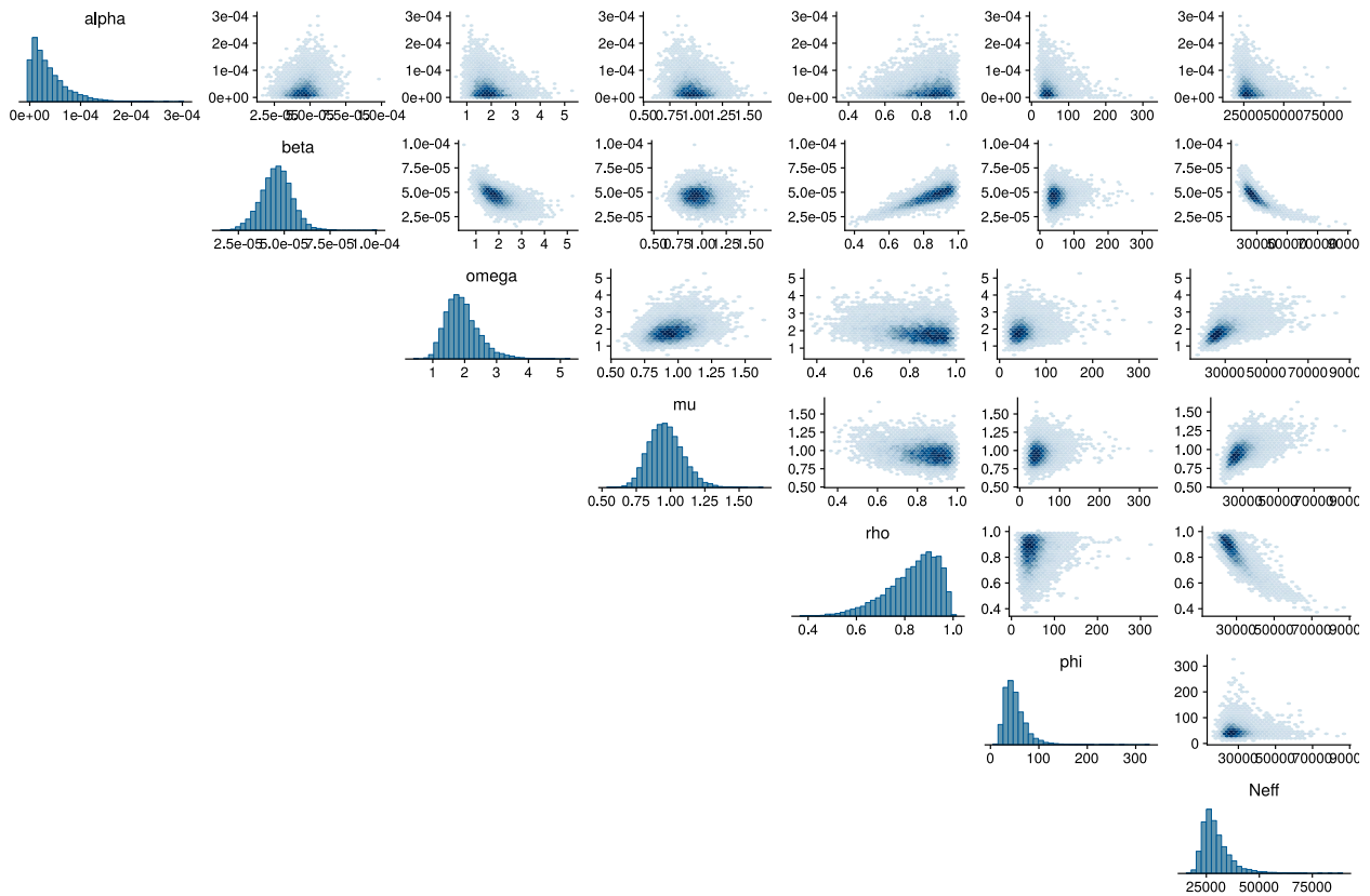
Figure B.2: Marginal histograms and pairwise scatterplots of posterior samples for parameters for the SEIR model fit to the Sierra Leone Ebola dataset using the estimation scale in Table B.3. The parameters on the estimation scales in this figure and their interpretations are provided in Table B.1.
