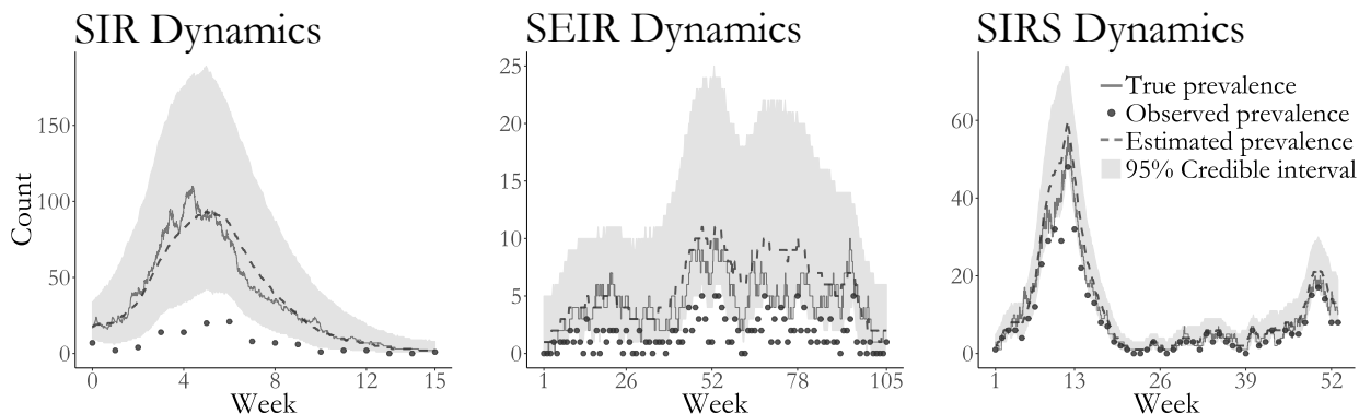
Figure 3.3: Estimated latent posterior distributions of disease prevalence in outbreaks simulated under SIR (left), SEIR (middle), and SIRS (right) dynamics. Depicted are the true unobserved prevalence (solid line), observed data (dots), pointwise posterior median prevalence (dashed line), and pointwise 95% credible intervals (shaded region). Latent posterior estimates are based on a thinned sample, with every 250 th sample retained.
