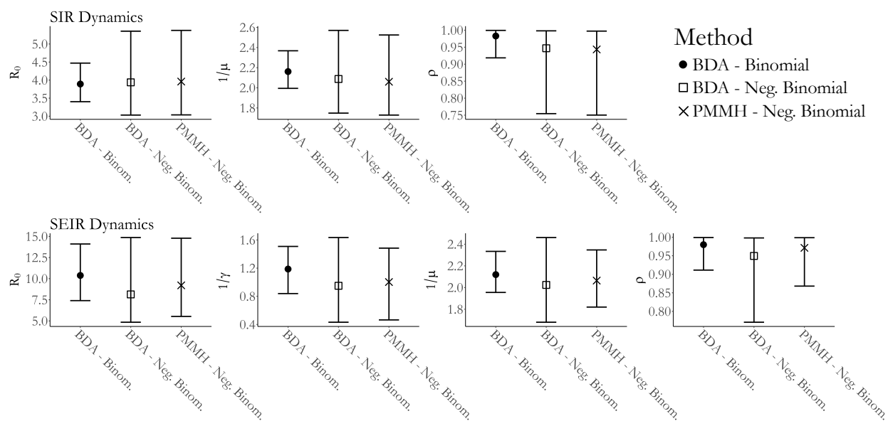
Figure A.26: Posterior medians and 95% credible intervals for SIR and SEIR models fit with BDA and PMMH to the British boarding school data under binomial and negative binomial emission distributions.
