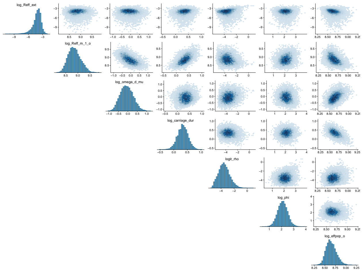
Figure B.14: Scatterplots of parameters for the SEIR LNA model fit to data from the Ebola outbreak in Liberia.
