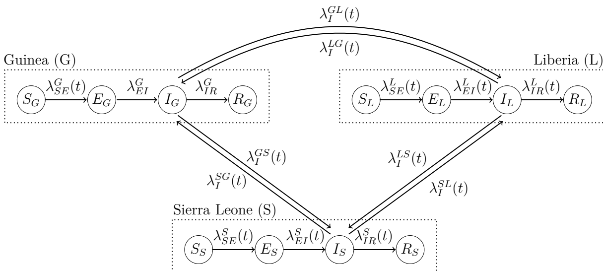
Figure B.5: Diagram of state transitions for a stratified SEIR model used in simulating an outbreak in Guinea, Liberia, and Sierra Leone. Dashed boxes denote countries, nodes in circles denote the model compartments: susceptible (S), exposed (E), infectious (I), recovered (R). Compartments are subscripted with country indicators. The number of susceptible individuals is equal to the effective population size, estimated as a parameter in the model, minus the numbers of exposed, infected, and recovered individuals. Solid lines with arrows indicate stochastic transitions between model compartments, which occur continuously in time. Rates at which individuals transition between compartments are denoted by \lambda and are subscripted by compartments and superscripted by countries, e.g., \lambda_{SE}^L is the rate at which susceptible individuals become exposed in Liberia, \lambda_I^{SG} is the rate at which an infected individual in Sierra Leone migrates to Guinea. The rate at which susceptible individuals in Guinea become infected is time varying with one changepoint at 33 weeks. Transmission in Liberia and Sierra Leone commenced at 10 and 19 weeks, respectively. Full expressions for the rates are given in Table B.19.
