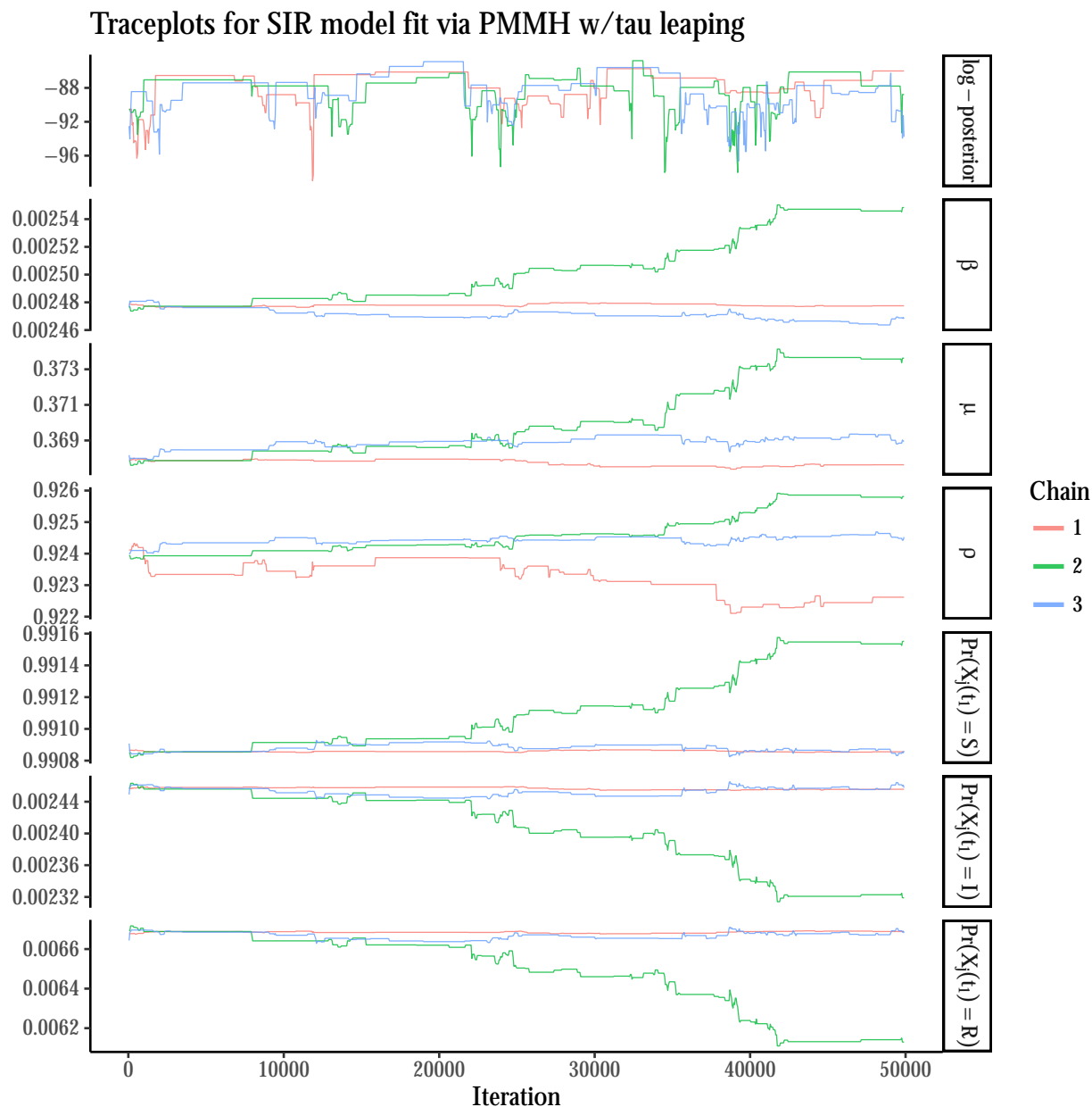
Figure A.22: Traceplots of the log-posterior and model parameters for the SIR model fit under binomial emissions using PMMH with 5,000 particles per chain and a time-step of 2 hours in the approximate \tau -leaping algorithm, following a tuning run of 2,000 iterations to estimate the RWMH covariance matrix and in initial burn-in of 100 iterations. \beta denotes the per-contact infectivity rate, \mu is the recovery rate, and \rho is the binomial sampling probability. Traceplots are thinned to display every 50 th iteration.
