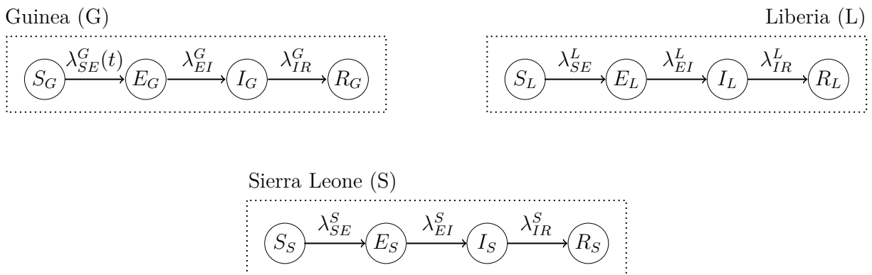
Figure 4.15: Diagram of state transitions for SEIR models fit to Ebola incidence data from Guinea, Liberia, and Sierra Leone. Dotted boxes denote countries, nodes in circles denote the model compartments: susceptible (S), exposed (E), infectious (I), recovered (R). Compartments are subscripted with country indicators. The number of susceptible individuals is equal to the effective population size, estimated as a parameter in the model, minus the numbers of exposed, infected, and recovered individuals. Solid lines with arrows indicate stochastic transitions between model compartments, which occur continuously in time. Rates at which individuals transition between compartments are denoted by \lambda and are subscripted by compartments and superscripted by countries, e.g., \lambda_{SE}^L is the rate at which susceptible individuals become exposed in Liberia. The rate at which susceptibles in Guinea become infected is time varying with one change-point at 33 weeks. Transmission in Liberia and Sierra Leone commenced at 10 and 19 weeks, respectively. Full expressions for the rates are given in Table B.24.
