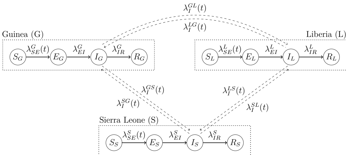
Figure 4.9: Diagram of state transitions for a stratified SEIR model fit to a simulated Ebola outbreak in Guinea, Liberia, and Sierra Leone. Dotted boxes denote countries, nodes in circles denote the model compartments: susceptible (S), exposed (E), infectious (I), recovered (R). Compartments are subscripted with country indicators. Solid lines with arrows indicate stochastic transitions between model compartments, which occur continuously in time. Dashed lines indicate virtual migrations, where infected individuals in one country contribute to the force of infection in another country but do not migrate. Rates at which individuals transition between compartments are denoted by \lambda and are subscripted by compartments and superscripted by countries, e.g., \lambda_{SE}^L is the rate at which susceptible individuals become exposed in Liberia, \lambda_I^{SG} is the rate at which an infected individual in Sierra Leone migrates to Guinea. The rate at which susceptibles in Guinea become infected is time varying with one change-point at 33 weeks. Transmission in Liberia and Sierra Leone commenced at 10 and 19 weeks, respectively. Full expressions for the rates are given in Table B.20.
