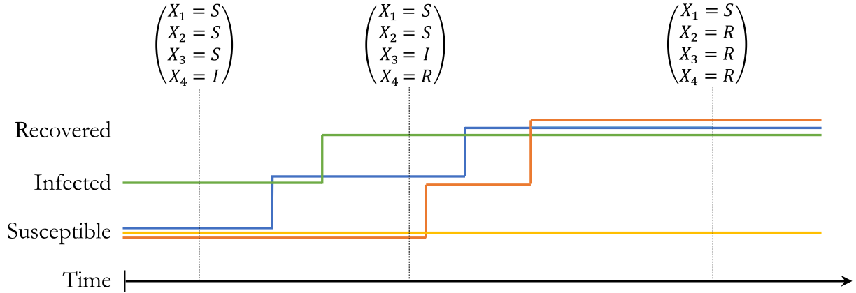
Figure 2.2: Diagram of subject-level paths (colored lines) for an SIR model in a population of size N=4 . Individuals transition through infection states continuously in time. The epidemic process is defined in terms of the infection states of individuals in the population.
