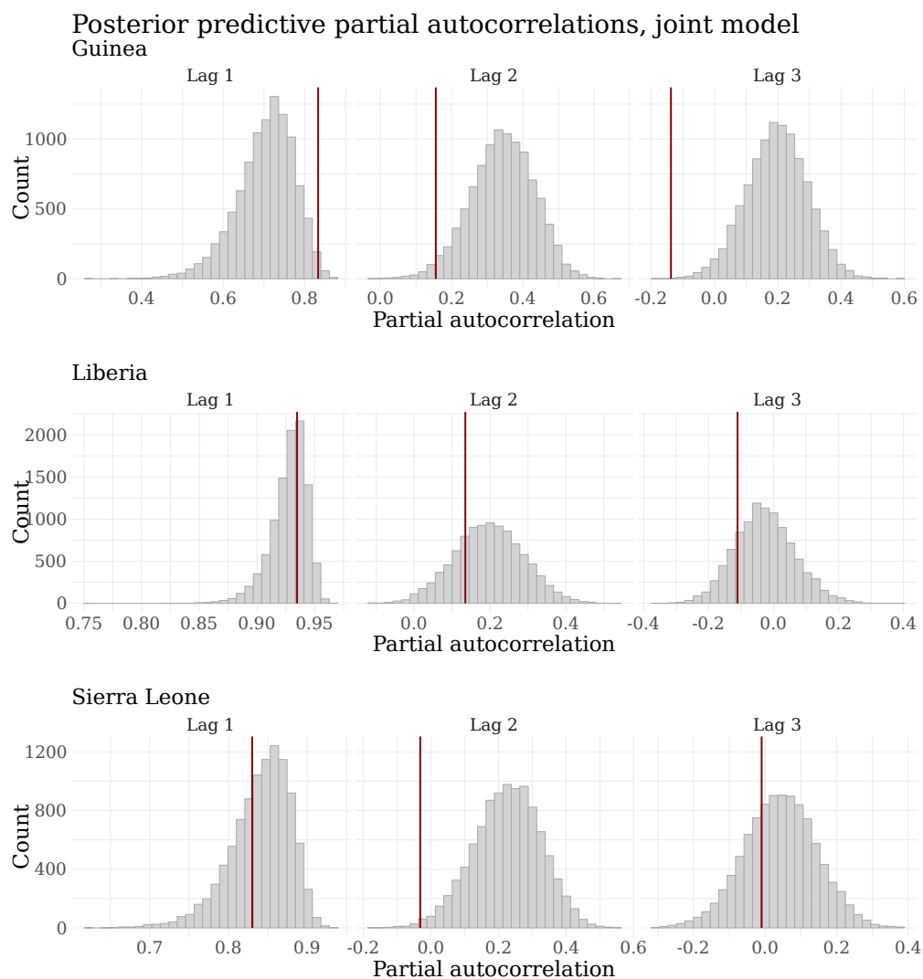
Figure B.37: Distributions of partial autocorrelations at lags 1, 2, and 3 for datasets generated under the full and partial posterior predictive distributions for the main stratified SEIR model fit via the ODE to data from the West Africa Ebola outbreak. Vertical red lines are the partial autocorrelations for the observed incidence data at the respective lags.
