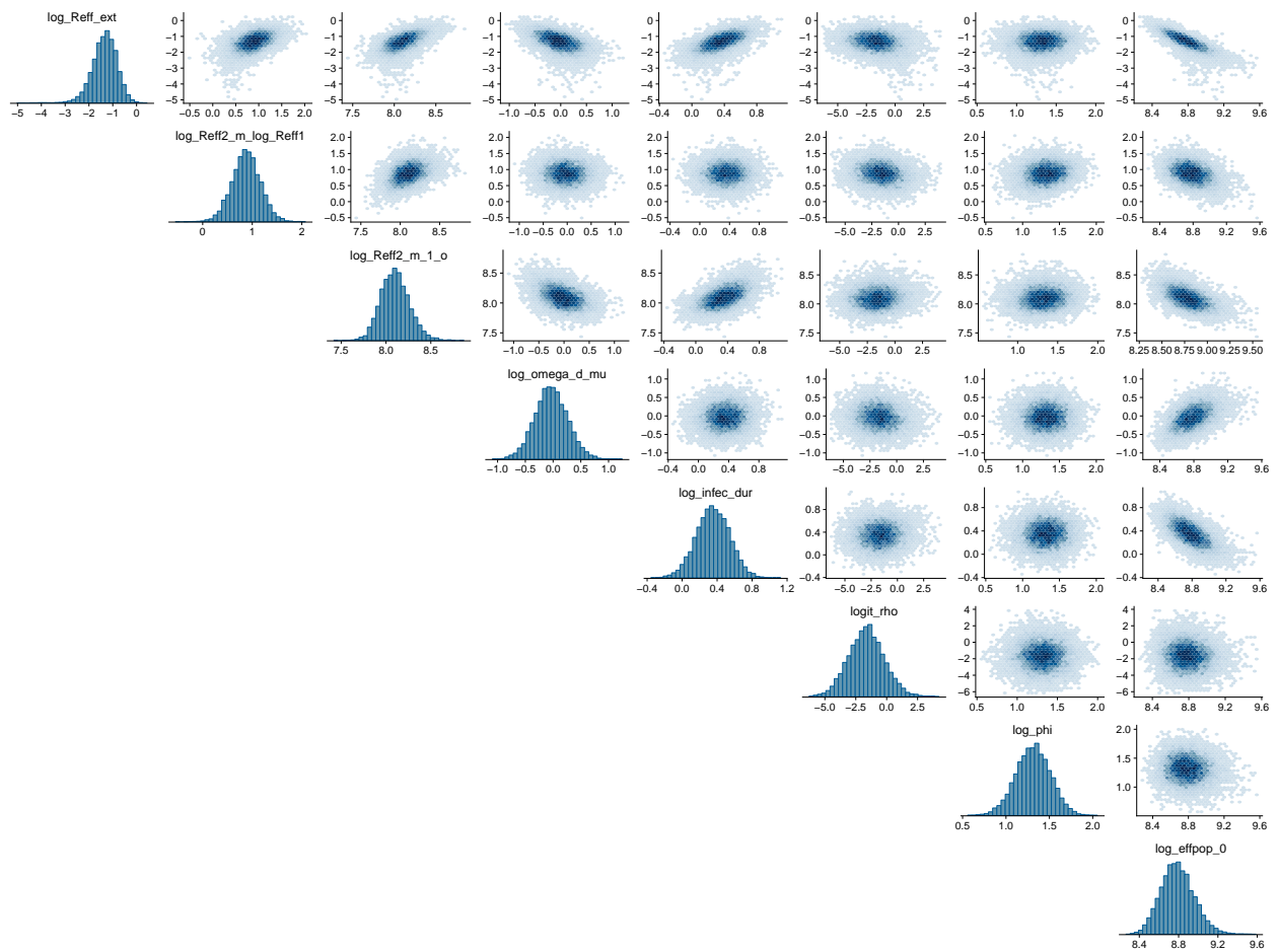
Figure B.20: Scatterplots of parameters for the SEIR ODE model fit to data from the Ebola outbreak in Guinea.
