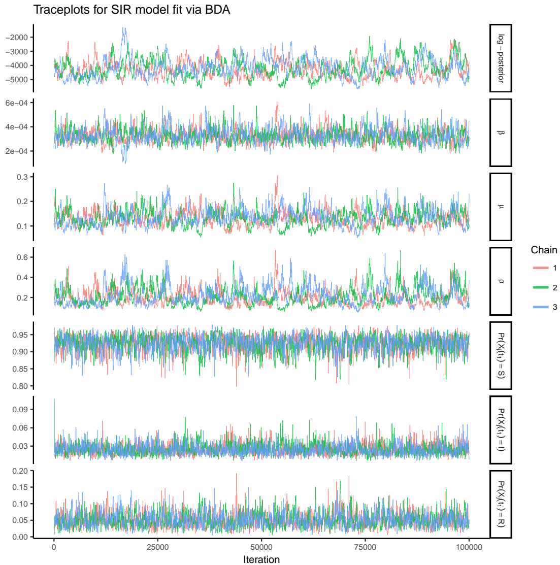
Figure A.1: Traceplots of the log-posterior and model parameters for the SIR model fit using Bayesian data augmentation following an initial burn-in of 10 iterations. \beta denotes the per-contact infectivity rate, \mu is the recovery rate, \rho is the binomial sampling probability. Traceplots are thinned to display every 50 th iteration.
