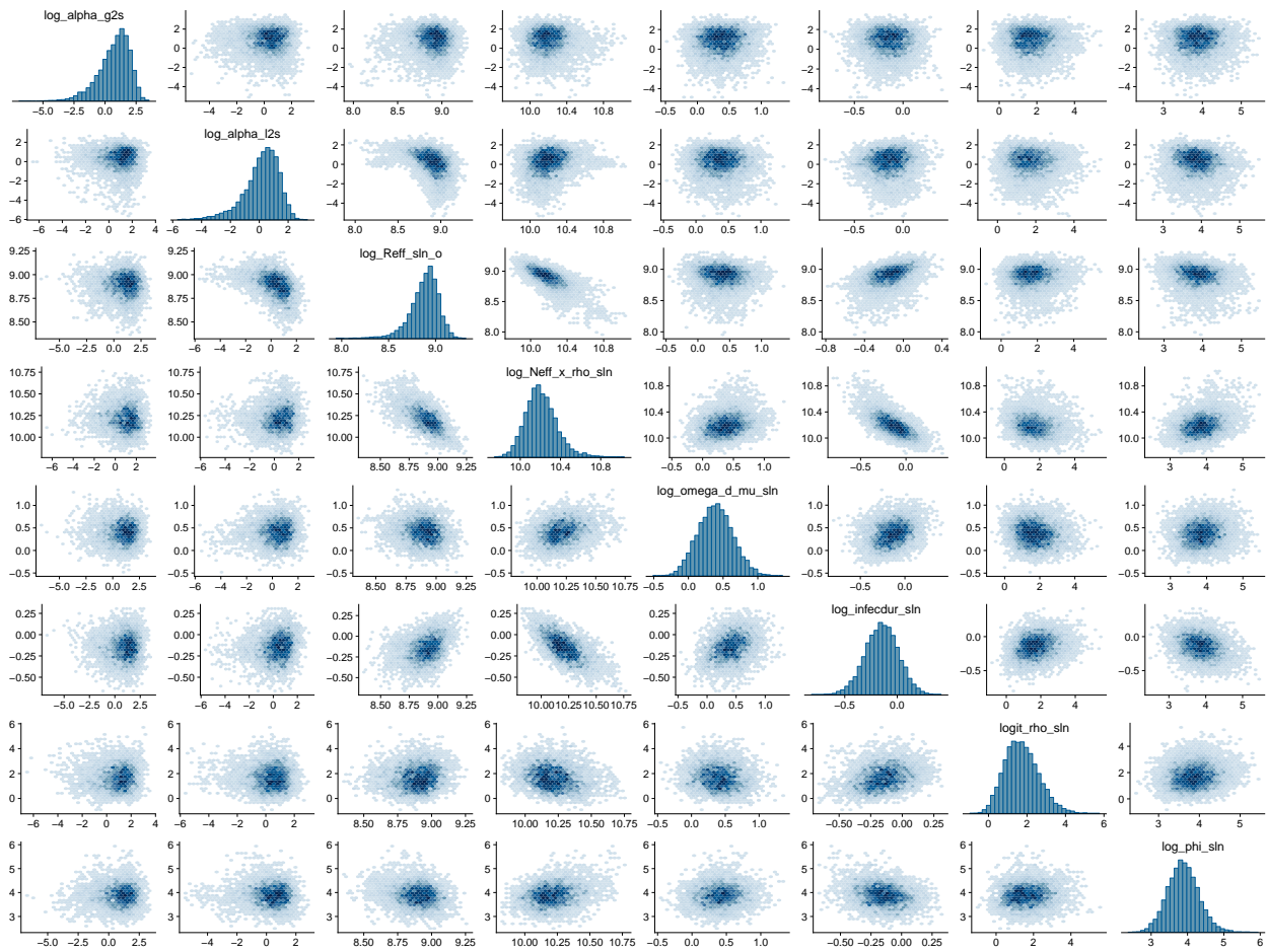
Figure B.30: Scatterplots of Sierra Leone-specific parameters in a stratified SEIR LNA model fit to data from the West Africa Ebola outbreak.
