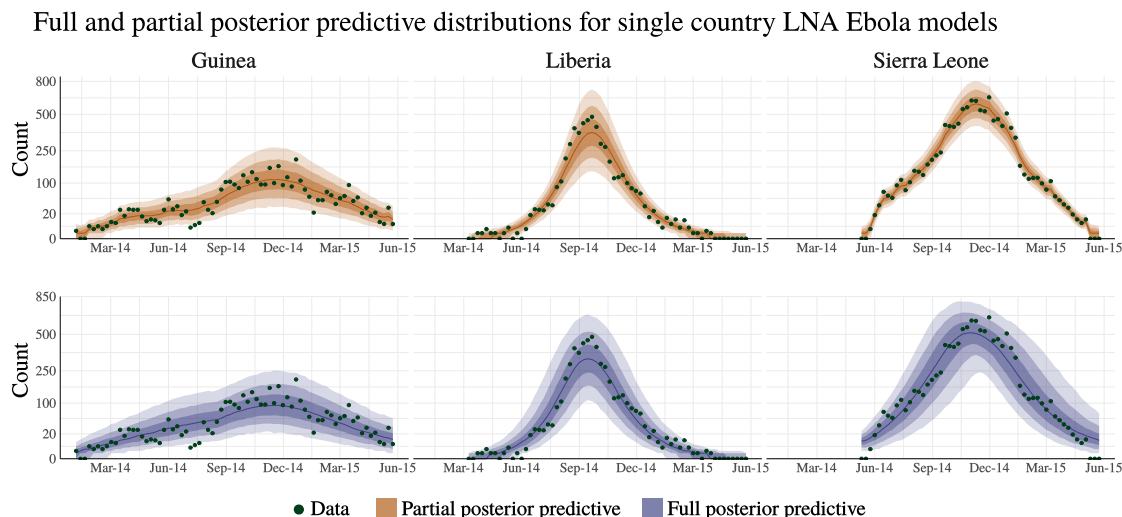
Figure 4.16: Partial and full posterior predictive distributions for country-specific SEIR LNA models for the West Africa Ebola outbreak. Green points correspond to the observed incidence. The shaded bands, in order of lightest to darkest, correspond to pointwise posterior 95%, 80%, and 50% credible intervals, with the pointwise posterior median given by the corresponding colored solid line.
