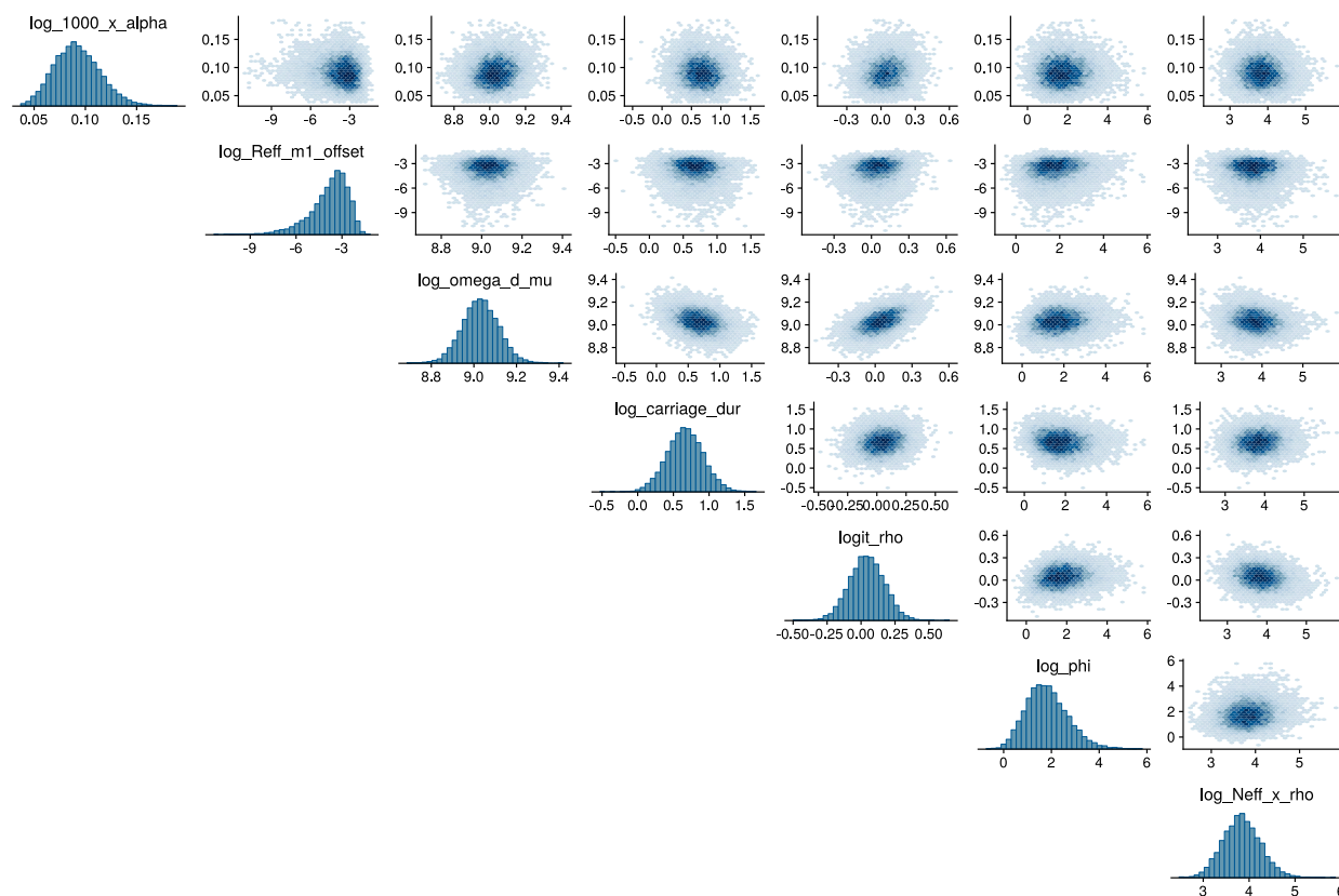
Figure B.4: Marginal histograms and pairwise scatterplots of posterior samples for parameters for the SEIR model fit to the Sierra Leone Ebola dataset using the estimation scale in Table B.3. The parameters on the estimation scales in this figure and their interpretations are provided in Table B.3.
