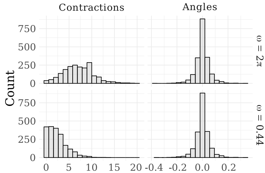
Figure B.1: Distributions of the numbers of contractions per ElliptSS update and the accepted angles for an MCMC chain for the joint Ebola model of Section 4.4 . An initial bracket width of 2\pi was used for the first 5,000 iterations (top row), after which the initial bracket width was set to 2\sqrt{2\log(10)\sigma_{ElliptSS}} , where \sigma_{ElliptSS} was the standard deviation of the accepted angles from the initial run (bottom row).
