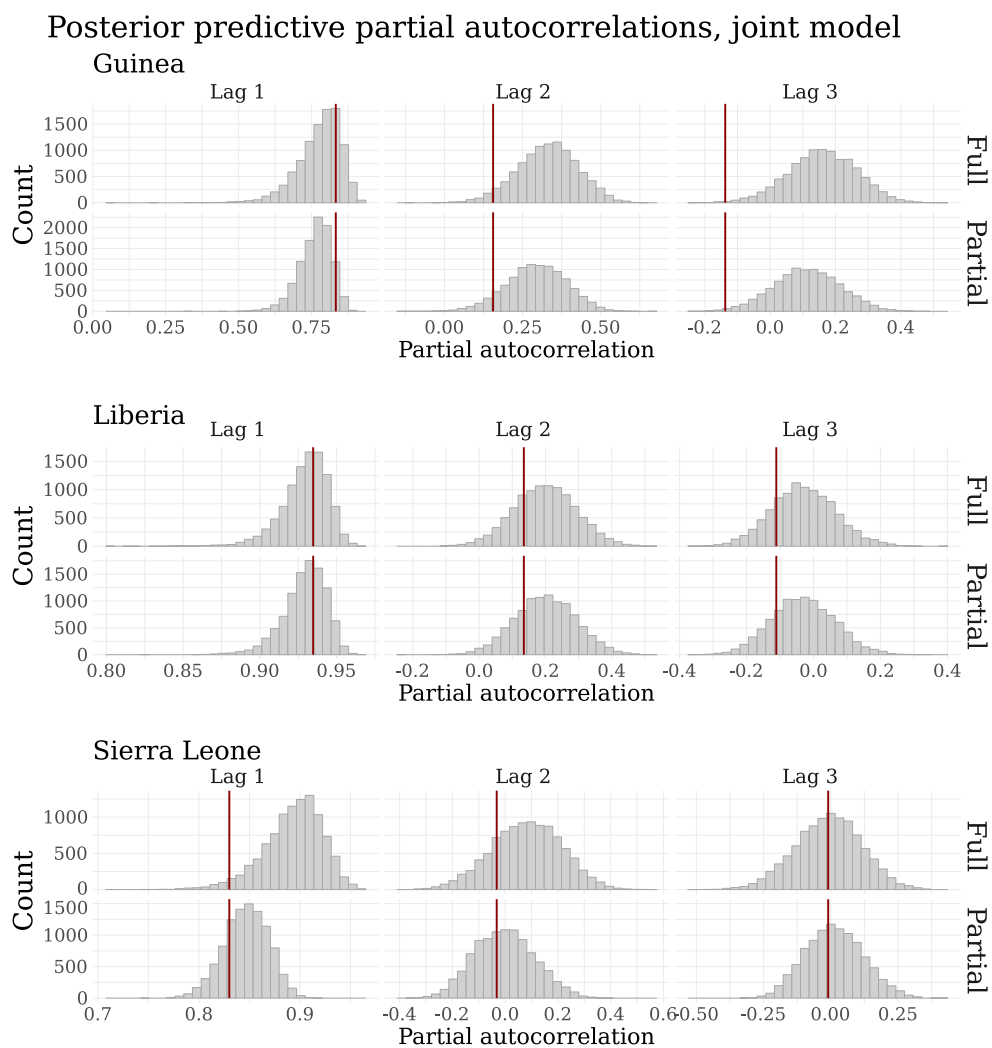
Figure B.31: Distributions of partial autocorrelations at lags 1, 2, and 3 for datasets generated under the full and partial posterior predictive distributions for the main stratified SEIR LNA model fit to data from the West Africa Ebola outbreak. Vertical red lines are the partial autocorrelations for the observed incidence data at the respective lags.
