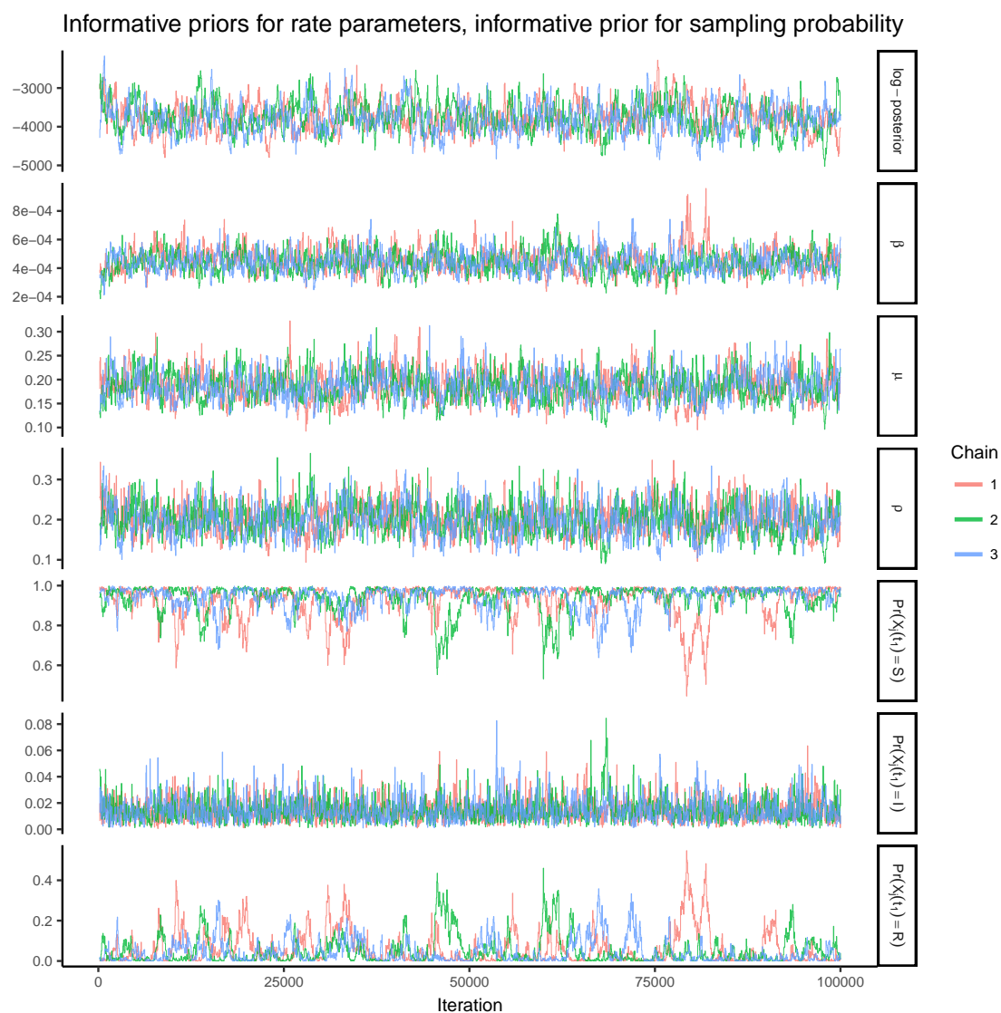
Figure A.16: Traceplots of the log-posterior and model parameters for the SIR model fit under informative priors for all model parameters. \beta denotes the per-contact infectivity rate, \mu is the recovery rate, \rho is the binomial sampling probability. Traceplots are thinned to display every 50 th iteration.
