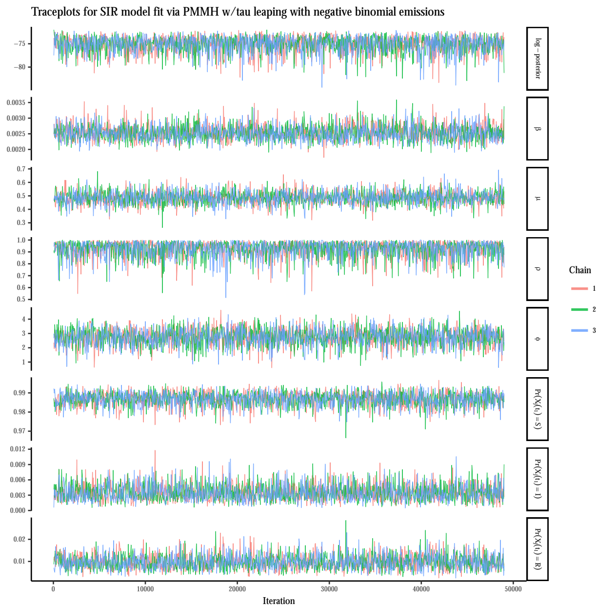
Figure A.29: Traceplots of the log-posterior and model parameters for the SIR model fit under negative binomial emissions using PMMH with 5,000 particles per chain and a time-step of 2 hours in the approximate \tau -leaping algorithm, following a tuning run of 2,000 iterations to estimate the RWMH covariance matrix and in initial burn-in of 100 iterations. \beta denotes the per-contact infectivity rate, \mu is the recovery rate, and \rho is the binomial sampling probability. Traceplots are thinned to display every 50 th iteration.
