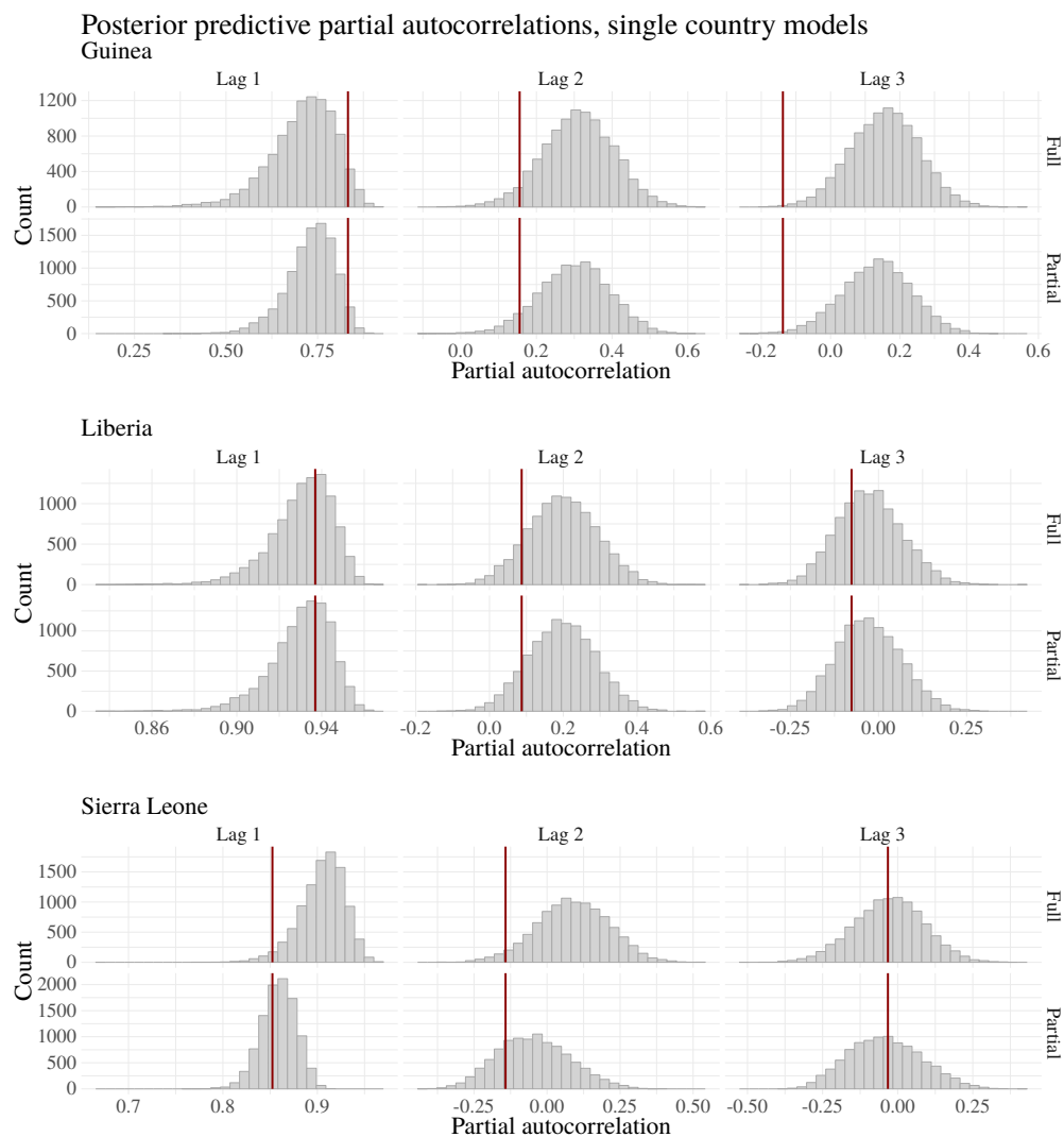
Figure B.17: Distributions of partial autocorrelations at lags 1, 2, and 3 for datasets generated under the full and partial posterior predictive distributions for the main country-specific SEIR LNA models fit to data from the West Africa Ebola outbreak. Vertical red lines are the partial autocorrelations for the observed incidence data at the respective lags.
