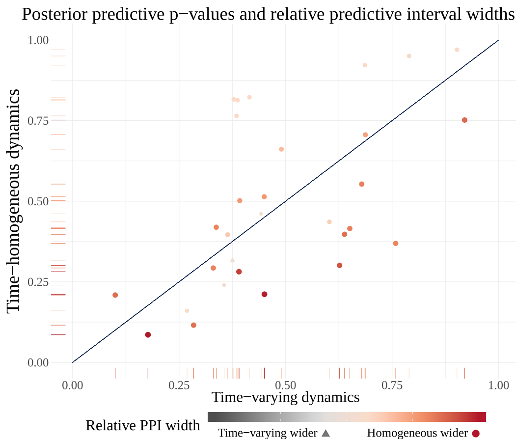
Figure 4.6: Comparison of models with time-varying and constant force of infection using posterior predictive p-values (PPPs) and relative posterior predictive interval (PPI) widths. Each point corresponds to the observed incidence in a given week. The X–Y coordinates give the PPPs under a model with a time-varying force of infection (FOI), where R_0 was modeled as a Gaussian Markov random field of order one, the PPP under a model with constant per-contact infection rate. The size and color of each point corresponds to the relative PPI width, computed as (\hat{\sigma}_{post,\ell}^{constant} - \hat{\sigma}_{post,\ell}^{RW1})/\hat{\sigma}_{post,\ell}^{RW1} , and the sign of the relative width is further emphasized by the shape of the point. Dots indicate that PPIs with constant FOI are wider, the lone triangle corresponds to the one data point where the PPI for the model with time-varying FOI was wider.
