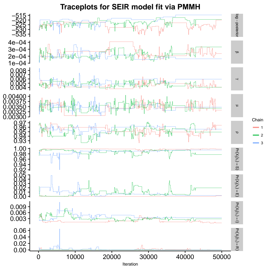
Figure A.15: Traceplots of the log-posterior and model parameters for the SEIR model fit using PMMH with 2,500 particles, following a tuning run of 5,000 iterations used to estimate the covariance matrix for the RWMH. \beta denotes the per-contact infectivity rate, \gamma is the rate at which an exposed individual becomes infectious, \mu is the recovery rate, \rho is the binomial sampling probability. Traceplots are thinned to display every 50 th iteration.
