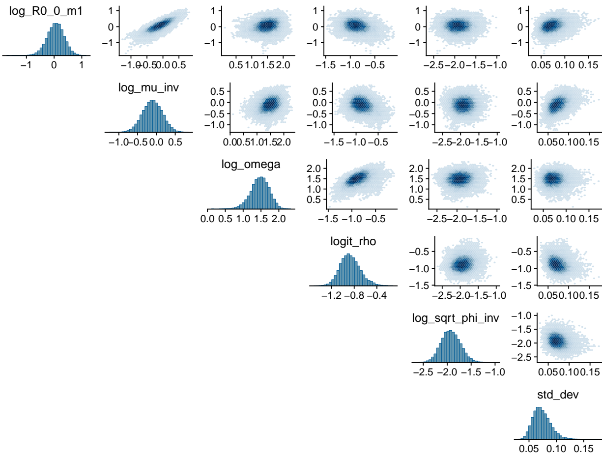
Figure C.2: Posterior histograms and pairwise hexplots for SIRS model parameters with time-varying force of infection.
