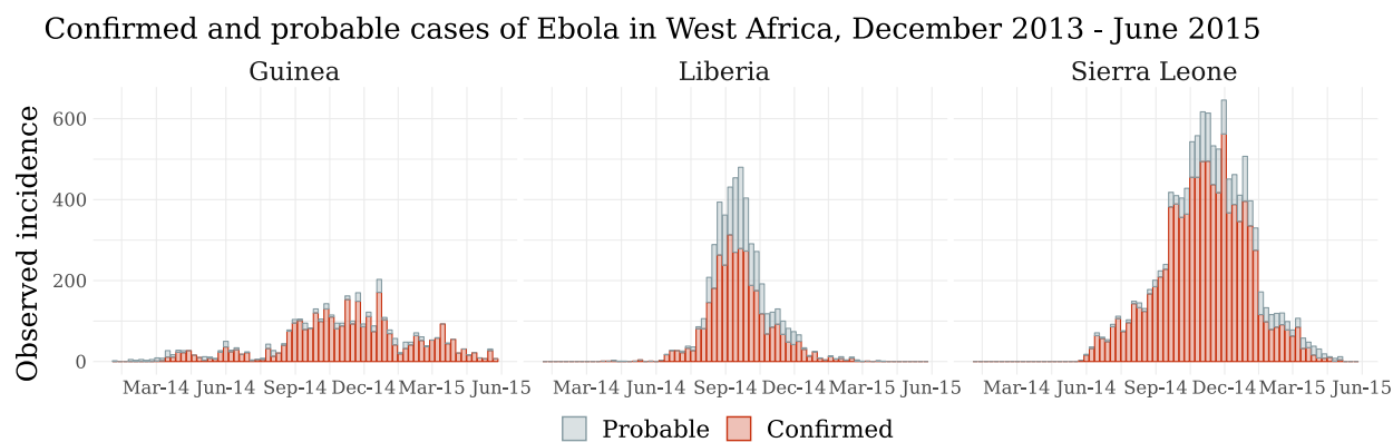
Figure 1.2: Weekly incidence of confirmed and probable cases of Ebola in Guinea, Liberia, and Sierra Leone.
