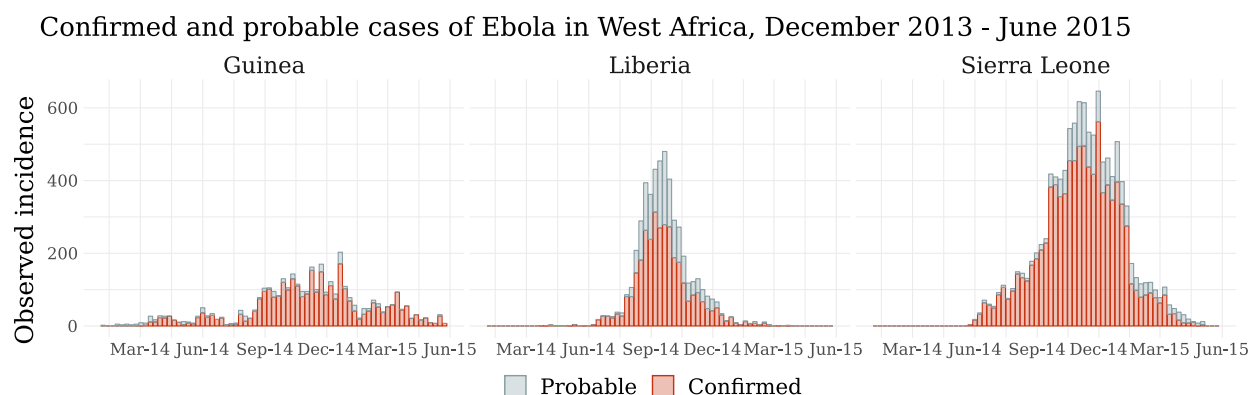
Figure 4.14: Weekly incidence of confirmed and probable cases of Ebola in Guinea, Liberia, and Sierra Leone.
