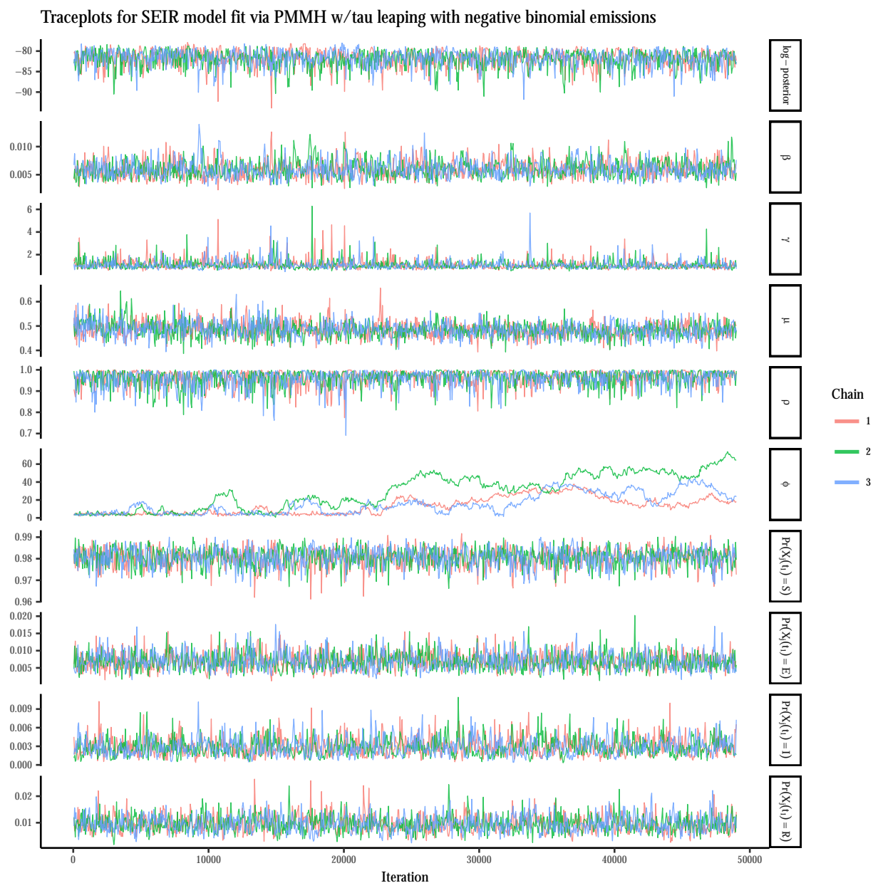
Figure A.30: Traceplots of the log-posterior and model parameters for the SEIR model fit under negative binomial emissions using PMMH with 5,000 particles per chain and a time-step of 2 hours in the approximate \tau -leaping algorithm, following a tuning run of 2,000 iterations to estimate the RWMH covariance matrix and in initial burn-in of 100 iterations. \beta denotes the per-contact infectivity rate, \mu is the recovery rate, \gamma is the rate at which immunity is lost, and \rho is the binomial sampling probability. Traceplots are thinned to display every 50 th iteration.
