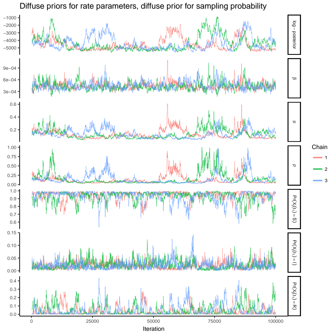
Figure A.19: Traceplots of the log-posterior and model parameters for the SIR model fit under diffuse priors for all model parameters. \beta denotes the per-contact infectivity rate, \mu is the recovery rate, \rho is the binomial sampling probability. Traceplots are thinned to display every 50 th iteration.
