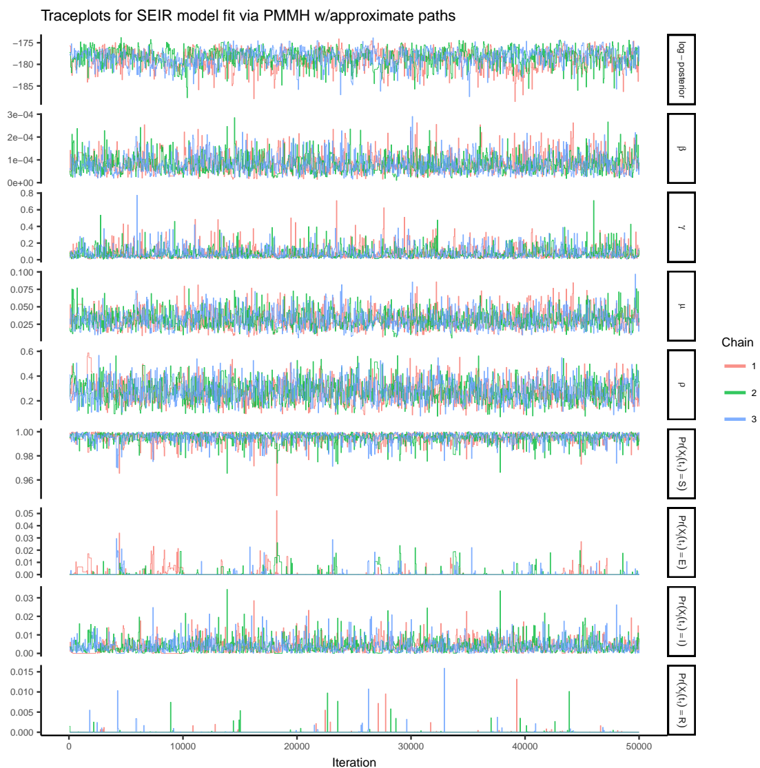
Figure A.5: Traceplots of the log-posterior and model parameters for the SEIR model fit using PMMH with 200 particles and a time step of 8 hours, following a tuning run of 5,000 iterations used to estimate the covariance matrix for the RWMH and an initial burn-in of 100 iterations. \beta denotes the per-contact infectivity rate, \gamma is the rate at which exposed individuals become infectious, \mu is the recovery rate, \rho is the binomial sampling probability. Traceplots are thinned to display every 50 th iteration.
