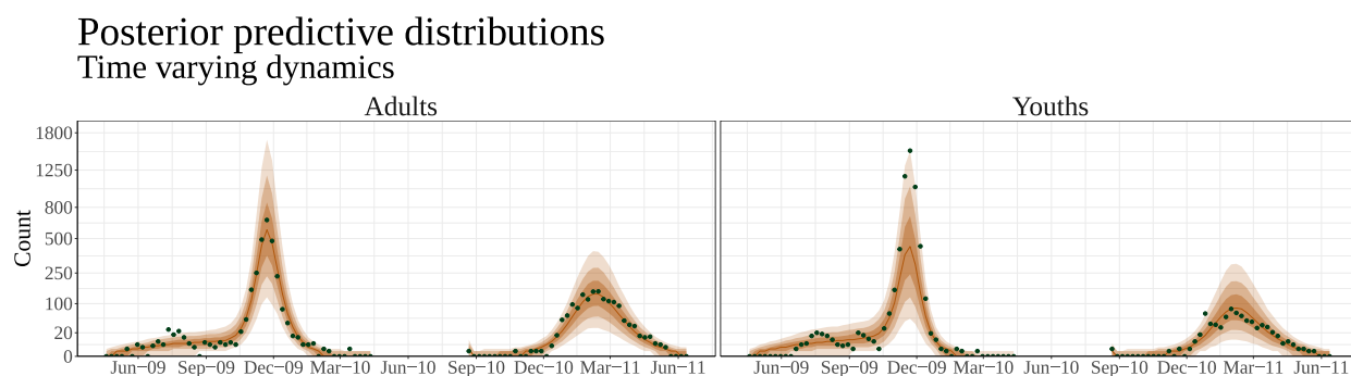
Figure 5.7: Posterior predictive distributions of a stratified SIRS ODE model with time-varying dynamics for A(H1N1)pdm09 in Finland.
