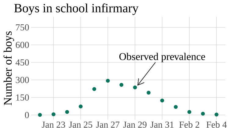
Figure 1.1: Data from an outbreak of influenza in a British boarding school.
