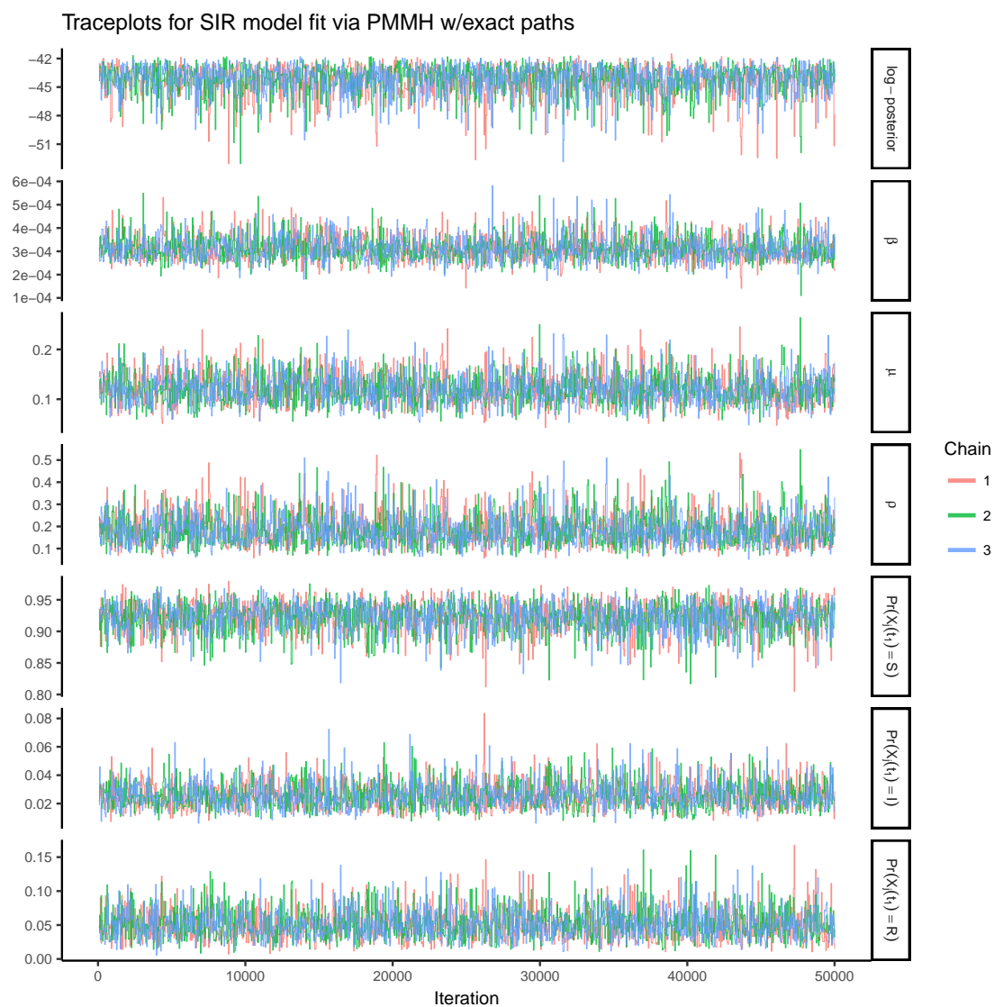
Figure A.3: Traceplots of the log-posterior and model parameters for the SIR model fit using PMMH with 100 particles, following a tuning run of 5,000 iterations used to estimate the covariance matrix for the RWMH and an initial burn-in of 100 iterations. \beta denotes the per-contact infectivity rate, \mu is the recovery rate, \rho is the binomial sampling probability. Traceplots are thinned to display every 50 th iteration.
