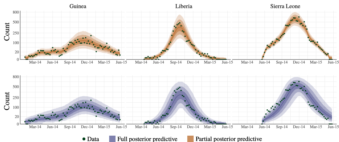
Figure 4.17: Partial and full posterior predictive distributions for a stratified SEIR LNA model for jointly modeling the Ebola outbreak in West Africa. Green points correspond to the observed incidence. The shaded bands, in order of lightest to darkest, correspond to pointwise posterior 95%, 80%, and 50% credible intervals, with the pointwise posterior median given by the corresponding colored solid line.
