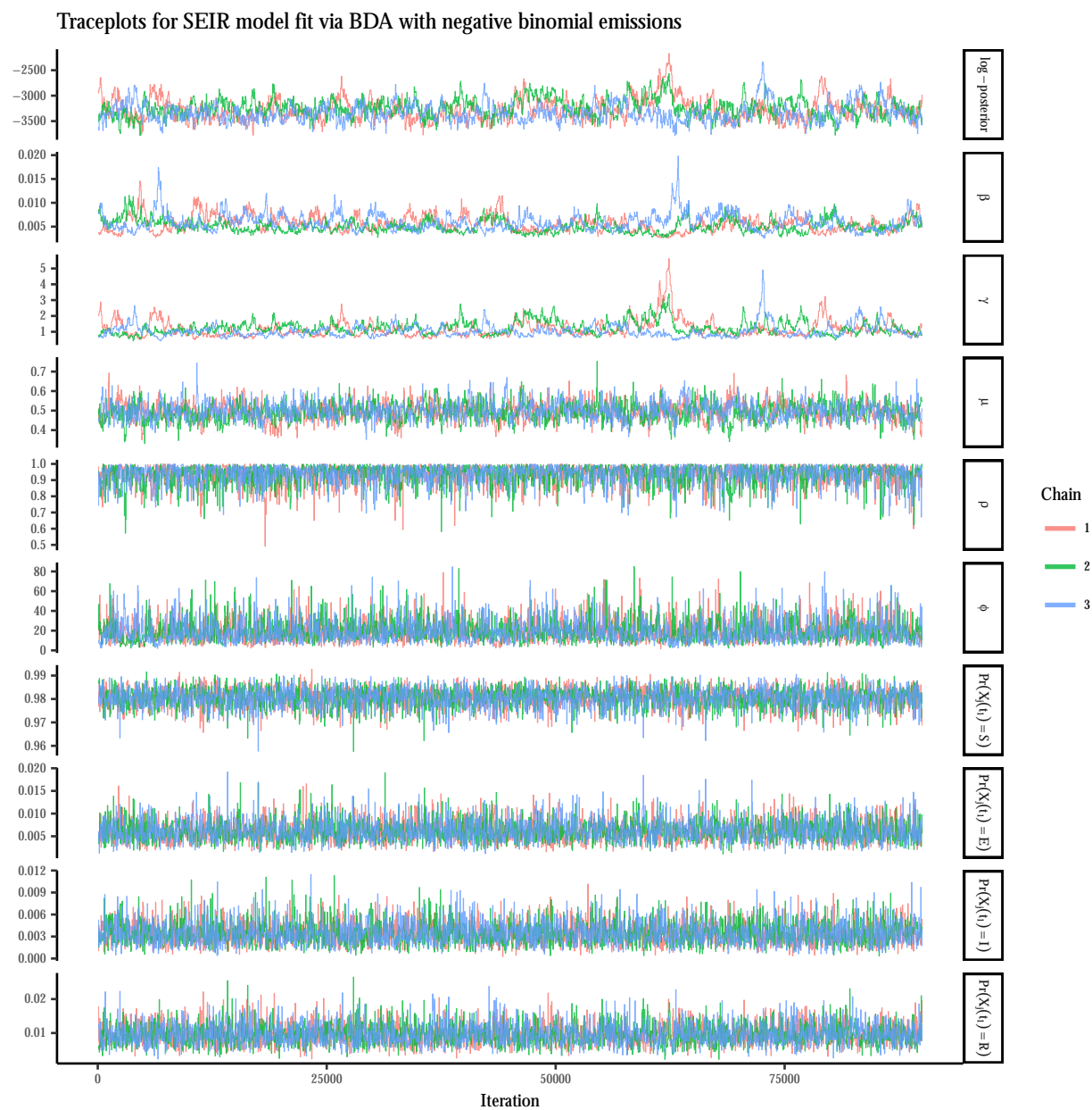
Figure A.28: Traceplots of the log-posterior and model parameters for the SEIR model fit under negative binomial emissions via BDA following an initial burn-in of 5,000 iterations. \beta denotes the per-contact infectivity rate, \mu is the recovery rate, \gamma is the rate at which immunity is lost, and \rho is the binomial sampling probability. Traceplots are thinned to display every 50 th iteration.
