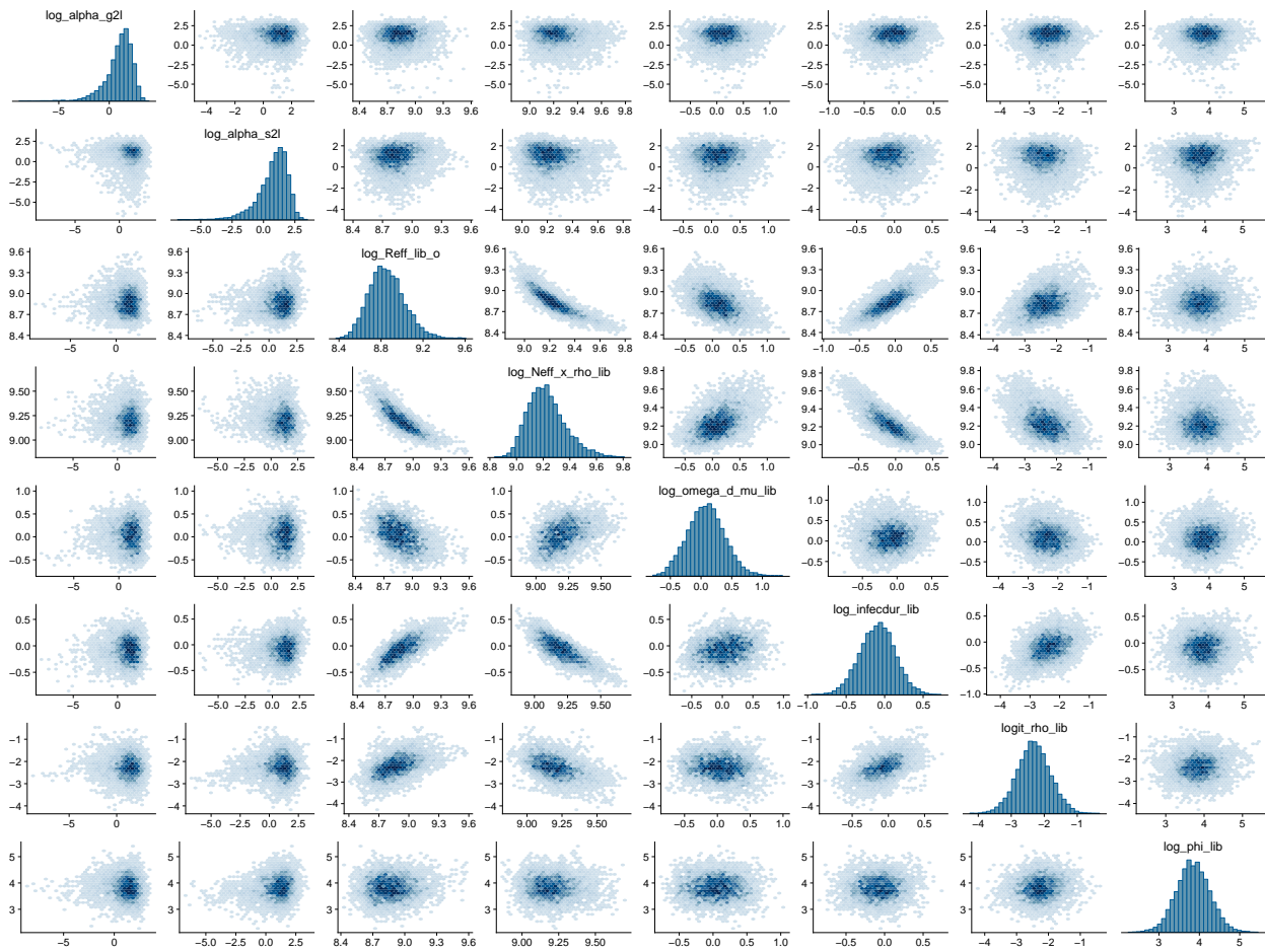
Figure B.8: Scatterplots of Liberia-specific parameters in a stratified SEIR model for a simulated Ebola outbreak.
