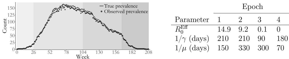
Figure 3.5: Simulated outbreak with SEIR dynamics that varied over four epochs (shaded regions). Weekly prevalence counts (points) were binomially sampled with sampling probability \rho = 0.95 from the true unobserved prevalence (solid line). The table presents the effective reproductive number computed based on the number of susceptibles at the beginning of each epoch, R_0^{\text{Eff}} = \beta(\tau)S(\tau)/\mu(\tau) , the mean latent period, 1/\gamma , and the mean infectious period, 1/\mu .
