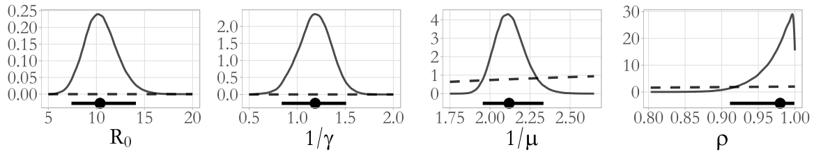
Figure 3.10: Posterior density estimates for R_0 = \beta N/\mu , the mean latent and infectious periods, 1/\gamma and 1/\mu , and the binomial sampling probability, \rho , from SIR and SEIR model parameters fit to the British boarding school data (solid lines). The posterior median and 95% Bayesian credible intervals are drawn below the density plots (solid lines with circles). The implied prior densities (dashed lines) for R_0 and the latent and infectious periods, and the prior density for the binomial sampling probability, are plotted over the posterior ranges.
