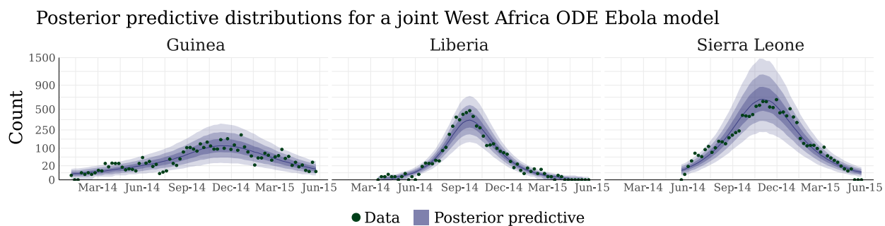
Figure 4.19: Partial and full posterior predictive distributions for a stratified SEIR ODE model for jointly modeling the Ebola outbreak in West Africa. Green points correspond to the observed incidence. The shaded bands, in order of lightest to darkest, correspond to pointwise posterior 95%, 80%, and 50% credible intervals, with the pointwise posterior median given by the corresponding colored solid line.
