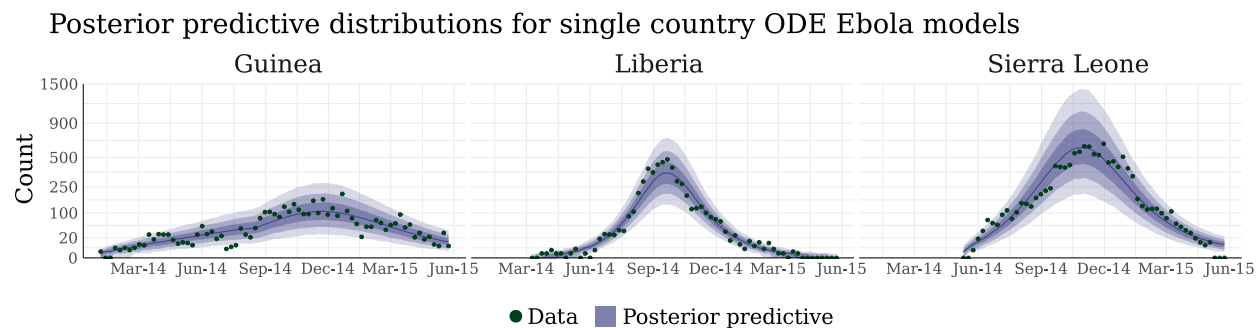
Figure 4.18: Partial and full posterior predictive distributions for country-specific SEIR ODE models for the West Africa Ebola outbreak. Green points correspond to the observed incidence. The shaded bands, in order of lightest to darkest, correspond to pointwise posterior 95%, 80%, and 50% credible intervals, with the pointwise posterior median given by the corresponding colored solid line.
