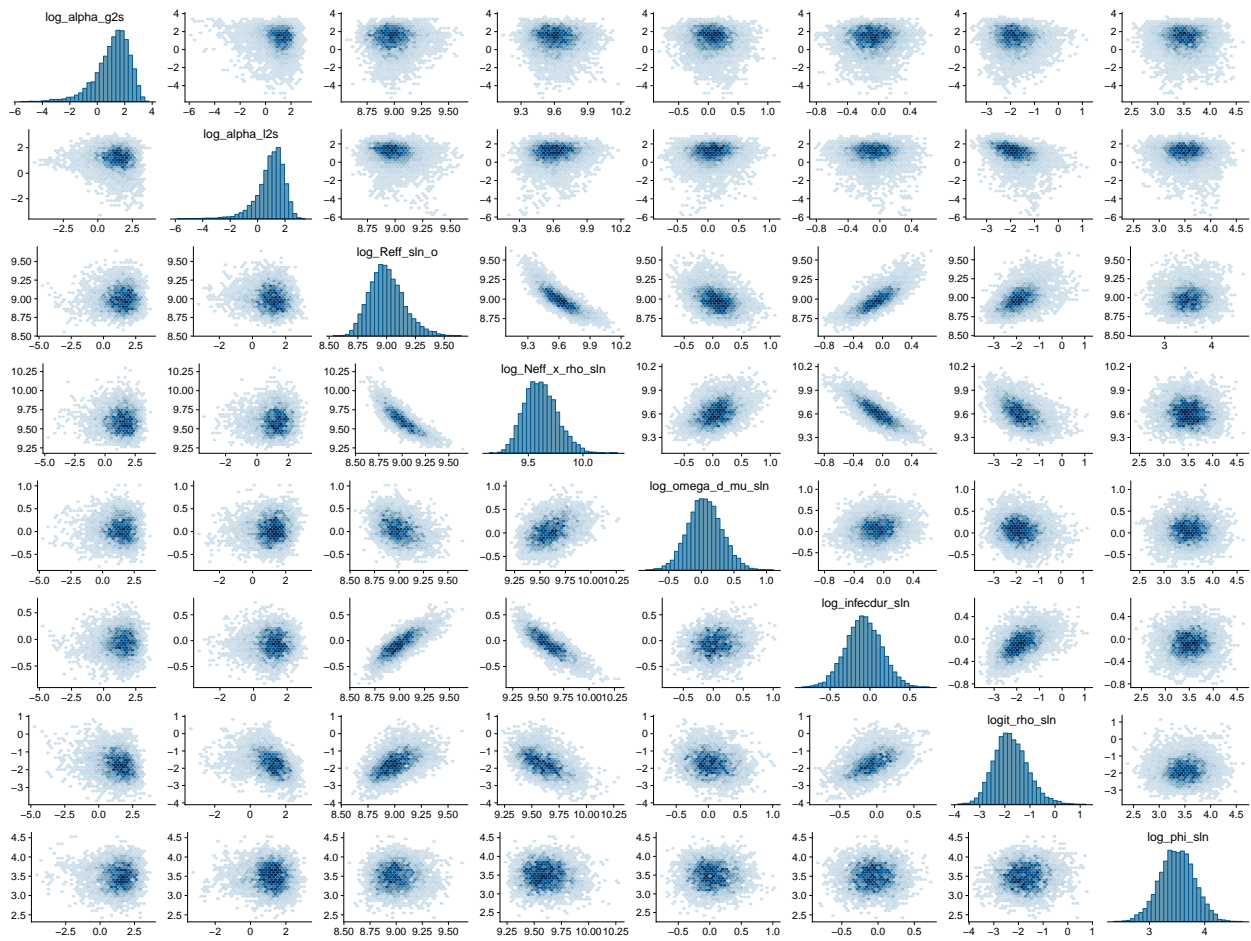
Figure B.9: Scatterplots of Sierra Leone-specific parameters in a stratified SEIR model for a simulated Ebola outbreak.
