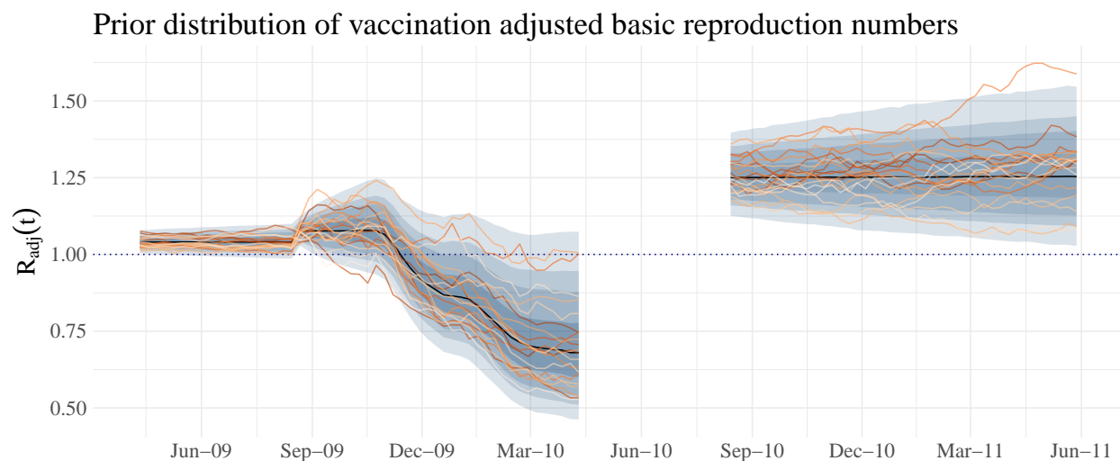
Figure C.6: Induced prior distribution of for vaccination adjusted basic reproduction numbers A(H1N1)pdm09 influenza in Finland. Shaded bands correspond to the central 50%, 80%, and 95% prior probability intervals.
