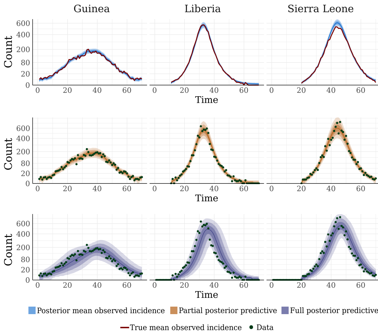
Figure 4.11: From top to bottom, the posterior mean observed incidence, partial posterior predictive, and full posterior predictive distributions. The solid red line is the incidence we would expect to observe if we knew the true incidence. Green points correspond to the observed incidence. The shaded bands, in order of lightest to darkest, correspond to pointwise posterior 95%, 80%, and 50% credible intervals, with the pointwise posterior median given by the corresponding colored solid line.
