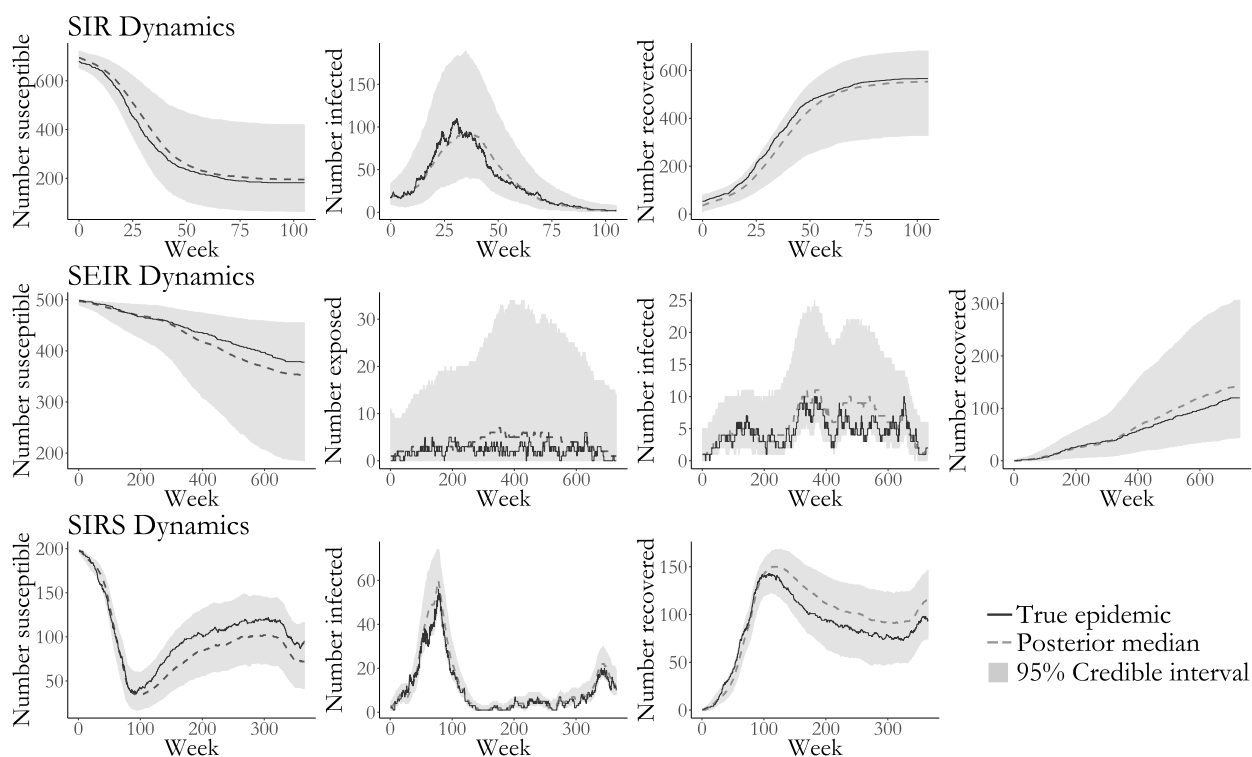
Figure A.11: Pointwise posterior medians (dashed lines) and pointwise 95% credible intervals for the numbers of individuals in each disease state for the SIR, SEIR, and SIRS models. True compartment counts are shown as solid lines. Estimates are based on a thinned sample, retaining the collection of disease histories at the end of every 250 th MCMC iteration.
