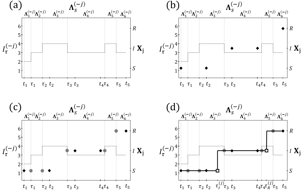
Figure 3.2: Procedure for constructing a subject–path proposal with SIR dynamics. (a) The dashed line depicts the number of infected individuals, excluding \mathbf{X}_j , the subject whose path is being sampled. The observation times, t_1, \dots, t_5 , and times at which other subjects change disease states, \tau_1, \dots, \tau_5 , are shown on the bottom axis. Rate matrices of the time–inhomogeneous CTMC (top axis) are constant within inter–event intervals (vertical lines). The state space of the subject–level process, \mathbf{X}_j , is shown on the right axis. (b) HMM step : Sample the state of \mathbf{X}_j at t_1, \dots, t_5 , conditional on the data and on the disease histories of other subjects. (c) Discrete time skeleton step : Sample the infection status at \tau_1, \dots, \tau_5 , conditional on the sequence of states sampled in the HMM step. (d) Event time step : Sample the infection and recovery times from endpoint–conditioned time–homogeneous CTMC distributions, conditional on the sequence of disease states sampled in the HMM and discrete time skeleton steps.
