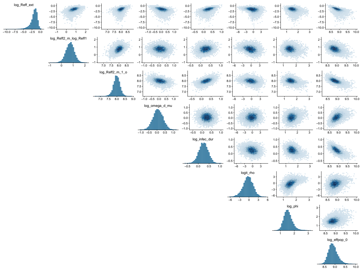
Figure B.12: Scatterplots of parameters for the SEIR LNA model fit to data from the Ebola outbreak in Guinea.
