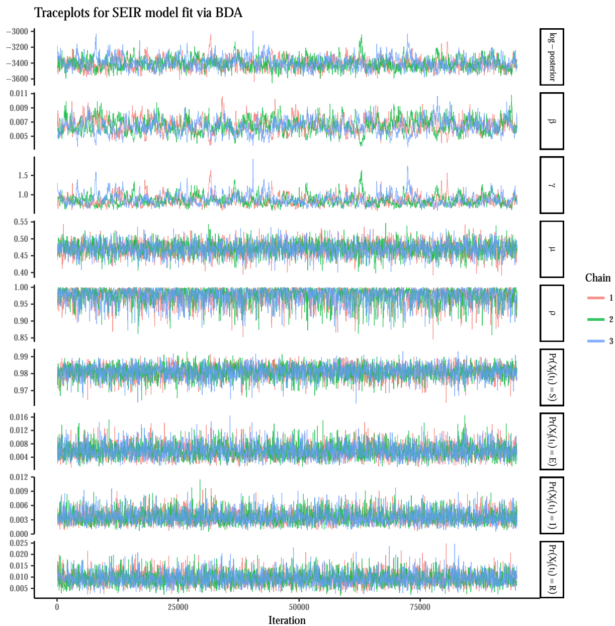
Figure A.21: Traceplots of the log-posterior and model parameters for the SEIR model fit under binomial emissions via BDA following an initial burn-in of 5,000 iterations. \beta denotes the per-contact infectivity rate, \mu is the recovery rate, \gamma is the rate at which immunity is lost, and \rho is the binomial sampling probability. Traceplots are thinned to display every 50 th iteration.
