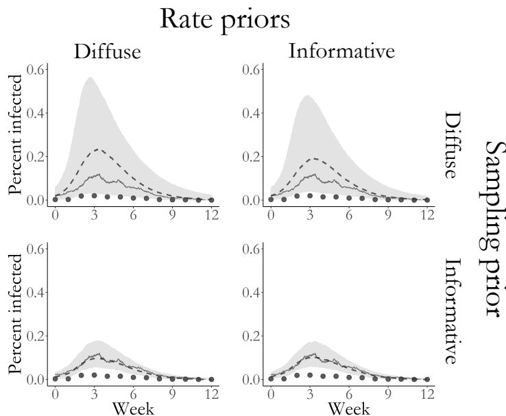
Figure 3.8: Estimated latent posterior distributions of disease prevalence in outbreaks simulated under four prior regimes for SIR model rate parameters and the binomial sampling probability. Depicted are the true unobserved prevalence (solid line), observed data (dots), pointwise posterior median prevalence (dashed line), and pointwise 95% credible intervals (shaded region). Latent posterior estimates are based on a thinned sample, with every 250 th sample retained.
