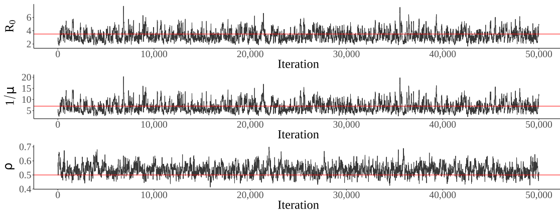
Figure 4.2: Posterior traceplots of parameters of interest sampled by a single MCMC chain of an SIR model fit to Poisson distributed incidence data. MCMC targeted the non-centered parameterization of the posterior 4.20, alternately updating \mathbf{Z}|\boldsymbol{\theta}, \mathbf{Y} via elliptical slice sampling, and \boldsymbol{\theta}|\mathbf{Z}, \mathbf{Y} via a multivariate random walk Metropolis algorithm. R_0 = \beta N/\mu is the basic reproductive number, 1/\mu is the mean infectious period duration, and \rho is the mean case detection rate. The true values of R_0 , 1/\mu , and \rho were 3.5, 7, and 0.5, respectively.
