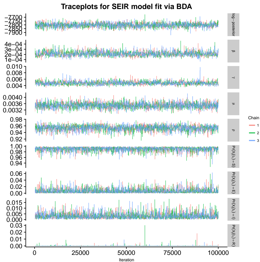
Figure A.14: Traceplots of the log-posterior and model parameters for the SEIR model fit using BDA following an initial burn-in of 100 iterations. \beta denotes the per-contact infectivity rate, \gamma is the rate at which an exposed individual becomes infectious, \mu is the recovery rate, \rho is the binomial sampling probability. Traceplots are thinned to display every 50 th iteration.
