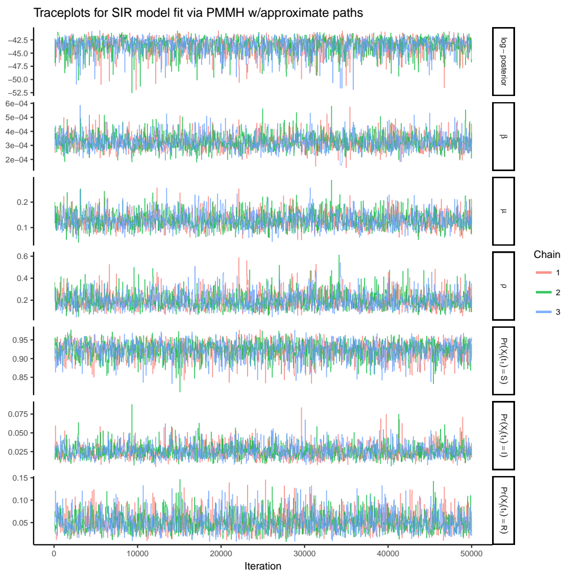
Figure A.2: Traceplots of the log-posterior and model parameters for the SIR model fit using PMMH with 100 particles and a time step of 8 hours, following a tuning run of 5,000 iterations used to estimate the covariance matrix for the RWMH and an initial burn-in of 100 iterations. \beta denotes the per-contact infectivity rate, \mu is the recovery rate, \rho is the binomial sampling probability. Traceplots are thinned to display every 50 th iteration.
