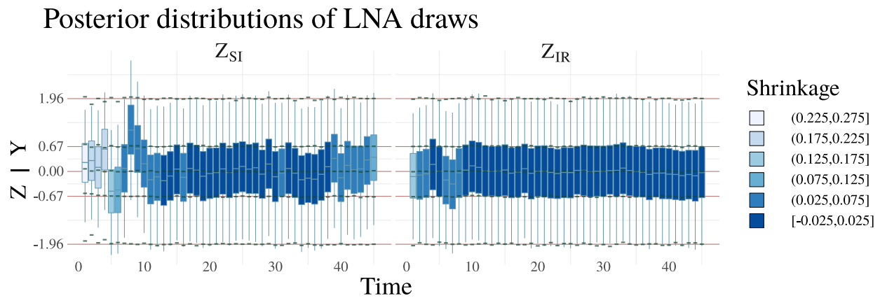
Figure 4.7: Posterior distributions of the LNA draws for infections and recoveries in an SIR model (blue boxplots). The lower and upper whisker tips correspond to the 2.5 th and 97.5 th posterior quantiles, the lower and upper hinges to the 25 th and 75 th quantiles, and the middle hash mark to the posterior median. The solid red lines are the theoretical quantiles of the posterior predictive distribution (or equivalently, the prior distribution) of the LNA draws, drawn at the quantiles of a standard normal distribution corresponding to the boxplot quantiles. The green ticks are the estimated quantiles of the posterior predictive distributions of the LNA draws, accounting for boundary conditions on the state space of the latent process and obtained by simulating LNA paths from the posterior predictive distribution. The posterior distributions of LNA draws are shaded according to the level of posterior shrinkage, computed as one minus the ratio of standard deviations of LNA draws in the posterior and prior.
