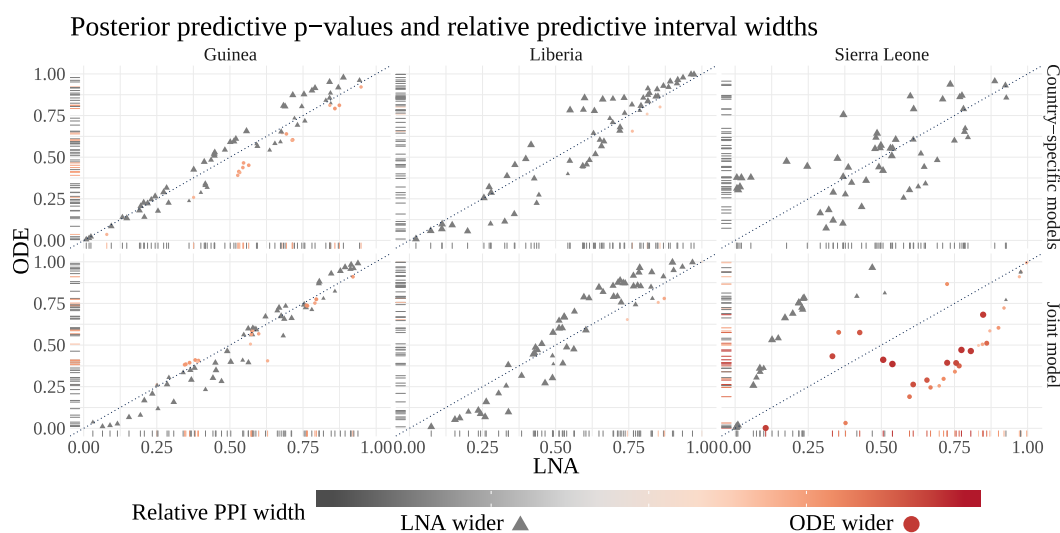
Figure 4.21: Comparison of SEIR models for Ebola fit using the LNA and ODE using posterior predictive p-values (PPPs) and relative posterior predictive interval (PPI) widths. The top row compares LNA and ODE country-specific models, while the bottom row compares LNA and ODE joint. Each point corresponds to the observed incidence in a given week. The X–Y coordinates give the PPPs of the data under LNA and ODE, respectively. The size and color of each point corresponds to the relative PPI width, computed as (\hat{\sigma}_{post,\ell}^{ode} - \hat{\sigma}_{post,\ell}^{lna})/\hat{\sigma}_{post,\ell}^{lna} , and the sign of the relative width is further emphasized by the shape of the point. Dots indicate that PPIs under the ODE are wider, while triangles corresponds to observations for which the PPI produced by the LNA is wider.
