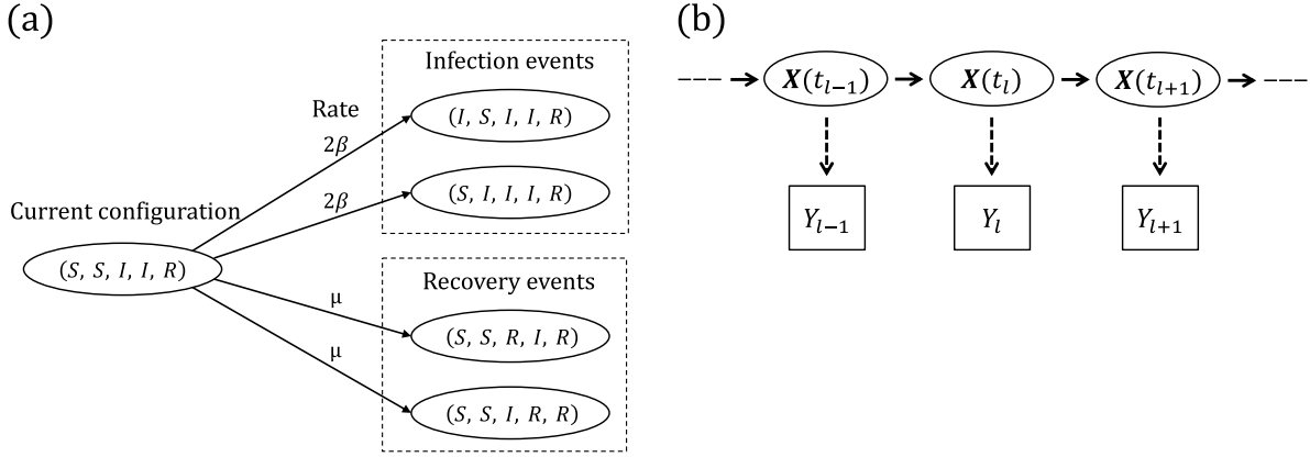
Figure 3.1: (a) SIR dynamics in a population of five subjects. The number of infecteds can increase from two to three via an infection of the first or second subject, reaching each of those configurations at rate 2\beta . The number of recovered individuals can increase from one to two via a recovery of the third or fourth subject, reaching each of those configurations at rate \mu . (b) Hidden Markov model for the joint distribution of the latent epidemic process and the data. The observations, \mathbf{Y}_\ell , \ell = 1, \dots, L , are conditionally independent given \mathbf{X}(t) , and \mathbf{Y}_\ell | I_{t_\ell}, \rho \sim \text{Binomial}(I_{t_\ell}, \rho) .
