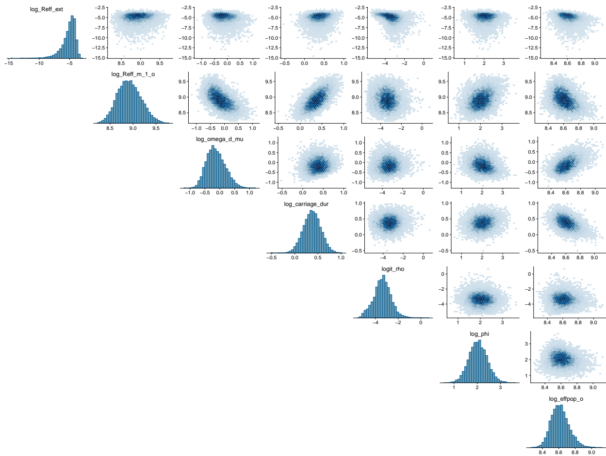
Figure B.22: Scatterplots of parameters for the SEIR ODE model fit to data from the Ebola outbreak in Liberia.
