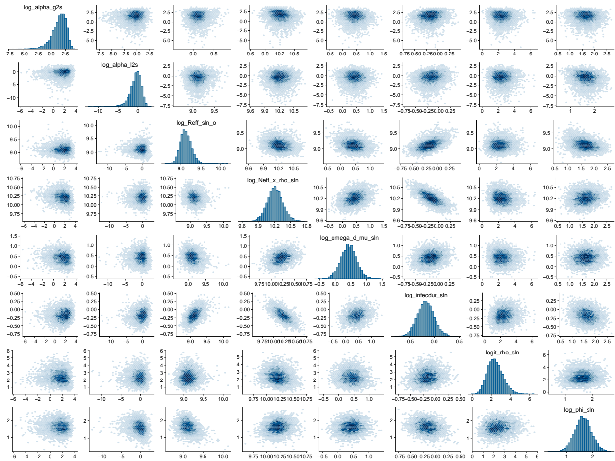
Figure B.36: Scatterplots of Sierra Leone-specific parameters in a stratified SEIR ODE model fit to data from the West Africa Ebola outbreak.
