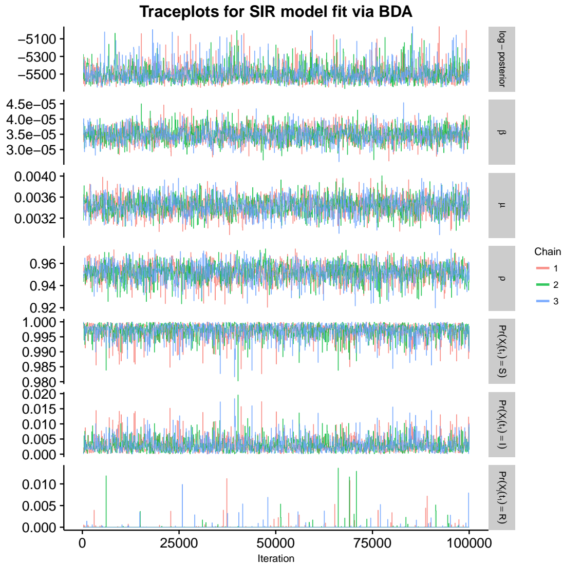
Figure A.12: Traceplots of the log-posterior and model parameters for the SIR model fit using BDA following an initial burn-in of 100 iterations. \beta denotes the per-contact infectivity rate, \mu is the recovery rate, \rho is the binomial sampling probability. Traceplots are thinned to display every 50 th iteration.
