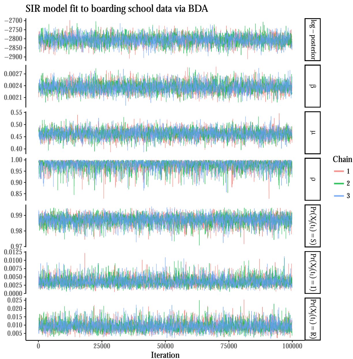
Figure A.20: Traceplots of the log-posterior and model parameters for the SIR model fit under binomial emissions using BDA following an initial burn-in of 100 iterations. \beta denotes the per-contact infectivity rate, \mu is the recovery rate, and \rho is the binomial sampling probability. Traceplots are thinned to display every 50 th iteration.
