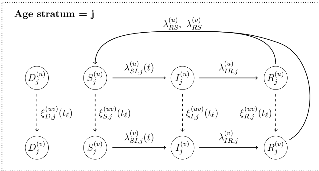
Figure 5.5: Diagram of state transitions for an age–vaccination stratified SIRS model for influenza in Finland. Both age strata, 0–19 and 20+, have the same compartmental structure. Nodes in circles denote model compartments, which are subscripted with age stratum and superscripted with vaccination status. Solid lines indicate stochastic transitions that occur continuously in time. Rates of disease state transitions, denoted by \lambda , are subscripted with the states from which, and to which, individuals flow and by the age stratum. Superscripts for transition rates indicate vaccination status. Dashed lines represent deterministic forcings from unvaccinated to vaccinated compartments that occur at discrete times. The mass of the forcing at time t , denoted \xi(t) , is subscripted by the compartment and age stratum, and superscripted by the direction of the forcing (unvaccinated to vaccinated). Individuals in the detached compartments of age stratum j , denoted D_j^{(u)} and D_j^{(v)} , are detached from the transmission process but may still be vaccinated.
