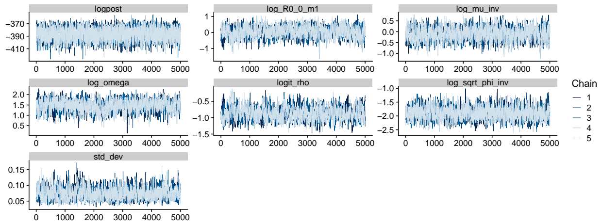
Figure C.1: Posterior traceplots for SIRS model parameters with time-varying force of infection.
