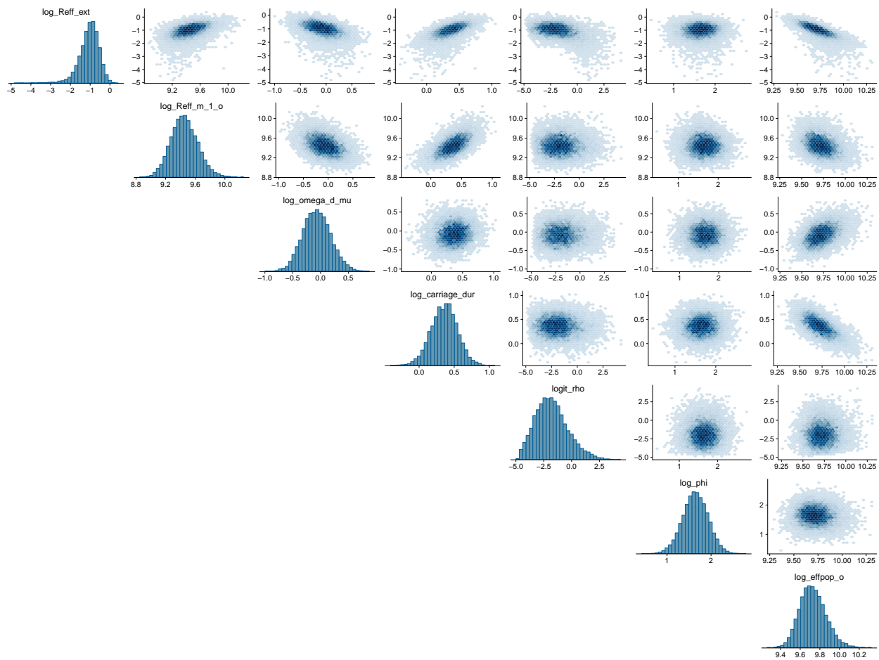
Figure B.24: Scatterplots of parameters for the SEIR ODE model fit to data from the Ebola outbreak in Sierra Leone.
