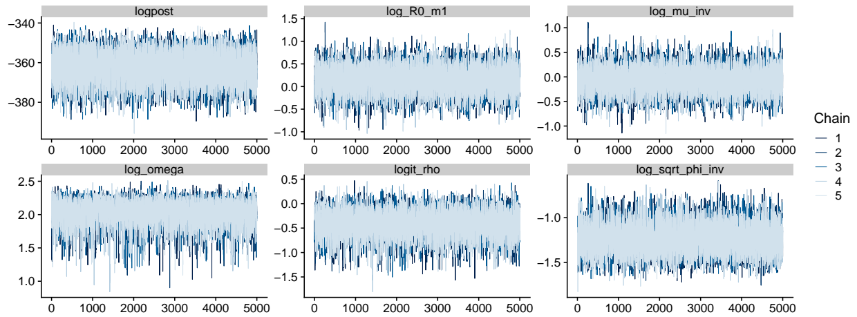
Figure C.3: Posterior traceplots for SIRS model parameters with time-homogeneous force of infection.
