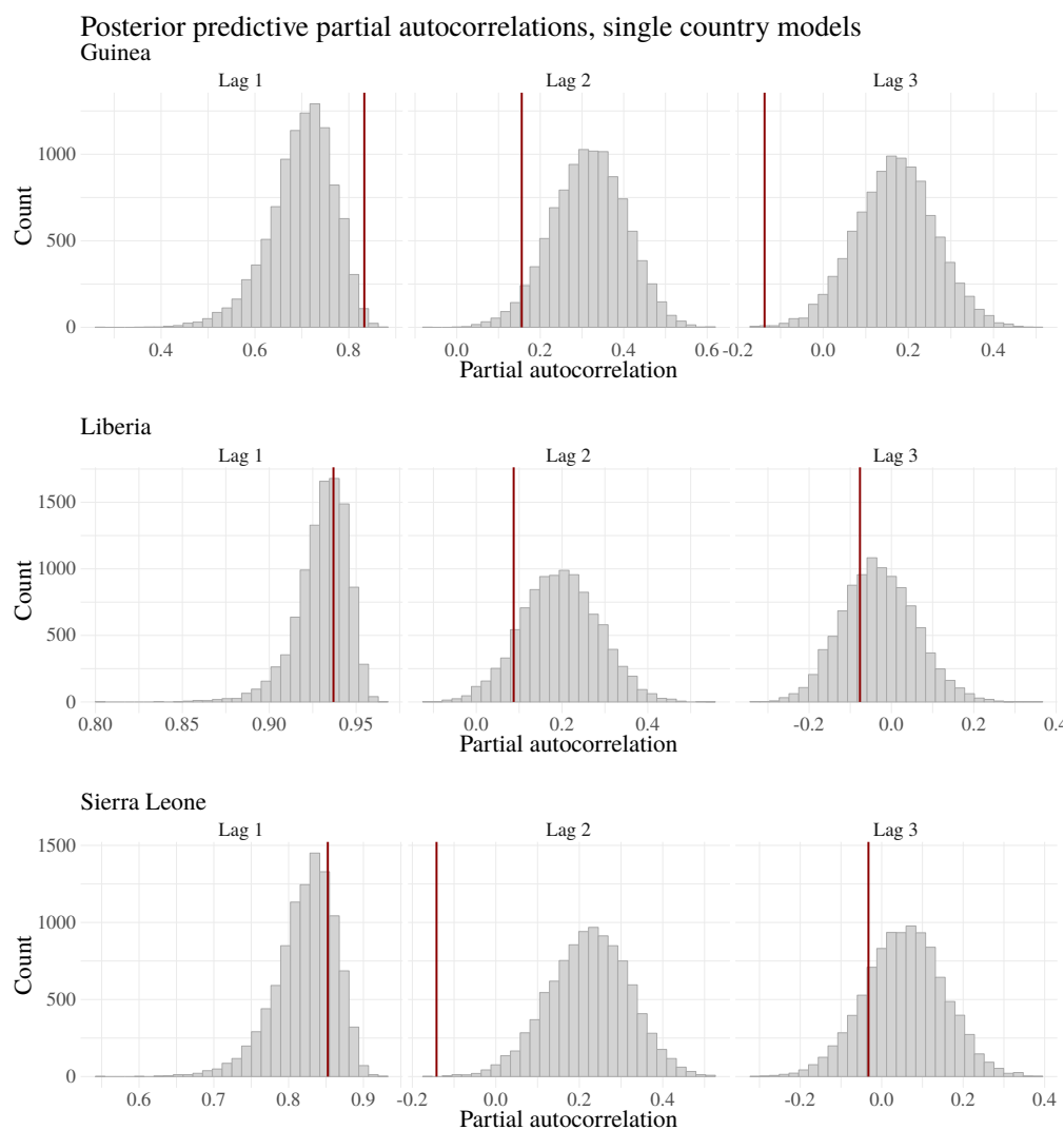
Figure B.25: Distributions of partial autocorrelations at lags 1, 2, and 3 for datasets generated under the full and partial posterior predictive distributions for the main country-specific SEIR ODE models fit to data from the West Africa Ebola outbreak. Vertical red lines are the partial autocorrelations for the observed incidence data at the respective lags.
