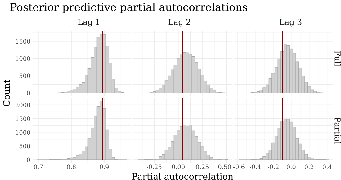
Figure 4.8: Distributions of partial autocorrelations at lags 1, 2, and 3 for datasets generated under the full and partial posterior predictive distributions. Vertical red lines are the partial autocorrelations for the observed incidence data at the respective lags.
