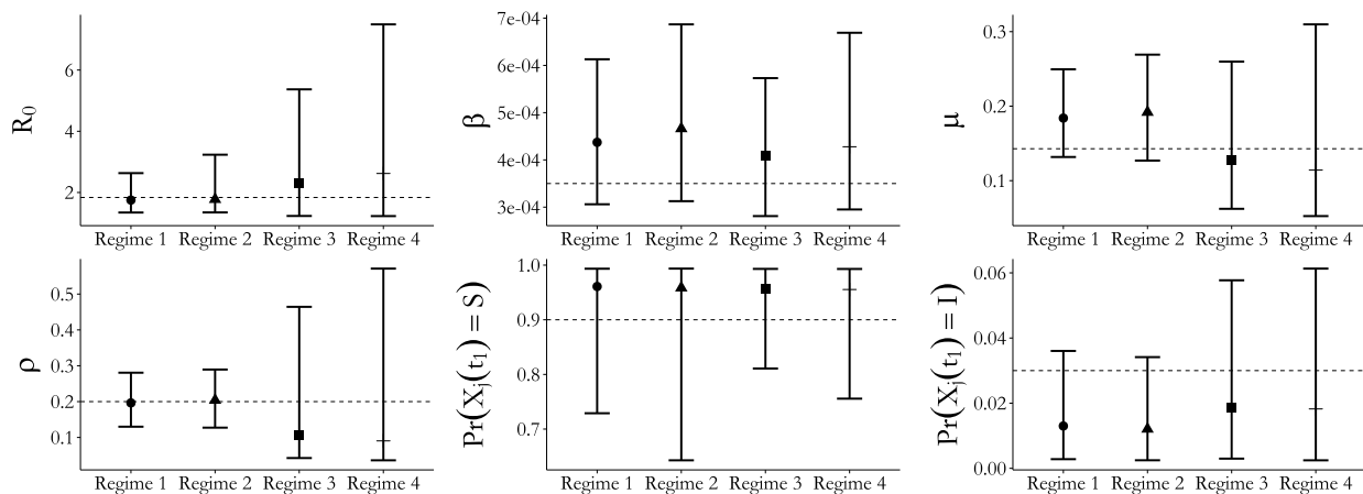
Figure 3.7: Posterior median estimates and 95% credible intervals for all SIR model parameters under four different prior regimes (Table A.14). Regimes 1 and 3 set informative priors for the per-contact infectivity and recovery rates. Regimes 1 and 2 set informative priors for the binomial sampling probability. The same mildly informative prior for the initial state probabilities was used in all four regimes.
