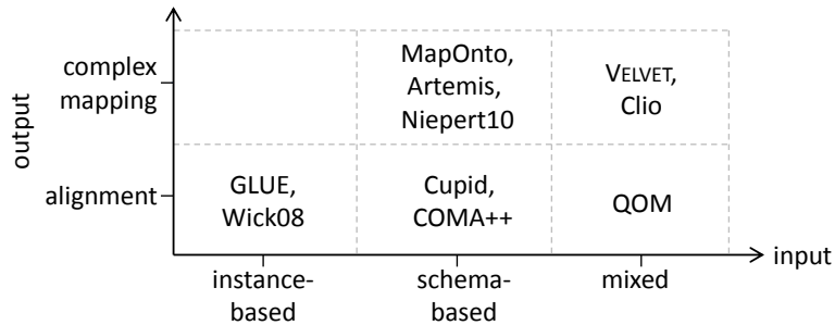
Figure 6.1: Classification of selected ontology matching systems, based on Euzenat and Shvaiko[40].
