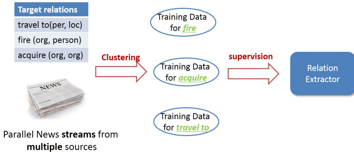
Figure 1.2: The basic idea of exploiting the temporal correspondence for event extraction: the system aims to extract a set of target relations and has a large corpus of parallel news streams from multiple sources as its unlabeled corpus; the system first clusters the sentences from parallel news according to the target relations and then uses them as the training data; the system then learns the relation extractor from the generated training sentences.
