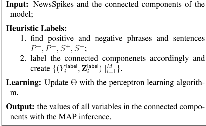
Figure 4.4: Learning from Heuristic Labels
