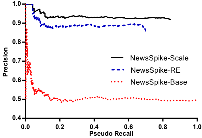
Figure 5.3: Precision pseudo-recall curves for all 150 event relations. NEWSPIKE-SCALE has AUC 0.79, 25% higher than NEWSPIKE-RE (0.63) and 54% higher than NEWSPIKE-BASE (0.51)
