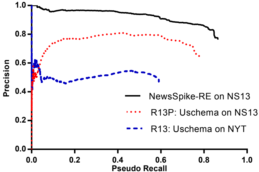
Figure 4.5: Precision pseudo-recall curves for all 30 event relations. NEWSPIKE-RE has AUC 0.80, more than doubling R13 (0.30) and 35% higher than R13P (0.59) for all event relations.
