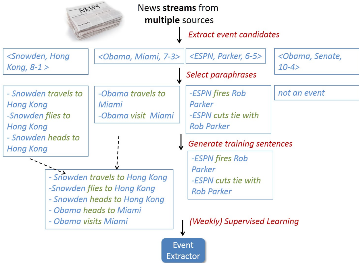
Figure 1.3: A running example to show the general framework of proposed system: to exploit the parallel news streams for relation extraction, the system could be composed of three stages. First, extracting event candidates from the parallel news streams; second, identifying parallel sentences describing the events; third, clustering sentences from different NewsSpikes and generating the training sentences; finally, learning event extractors for the target relations with supervised or distant supervised algorithms.
