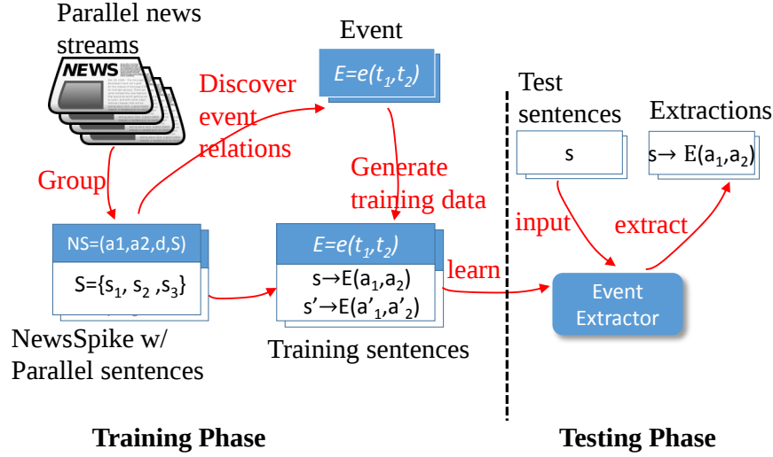
Figure 4.1: During its training phase, NEWSPIKE-RE first groups parallel sentences as NewsSpikes . Next, the system automatically discovers a set of event relations. Then, a probabilistic graphical model clusters sentences from the NewsSpike as training data for each discovered relation, which is used to learn sentential event extractors. During the testing phase, the extractor takes test sentences as input and predicts event extractions.
