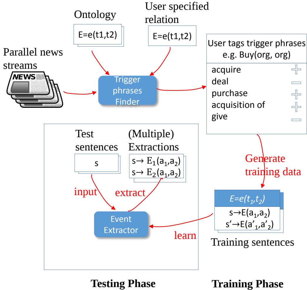
Figure 5.1: System overview of NEWSPIKE-SCALE: the system allows users to specify new event relations and add them to the target ontology. During the training phase, the system first finds a set of trigger phrases for every relation; it presents the trigger phrases to users with their context; NEWSPIKE-SCALE then employs the graphical model of NEWSPIKE-RE to generate training sentences, which are used to learn sentential event extractors. During the testing phase, the extractor takes a test sentence as input and predicts event extractions.
