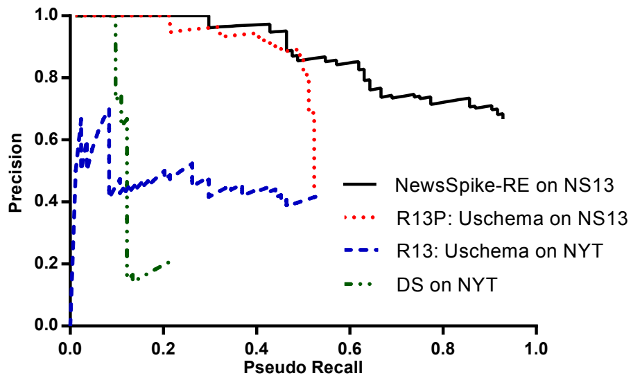
Figure 4.6: Precision pseudo-recall curves for buy(org, org) , this figure includes the distant supervision algorithm MIML learned from matching the Freebase relation to The New York Times. NEWS SPIKE-RE has AUC 0.80, more than doubling R13 (0.30) and 35% higher than R13P (0.59) for buy(org, org) event relations.
