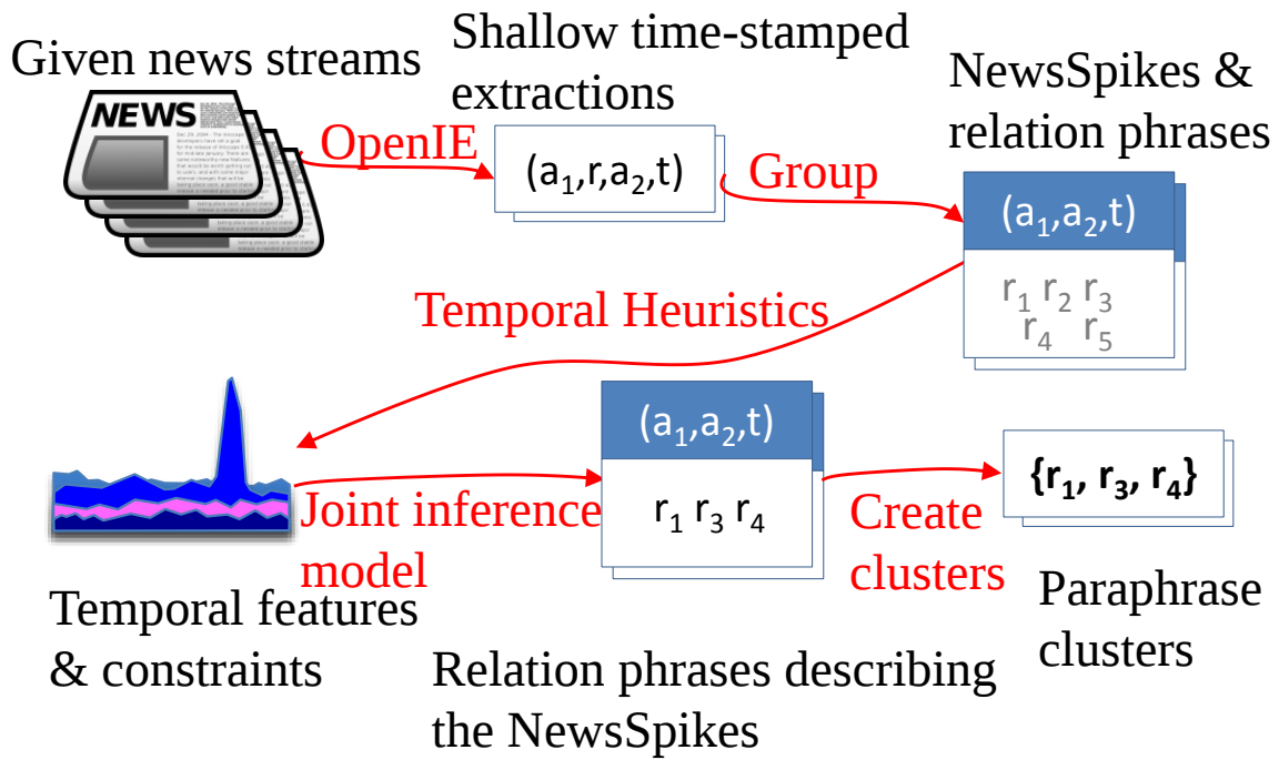
Figure 3.1: NEWSPIKE-PARA first applies open information extraction to articles in the news streams, obtaining shallow extractions with time-stamps. Next, an NewsSpike (NewsSpike) is obtained after grouping daily extractions by argument pairs. Temporal features and constraints are developed based on our temporal correspondence heuristics and encoded into a joint inference model. The model finally creates the paraphrase clusters by predicting the relation phrases that describe the NewsSpike.
