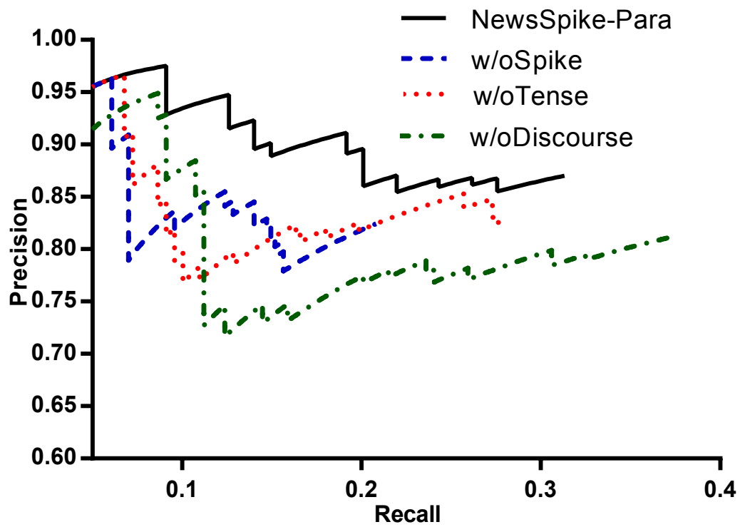
Figure 3.4: Precision recall curves on hard, diverse cases for NEWSPIKE-PARA, w/oSpike, w/oTense and w/oDiscourse.
