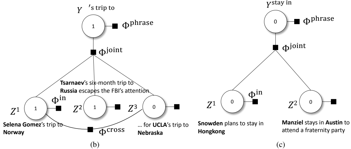
Figure 4.3: (a) The connected components depicted as plate model, where each Y is a Boolean variable for a relation phrase and each Z is a Boolean variable for a training sentence for with that phrase; (b) and (c) are example connected components for the event phrases 's trip to and stay in respectively. The goal of the model is to set Y = 1 for good paraphrases of a relation and to set Z = 1 for good training sentences.
