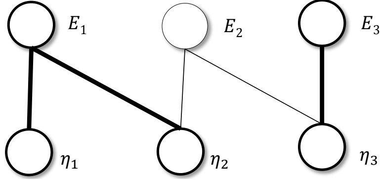
Figure 4.2: A simple example of the edge-cover algorithm with K=2 , where E_i are event relations and \eta_j are NewsSpikes. The optimal solution selects E_1 with edges to \eta_1 and \eta_2 , and E_3 with edge to \eta_3 . These two event relations cover all the NewsSpikes.
