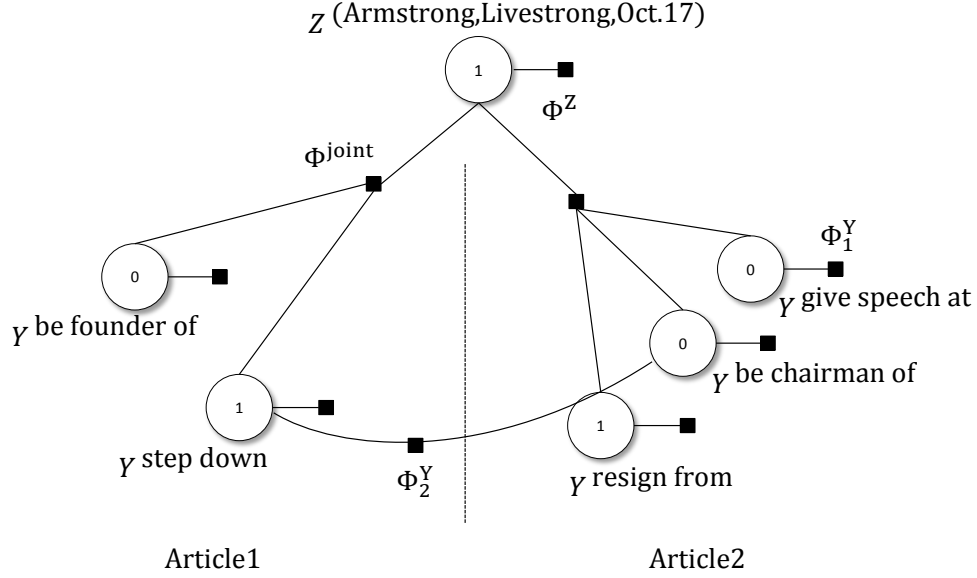
Figure 3.2: an example model for NewsSpike (Armstrong, Livestrong, Oct 17). Y and Z are binary random variables. \Phi^Y , \Phi^Z and \Phi^{\text{joint}} are factors. be founder of and step down come from article 1 while give speech at, be chairman of and resign from come from article 2.
