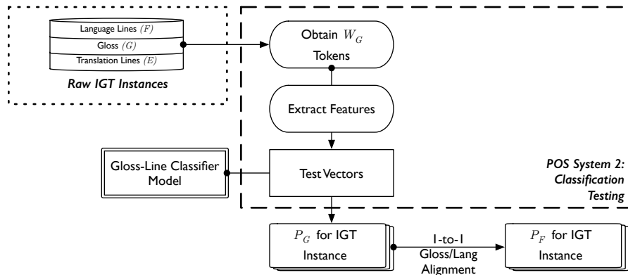
Figure 6.5: Flowchart illustrating the testing step of the classification-based tagging approach.
