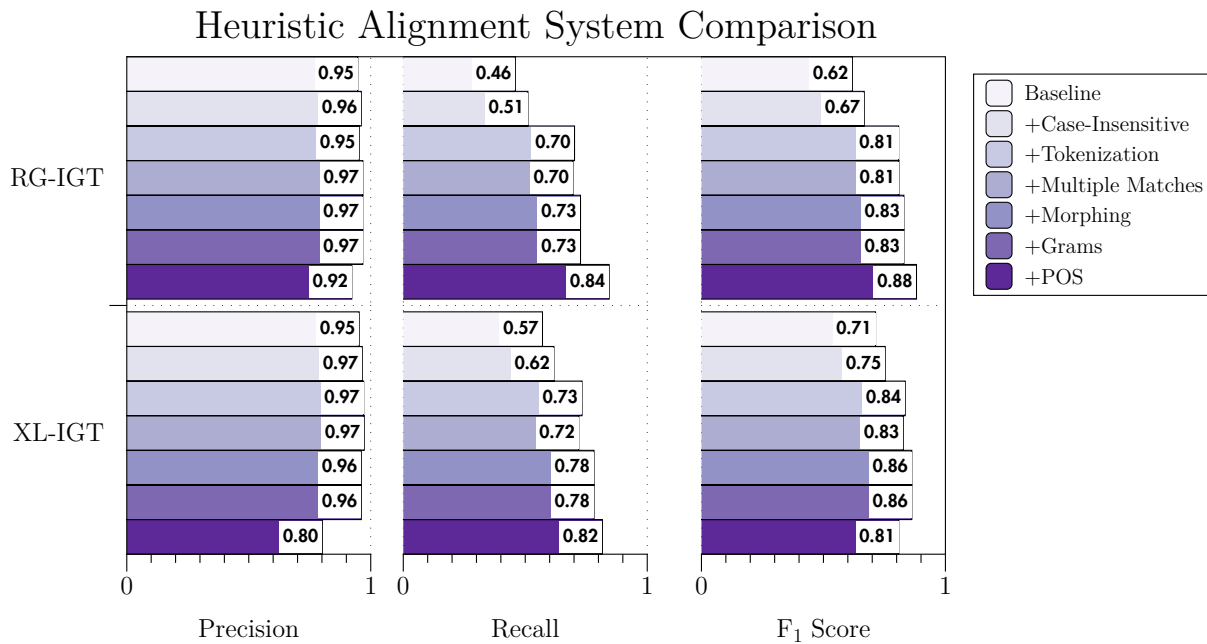
Figure 5.1: Graph showing the performance of the heuristic matching approach between gloss and translation as heuristics are added going from top to bottom.
