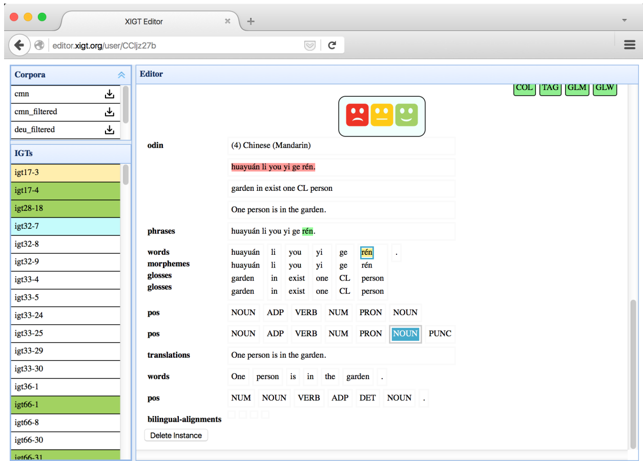
Figure 8.8: INTENT-enriched information is automatically generated by the editor interface for inspection by the annotator. Future releases will include the ability for annotators to correct the enriched data, as well as view other information such as word alignment.
