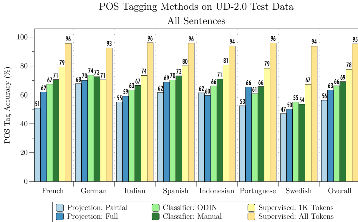
Figure 6.10: Bar graph showing the POS tag accuracies for the POS tagging on monolingual UD-2.0 test data.
