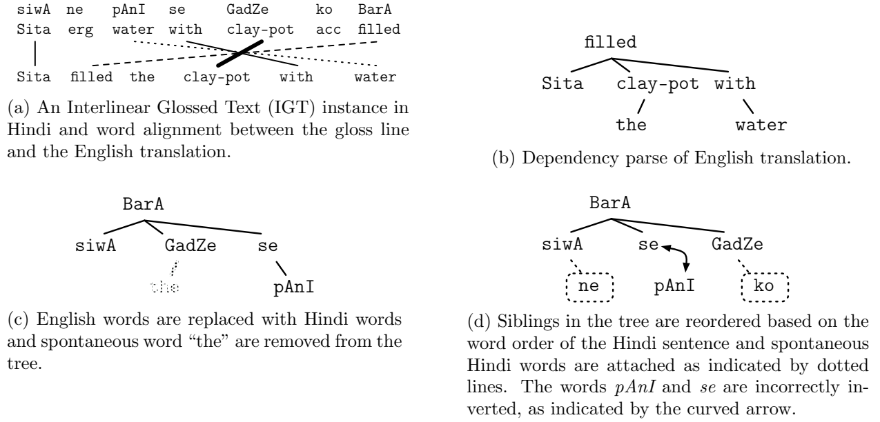
Figure 7.16: An example of projecting a dependency tree from English to Hindi.
