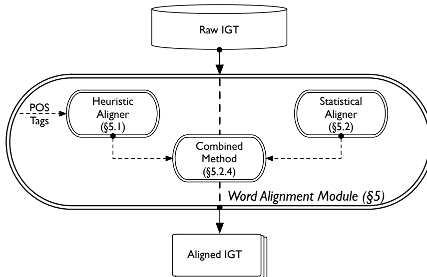
Figure 3.2: Overview of the word alignment module and its different settings.
