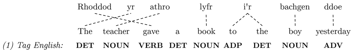
Figure 2.2: Sentence from Fig. 2.1, with English Sentence POS Tagged.
