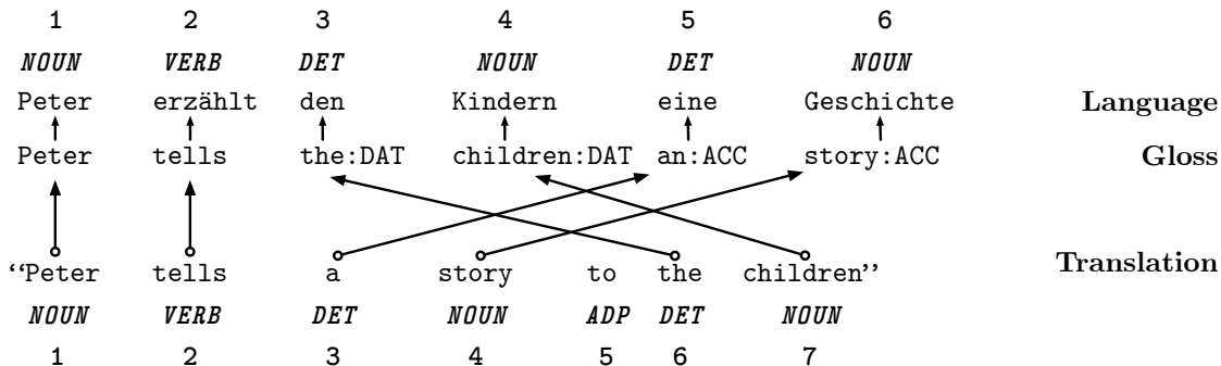
Instance 3.4: IGT instance demonstrating how POS tags can be projected from the translation line to the language line by way of the the gloss line.
