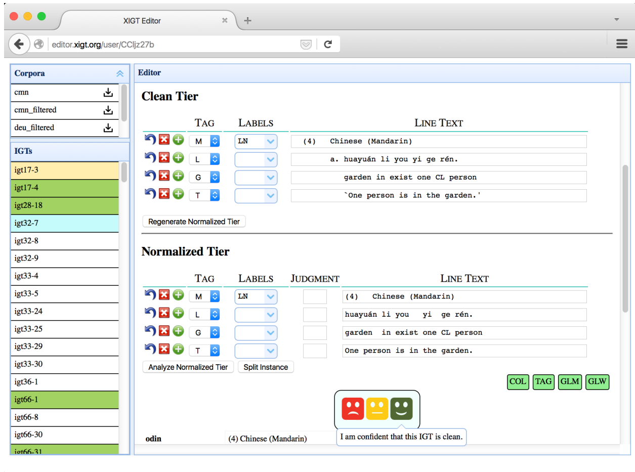
Figure 8.7: Overview of the XIGT editor interface for cleaning IGT instances. The editor allows annotators to clean corruption from XIGT instances, normalize the data so that it is ready for the automated methods of INTENT and other systems, and provide a cleanliness rating and other comments that are saved in the IGT instance metadata.
