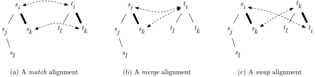
Figure 7.8: Definition of a match , merge , and swap edges in a tree pair.
