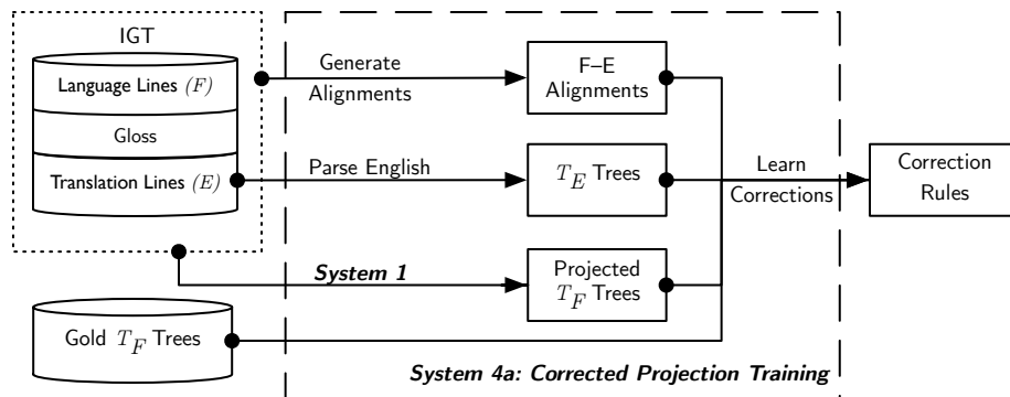
(a) Flowchart illustrating the training phase of learning the correction patterns.
