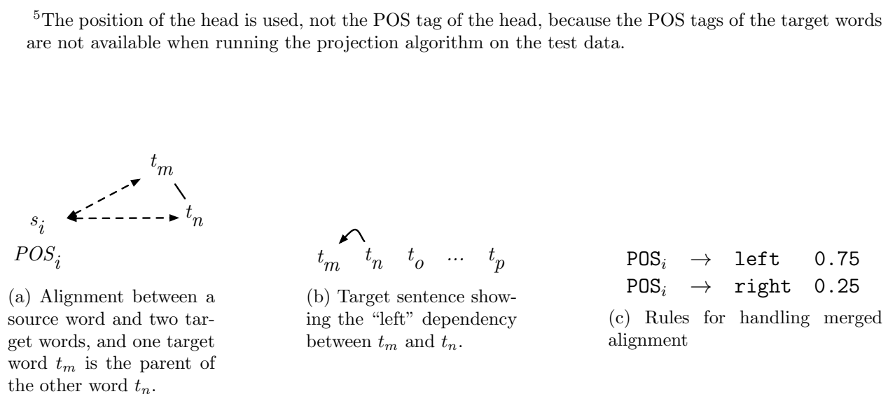
Figure 7.15: Example of merge alignment and derived rules.
