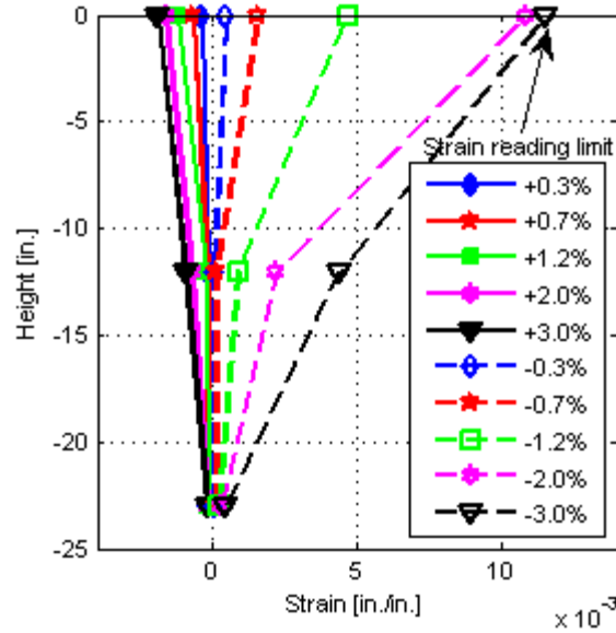
d). DS-2 - South reinforcing bar of column.
