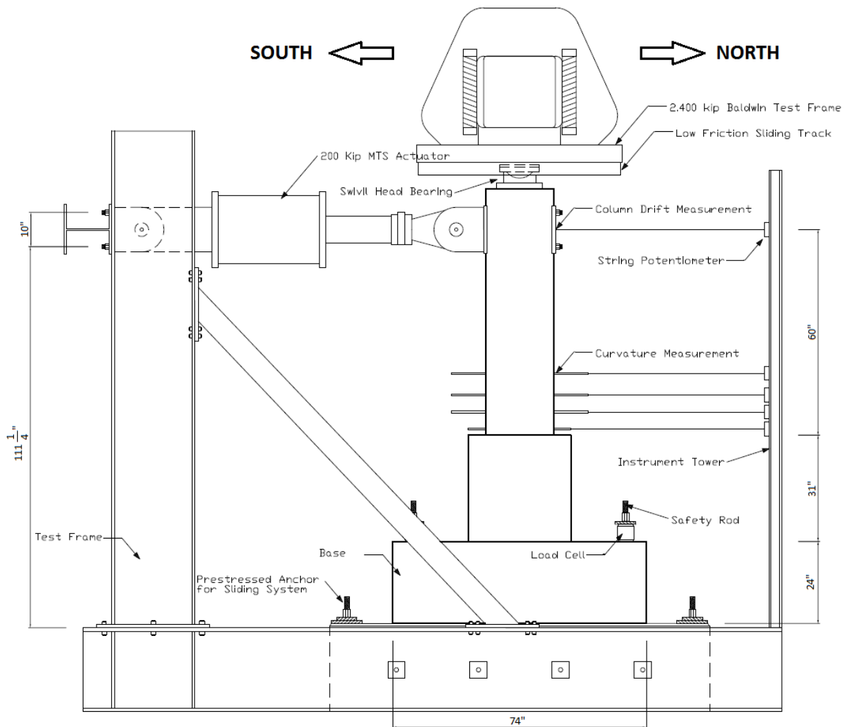
Figure 3-1. Test setup
