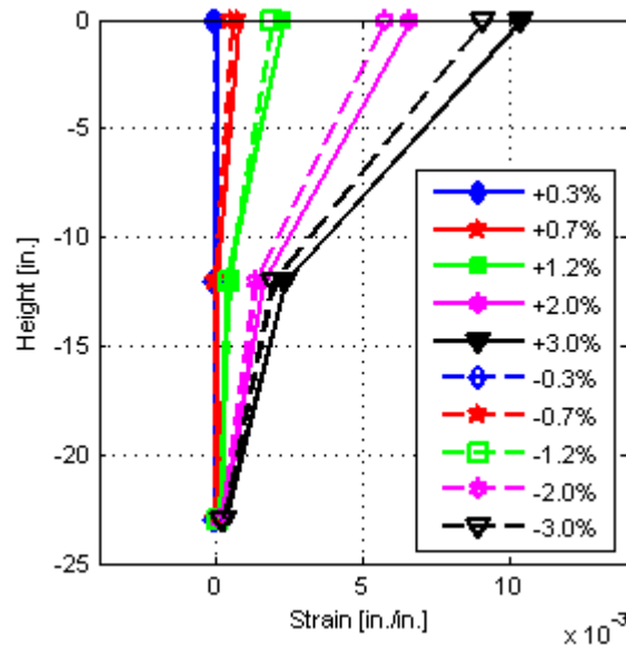
f). DS-2 - East reinforcing bar of column.
