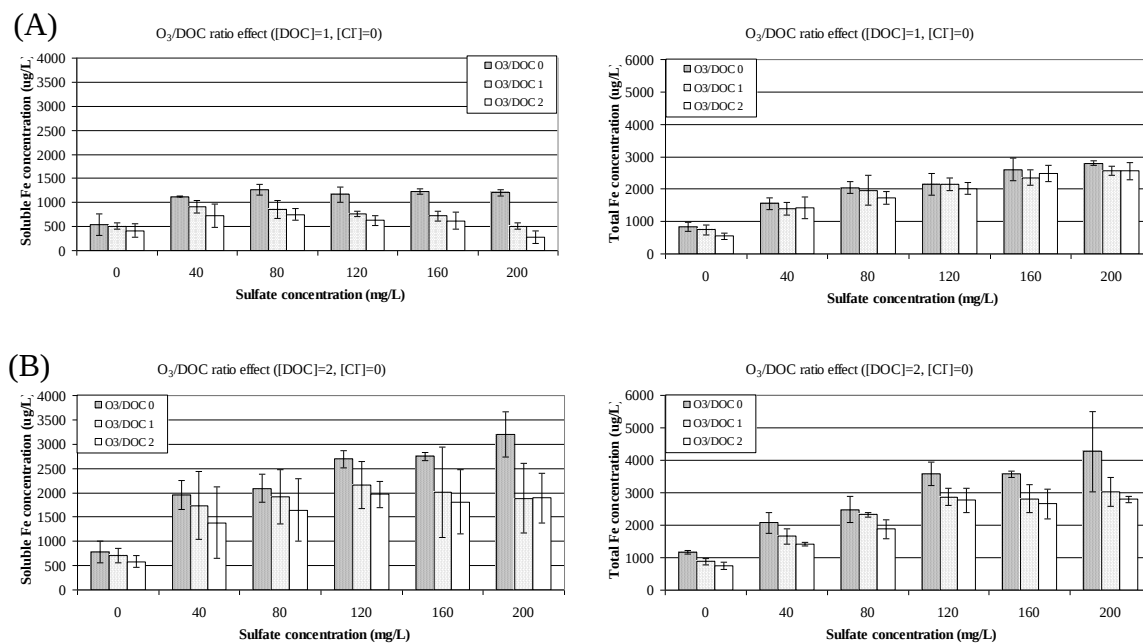
Figure 7.6 Effects of sulfate and NOM altered using varying O 3 /DOC ratios on average soluble and total iron concentrations released from iron coupons during exposure week 7 to 9 (A) DOC 1 mg/L and (B) DOC 2 mg/L. The error bar corresponds to \pm 1 standard deviation.
