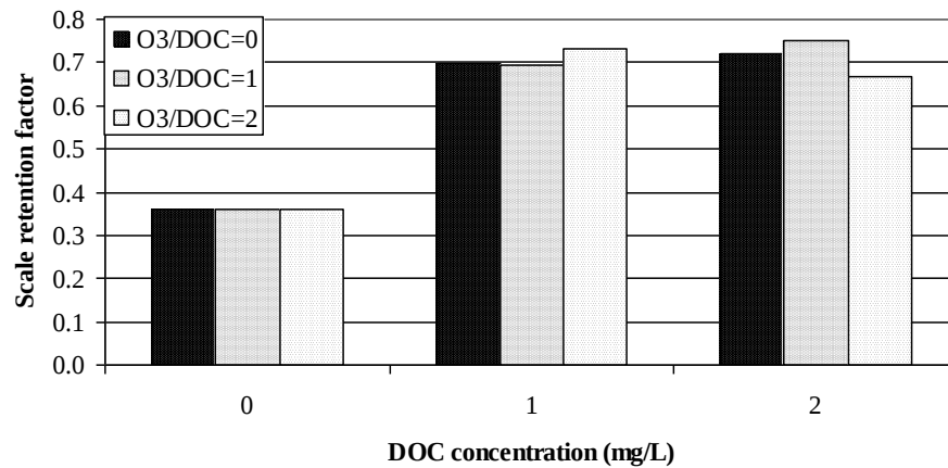
Figure 7.7 Impacts of NOM concentrations and its alteration by oxidation using varying O 3 /DOC ratios on (A) apparent corrosion rates and (B) scale retention factors determined based on weight loss measurements for iron coupons exposed to the baseline water chemistry.
