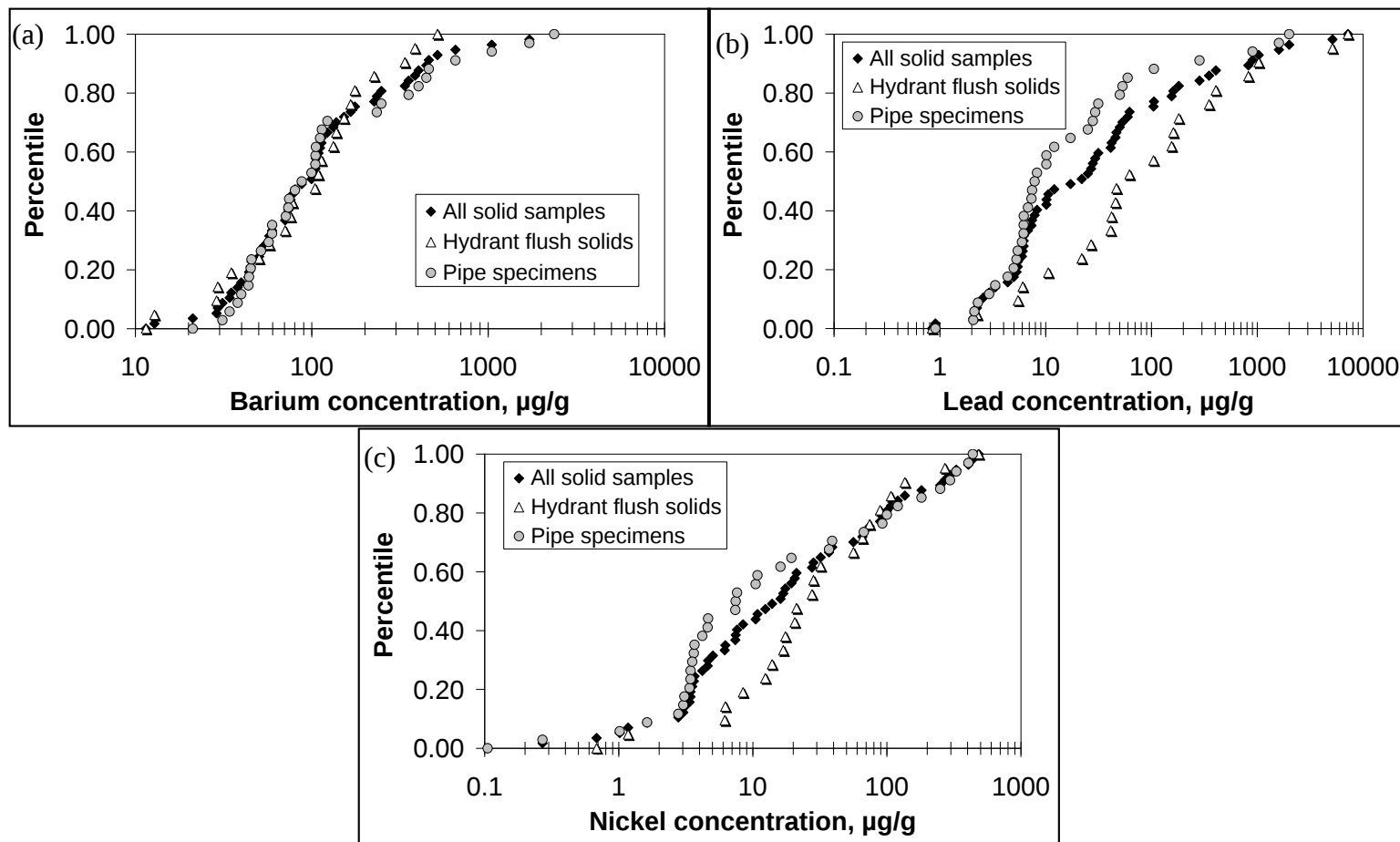
Figure 4.5 Cumulative occurrence profiles for (a) barium, (b) lead, and (c) nickel in deposit samples.
