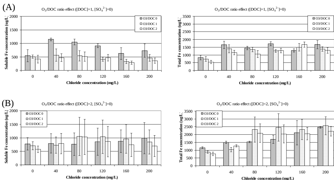
Figure 7.5 Effects of chloride and NOM altered using varying O 3 /DOC ratios on average soluble and total iron concentrations released from iron coupons during exposure week 7 to 9 (A) DOC 1 mg/L and (B) DOC 2 mg/L. The error bar corresponds to ±1 standard deviation.
