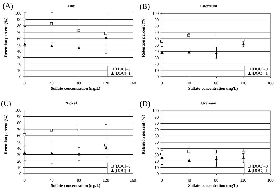
Figure 6.16 Impacts of sulfate and NOM on the retention by corrosion scales of (A) zinc; (B) cadmium; (C) nickel; and (D) uranium. Initial concentrations of the heavy metals are 5 \mu\text{g/L} in all cases.
