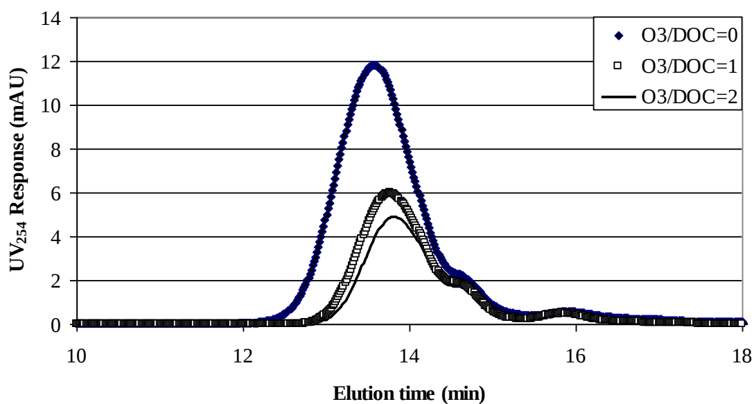
Figure 7.1 High performance size exclusion chromatography (HPSEC) chromatograms of Suwannee River NOM at three O_3/DOC ratios.
