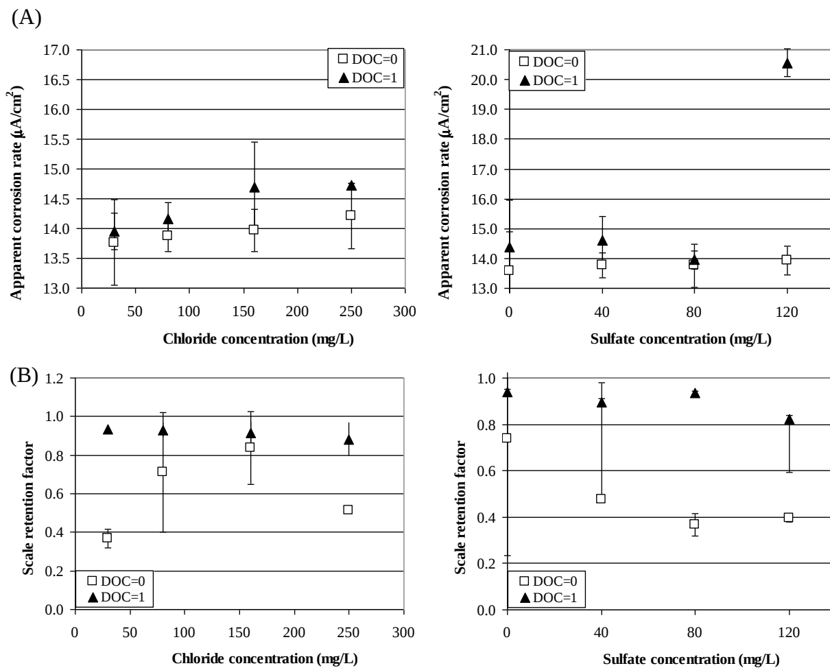
Figure 6.12 Impacts of chloride/sulfate and NOM concentrations on (A) apparent corrosion rates and (B) scale retention factors based on weight loss measurements for iron coupons.
