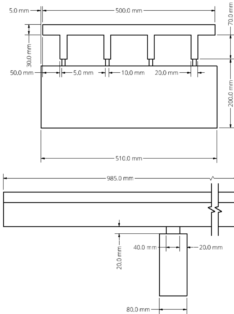
Figure 3.3: Dimensions of the model-scale bridge structure.
