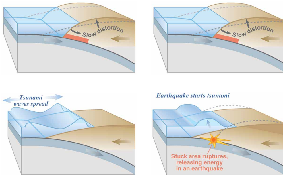
Figure 1.1: Schematic of the formation of a tsunami in a subduction zone arranged in clockwise direction. (Credits: USGS [3])
