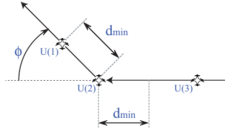
Fig. 6 Increased spacing needed ( d_{min} in Eq. 26) for heading change \phi .
