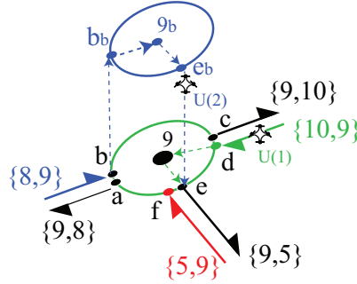
Fig. 7 Potential conflict at e when UAVs U(1) and U(2) merge into edge \{9,5\} .
