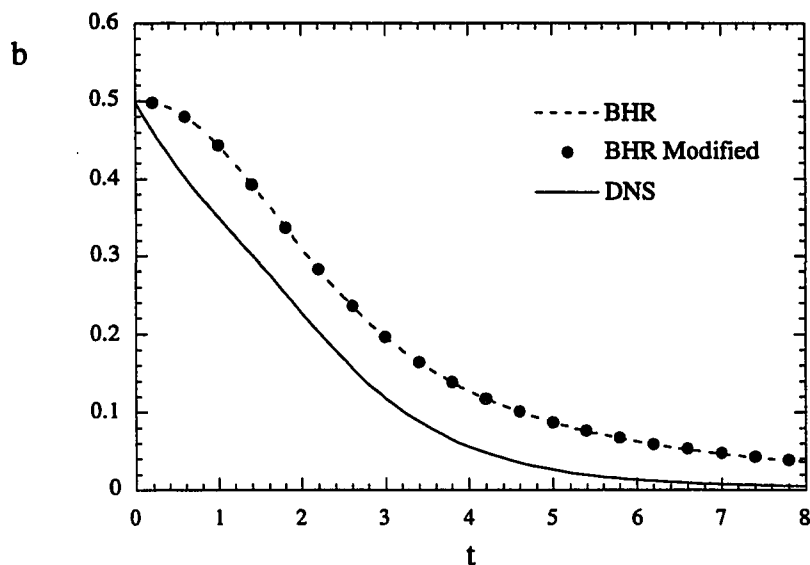
Figure 7.2: Evolution of b for Run Acc1c DNS and BHR models
