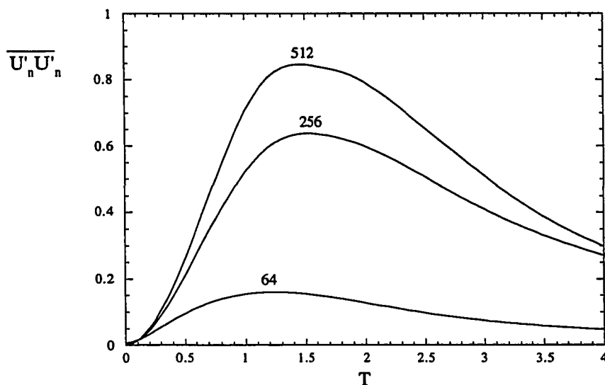
Figure 6.46: \overline{U'_n U'_n} vs. T for non-Boussinesq cases with an initial density ratio of 4 at various R_o
