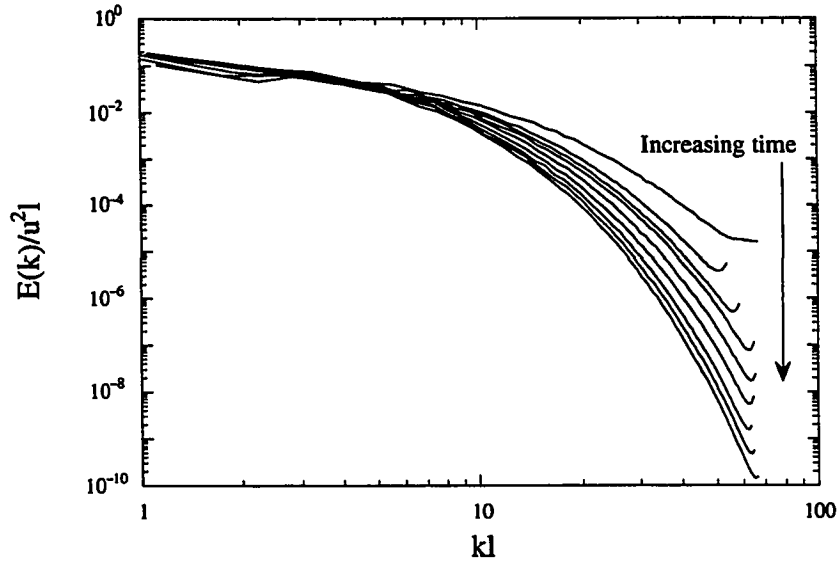
Figure 4.11: Large-scale normalization of the energy spectrum evolution for Run 55a
