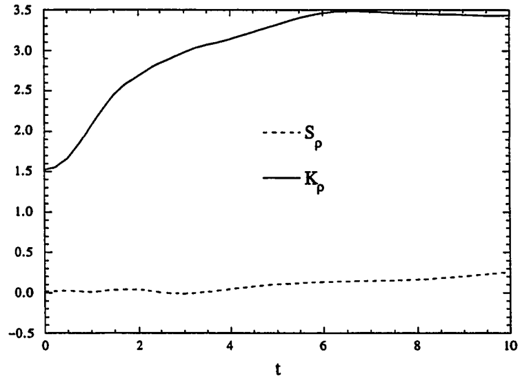
Figure 5.7: Skewness and Kurtosis of the density field for Run Iso3
