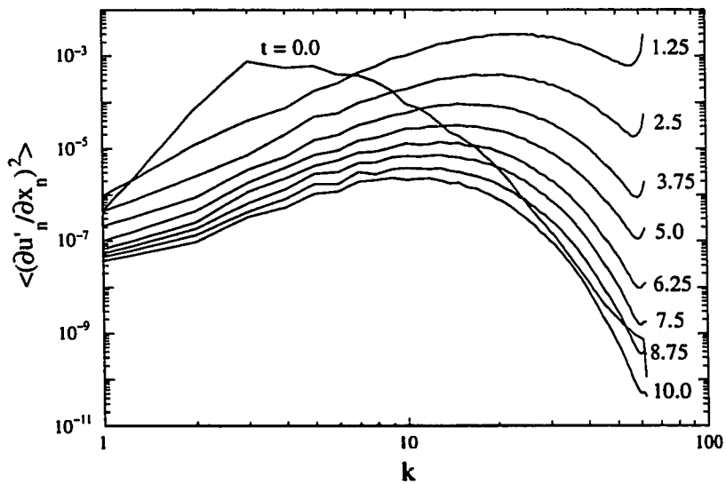
Figure 4.35: Spectra of the square-divergent velocity field condition for Run 55
