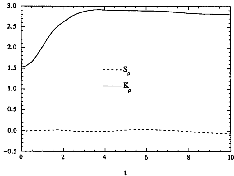
Figure 4.28: Evolution of the skewness and kurtosis of the density field for Run 55a
