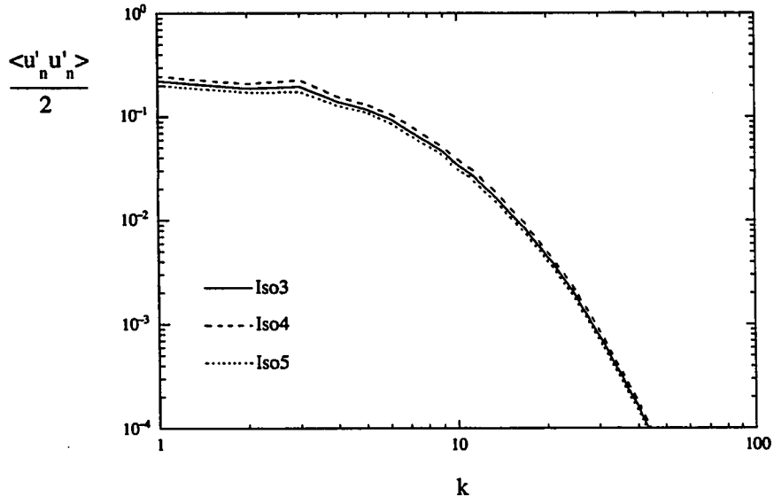
Figure 5.10: Initial spectrum of u'_n u'_n / 2 for Run Iso3, Iso4 and Iso5
