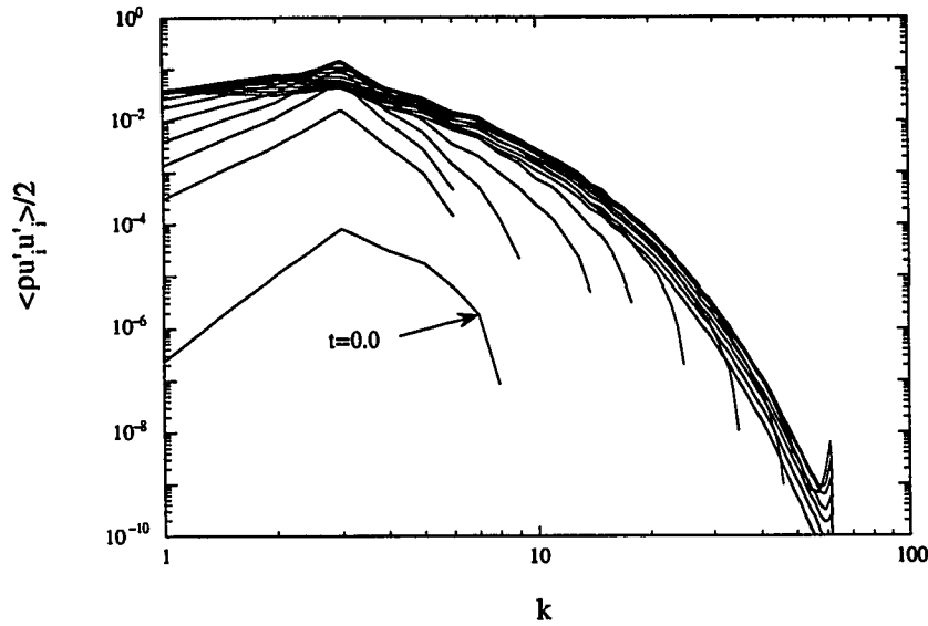
Figure 6.41: Spectral evolution of \rho u'_n u'_n / 2 at Re_o = 256 for initial density ratio of 4 case (Run Acc1c)
