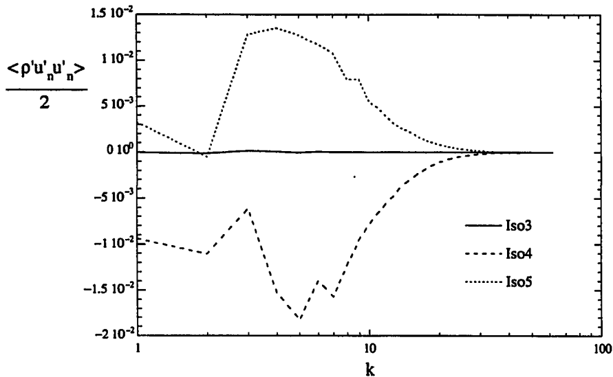
Figure 5.12: Initial spectrum of \rho' u'_n u'_n/2 for Run Iso3, Iso4 and Iso5
