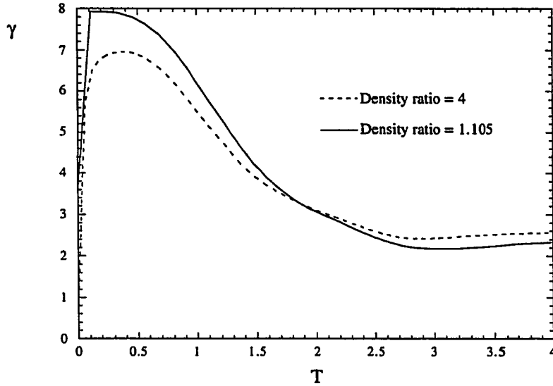
Figure 6.6: Measure of anisotropy of the mean-squared velocity for the initial density ratio = 1.105 case (solid lines) and the initial density ratio = 4 case (dashed lines)
