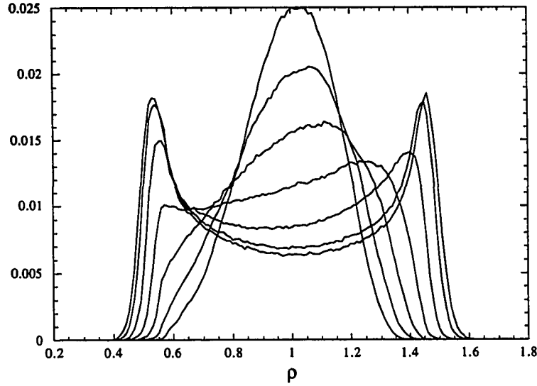
Figure 5.30: Density pdf evolution, t = 0.0 to 1.5 by 0.25 , for Run Iso5
