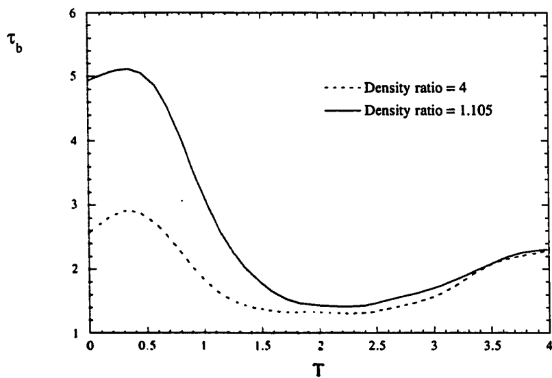
Figure 6.30: Comparison of the time scale of decay for b(t) at R_o = 256 for initial density ratio of 1.105 case (Run Acc1a) and 4 case (Run Acc1c)
