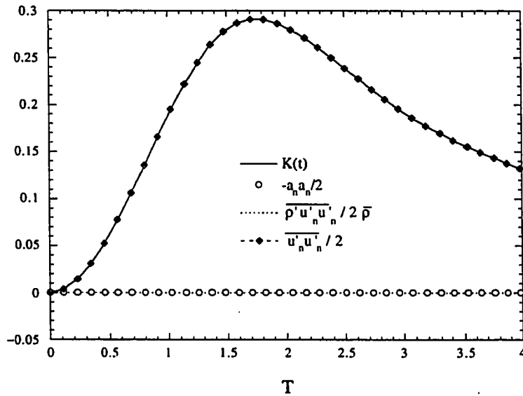
Figure 6.7: Terms of the total turbulent kinetic energy per unit mass for the initial density ratio = 1.105 case (Run Accl1a)
