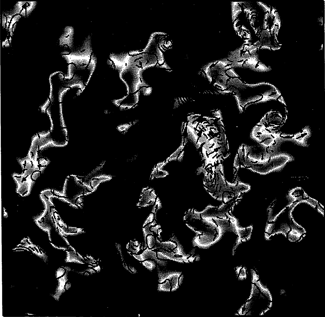
Figure 5.25: Two Dimensional slice of the x-y plane for Run Iso5
