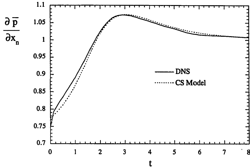
Figure 7.9: Evolution of \overline{v'(\partial p'/\partial x_n)} for Run Acc1c DNS and the CS model
