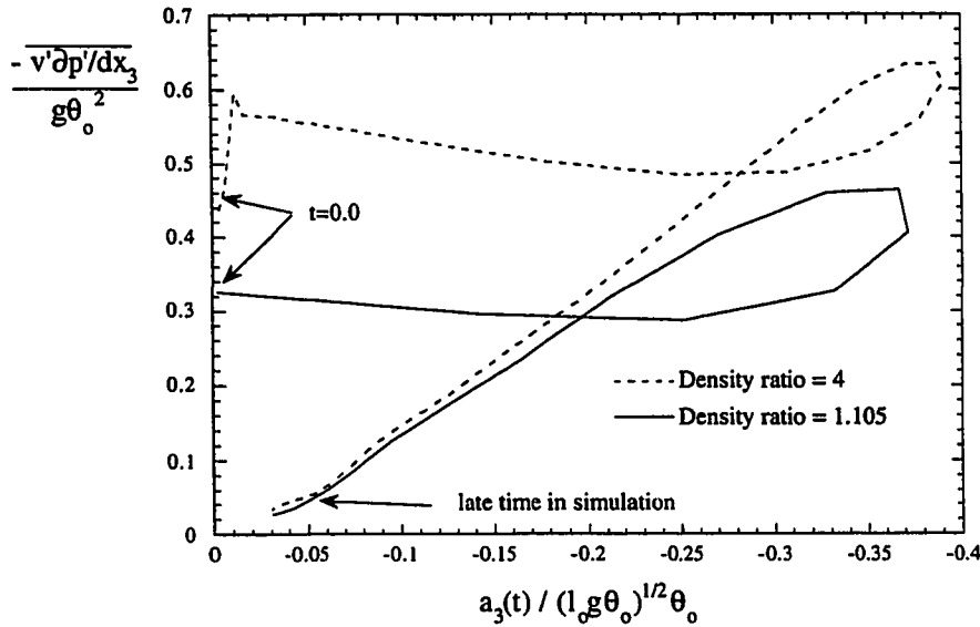
Figure 6.20: Nondimensional -\overline{v' \partial p' / \partial x_3} vs. nondimensional a_3 for initial density ratio of 1.105 and 4 cases at R_o = 256
