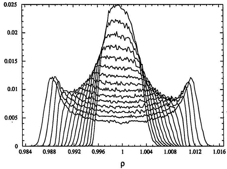
Figure 6.65: PDF evolution, for T=0.0 to 1.75 by 0.125, of the density field at R_o = 64 for initial density ratio of 4 case (Run Acc3c)
