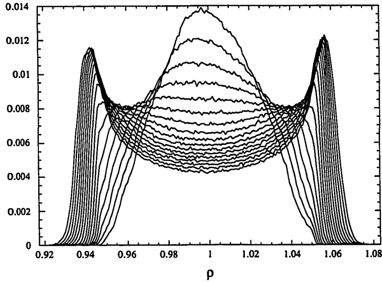
Figure 6.31: PDF evolution, for T=0.0 to 2.0 by 0.125 , of the density field at R_o = 256 for initial density ratio of 1.105 case (Run Acc1a)
