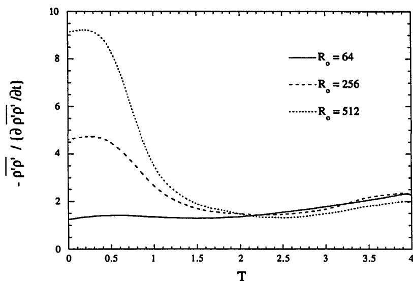
Figure 6.63: Evolution of the time scale of decay of the variance of the fluctuating density field for initial density ratio of 4 case at various R_o
