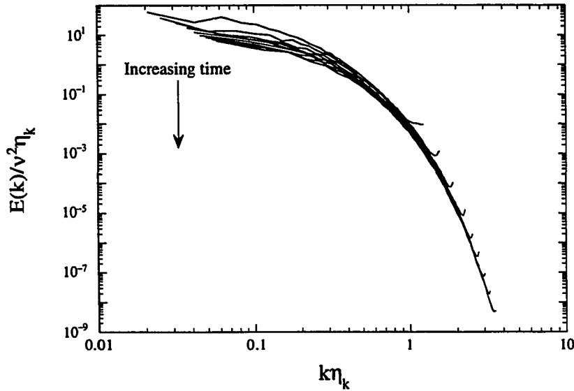
Figure 4.12: Small-scale normalization of the energy spectrum evolution for Run 55a
