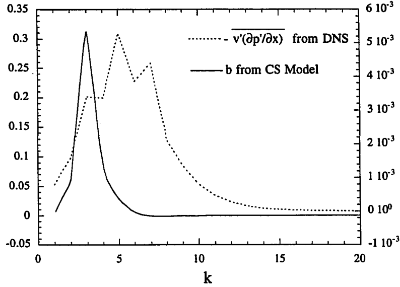
Figure 7.10: Spectra of \overline{v'(\partial p'/\partial x_n)} for Run Acc1c DNS and of b for the CS model at t = 0.1
