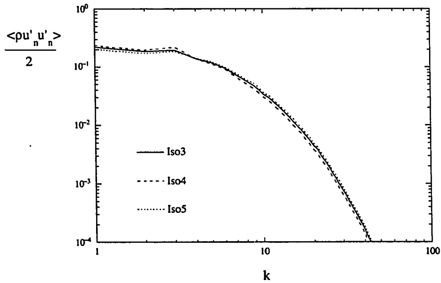
Figure 5.11: Initial spectrum of \rho u'_n u'_n / 2 for Run Iso3, Iso4 and Iso5
