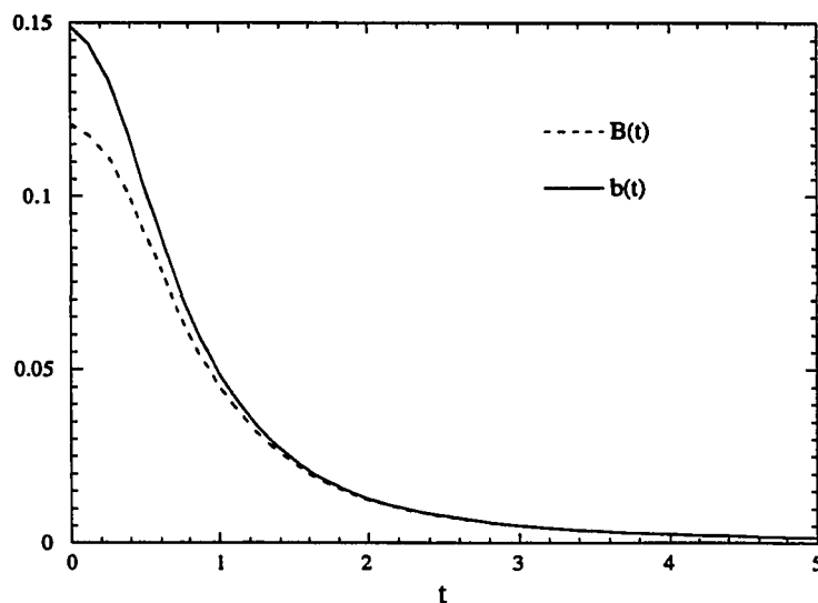
Figure 5.26: Evolution of b(t) = -\overline{\rho'v'} and B(t) = \overline{\rho'\rho'}/\bar{\rho}^2 for Run Iso4
