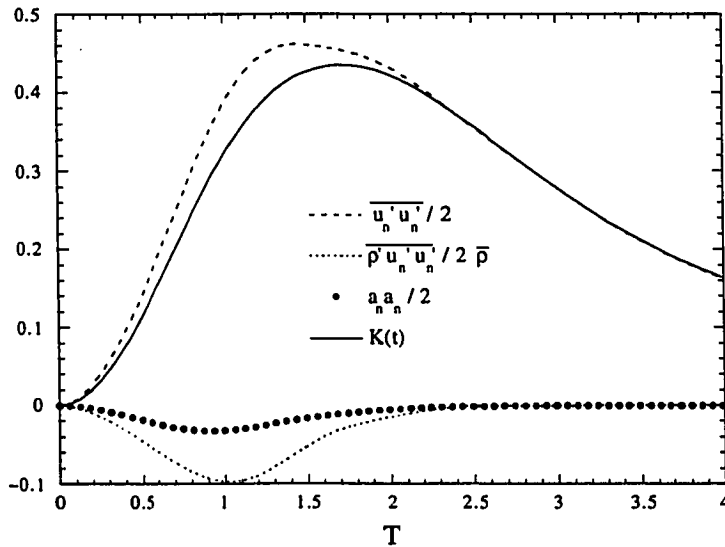
Figure 6.49: Terms of the total turbulent kinetic energy per unit mass for the initial density ratio of 4 cases at R_o = 512 (Run Acc2c)
