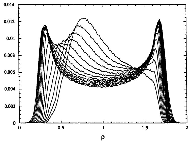
Figure 6.66: PDF evolution, for T=0.0 to 1.75 by 0.125, of the density field at R_o = 512 for initial density ratio of 4 case (Run Acc2c)
