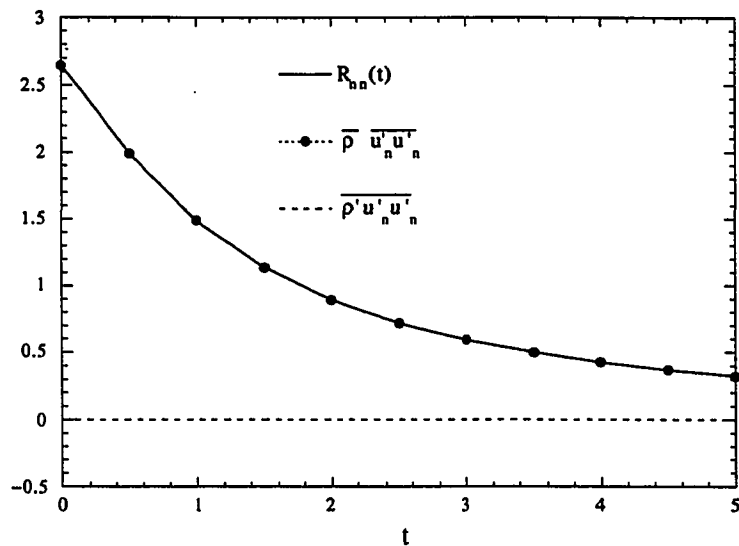
Figure 5.1: The evolution of R_{nn} for Run Iso3
