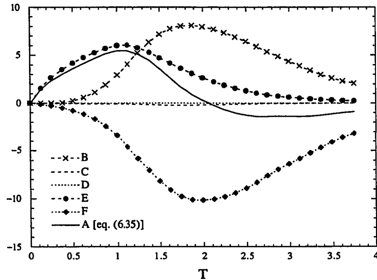
Figure 6.23: Terms of the enstrophy evolution equation [eq. (6.35)] for initial density ratio of 4 case (Run Acc1c)
