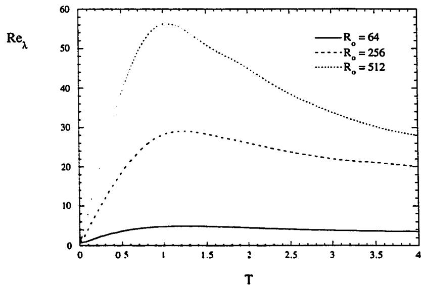
Figure 6.53: Taylor Reynolds number evolution for the density ratio of 4 cases at various R_o
