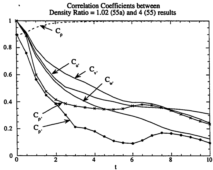
Figure 4.37: Correlation coefficients for the velocity, density and pressure fields between Run 55 and Run 55a
