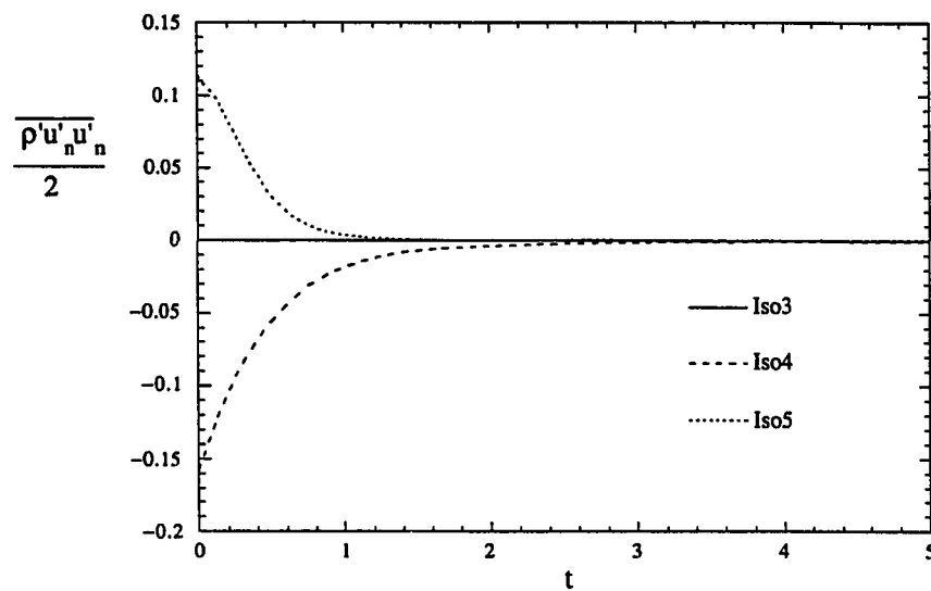
Figure 5.17: Evolution of \overline{\rho' u'_n u'_n} for Runs Iso3 (nearly constant-density), Iso4 (light fluid moving fast) and Iso5 (heavy fluid moving fast)
