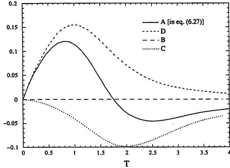
Figure 6.8: Terms in the evolution equation [eq. (6.27)] for \overline{\rho u_i' u_i'}/2 for initial density ratio of 1.105 case (Run Ac1a)
