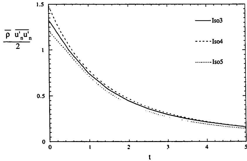
Figure 5.14: Evolution of \bar{\rho} \overline{u'_n u'_n} for Runs Iso3 (nearly constant-density), Iso4 (light fluid moving fast) and Iso5 (heavy fluid moving fast)
