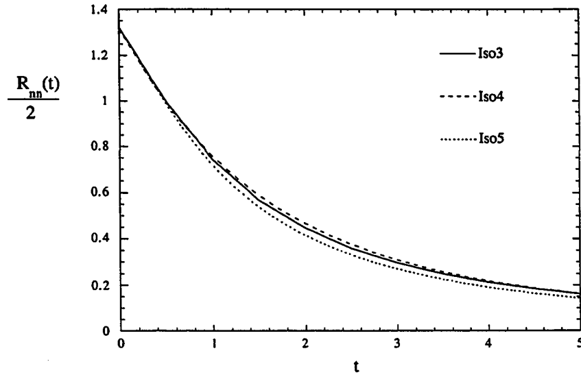
Figure 5.13: Total turbulent kinetic energy density evolution for Runs Iso3 (nearly constant-density), Iso4 (light fluid moving fast) and Iso5 (heavy fluid moving fast)
