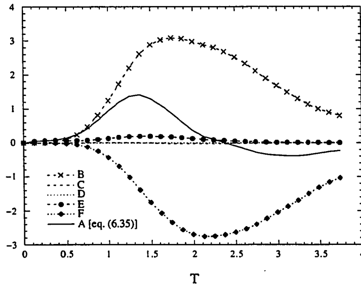
Figure 6.26: Terms of the z-direction contribution to the enstrophy evolution equation [eq. (6.35)] for initial density ratio of 4 case (Run Acc1c)
