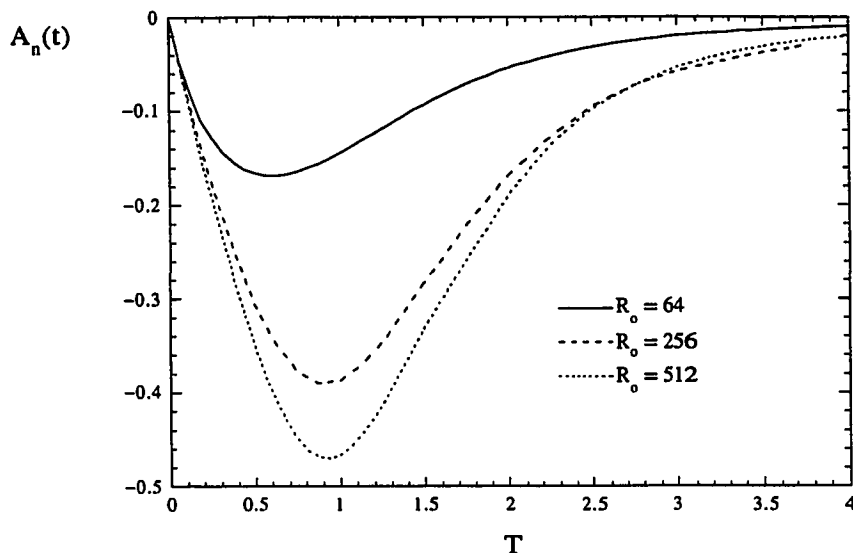
Figure 6.51: Turbulent mass flux for initial density ratio of 4 cases at various R_o
