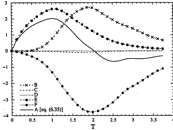
Figure 6.25: Terms of the x-direction contribution to the enstrophy evolution equation [eq. (6.35)] for initial density ratio of 4 case (Run Acc1c)
