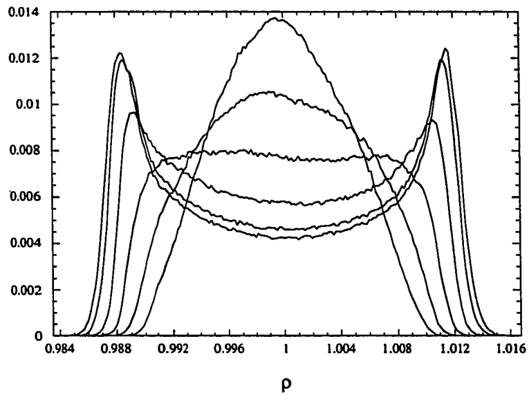
Figure 5.8: PDF evolution, t = 0.0 to 1.5 by 0.25 , for Run Iso3
