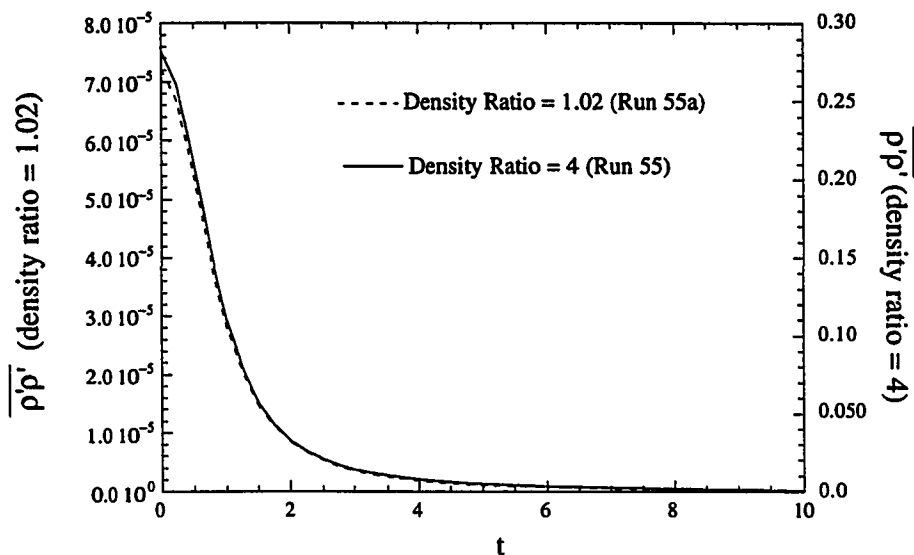
Figure 4.19: Evolution of \overline{\rho'\rho'} for Run 55 and Run55a
