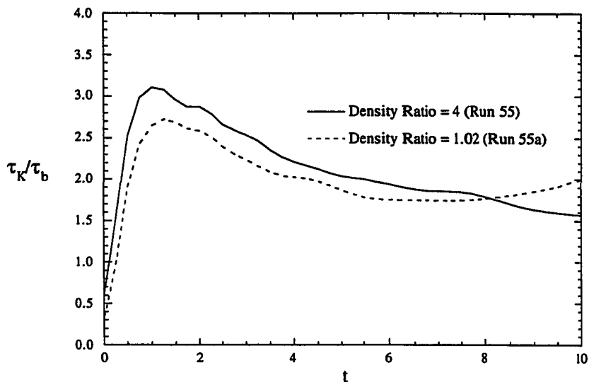
Figure 4.24: Mechanical-to-density time-scale ratio for Run 55 and 55a
