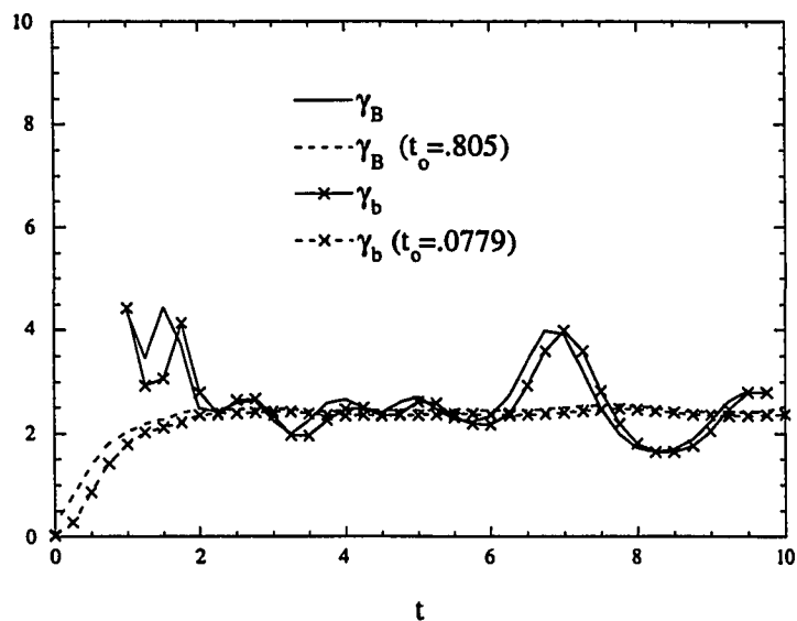
Figure 4.22: Power law exponents for the decay of b(t) and B(t) for Run 55
