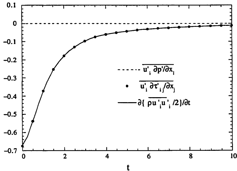
Figure 4.5: Terms in the evolution equation [eq. (4.4)] for the total kinetic energy density for Run 55a
