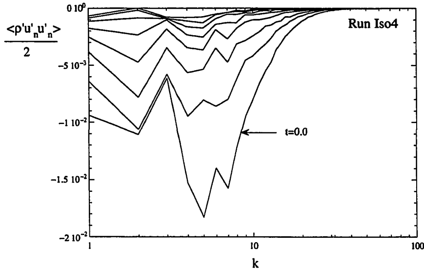
Figure 5.33: Spectral evolution of \rho' u'_n u'_n / 2 for Run Iso4
