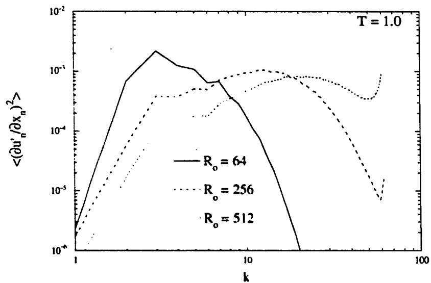
Figure 6.69: Spectra of (\partial u'_n / \partial x_n)^2 at T = 1.0 for different R_o
