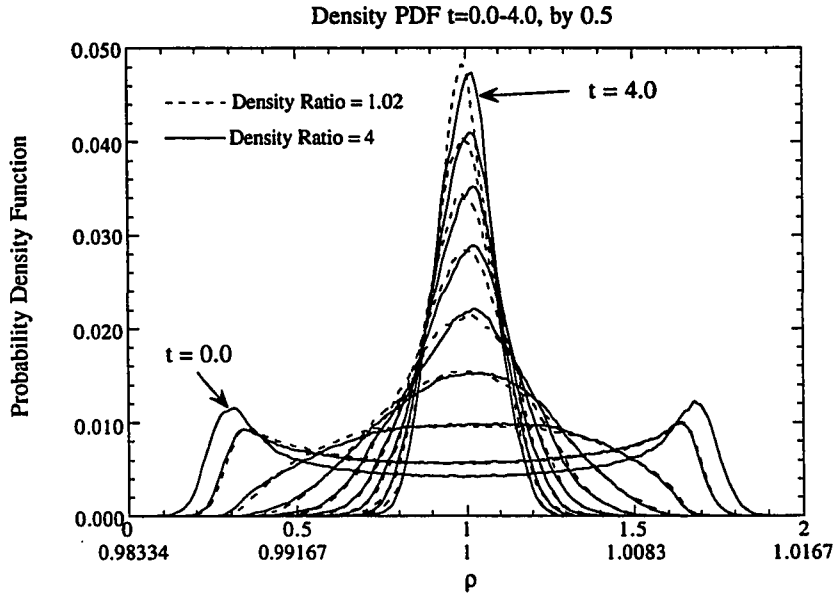
Figure 4.27: Density pdf evolution for Run 55 and Run 55a
