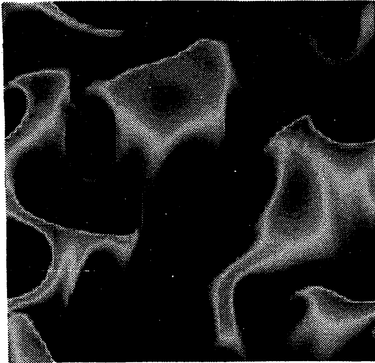
Figure 6.33: x-z cross-section of the density field near the y-midplane for an accelerated case at T = 1 . Heaviest fluid is orange and the lightest is purple.
