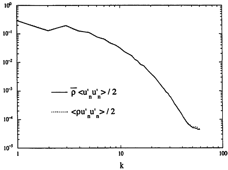
Figure 4.16: Initial spectrum for \bar{\rho} \langle u'_i u'_i \rangle / 2 and \langle \rho u'_i u'_i \rangle / 2 for Run 55
