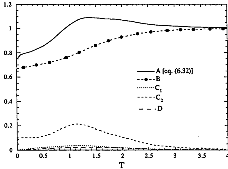
Figure 6.55: Evolution of terms in the mean-pressure-gradient equation [eq. (6.32)] for initial density ratio of 4 case at R_o = 512 (Run Acc1c)
