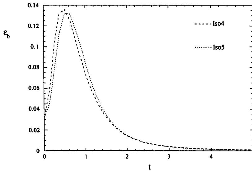
Figure 5.28: b(t) dissipation rate evolution for Runs Iso4 and Iso5
