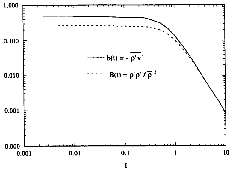
Figure 4.21: Evolution of b(t) and B(t) for Run 55
