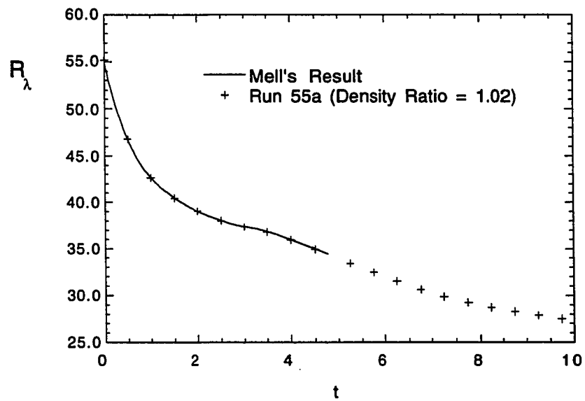
Figure 4.9: Evolution of R_\lambda comparison with Mell's result and Run 55a
