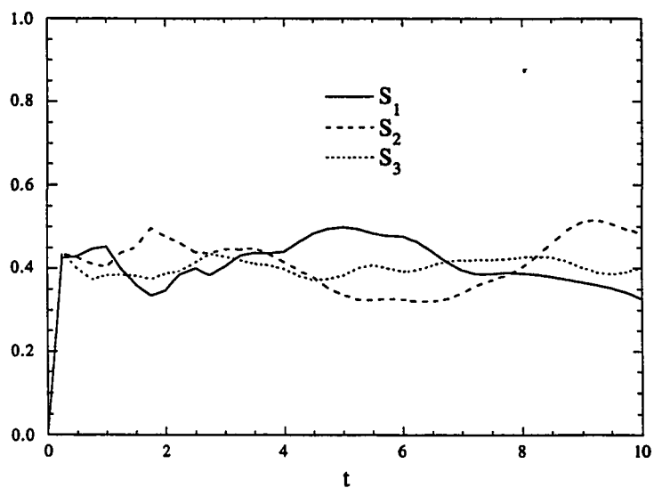
Figure 5.4: The velocity derivative skewness for the three components of velocity for Run Iso3
