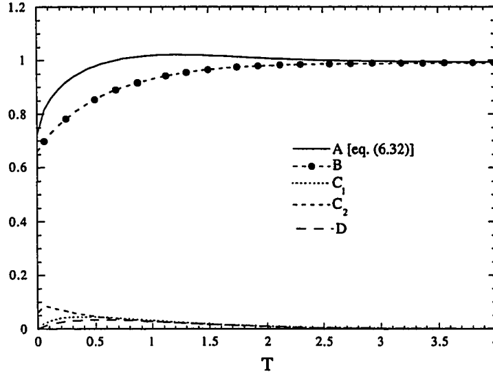
Figure 6.54: Evolution of terms in the mean-pressure-gradient equation [eq. (6.32)] for initial density ratio of 4 case at R_o = 64 (Run Acc1c)
