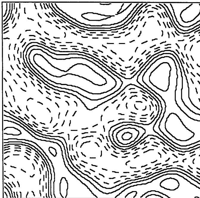
Figure 4.1: Typical 2-D slice of the 3-D initial density field
