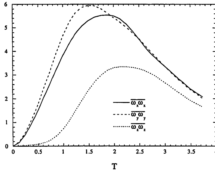
Figure 6.24: Contributions from each direction to the enstrophy for initial density ratio of 4 case (Run Acc1c)
