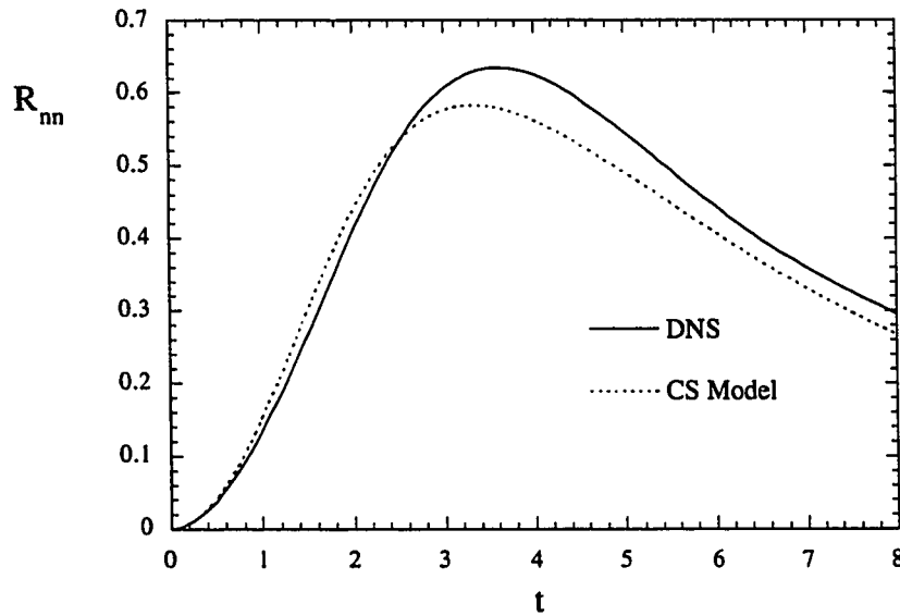
Figure 7.8: Evolution of R_{nn} for Run Acc1c DNS and the CS model
