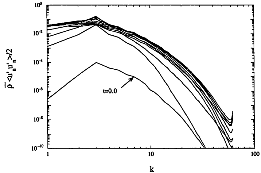
Figure 6.42: Spectral evolution of \bar{\rho} u'_n u'_n / 2 at R_o = 256 for initial density ratio of 4 case (Run Acc1c)
