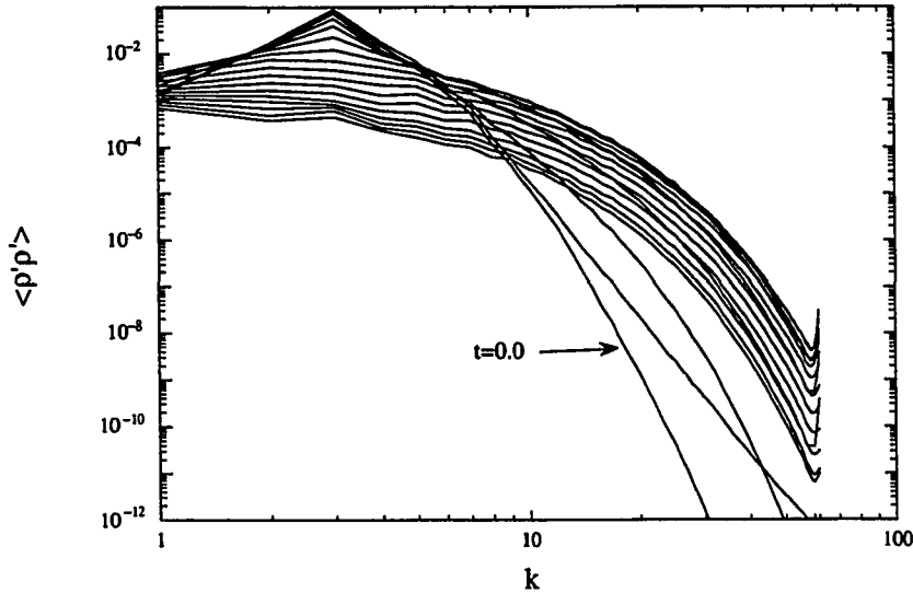
Figure 6.44: Spectral evolution of \rho' \rho' at R_o = 256 for initial density ratio of 4 case (Run Acc1c)
