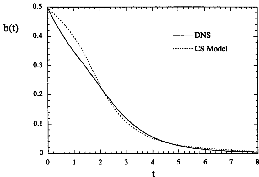
Figure 7.6: Evolution of b for Run Acc1c DNS and the CS model
