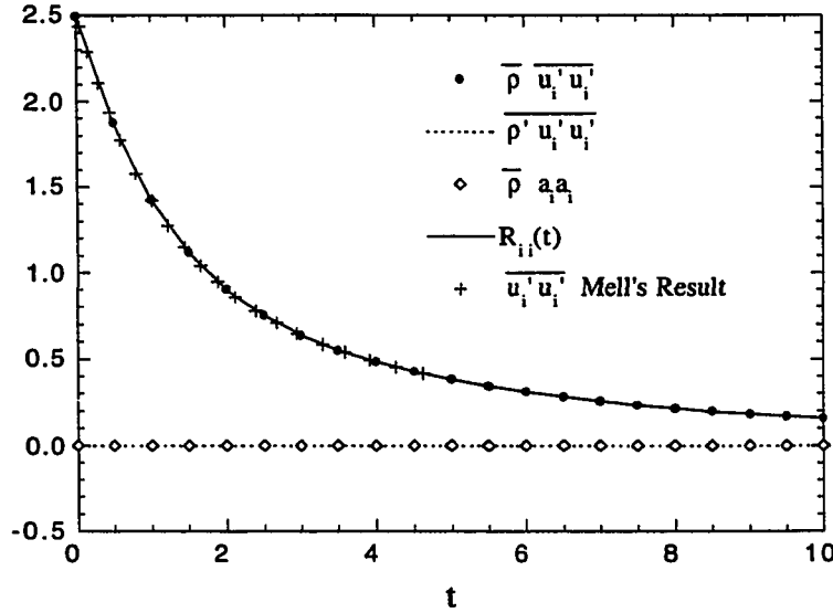
Figure 4.4: Evolution of R_{ii} for Run 55a
