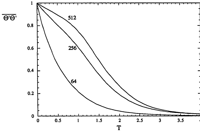
Figure 6.61: \overline{\Theta'\Theta'} vs. T as a function of R_o for non-Boussinesq cases with an initial density ratio of 4
