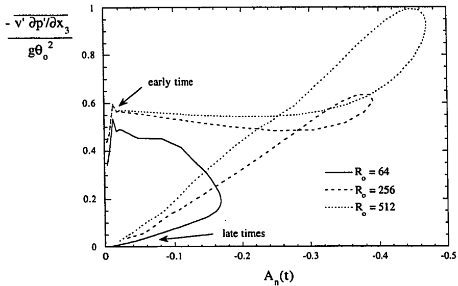
Figure 6.60: Nondimensional -\overline{v'\partial p'/\partial x_3} as a function of nondimensional a_3(t) for initial density ratio of 4 cases at various R_o
