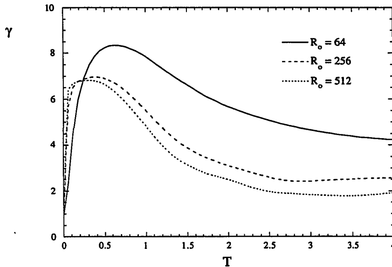
Figure 6.47: Measure of anisotropy of the mean-squared velocity for the initial density ratio of 4 cases for various R_o
