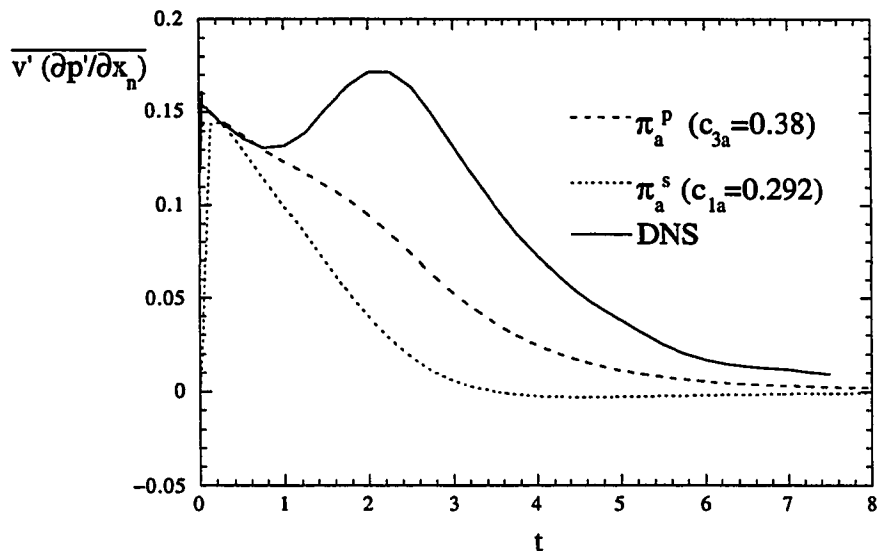
Figure 7.1: \overline{v'(\partial p'/\partial x_n)} term and models for Run Acc1c
