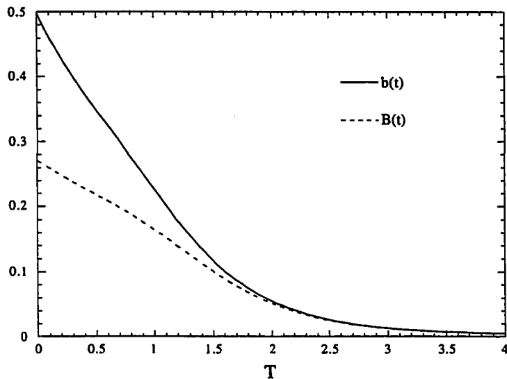
Figure 6.29: Comparison of b(t) and B(t) evolution for initial density ratio of 4 case at R_o=256 (Run Acc1c)
