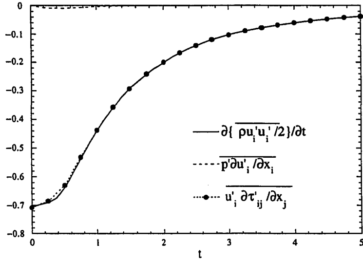
Figure 5.22: Terms in the evolution equation [eq. (4.4)] for total kinetic energy density for Run Iso5
