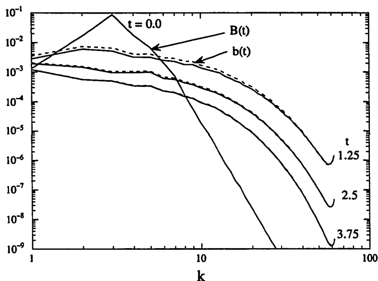
Figure 4.33: Density self-correlation and negative density-specific volume correlation spectra for Run 55
