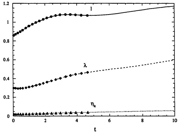
Figure 4.8: Length as a function of time comparison with Mell's result and Run 55a
