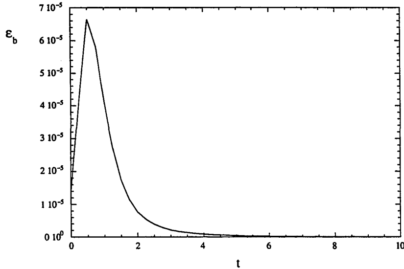
Figure 5.6: Dissipation rate evolution for b(t) = -\overline{\rho'v'} for Run Iso3
