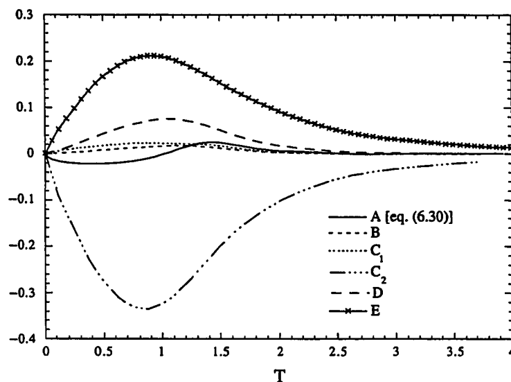
Figure 6.11: Terms of the evolution equation [eq. (6.30)] for \overline{\rho' u_i' u_i} / 2 for initial density ratio of 4 case (Run Acc1c)
