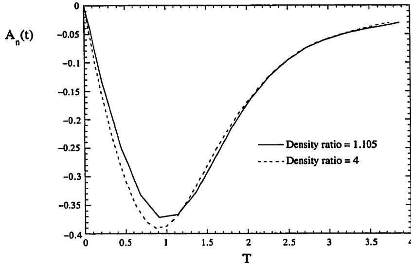
Figure 6.12: Turbulent mass flux for initial density ratio of 1.105 case (Run Ac1a) and the initial density ratio of 4 case (Run Ac1c)
