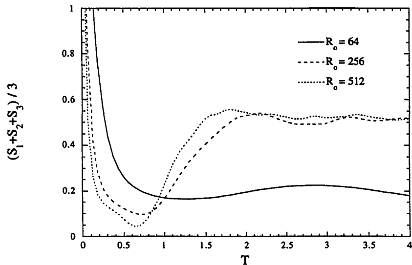
Figure 6.52: Average velocity derivative skewness for the density ratio of 4 cases at various R_o
