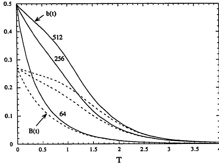
Figure 6.64: Comparison of b(t) and B(t) evolution for initial density ratio of 4 case at various R_o
