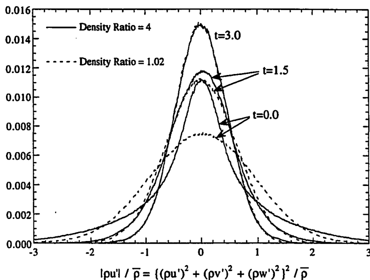
Figure 4.31: Momentum pdf evolution for Run 55 and Run 55a
