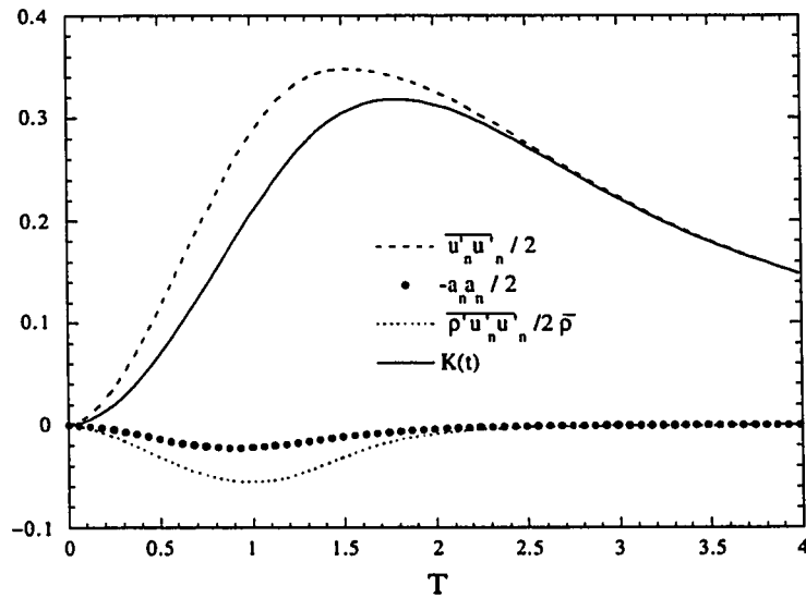
Figure 6.9: Terms of the total turbulent kinetic energy per unit mass for the initial density ratio = 4 case at R_o = 256 (Run Ac1c)
