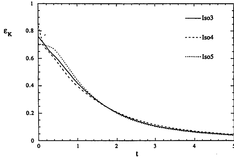
Figure 5.15: Total kinetic energy density dissipation rate for Runs Iso3 (nearly constant-density), Iso4 (light fluid moving fast) and Iso5 (heavy fluid moving fast)
