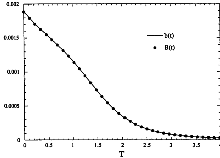
Figure 6.28: Comparison of b(t) and B(t) evolution for initial density ratio of 1.105 case at R_o=256 (Run Acc1a)
