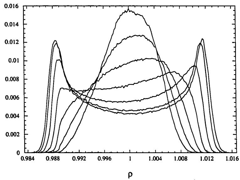
Figure 5.38: Density pdf evolution, t = 0.0 to 1.5 by 0.25, for Run Iso8
