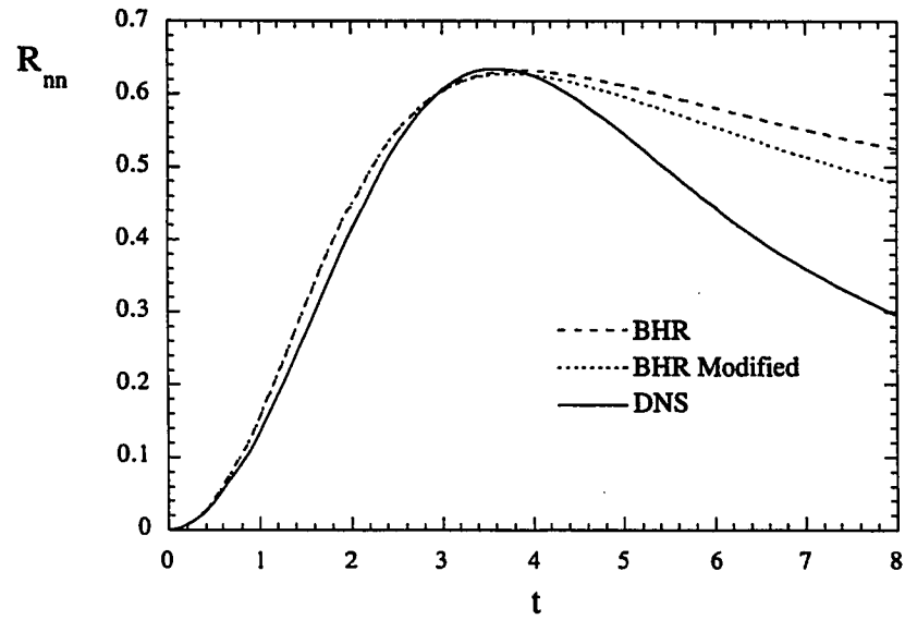
Figure 7.4: Evolution of R_{nn} for Run Acc1c DNS and BHR models
