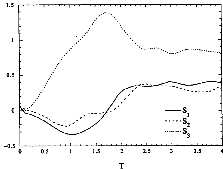
Figure 6.14: Velocity derivative skewness for each component for the initial density ratio of 1.104 case (Run Acc1a)
