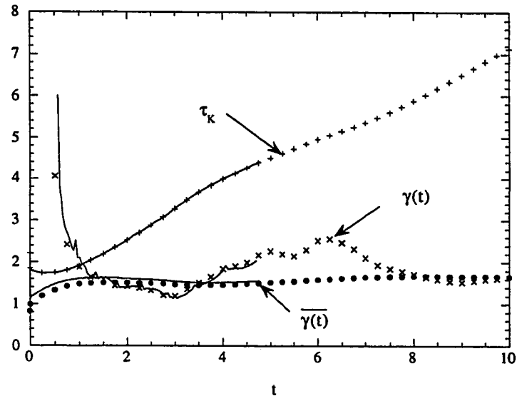
Figure 4.6: Time scale and power law exponents for Run 55a and comparison to Mell's results (solid lines)
