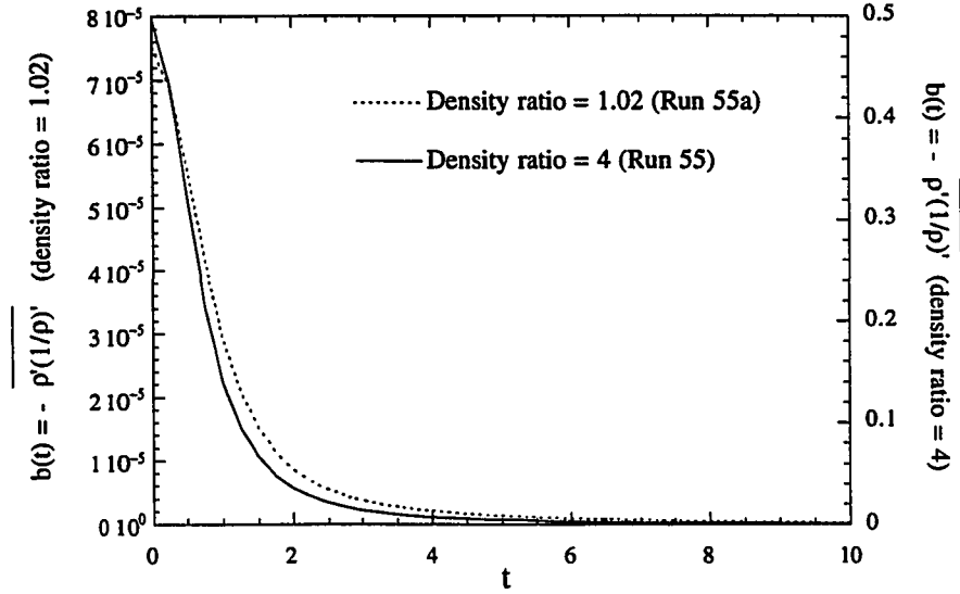
Figure 4.18: Comparison of the evolution of b(t) for Run 55 and Run 55a
