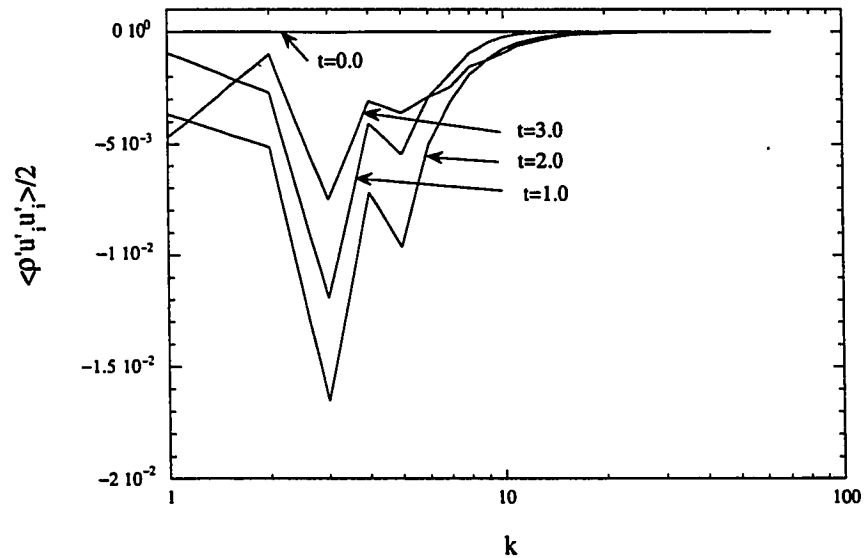
Figure 6.43: Spectral evolution of \rho' u'_n u'_n / 2 at R_o = 256 for initial density ratio of 4 case (Run Acc1c)
