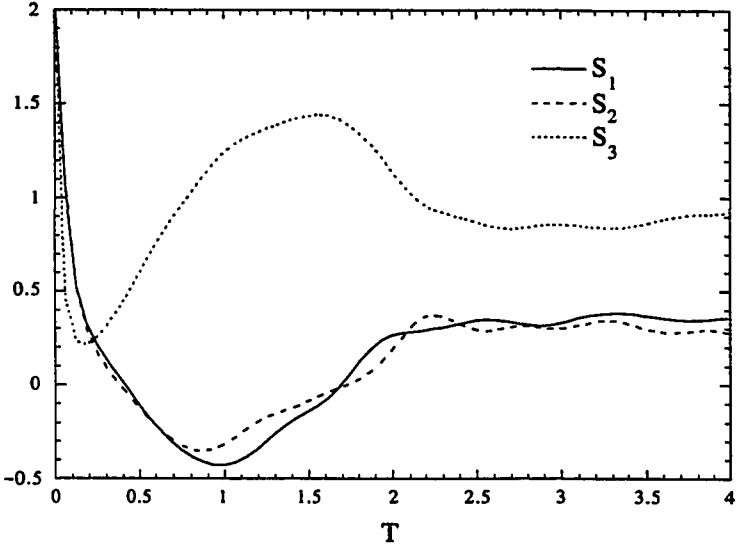
Figure 6.15: Velocity derivative skewness for each component for the initial density ratio of 1.104 case (Run Acc1a)
