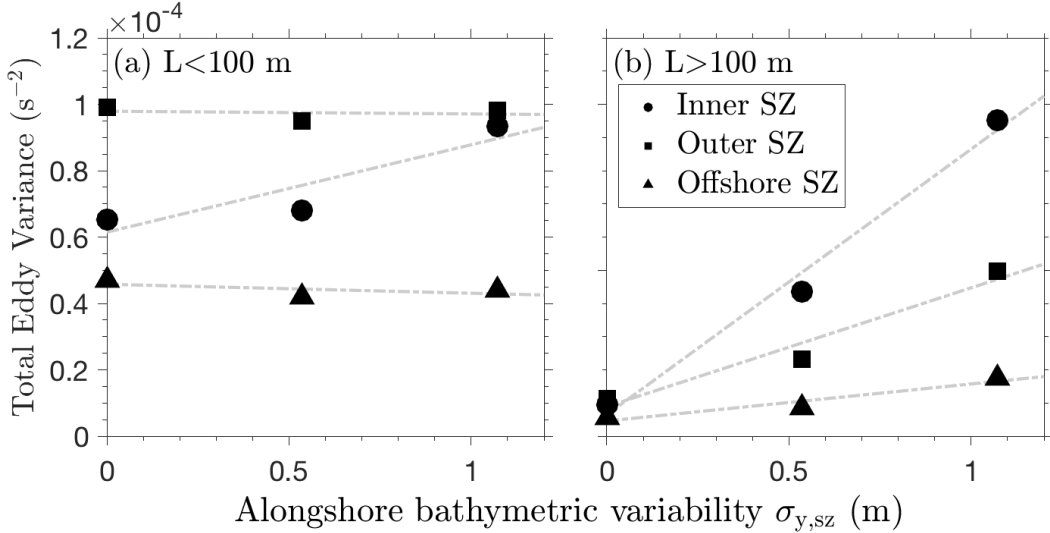
Figure 4.1: The average total variance of small (a, L < 100 m) and large (b, L > 100 m) eddy length scales for the inner surf zone (SZ) (circles, 0.2 < x/L_{sz} < 0.5 ), outer surf zone (squares, 0.5 < x/L_{sz} < 1 ), and offshore of the surf zone (triangles, 1 < x/L_{sz} < 1.5 ) versus the alongshore standard deviation of surfzone bathymetric variability for each simulation (S3, S4, S5). A linear fit is shown for each region (grey dashed lines).
