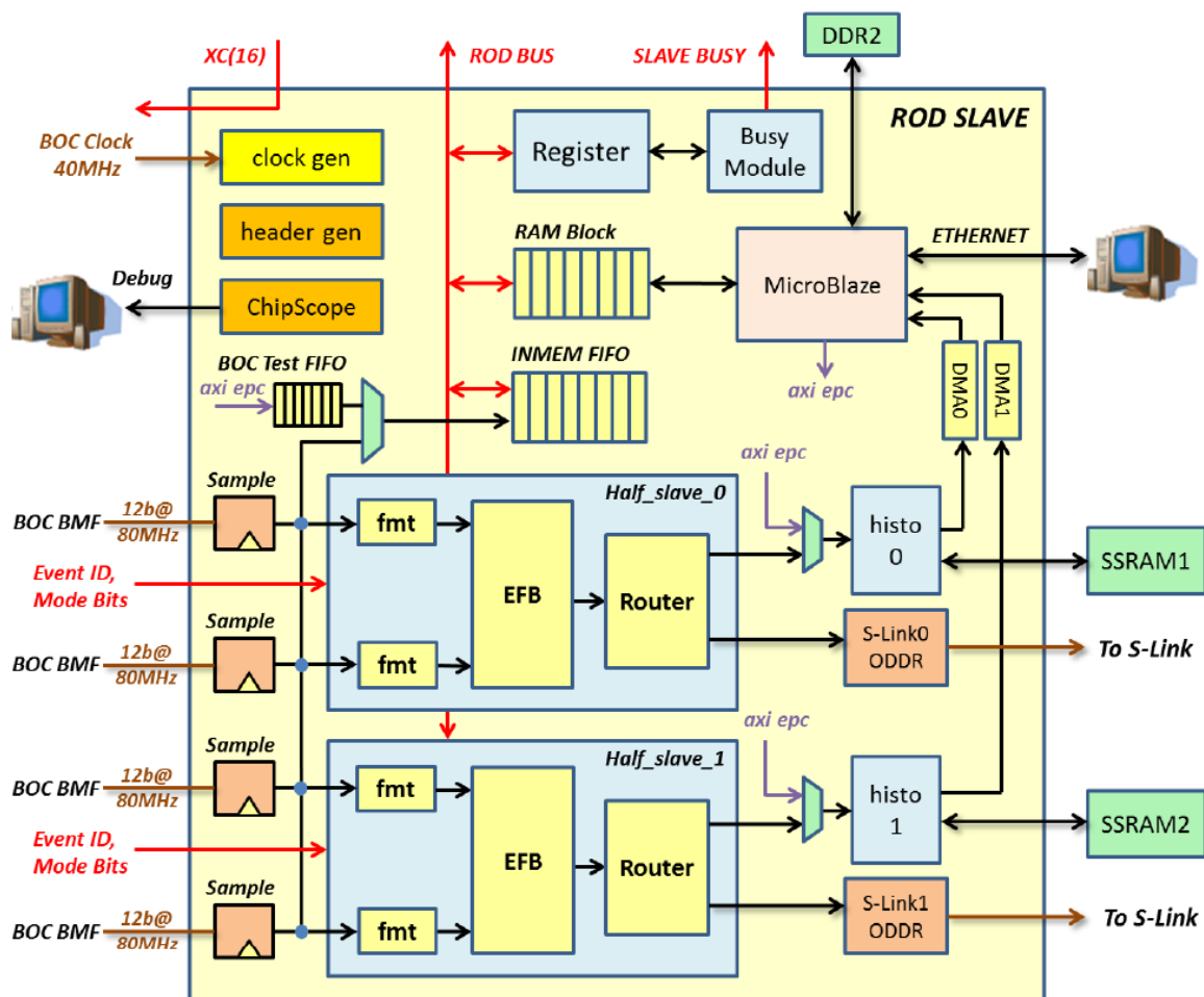
Figure 2.2: ROD Slave Diagram [4]
