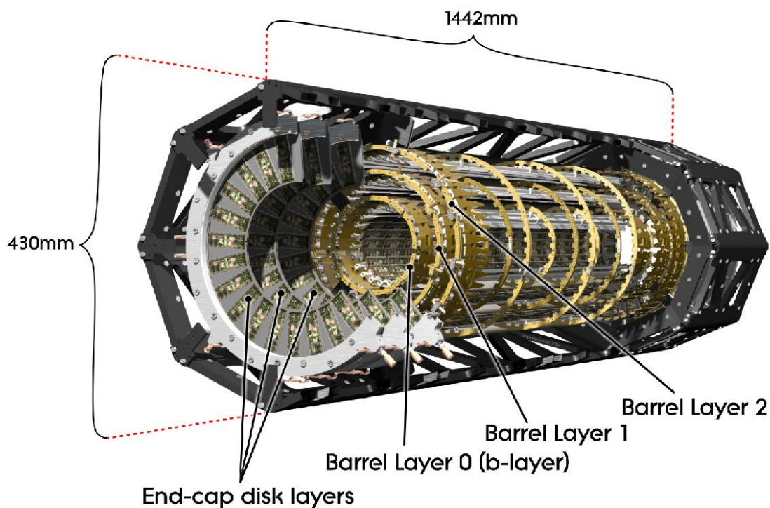
Figure 1.3: The Pixel Detector before the insertion of IBL [1]
