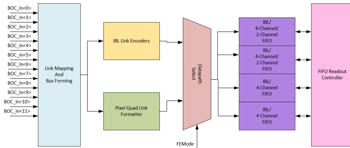
Figure 3.4: Formatter Datapath showing L1/L2 integrated with IBL
