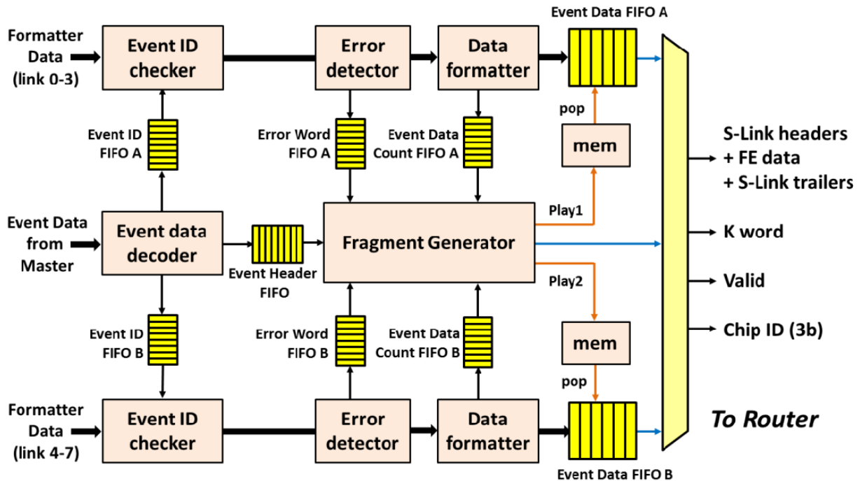
Figure 2.5: Block diagram of the Event Format Builder [4]
