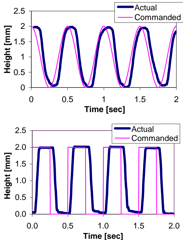
Figure 9 a,b. 2 Hz sine wave and square wave tracking
