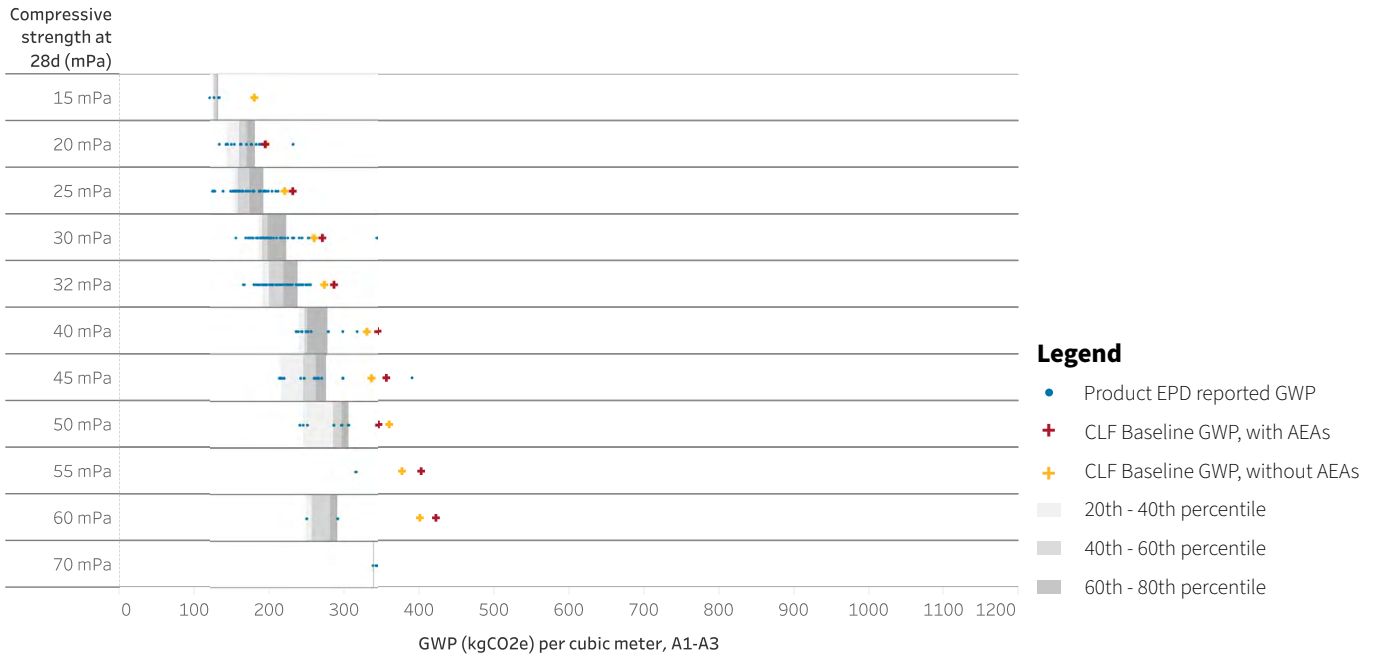
Figure 27. Range of applicable product EPDs and CLF Baselines.
