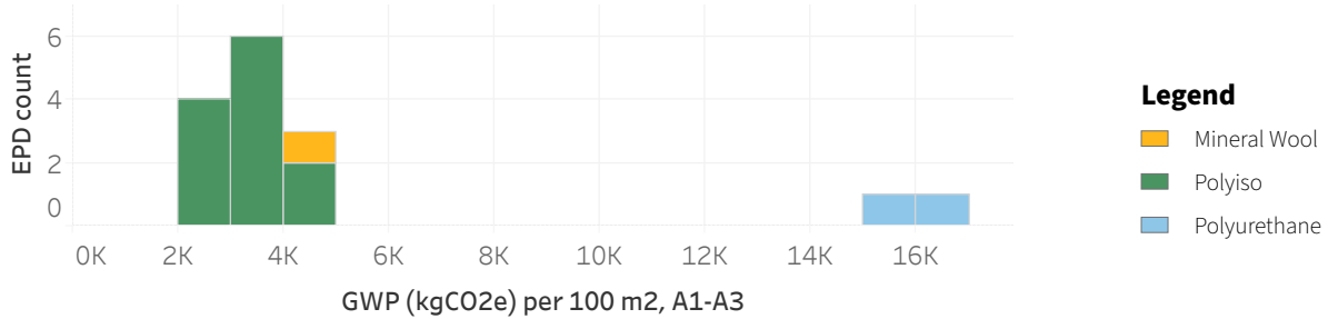
Figure 4. Product EPD GWP by insulating material. Some IMP products with a proprietary hybrid foam core are grouped here with polyiso as polyiso is a similar generic insulating material in terms of R-value and GWP. 2 The polyurethane core products have a much higher carbon footprint due to the use of HFC blowing agents that emit to the atmosphere during foam production.
