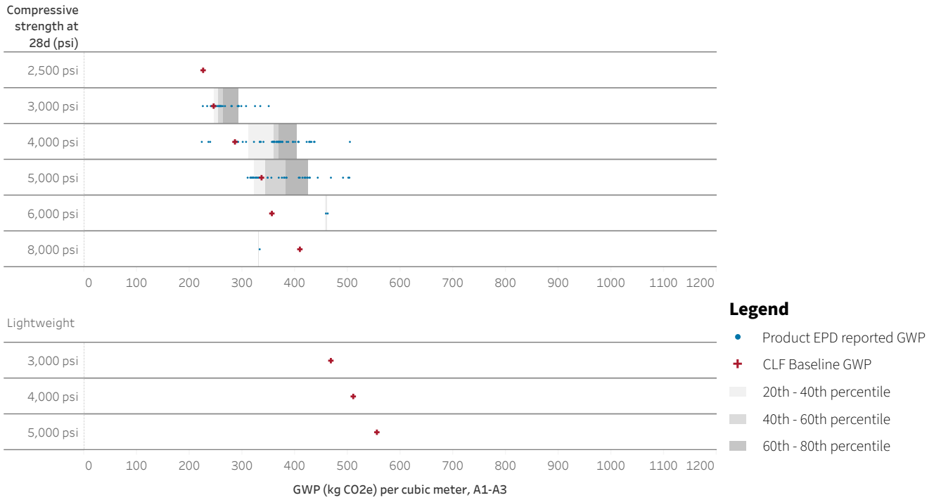
Figure 17. Range of applicable product EPDs and CLF Baselines.
