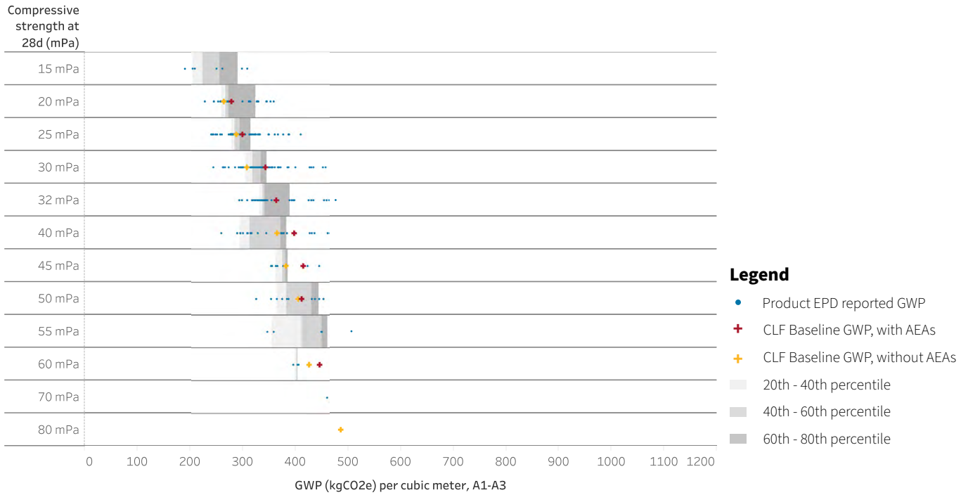
Figure 36. Range of applicable product EPDs and CLF Baselines.
