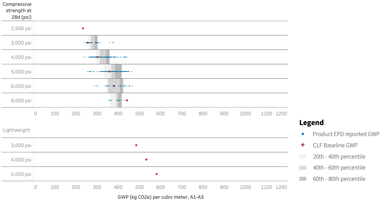
Figure 15. Range of applicable product EPDs and CLF Baselines.
