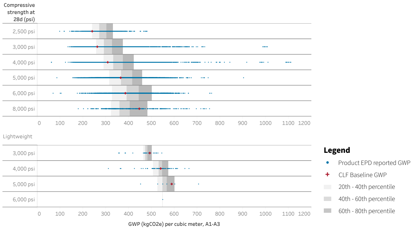
Figure 9. Range of applicable product EPDs and CLF Baselines.
