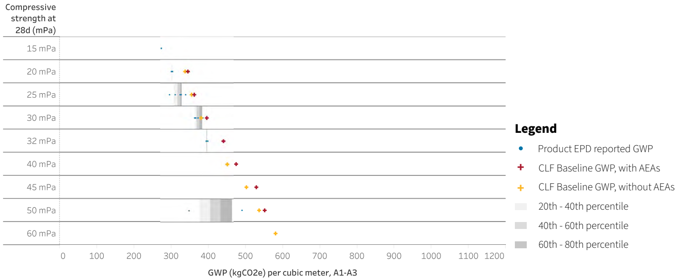
Figure 38. Range of applicable product EPDs and CLF Baselines
