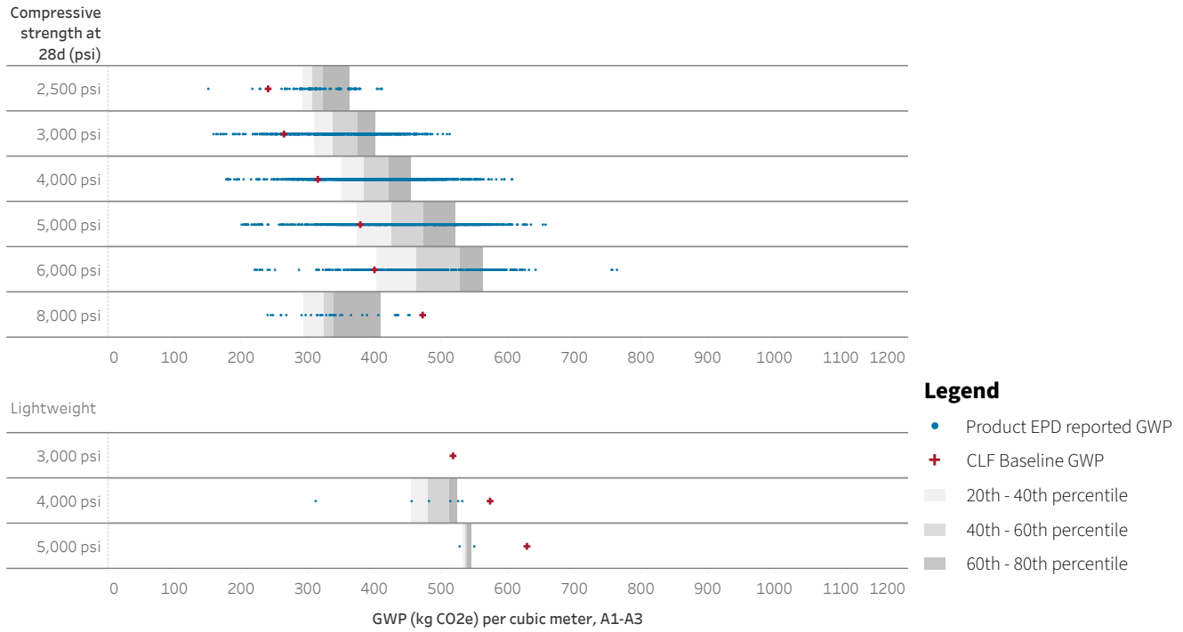
Figure 25. Range of applicable product EPDs and CLF Baselines.
