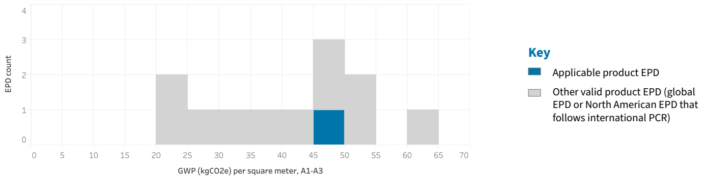
Figure 2. Range of global processed glass product EPDs. The single applicable product EPD represents a laminated glass product made of two layers of tempered glass bonded with a polyvinyl butyral (PVB) interlayer.
