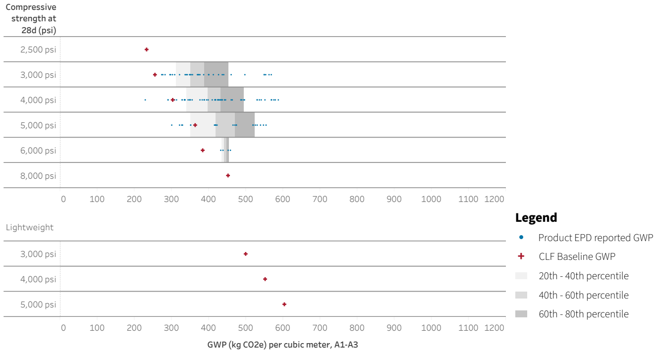
Figure 23. Range of applicable product EPDs and CLF Baselines.
