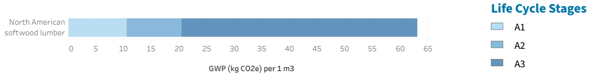
Figure 1. GWP contribution by life cycle stage. A1 = forestry operations; A2 = transport of roundwood to mill; and A3 = lumber production at mill.
