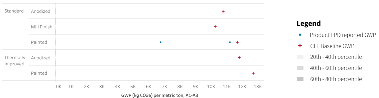
Figure 2. Range of applicable product EPDs and CLF Baselines.
