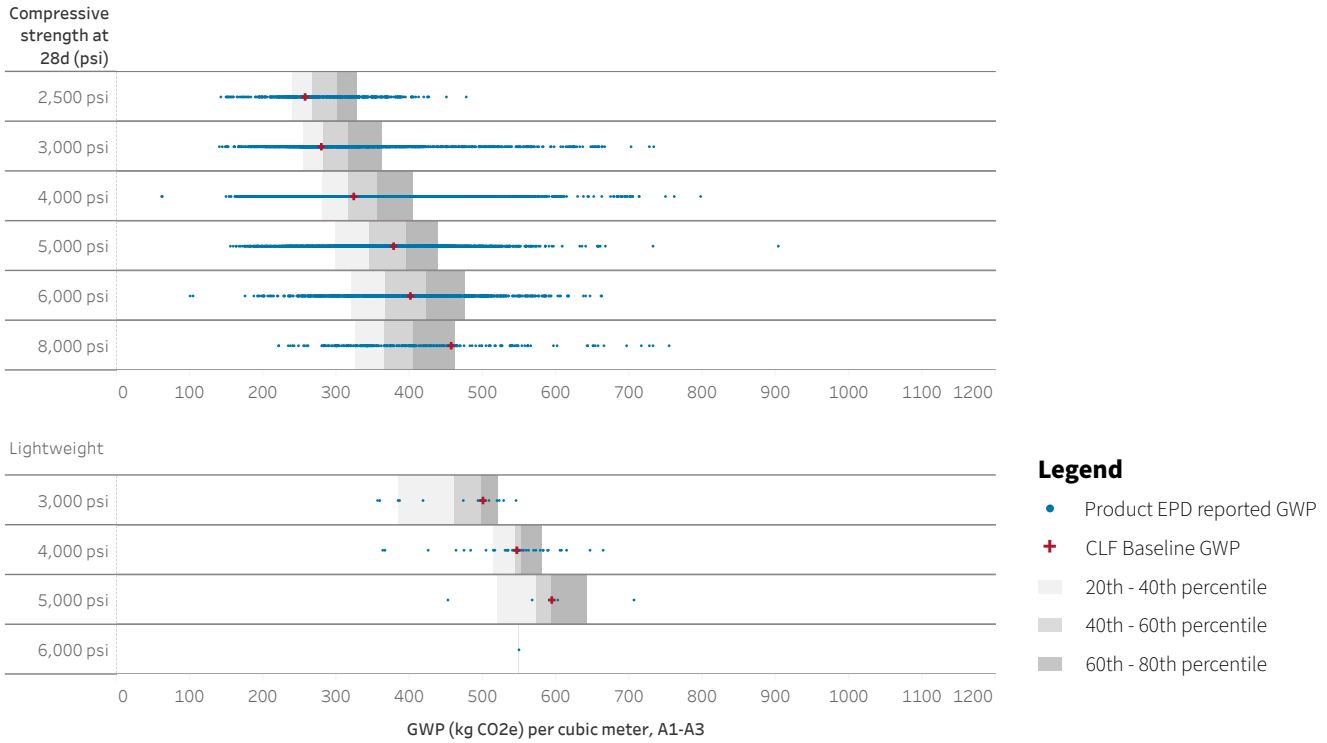
Figure 11. Range of applicable product EPDs and CLF Baselines.
