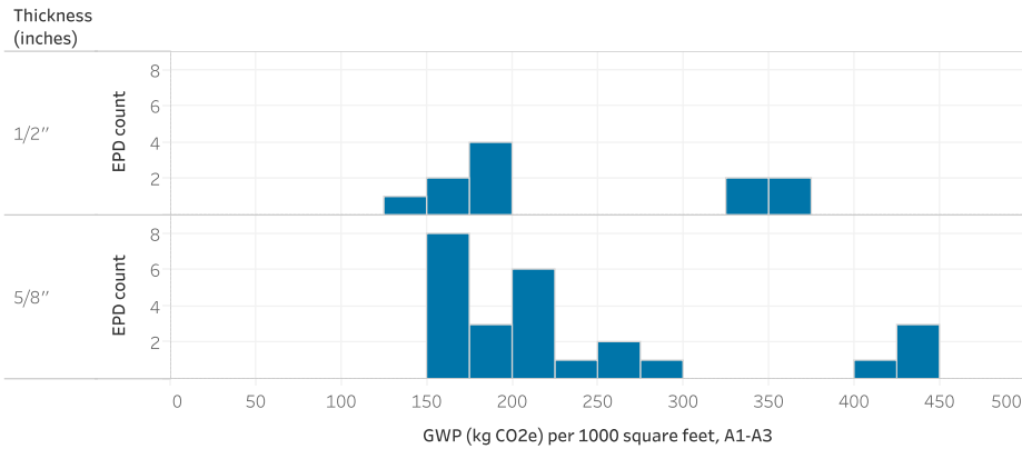
Figure 4. Distribution of applicable product EPDs.
