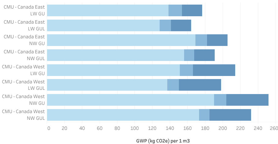
Figure 1. GWP contribution by life cycle stage. “NW” = normal weight. “LW” = lightweight. “GU” = general use (portland) cement. “GUL” = portland-limestone cement. The product types shown are based on the eight valid IW-EPDs in North America, from the Canadian Concrete Masonry Producers Association (CCMPA). 1
