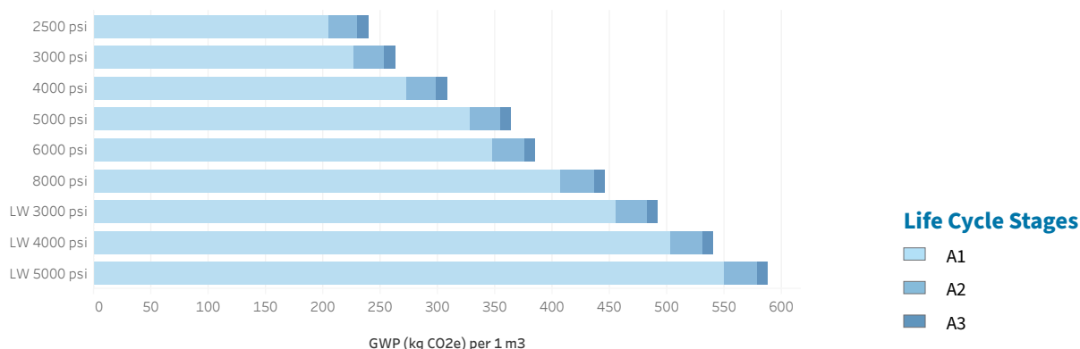
Figure 1. GWP contribution by life cycle stage. This chart is an approximation. Total GWP values are based on the NRMCA USA national benchmark GWP values per 28-day strength class. CLF calculated the approximate industry-average percent contribution by life cycle stage per strength class by averaging the minimum and maximum percent contributions by strength class provided in Table 15 of the NRMCA industry EPD background LCA report. 1
