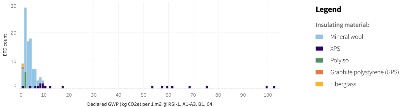
Figure 11. Board insulation product EPDs by insulating material.
