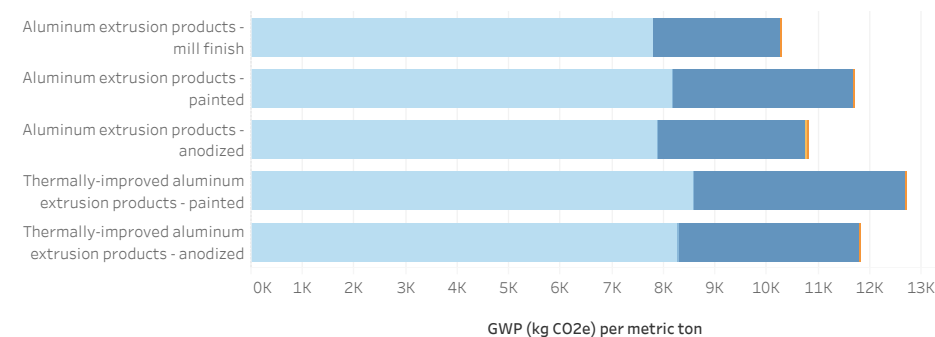
Figure 1. GWP contribution by life cycle stage. A1 = primary aluminum production and processing of recycled aluminum to create semi-finished products; A2 = transport of semi-finished products to extrusion manufacturing facility; A3 = extrusion, thermal improvement, surface treatment; C2 = end-of-life transport; C4 = disposal. A2, C2, and C4 are not visible or barely visible in this chart due to their relatively small values. D stage impacts are also included in the industry EPDs but are excluded here.
