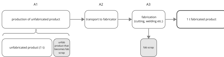
Figure 2. Life cycle stages and fabrication scrap in fabricated steel product EPDs.
