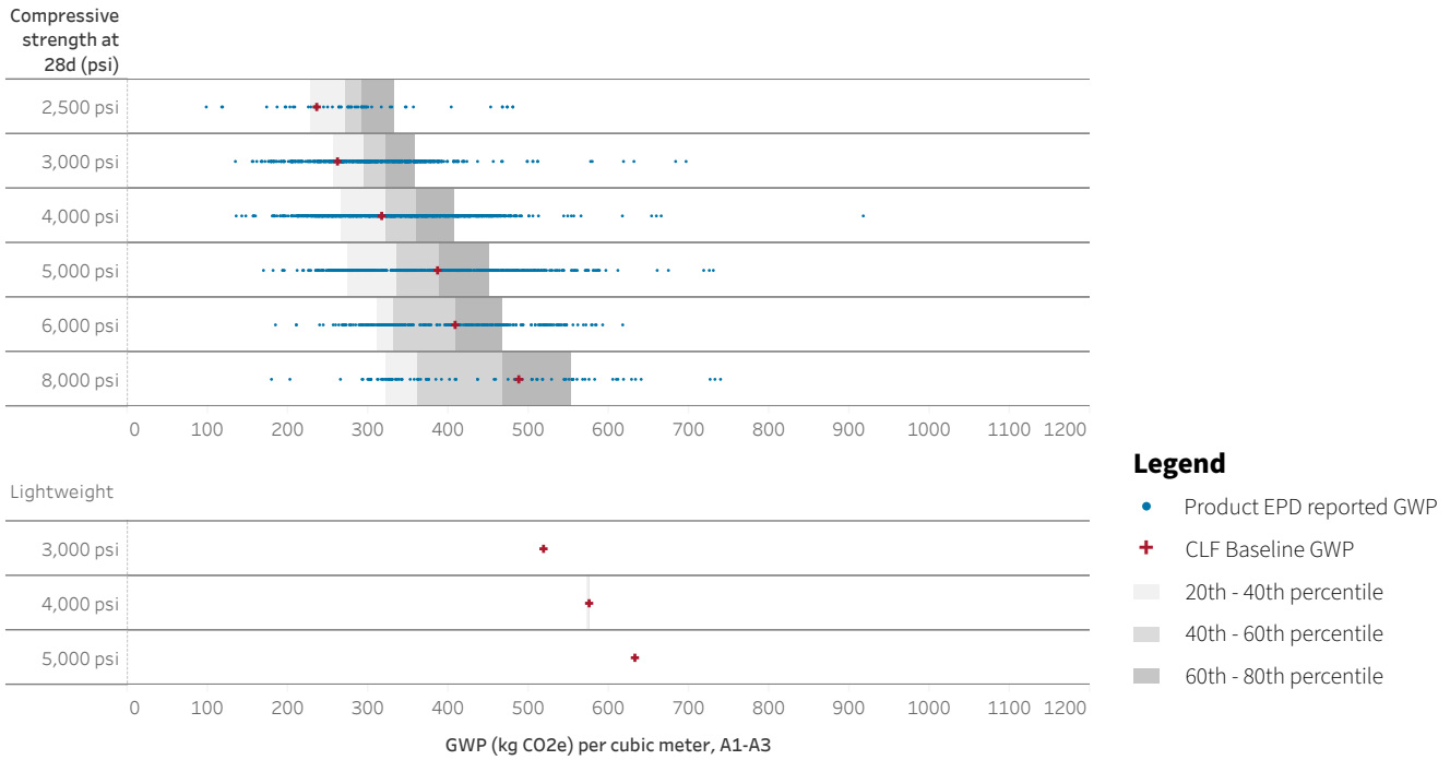
Figure 13. Range of applicable product EPDs and CLF Baselines.
