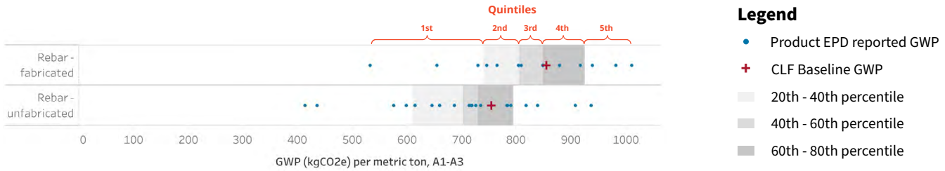
Figure 3. [Example one-dimensional scatter plot] Range of applicable product EPDs and CLF Baselines.
