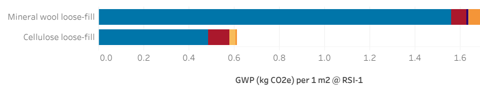
Figure 1. GWP Contribution by Life Cycle Stage. The IW-EPDs for mineral wool and cellulose loose-fill insulation aggregate stages A1-A3, and also include additional stages A4, A5, C2, and C4. There is no IW-EPD for fiberglass loose-fill insulation.
