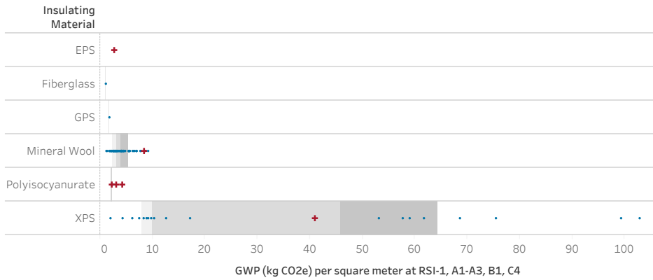
Figure 4. Range of applicable product EPDs and CLF Baselines, including XPS. Scope includes A1-A3, B1, and C4, unlike most categories in this report. For non-XPS products, B1 generally equals zero and C4 is negligible (approximately 1% or less of total GWP).
