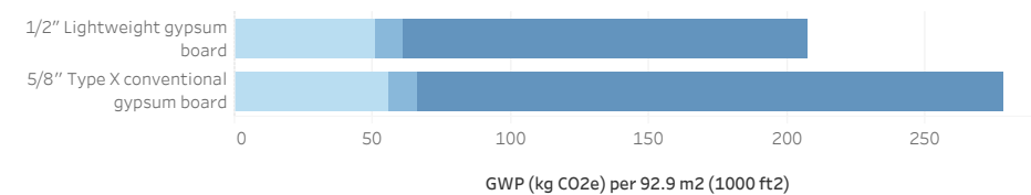
Figure 1. GWP contribution by life cycle stage. A1: extraction and upstream production, including gypsum mining to procure gypsum ore and gypsum facing and backing paper production. A2: transport of gypsum ore and gypsum paper to gypsum board product manufacturing facility. A3: gypsum board product manufacture: heating / dehydrating natural gypsum, mixing, forming into boards, drying.
