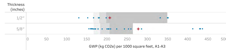
Figure 2. Range of applicable product EPDs and CLF Baselines.
