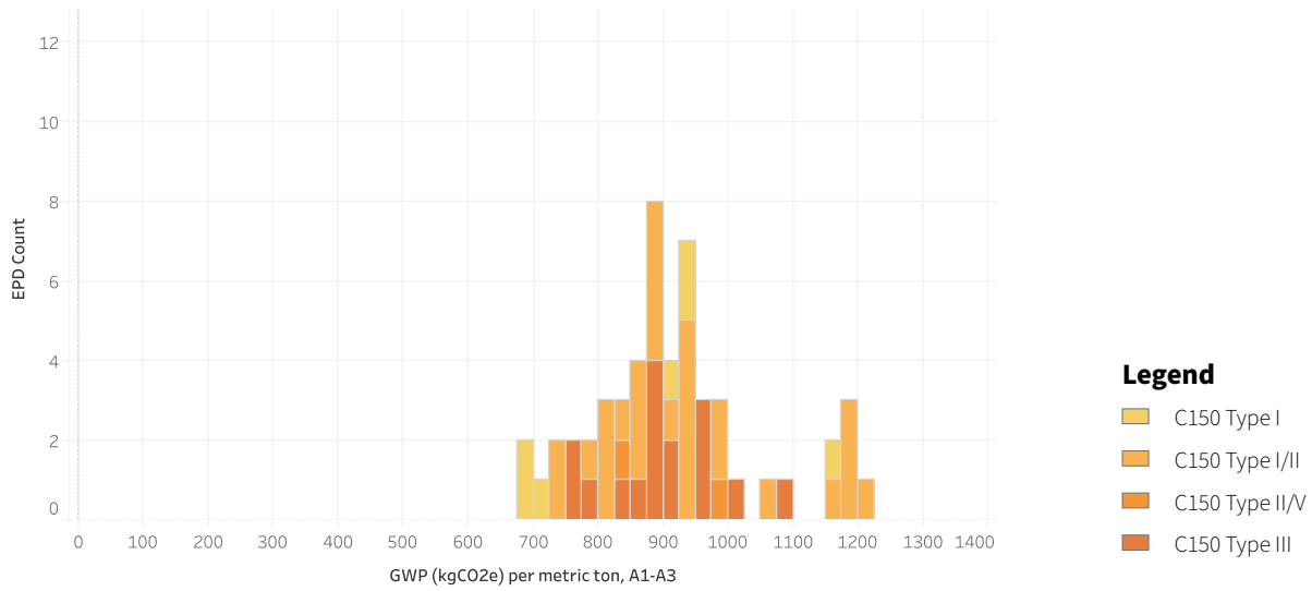
Figure 9. Portland cement EPD GWP distribution by ASTM C150 type.
