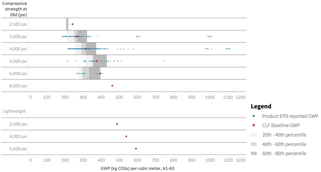
Figure 19. Range of applicable product EPDs and CLF Baselines.
