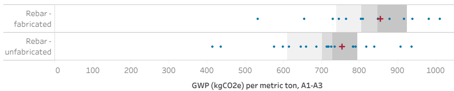
Figure 2. Range of applicable product EPDs and CLF Baselines.
