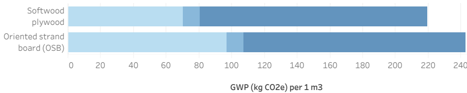
Figure 2. [Example] GWP Contribution by Life Cycle Stage.
