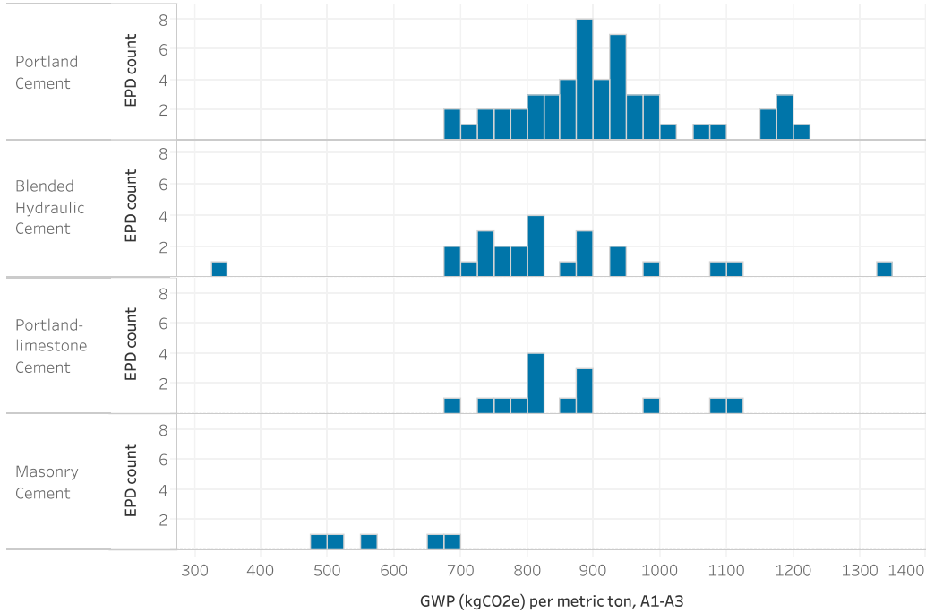
Figure 4. Distribution of applicable product EPDs.
