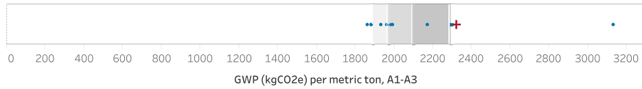
Figure 2. Range of applicable product EPDs and CLF Baseline.
