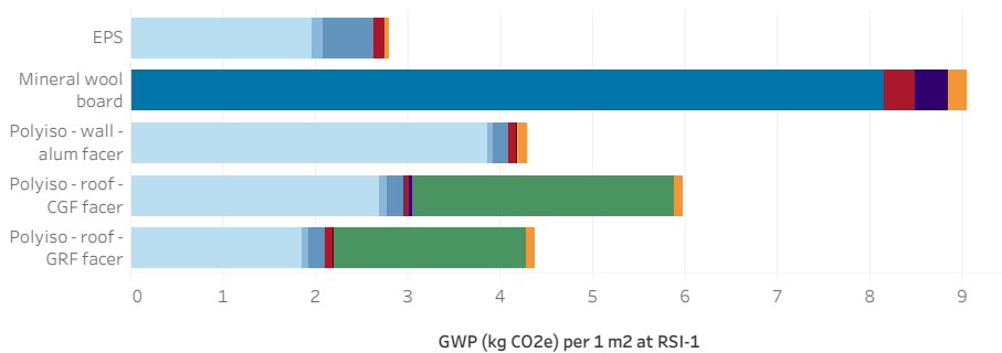
Figure 1. GWP contribution by life cycle stage. Board insulation, excluding XPS. Data for EPS, polyiso wall and roof boards, and heavy-density mineral wool boards are from the industry-wide EPDs.
