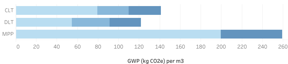
Figure 1. GWP contribution by life cycle stage. As there are no industry EPDs for this product type, the information displayed here is from product EPDs. For DLT and MPP, this is based on the one EPD available for each. 4,5 For CLT, this is based on an average of the collection of applicable product EPDs.
