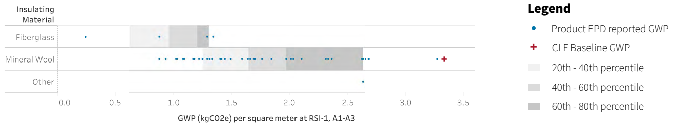
Figure 2. Range of applicable product EPDs and CLF Baseline.
