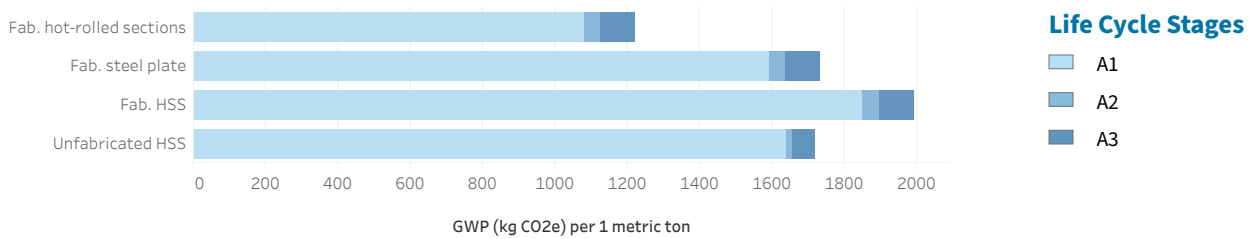
Figure 1. GWP Contribution by Life Cycle Stage. For the three fabricated product types, A1 = making of the steel shape including steel production, hot rolling, and additional production steps for plate and HSS; A2 = transport to fabricator; A3 = final fabrication. For the unfabricated HSS, A1 = steelmaking to coil production; A3 = HSS manufacture.
