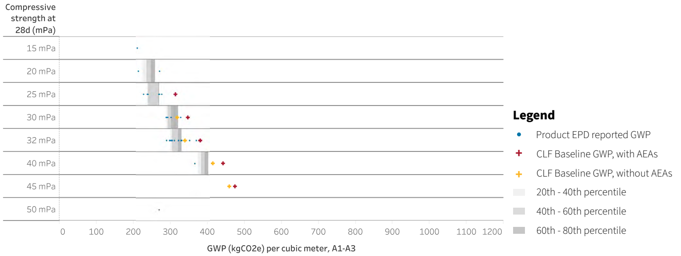
Figure 31. Range of applicable product EPDs and CLF Baselines.
