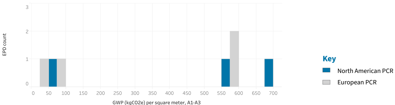
Figure 3. Range of global processed IGU product EPDs.
