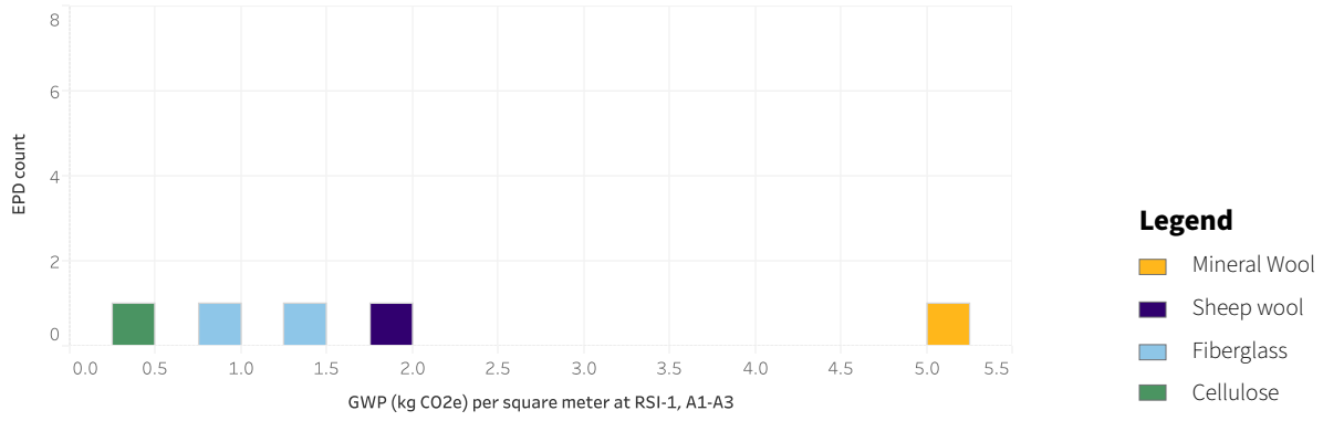
Figure 6. Loose-fill insulation product EPDs by insulating material. Given the functional similarity of the different loose-fill insulation product types, this chart provides context for their comparative GWP values.
