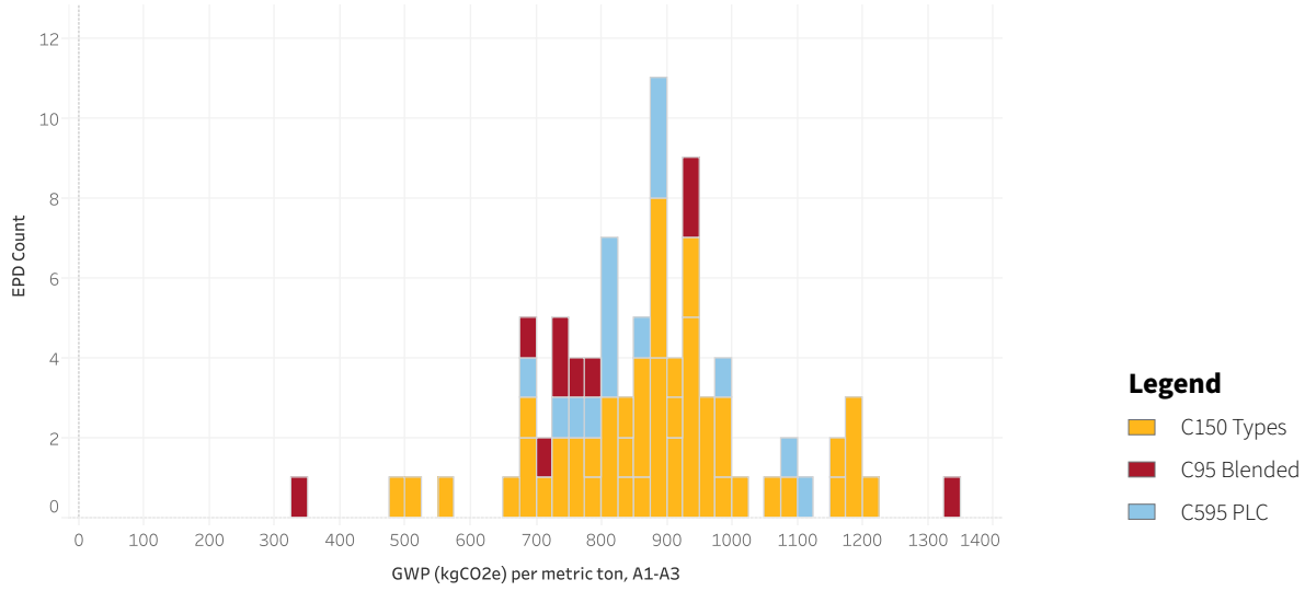
Figure 8. GWP distribution of EPDs - combined. While these product types – portland cement, portland-limestone cement, and blended hydraulic cement – have separate CLF Material Baselines, they are combined in this chart to provide further context for their comparative GWP values.
