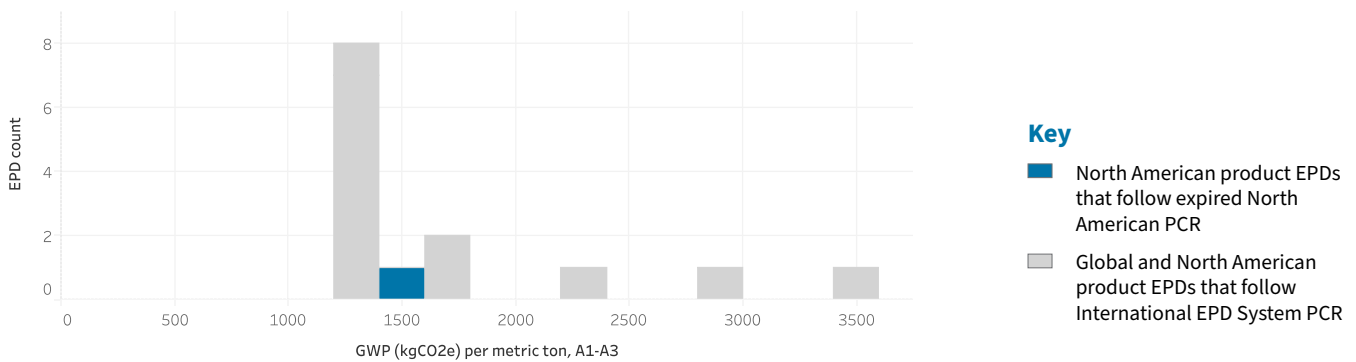
Figure 5. Range of global flat glass product EPDs.
