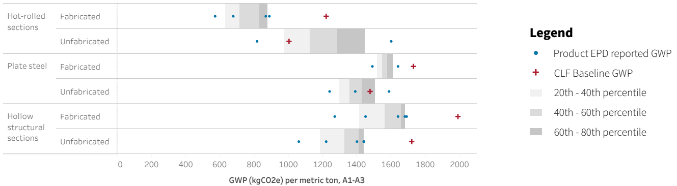
Figure 2. Range of marginally applicable product EPDs.
