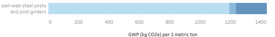
Figure 1. GWP Contribution by Life Cycle Stage. A1 = steel making and hot rolling to produce structural steel shapes; A2 = transport to OWSJ manufacturing facility; A3 = fabrication of OWSJ.
