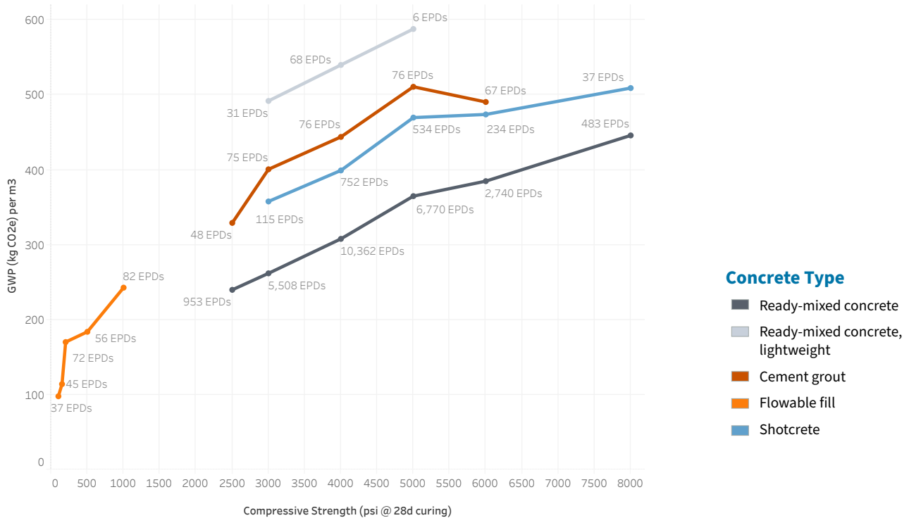
Figure 1. Concrete GWP and EPD count by type and compressive strength. This chart describes USA concrete EPDs. Each type-compressive strength data point (e.g., shotcrete-4000 psi) includes a count of the applicable product EPDs in CLF’s data set and the average A1-A3 GWP per m 3 (location along the y-axis).
