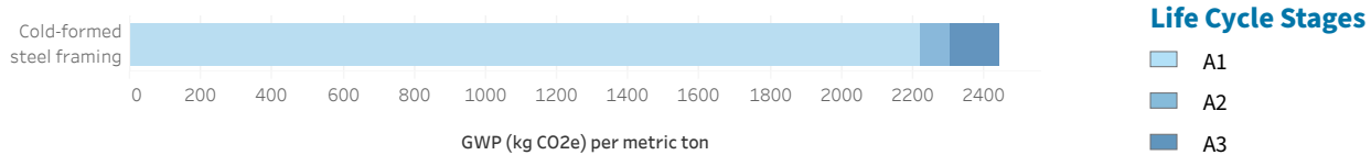
Figure 1. GWP Contribution by Life Cycle Stage. A1 = steelmaking, rolling into coil, hot-dip galvanization; A2 = transport of hot-dipped galvanized coil to manufacturing facility; A3 = manufacture of steel framing members via roll forming.
