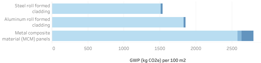
Figure 1. GWP contribution by life cycle stage. A1 = steelmaking and aluminum-making, rolling into coil, plastics production (MCM only); A2 = transport of coil and plastic to roll forming or MCM facility; A3 = manufacture of panels via roll forming or laminating.
