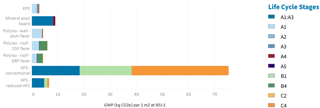
Figure 2. GWP contribution by life cycle stage. Board insulation, including XPS. Data for EPS, polyiso wall and roof boards, and heavy-density mineral wool boards are from the industry-wide EPDs. The data for XPS (one set for conventional blowing agent mix, one set for reduced-HFC blowing agent mix) are averages from a collection of product EPDs.
