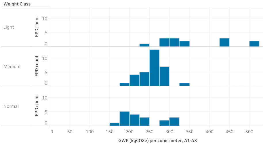
Figure 4. Distribution of applicable product EPDs.
