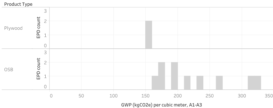
Figure 3. Range of global wood sheathing product EPDs. These are not applicable to the CLF Baselines and are shown here for reference only.
