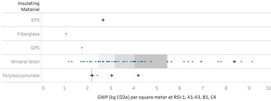
Figure 3. Range of applicable product EPDs and CLF Baselines, excluding XPS. Scope includes A1-A3, B1, and C4, unlike most categories in this report. For non-XPS products, B1 generally equals zero and C4 is negligible (approximately 1% or less of total GWP). XPS is excluded here to better see the data points on a horizontal axis scale of 0 - 10.
