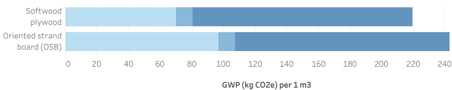
Figure 1. GWP Contribution by Life Cycle Stage. A1 = roundwood (including forestry operations) and resin production; A2 = transport to mill; A3 = plywood / OSB manufacturing.
