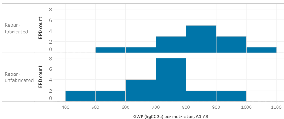
Figure 4. Distribution of applicable product EPDs.
