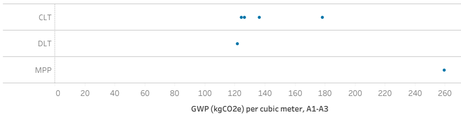
Figure 2. Range of applicable product EPDs. In other appendices, this figure also includes CLF Baseline values. There are no 2023 CLF Baselines for mass timber panel product types.
