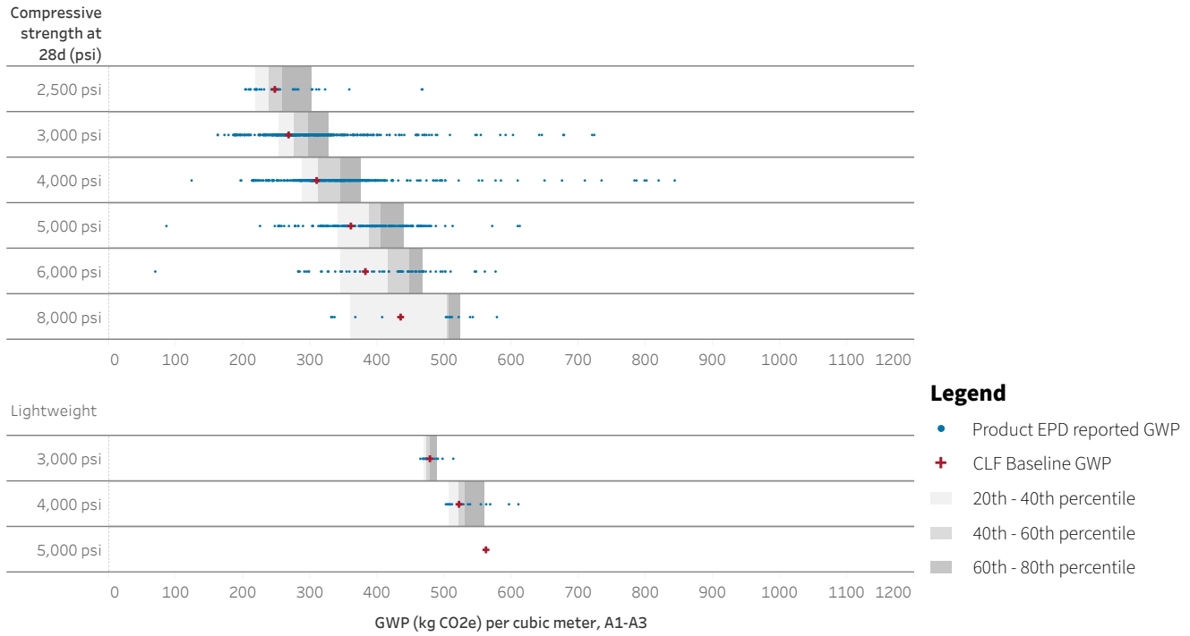
Figure 21. Range of applicable product EPDs and CLF Baselines.
