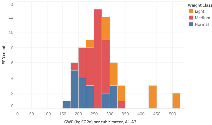
Figure 7. Distribution of product EPD GWP by weight class.
