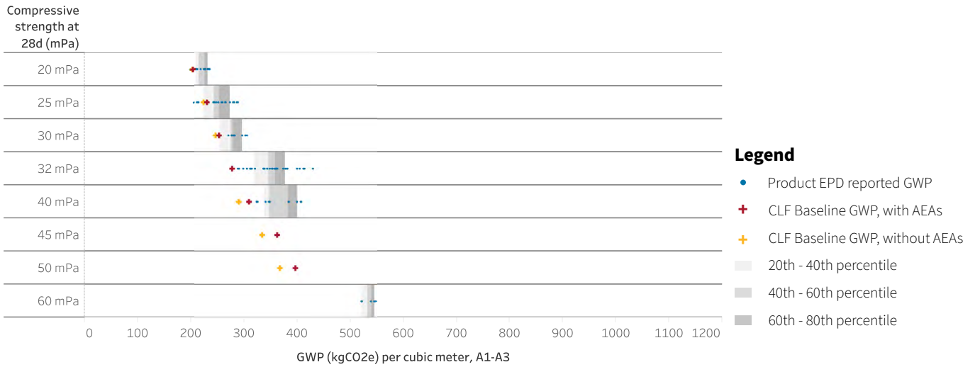
Figure 33. Range of applicable product EPDs and CLF Baselines.
