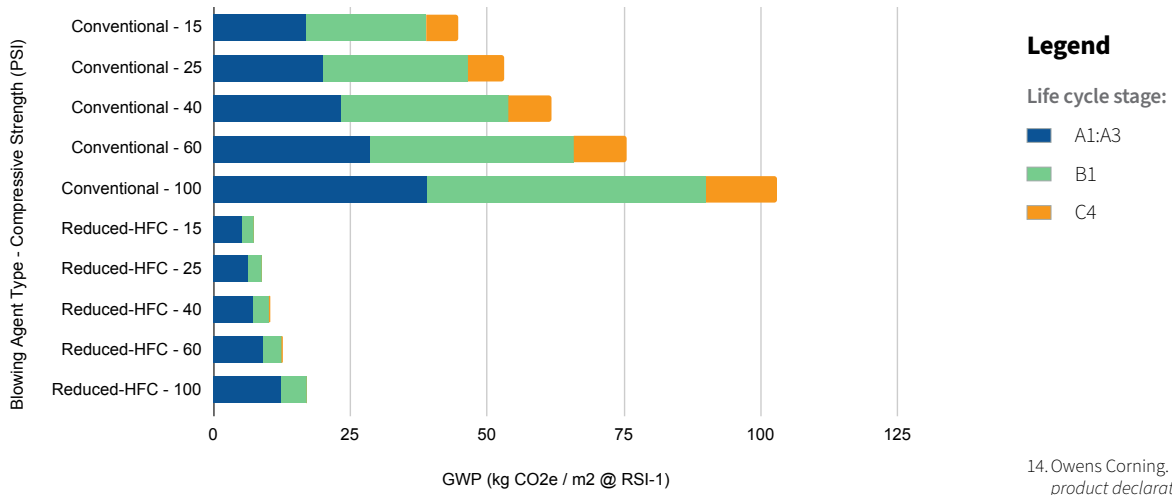
Figure 12. XPS compressive strength vs. GWP (kg CO 2 e per 1 m 2 at RSI-1). One manufacturer's conventional and reduced-HFC blowing agent products are included. 14
