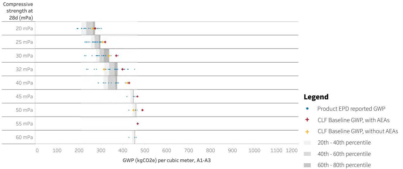
Figure 29. Range of applicable product EPDs and CLF Baselines.
