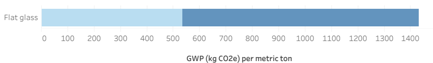
Figure 1. GWP contribution by life cycle stage. The flat glass industry-wide EPD reports cradle-to-gate performance broken down by raw material extraction (including transport of the materials to the glass manufacturer, all shown as A1 in this chart) and flat glass production (A3).
