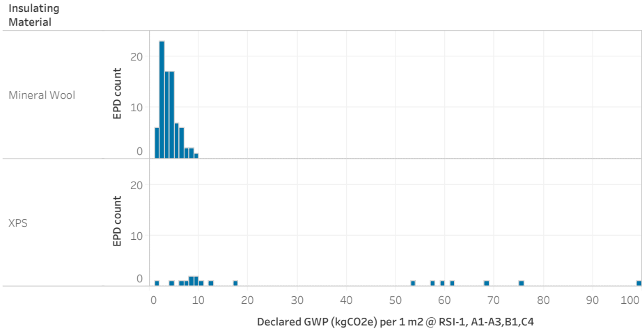
Figure 6. Distribution of applicable product EPDs. Life cycle stages in product EPD data. The summary statistics in Figure 4 aim to represent life cycle stages A1-A3 (product stage), B1 (to account for blowing agent emissions during building life), and C4 (to account for blowing agent emissions during disposal). For XPS, B1 and C4 impacts are significant. For non-XPS board insulation products (that are not responsible for GHG emissions due to blowing agent leakage after manufacturing), B1 GWP is zero and C4 is negligible.
