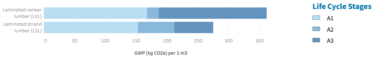
Figure 1. GWP contribution by life cycle stage. A1 = roundwood (including forestry operations), resin, and veneer (where applicable) production; A2 = transport to mill; A3 = SCL manufacturing.
