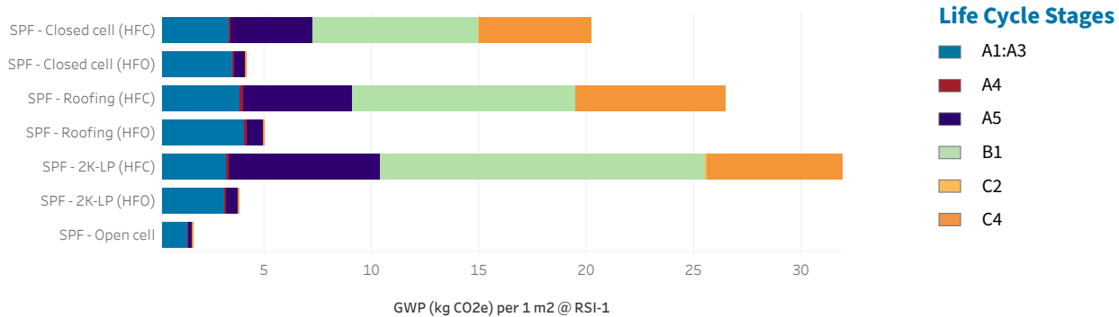
Figure 2. GWP Contribution by Life Cycle Stage. The IW-EPDs for spray polyurethane foam insulation aggregate stages A1-A3, and also include stages A4, A5 (when the foam is produced on-site), B1 (accounting for blowing agent emissions during the life of the building), C2 (negligible impacts), and C4 (dominated by blowing agent emissions after disposal). 1,2
