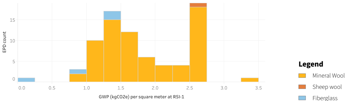
Figure 8. Blanket insulation product EPDs by insulating material. Given the functional similarity of the different blanket insulation product types, this chart displays the same data points as the charts above but grouped together to provide further context for their comparative GWP values.
