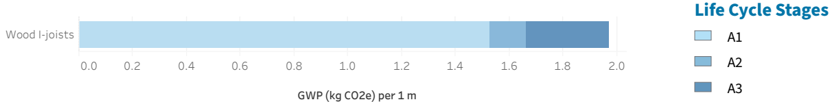
Figure 1. GWP Contribution by Life Cycle Stage. A1 = production of input materials: chord and web materials and resins; A2 = transport to manufacturing facility; A3 = manufacture of I-joists.
