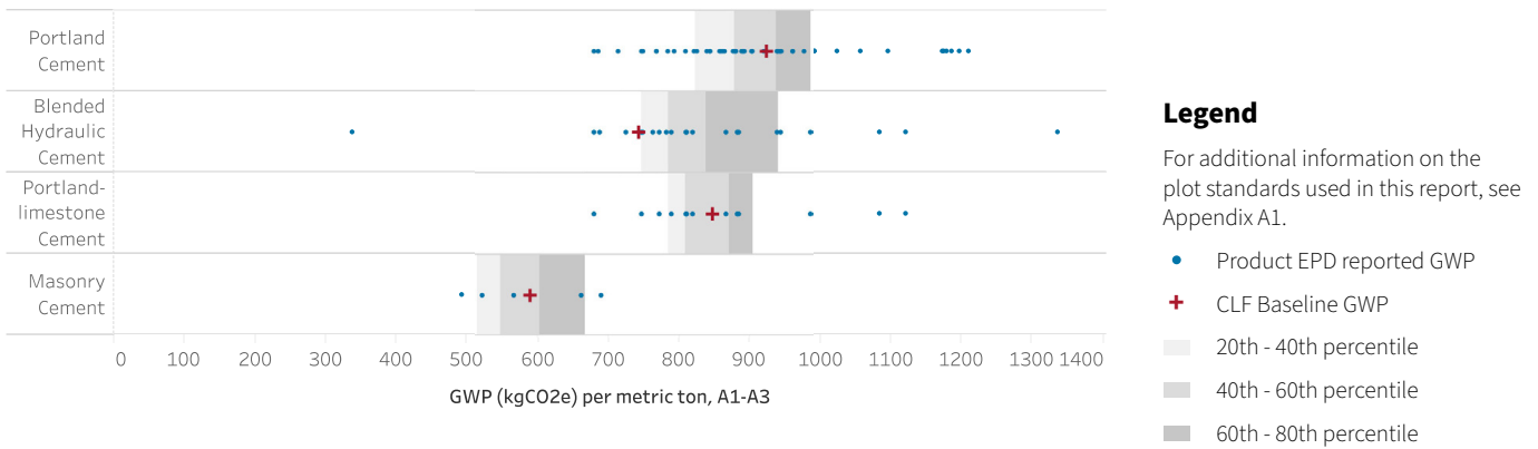
Figure 2. Range of applicable product EPDs and CLF Baselines.
