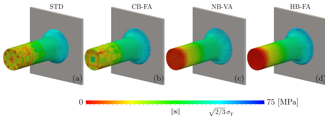
Figure 7.3: \|\mathbf{s}\| at T = 0.25 for different MPM strategies. (a) The standard MPM [STD] (b) Cell-based full approximation [CB-FA] (c) Node-based volumetric approximation [NB-VA] and (d) Hybrid-based full approximation [HB-FA].
