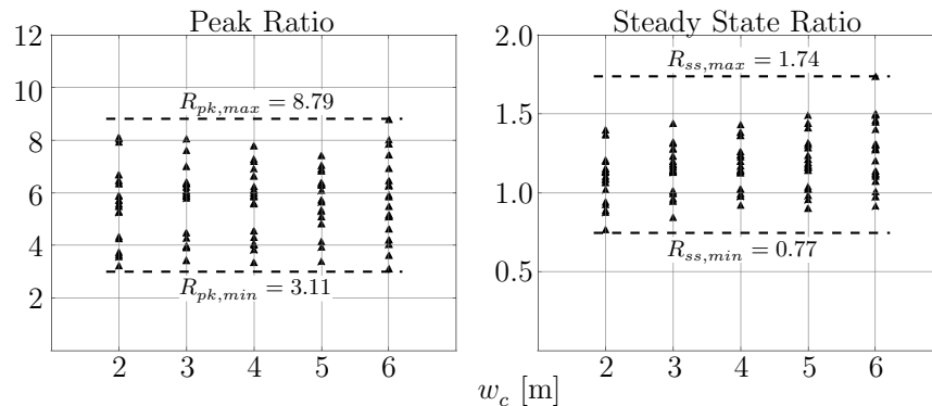
Figure 7.46: Peak and steady state to static force equivalent for select data points.
