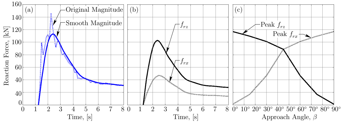
Figure 7.51: Reaction force comparison. (a) Reaction force magnitude before and after smoothing as a function of time. (b) The x and z components of the reaction force as a function of time for \beta = 30^\circ . (c) Peak force as a function of approach angle.
