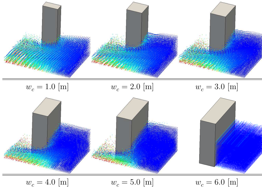
Figure 7.32: Isometric view of plastic deformation at t = 3.0 s for \phi_F = 10^\circ and H_b = 3.5 [m]. The column width increases until it forms a rigid barrier. The red particles have |\epsilon_p| = 10.0 while the blue particles have |\epsilon_p| \approx 0.0 .
