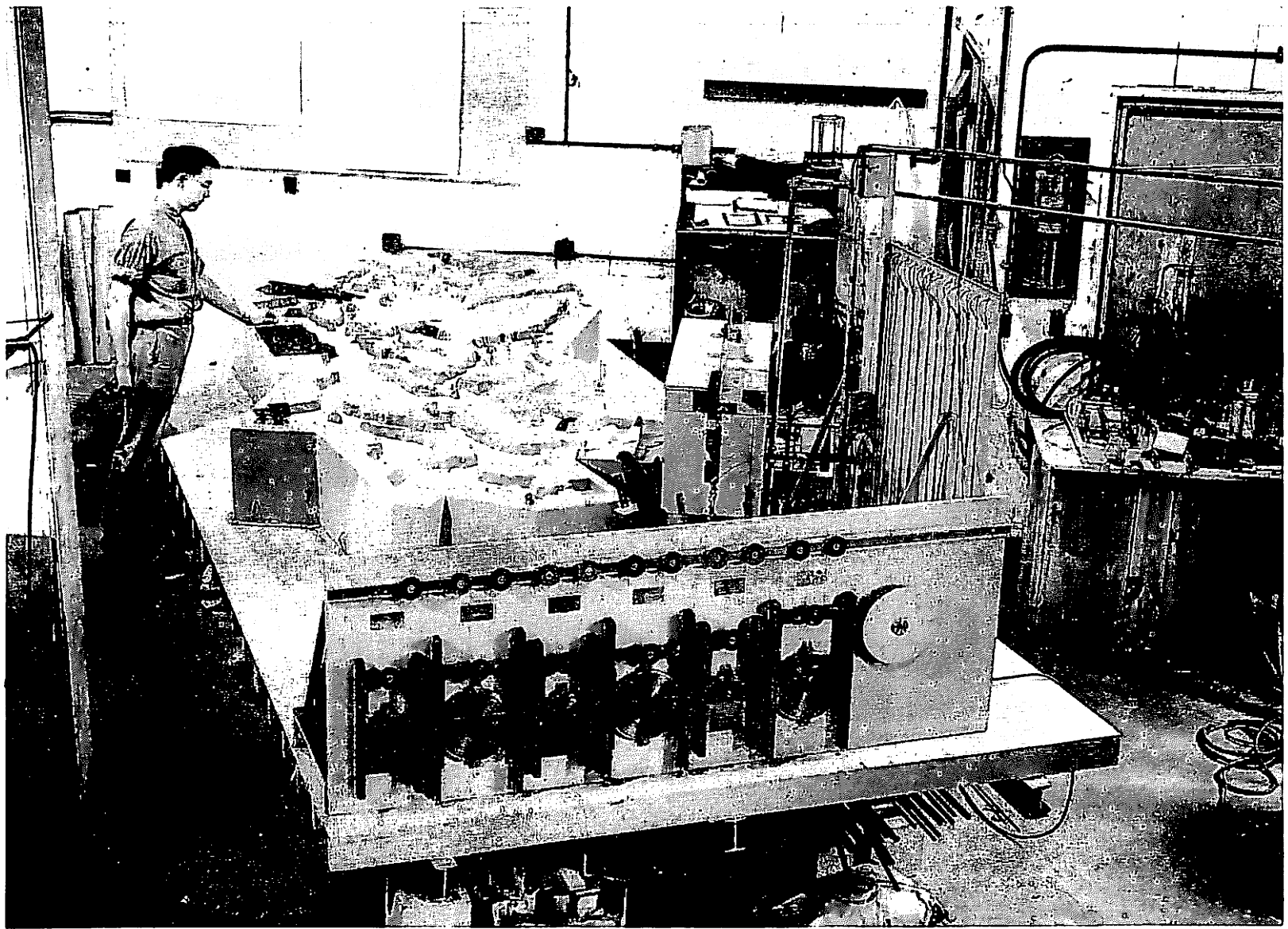
FIGURE 4. Completed model basin.
