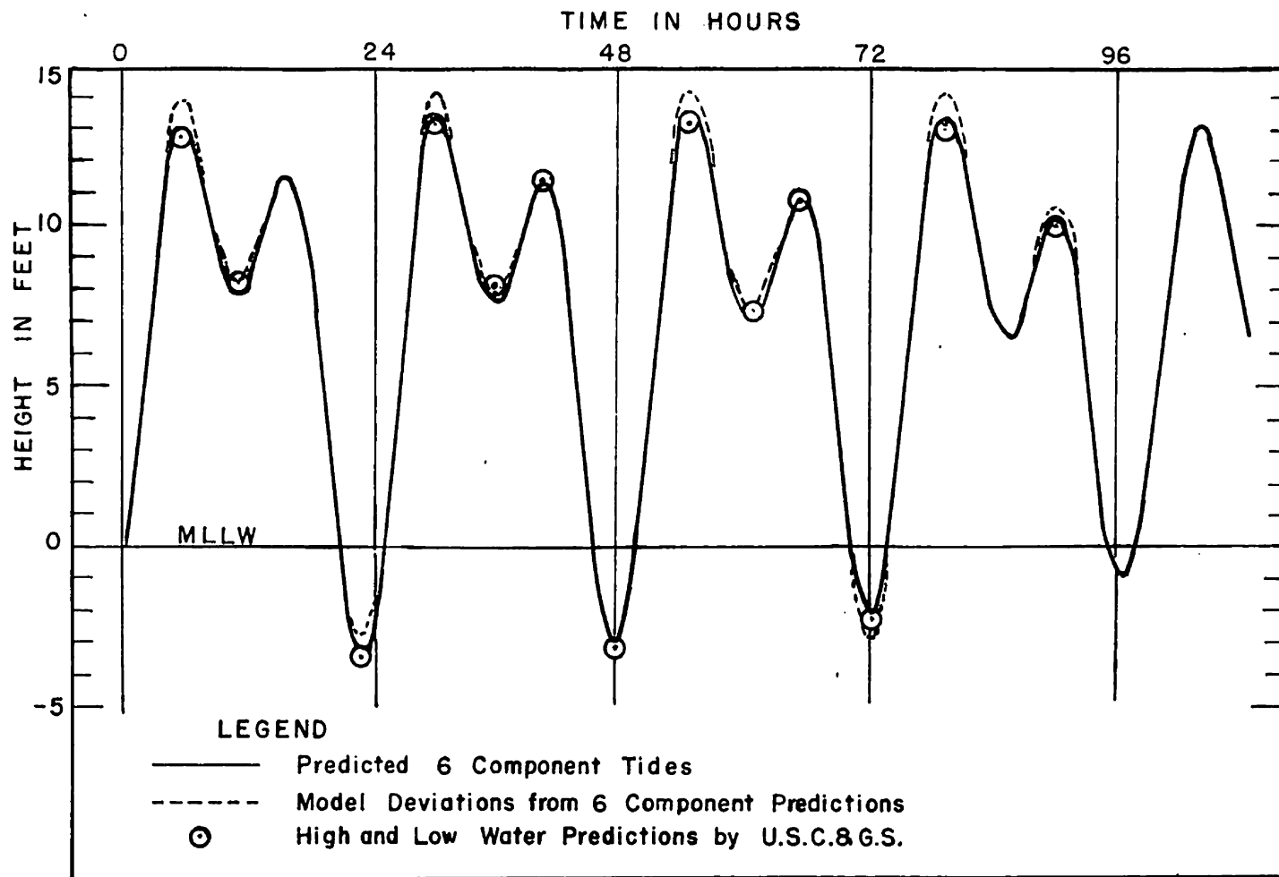
FIGURE 6. Comparison of prototype and model tides of Puget Sound, based on six components and corresponding heights of high and low water taken from the U. S. C. & G. S. Tide Tables.
