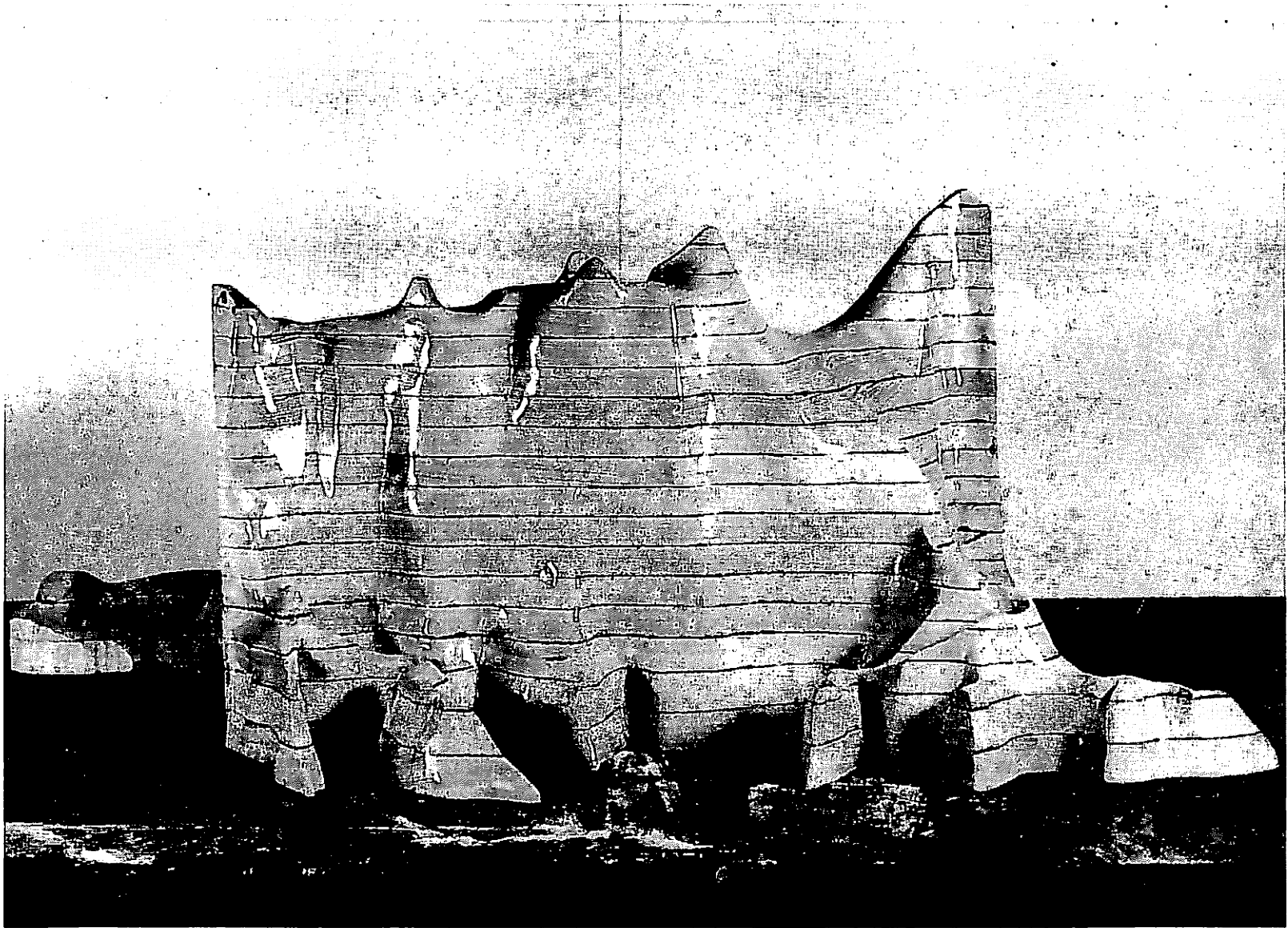
FIGURE 2. Wood pattern for casting section of basin.
