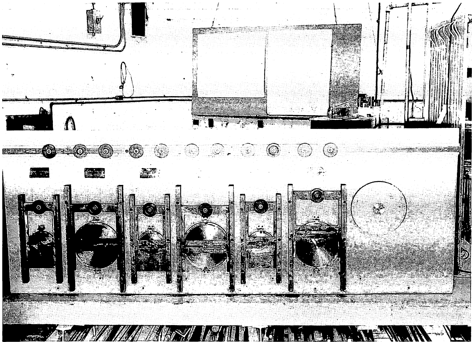
FIGURE 5. Tide machine panel showing Scotch yokes, summation wire and reduction drum.
