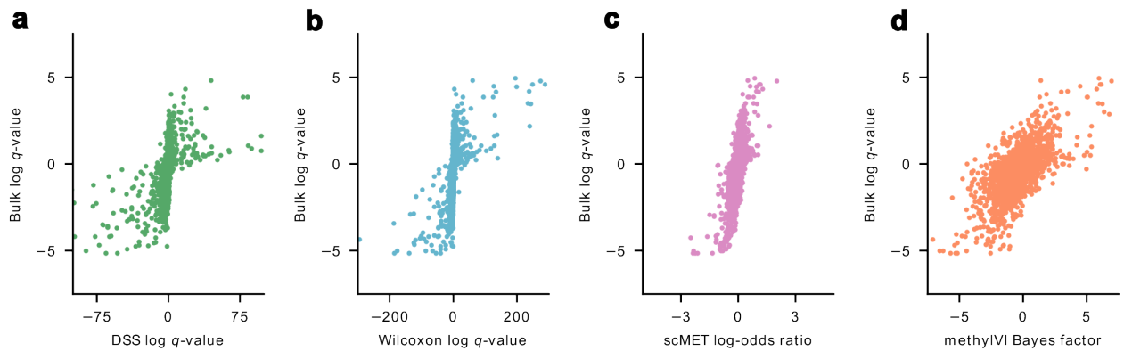
Figure A.5.5: CpG differentially methylated gene test results for MethylVI and baseline methods. a-d, MethylVI and baseline differentially methylated gene testing results when applied to CpG gene body methylation features for excitatory versus inhibitory neurons from Luo et al.[111] based on consistency vs results from bulk data.
