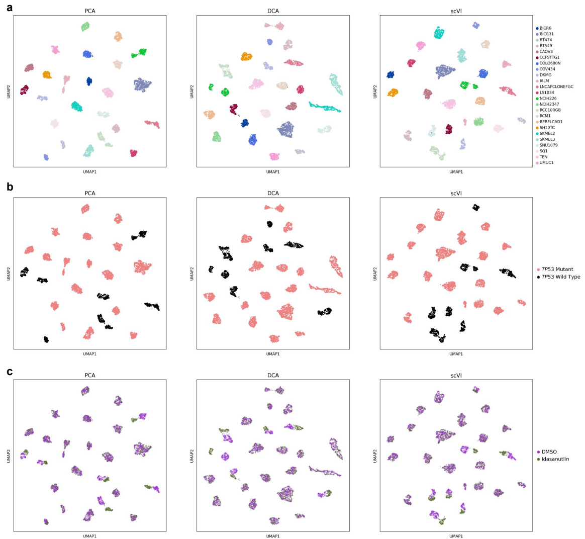
Figure A.4.4: Latent representations of non-contrastive baseline models for McFarland et al. [115] a-c, UMAP plots of noncontrastive baseline workflows. Here we depict the results of a standard scRNA-seq analysis workflow (i.e., normalization followed by principal component analysis and UMAP) as well as the latent representations learned by DCA and scVI. Plots are colored by cell line (a), TP53 mutation status (b) and treatment (c).
