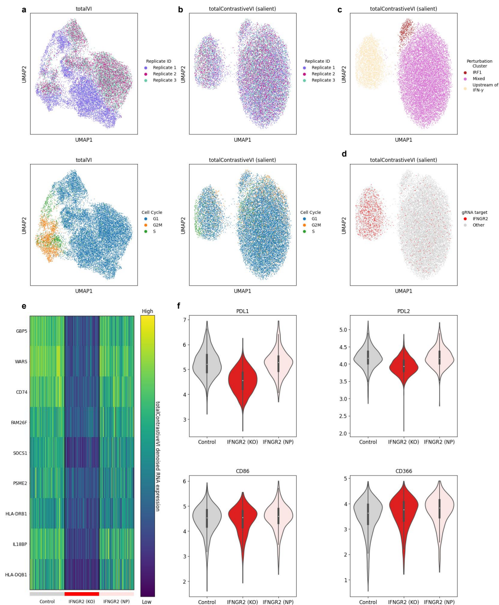
Figure 4.4: Applying to totalContrastiveVI to isolate perturbation-induced variations in joint RNA and protein measurements. a-b , UMAP visualizations of totalVI's embeddings ( a ) and totalContrastiveVI's salient embeddings ( b ) colored by replicate number and cell cycle stage. c , Visualization of the three clusters revealed in the totalContrastiveVI salient latent space. d , Visualization of cells that expressed IFNGR2 gRNA in totalContrastiveVI's salient latent space. e , totalContrastiveVI denoised RNA expression levels (log library size normalized; Section 4.B) of immune-related genes for control cells, cells with knocked out (KO) IFNGR2 genes, as well as cells expressing IFNGR2 gRNA but which were non-perturbed (NP). f , Distributions of log(totalContrastiveVI denoised protein + 1) for control cells as well as the IFNGR2 KO and NP cells.
