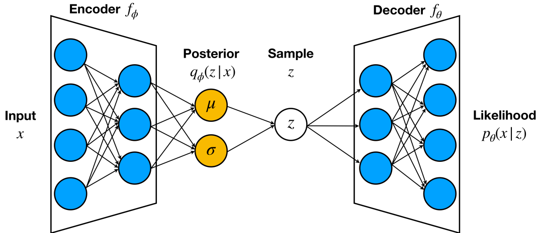
Figure 2.1: The variational autoencoder architecture. An encoder neural network transforms maps an observed data points to the approximate posterior distribution of its latent variables. Samples from the posterior are then transformed back to the parameters of a likelihood function in the original data space via a corresponding decoder neural network.
