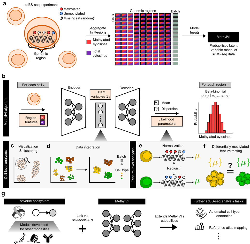
Figure 5.2: Overview of MethyIVI. a , For each cell, an scBS-seq experiment produces a set of binary values indicating whether a cytosine is methylated (red) or unmethylated (blue). To accommodate variable cytosine coverage across cells, cytosine-level measurements are aggregated across predefined genomic regions (e.g., gene bodies) to produce two values per region: the number of methylated cytosines (red) and total number of covered cytosines (purple). These aggregated region features are used as input to the MethyIVI model. b , The MethyIVI algorithm. For each cell i , a vector \mathbf{y}_i containing the number of methylated cytosines at each region and a vector \mathbf{n}_i containing the total number of profiled cytosines at each region are fed as inputs to the model. These vectors are transformed into the posterior distribution of \mathbf{z}_i , a lower-dimensional representation of the given cell's state. c-d , These latent representations can be used as input to clustering or visualization algorithms ( c ) and enable integration of datasets across experimental conditions when corresponding covariates are provided as model inputs ( d ). e-f , A cell's latent representation is transformed to the parameters of a beta-binomial distribution, which can assist with feature-level tasks, such as estimating normalized methylation levels \mu within genomic regions ( e ) or performing differentially methylated gene testing ( f ). g , Our scvi-tools [53] implementation facilitates further extension of MethyIVI's capabilities using components from other scverse [165] probabilistic models developed for additional analysis tasks, but which were originally designed for other modalities.
