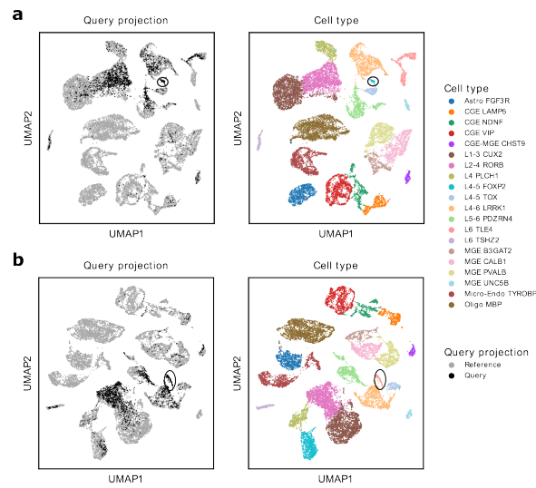
Figure A.5.8: Assessing the robustness of our MethylANVI plus scArches reference atlas mapping workflow to cell types not present in the reference data. a-b , For these experiments L4-5 FOXP2 neurons ( a ) or L6 TLE4 neurons ( b ) were held out from the reference data while remaining in the query dataset. Black circles indicate cell types held out from the reference.
