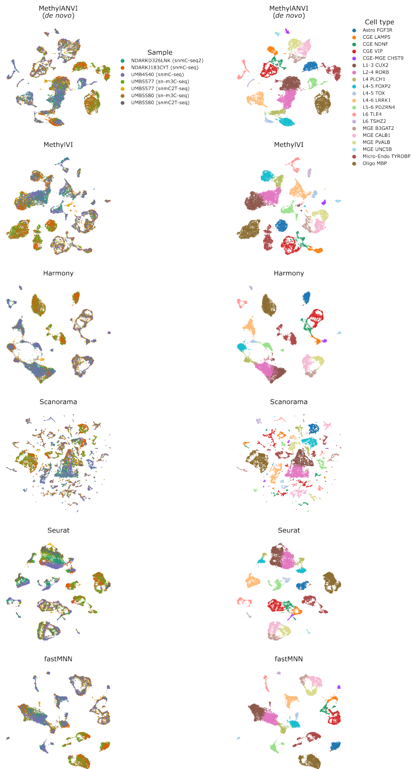
Figure A.5.7: Qualitative atlas integration results for de novo integration baselines on the frontal cortex data from Luo et al. [113].
