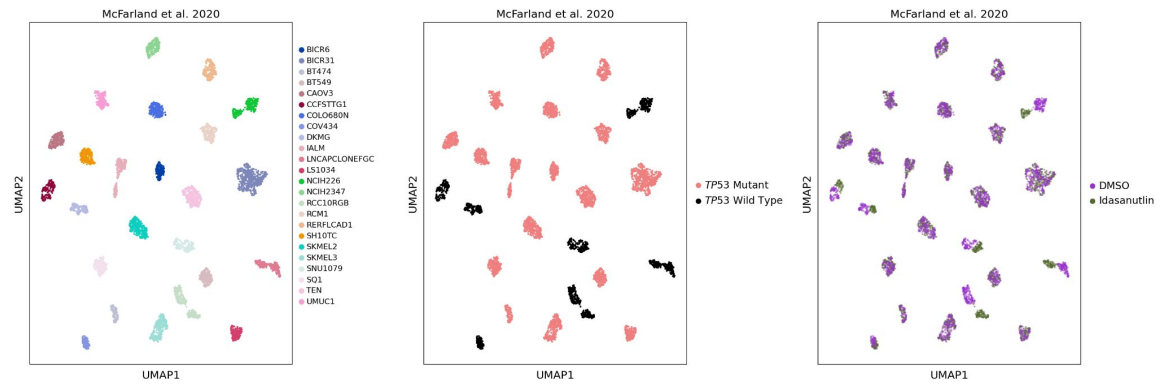
Figure A.4.1: Visualization of MIX-seq dataset from McFarland et al. [115] using the visualization workflow of McFarland et al. [115]. The MIX-seq dataset from McFarland et al. [115] is visualized using the original workflow of McFarland et al. [115] (i.e., applying UMAP to normalized count data). The plots are colored by cell line (left), TP53 mutation status (center), and treatment (right).
