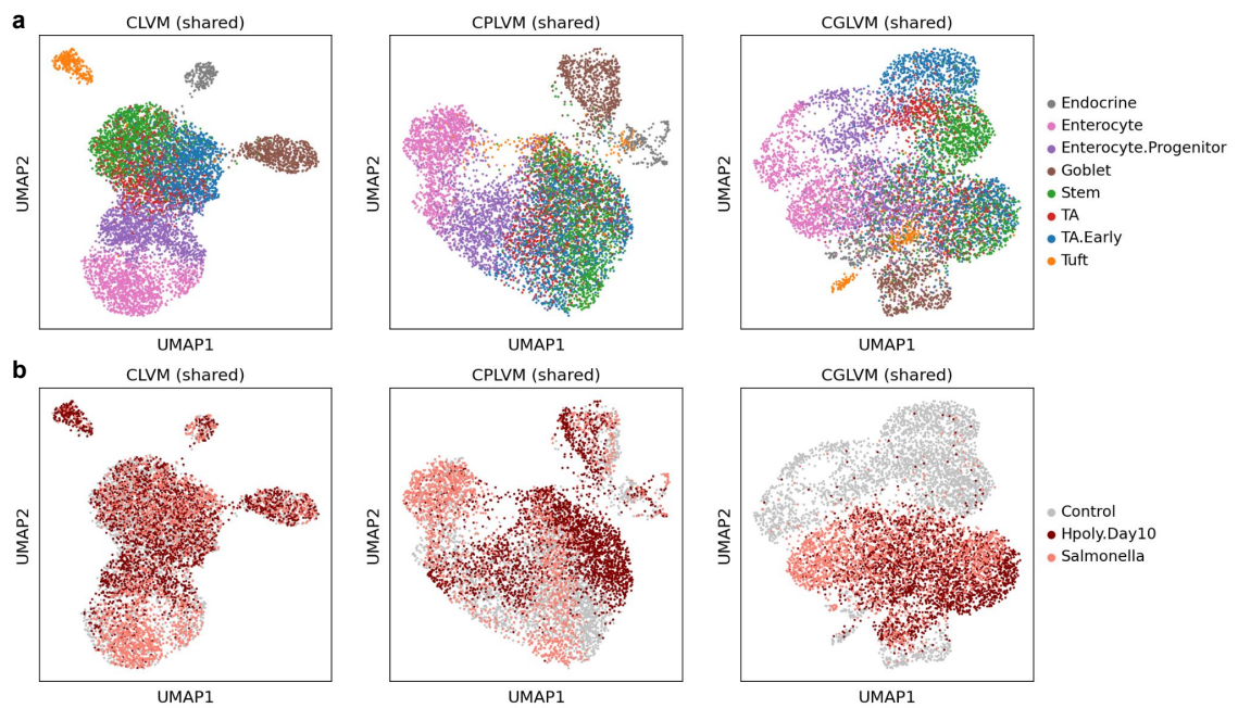
Figure A.4.5: Baseline contrastive models' shared latent representations of Haber et al. [64] a-b , UMAP plots depicting baseline contrastive models' shared latent representations of all cells (i.e. treatment and control) from the mice intestinal epithelial cell infection dataset from Haber et al. [64]. Cells colored by cell type (a) and infection (b).
