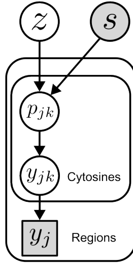
Figure 5.1: The MethylVI generative process. We assume that the probability of an individual cytosine k in region j being methylated ( p_{jk} ) is generated conditional on a cell’s underlying state ( z ). The methylation statuses of individual cytosines ( y_{jk} ) are then summed up to obtain the total number of methylated cytosines in a region ( y_j ). Shaded nodes denote observed values, while unshaded nodes correspond to hidden values. Square nodes denote variables whose values are computed deterministically from random variables.
