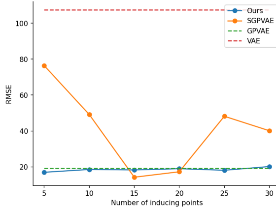
Figure 6.2: Assessing the impact of the number of inducing points on the moving ball dataset. For different numbers of local inducing points h , we trained FA-SGPVAE models and assessed their performance at recovering videos’ latent trajectories. We similarly assessed the performance of varying the number of global inducing points m for SGPVAE. For comparison we also include results from training a standard VAE and the full GPVAE model.
