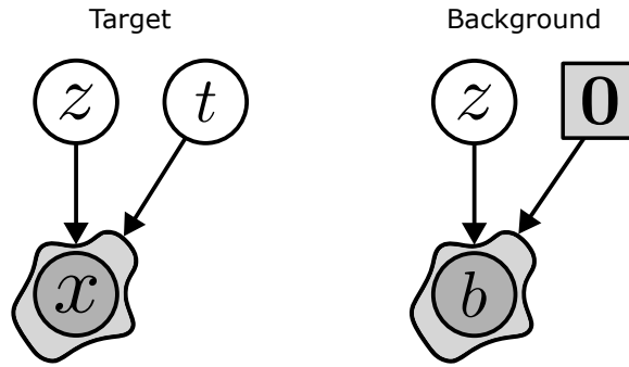
Figure 4.1: The ContrastiveVI generative process. Target (i.e., perturbed) cells are assumed to be generated from two sets of latent variables with distinct semantic meanings. Shared variables z correspond to perturbation-agnostic variations shared with controls, while salient variables t capture perturbation-induced effects. Background (i.e., control) cells are assumed to be generated solely from z with the salient variables t fixed at a constant.
