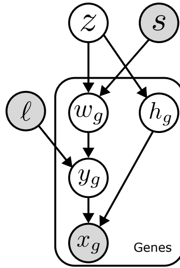
Figure 2.1: Graphical model depiction of the single-cell variational inference (scVI) model of Lopez et al. [107]. Shaded nodes indicate observed variables, unshaded nodes indicate hidden variables, and plates denote independent replication.
