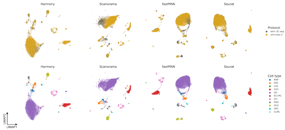
Figure A.5.1: UMAP plots of dentate gyrus methylome data from Liu et al. [102] after integration across sequencing protocols with baseline data integration methods.
