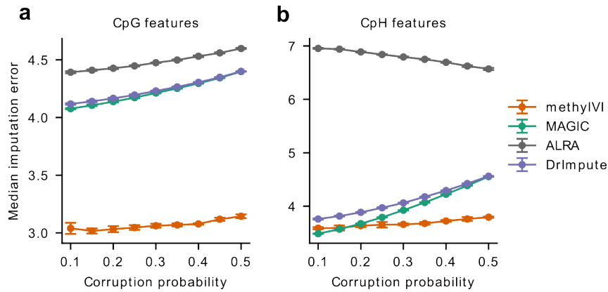
Figure A.5.2: Benchmarking MethyVI's ability to recover methylation levels in cells for features with no coverage. a-b, Investigation of MethyVI and baseline methods' ability to recover missing values for CpG features (a) and CpH features (b) from Luo et al. [111], where coverage levels were randomly corrupted (i.e., set to zero) for a range of probabilities.
