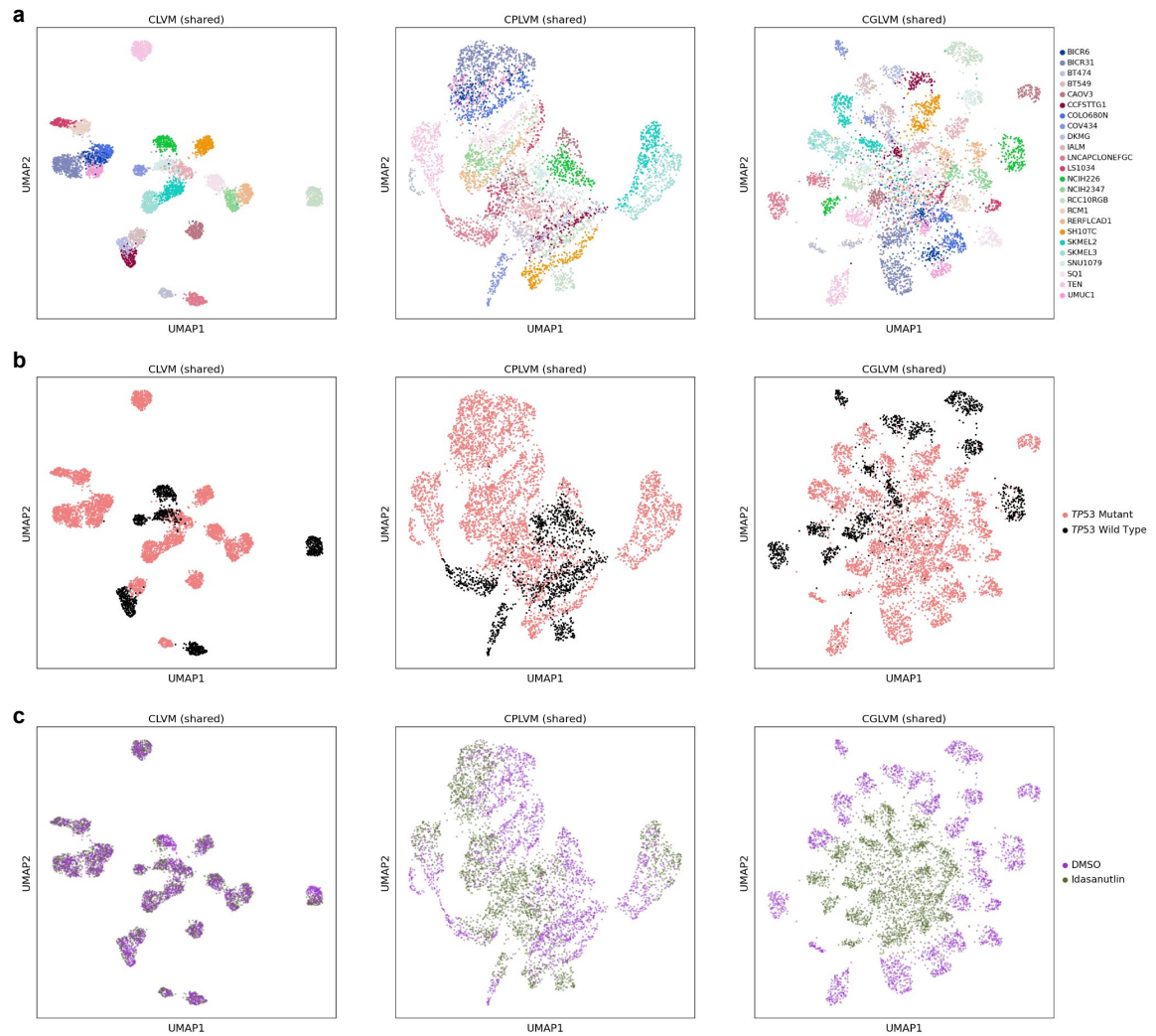
Figure A.4.2: Shared latent representations of baseline contrastive models for McFarland et al. [115] a-c, UMAP plots of baseline contrastive models CLVM, CPLVM, and CGLVM's shared latent representations for McFarland et al. [115] colored by cell line (a), TP53 mutation status (b), and treatment (c).
