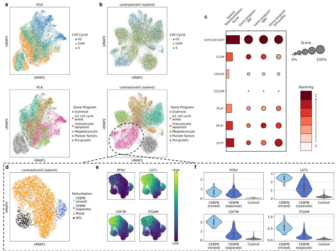
Figure 4.3: Isolating CRISPR-perturbation-induced variations in a large-scale Perturb-Seq experiment with contrastiveVI. a-b , UMAP plots of a standard scRNA-seq analysis workflow consisting of normalization followed by PCA ( a ) and contrastiveVI's salient latent space ( b ) colored by cell cycle stage (top) and induced gene program identified by Norman et al. [127] (bottom). c , Quantitative metrics capturing separation by gene program label in contrastive models' salient latent spaces and non-contrastive models' single latent spaces. (*) denotes non-contrastive baseline methods, for which metrics were computed on the given method's single latent space. Metrics were normalized as done in Figure 4.1. d-f Exploration of the granuloctye/apoptosis subclusters revealed in contrastiveVI's salient latent space. RNA expression values depicted in ( e ) and ( f ) were denoised using contrastiveVI then log library size transformed (Section 4.B). Centers of box plots represent median expression values and upper (lower) box bounds denote the third (first) quartile; upper (lower) whiskers represent third quartile + 1.5×inter-quartile range (first quartile - 1.5×inter-quartile range). Minimum and maximum values denoted by ends of corresponding violin plots. Violin plots depict expression values for CEBPB -perturbed cells ( n = 311 ) that formed a separate cluster in the UMAP plot in ( d ), a group of CEBPB -perturbed cells that mixed with the larger main cluster with other perturbations ( n = 52 ), and control cells ( n = 7,275 ).
