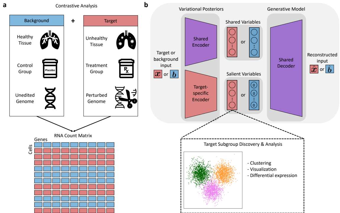
Figure 4.1: Overview of contrastiveVI. Given a reference background dataset and a target dataset of interest, contrastiveVI separates the variations shared between the two datasets and the variations enriched in the target dataset. a , Example background and target data pairs. Samples from both conditions produce an RNA count matrix with each cell labeled as background or target. b , Schematic of the contrastiveVI model. A shared encoder network embeds a cell, whether target (red) or background (blue), into the model's shared latent space, which captures variations common to target and background cells. A second target-cell-specific encoder embeds target cells into the model's salient latent space, which captures variations enriched in the target data and not present in the background. For background cells the values of the salient latent factors are fixed to be a zero vector. Both target and background cells' latent representations are transformed back to the original gene expression space using a single shared decoder network.
