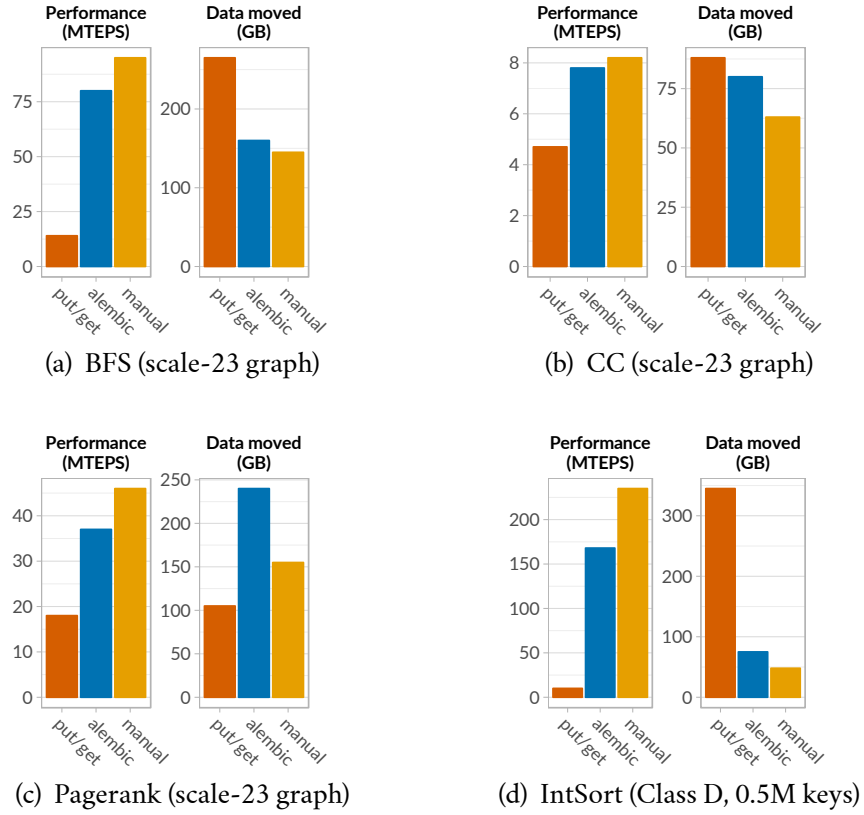
Figure 2.3. Application kernel performance: comparing manually-optimized movement against compiler-generated migration. Experiments were done on 12 nodes with 8 cores per node. Overall, Alembic performs competitively with manually-optimized communication, and significantly better than naive puts and gets. This performance is due in part to reduced data movement, which is also shown. The outlier, Pagerank, is explained in §2.5.1.5.
