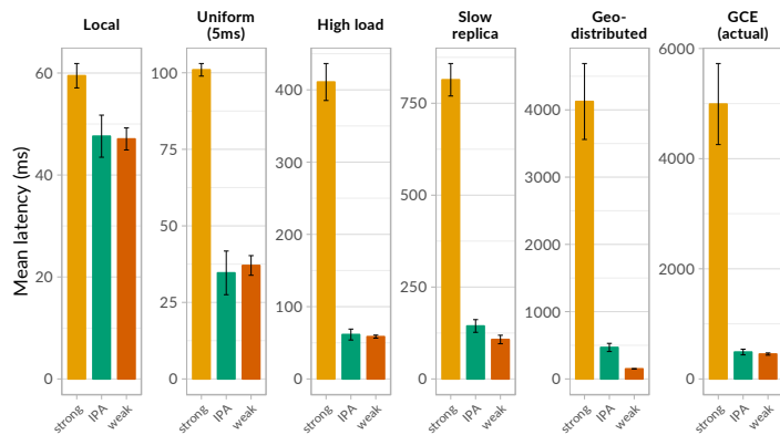
Figure 5.14. Twitter clone: mean latency (all actions). The IPA version performance comparably with weak consistency in all but one case, while strong consistency is 2-10× slower.
