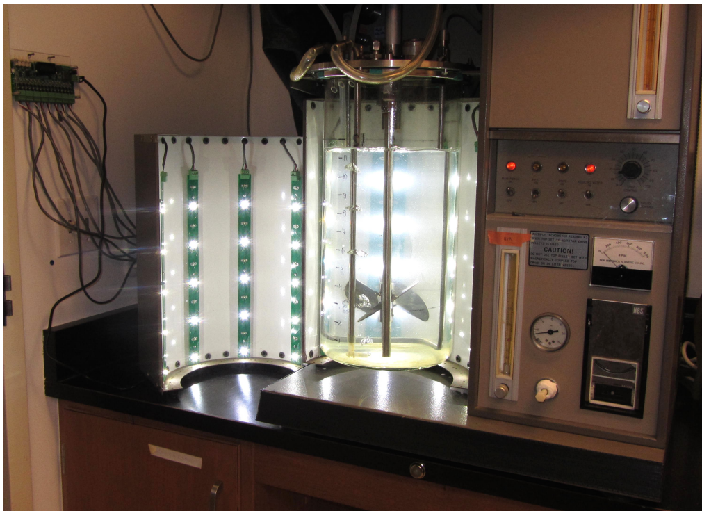
Supplemental figure 1: 15L photobioreactor with LED lighting.
