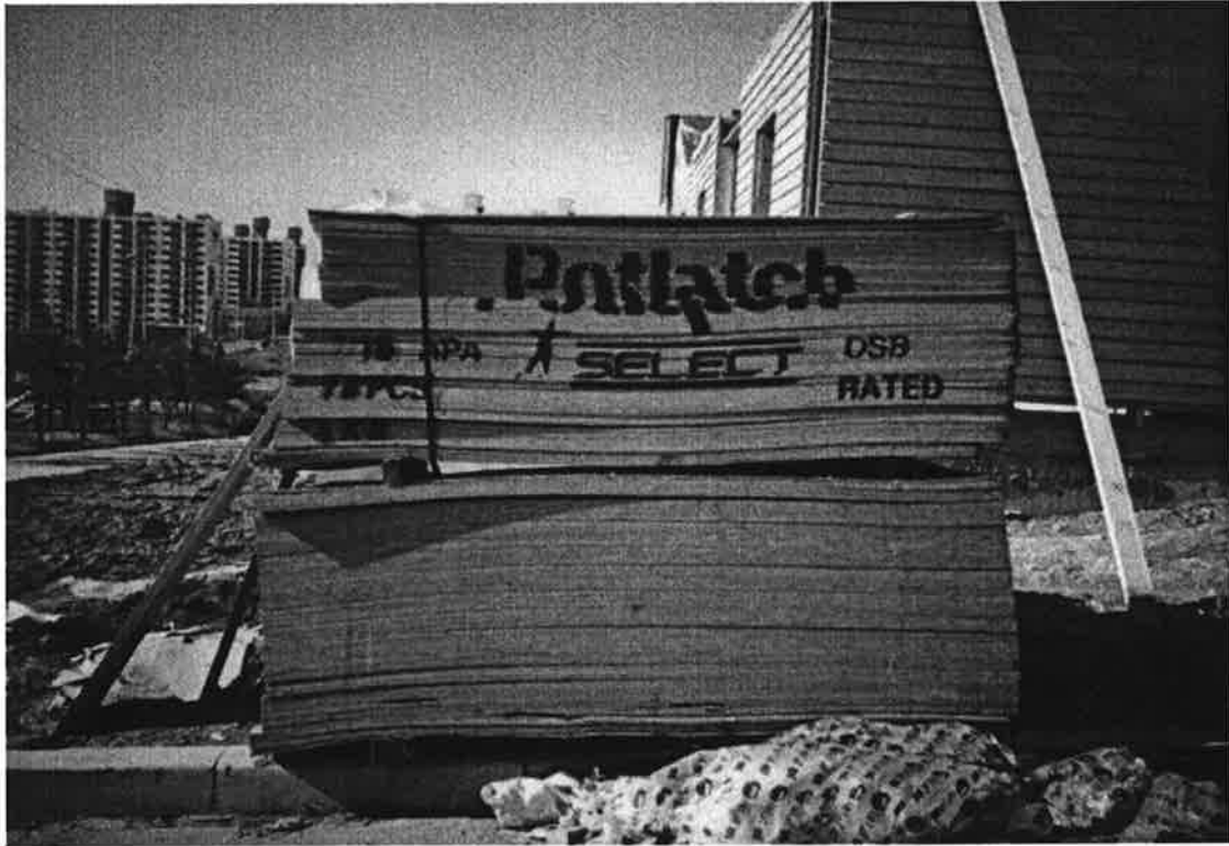
Figure 26. Improper site storage of OSB panels.
